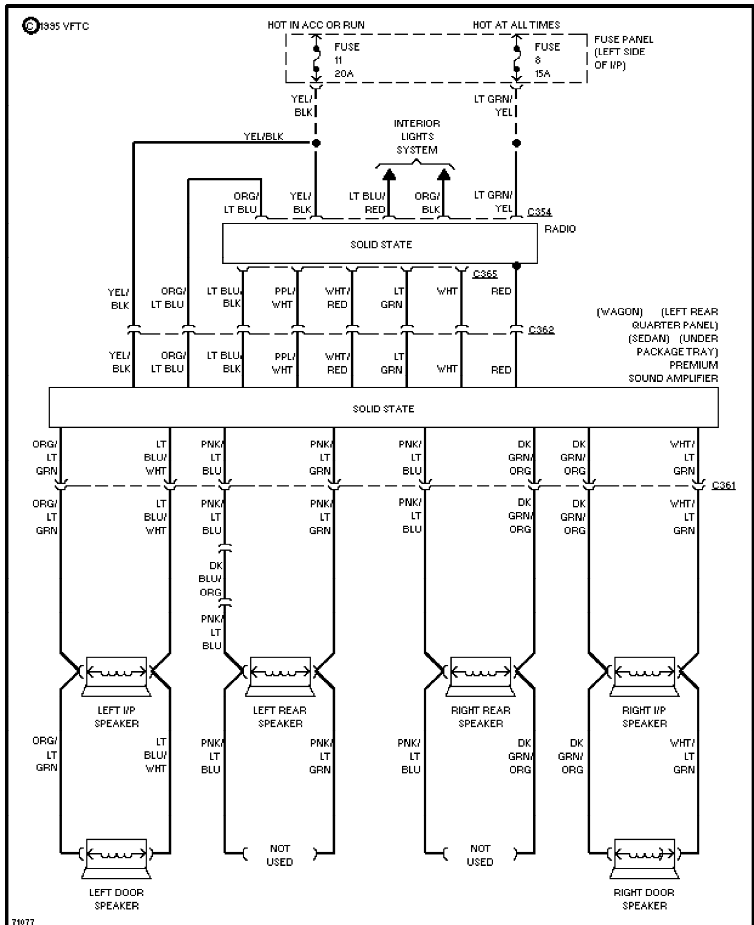
Fig. 14: Premium Sound Radio Circuit, Standard/AAY 1989 Ford Taurus LX
