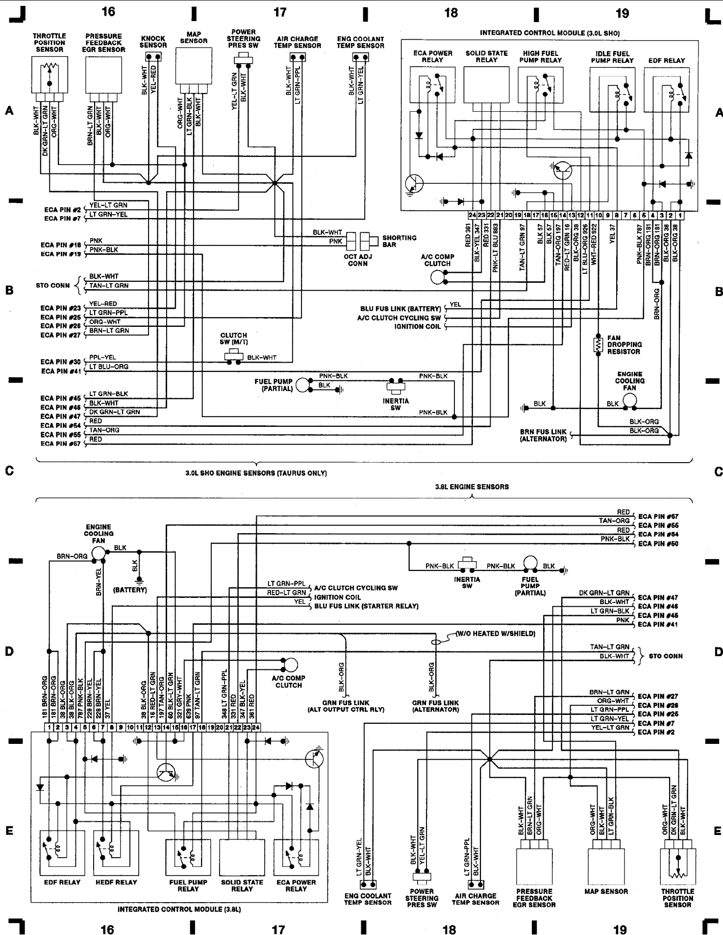
Fig. 5: Engine Control Sensors 1989 Ford Taurus LX
