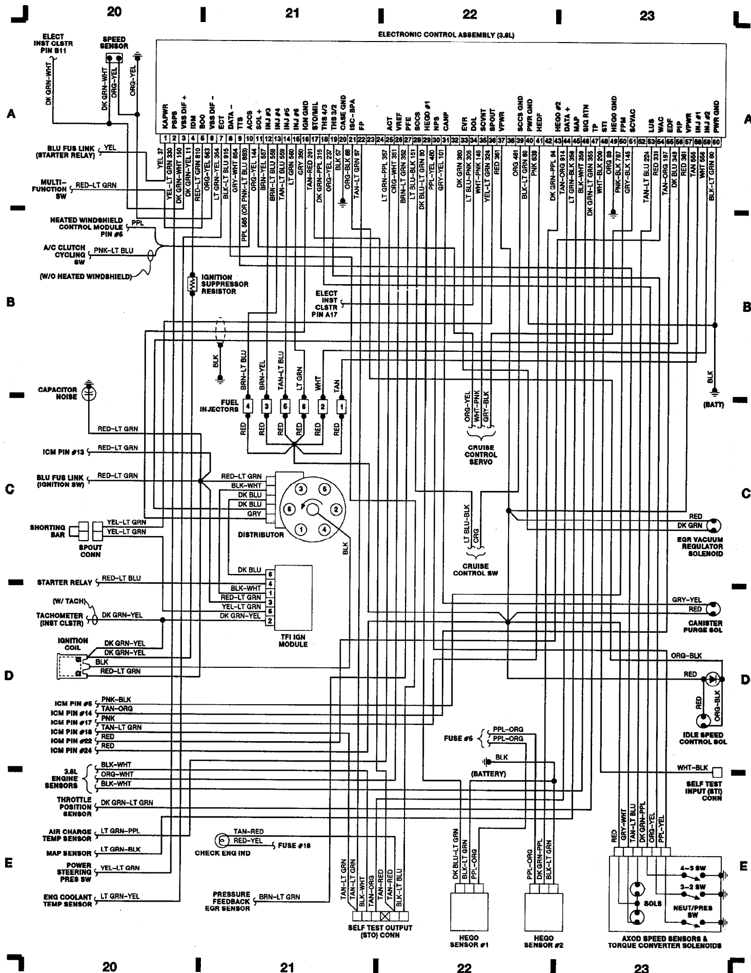
Fig. 6: Computer Engine Control (3.8L) 1989 Ford Taurus LX
