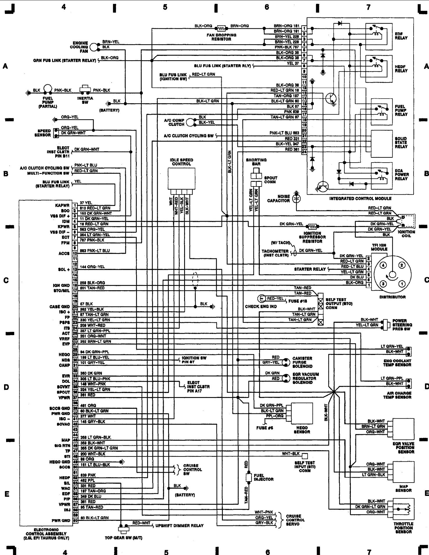
Fig. 2: Computer Engine Control (2.5L) 1989 Ford Taurus LX
