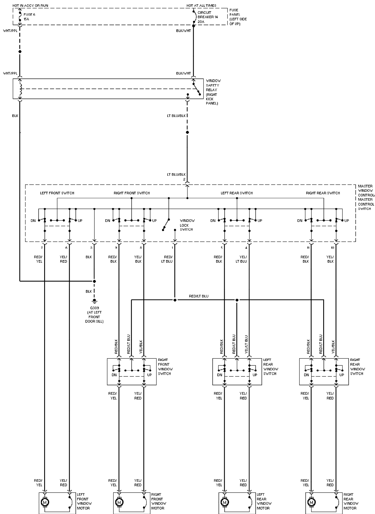
Fig. 13: Power Window Circuit 1989 Ford Taurus LX
