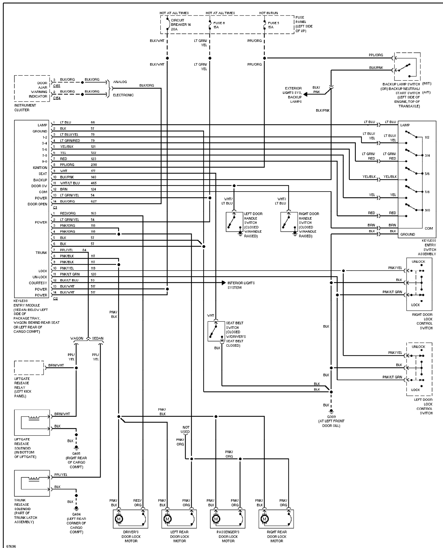
Fig. 9: Keyless Entry Circuit 1989 Ford Taurus LX
