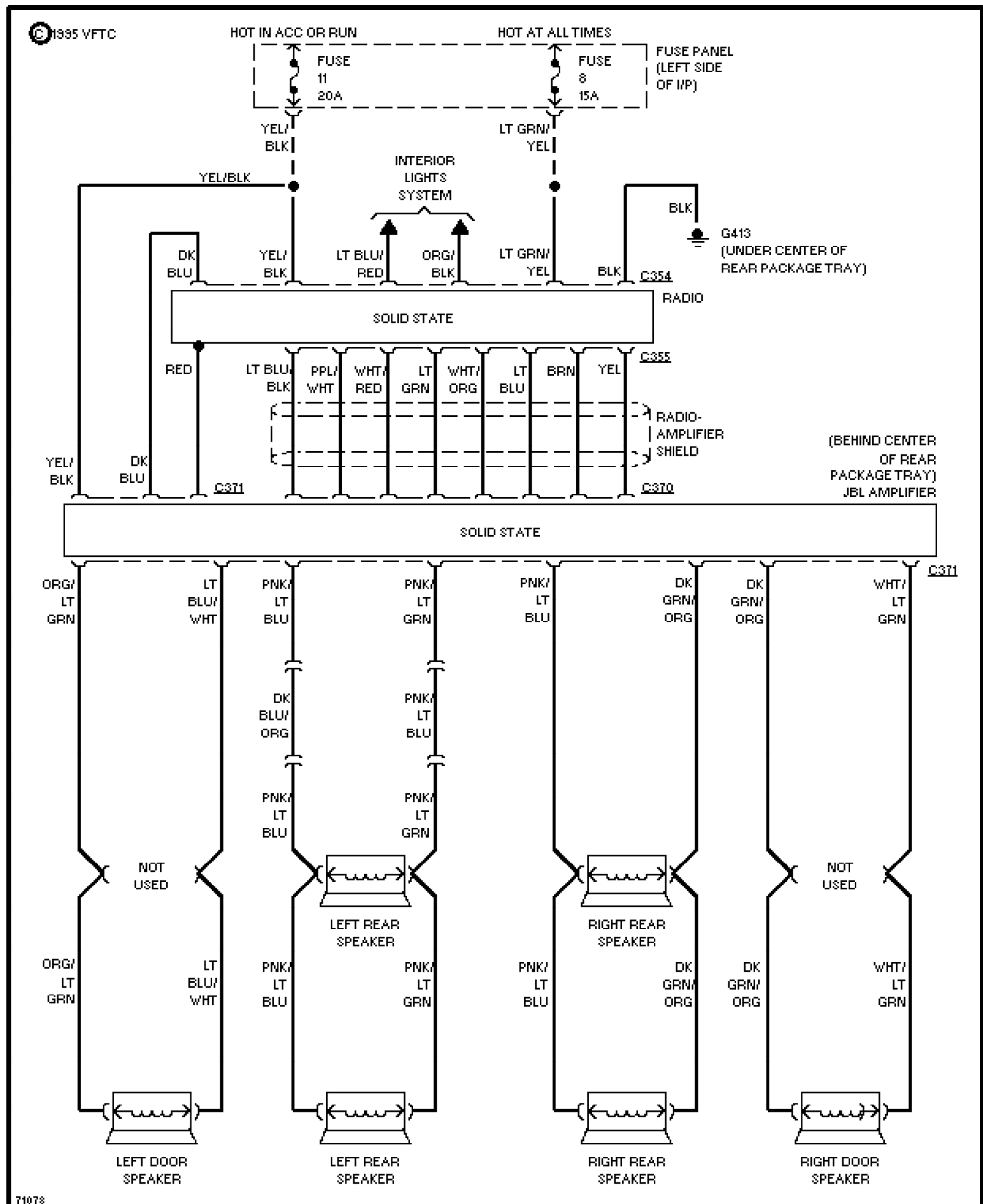
Fig. 15: Premium Sound Radio Circuit, W/ EPC/JBL 1989 Ford Taurus LX
