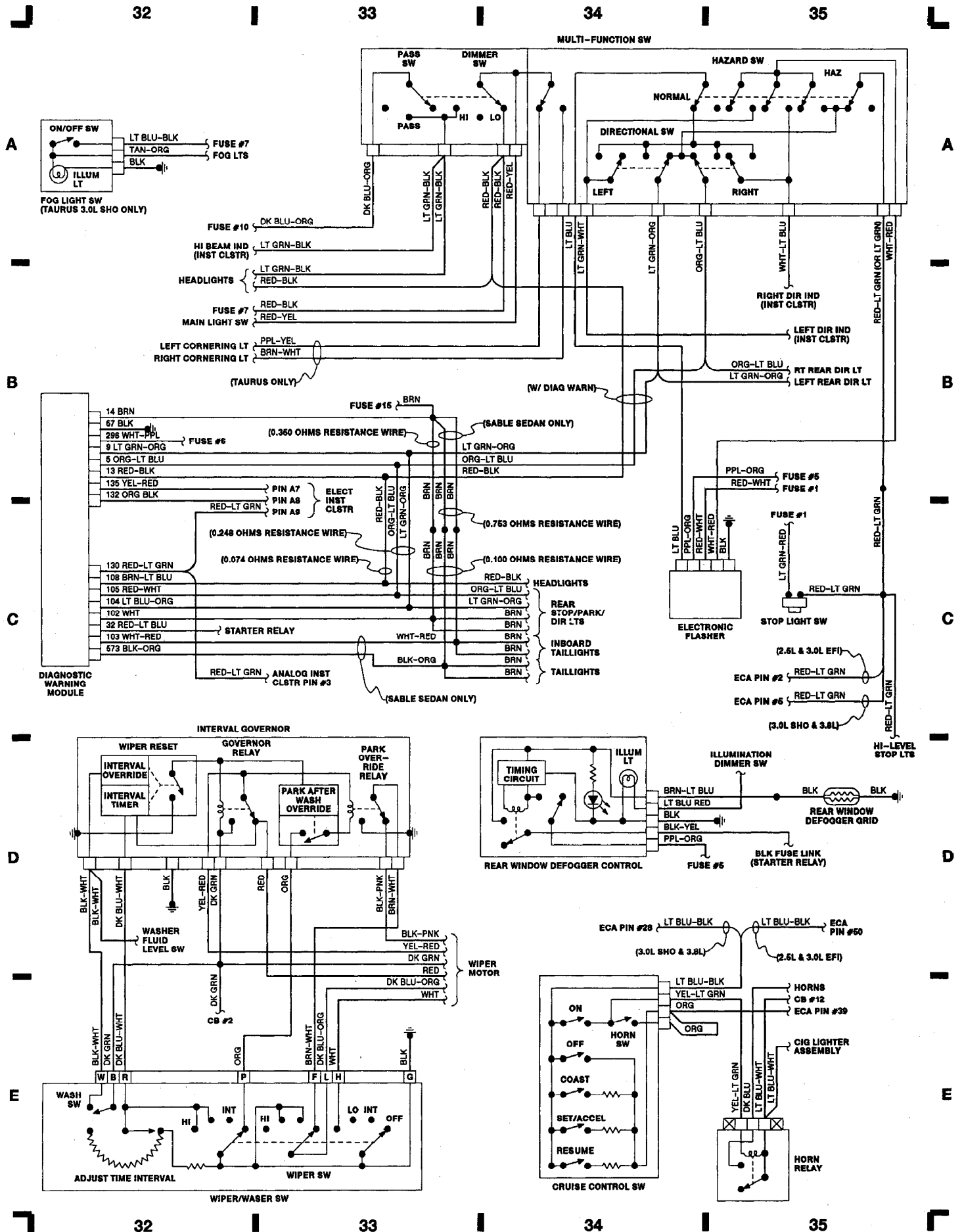
Fig. 9: Multi-Function Switch, Wiper/Washer System & Diagnostic Module 1989 Ford Taurus LX
