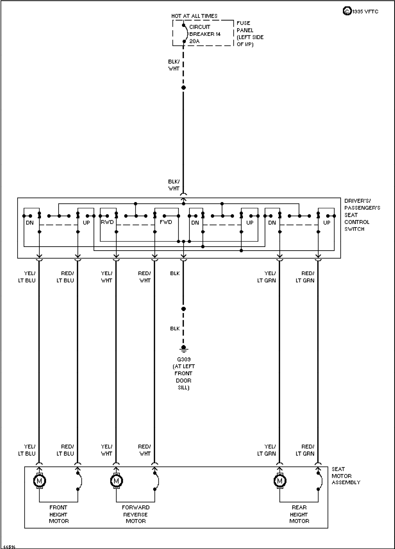
Fig. 12: Power Seat Circuit 1989 Ford Taurus LX
