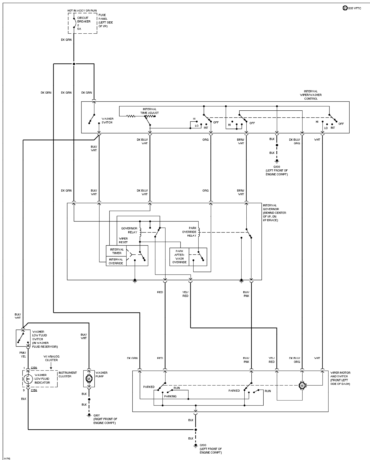
Fig. 27: Interval Wiper/Washer Circuit 1989 Ford Taurus LX
