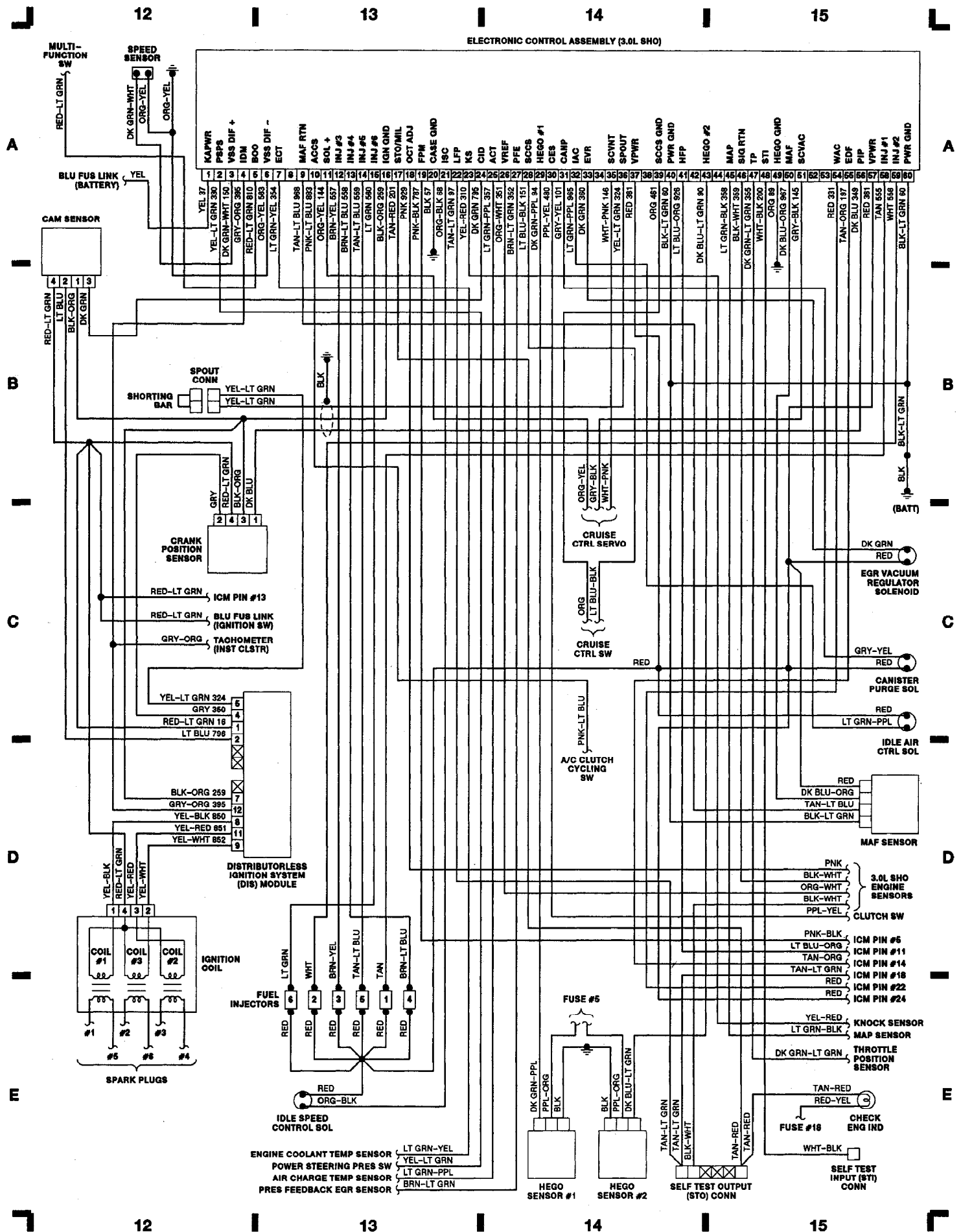
Fig. 4: Computer Engine Control (3.0L SHO) 1989 Ford Taurus LX
