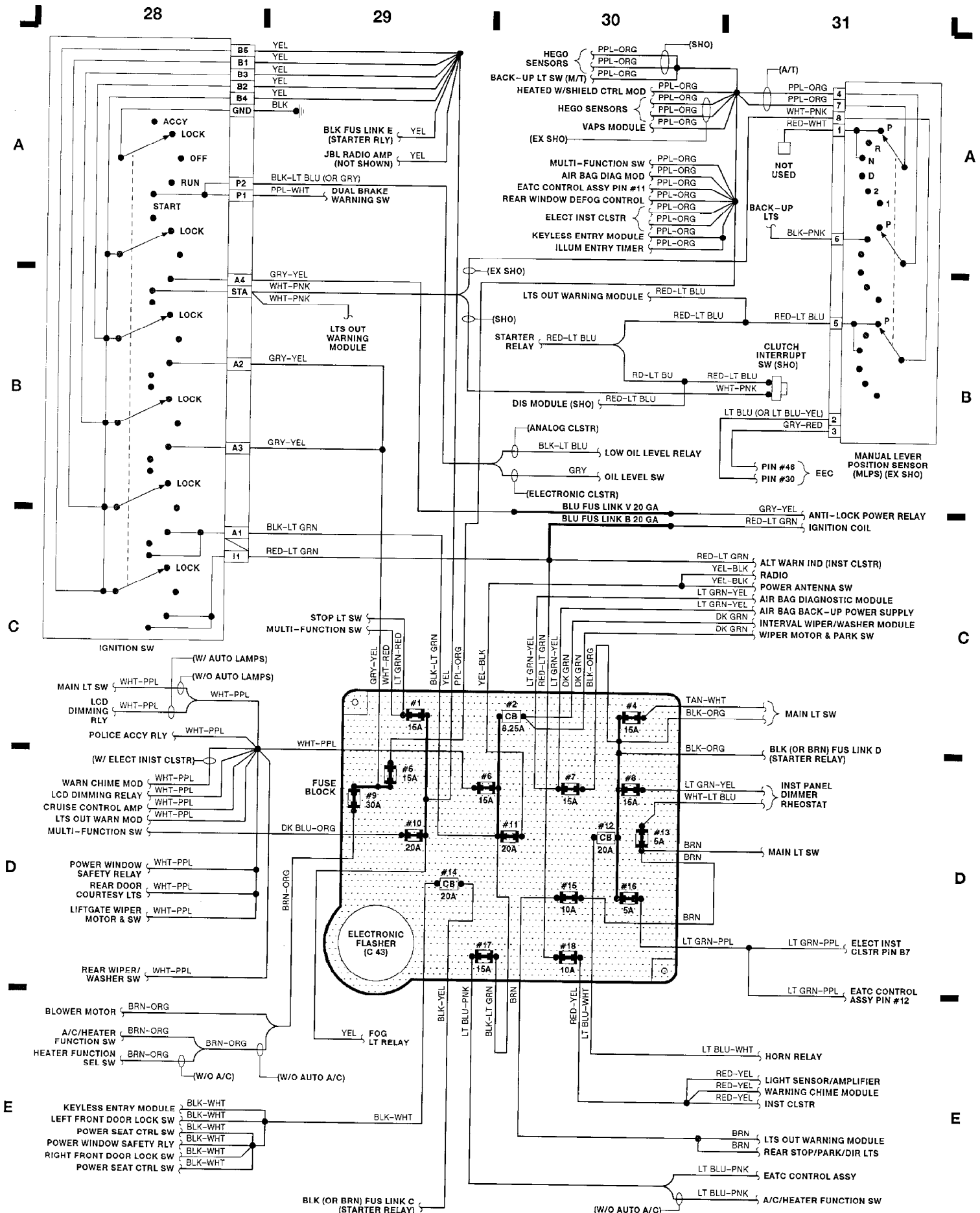
Fig. 8: Fuse Block, Ignition Switch, MLPS (Grid 28-31) 1991 Ford Taurus LX
