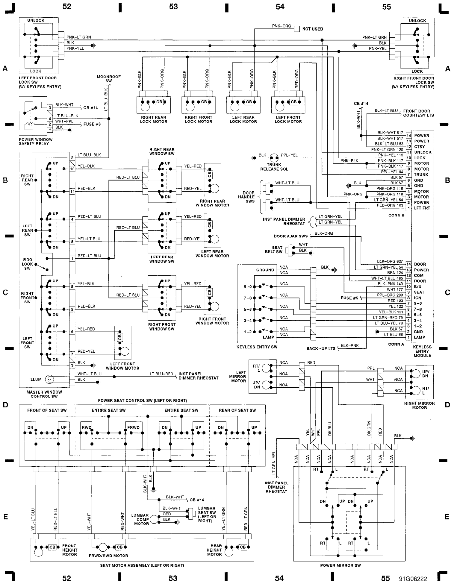
Fig. 14: Keyless Entry, Power Seat/Window (Grid 52-55) 1991 Ford Taurus LX
