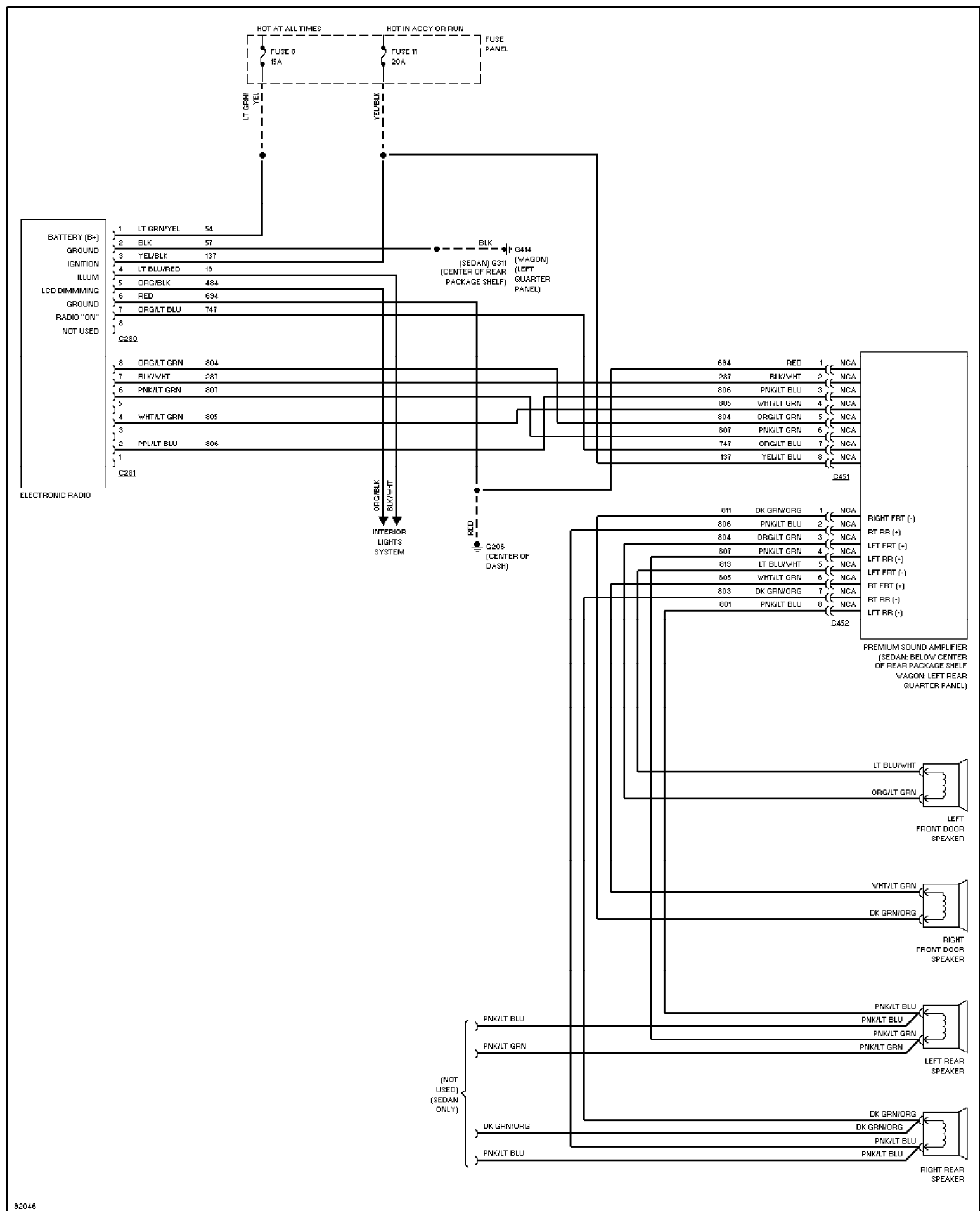
Fig. 16: Radio Circuits, Premium Radio 1991 Ford Taurus LX
