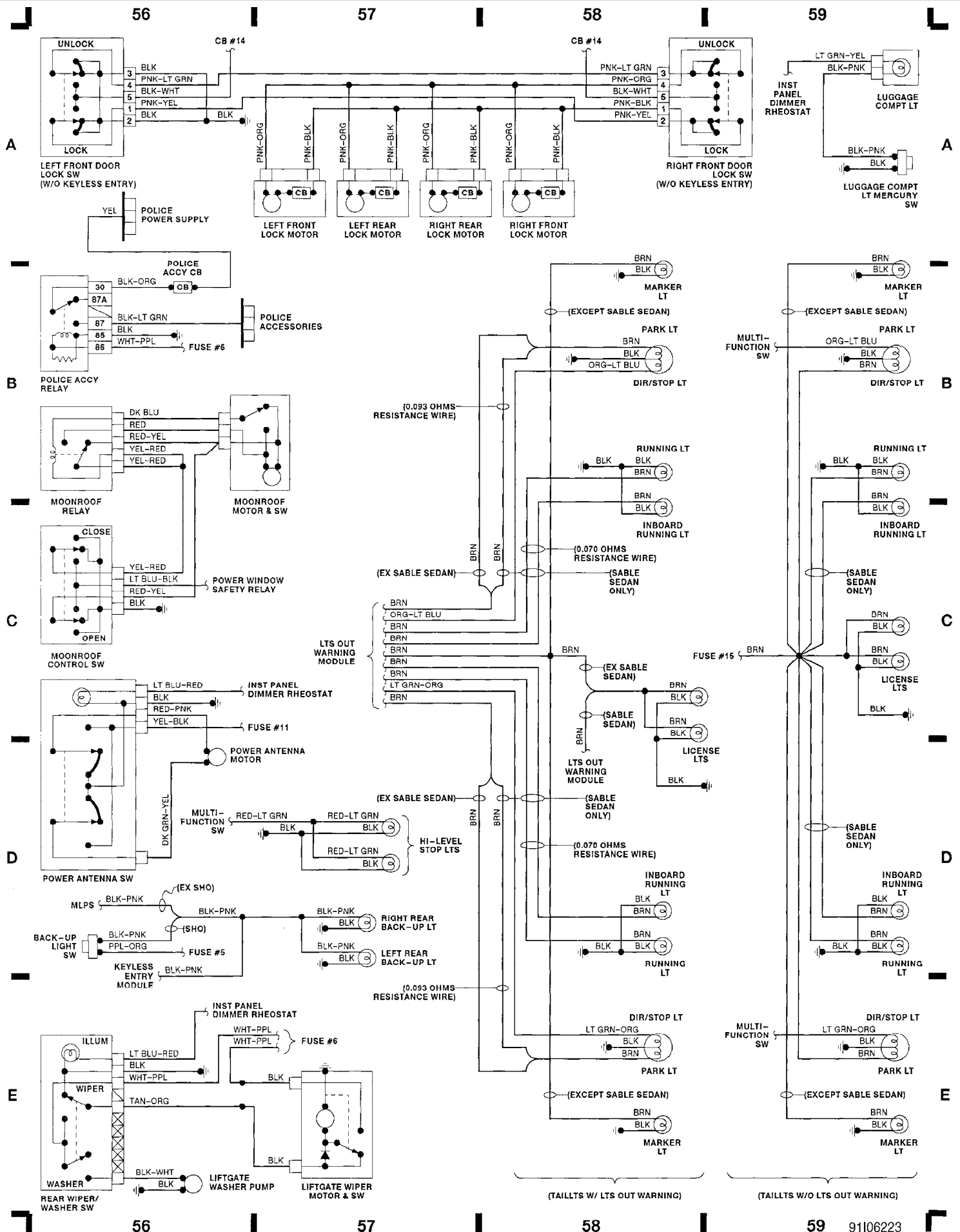
Fig. 15: Power Doors (W/O Keyless), Taillights (Grid 56-59)
