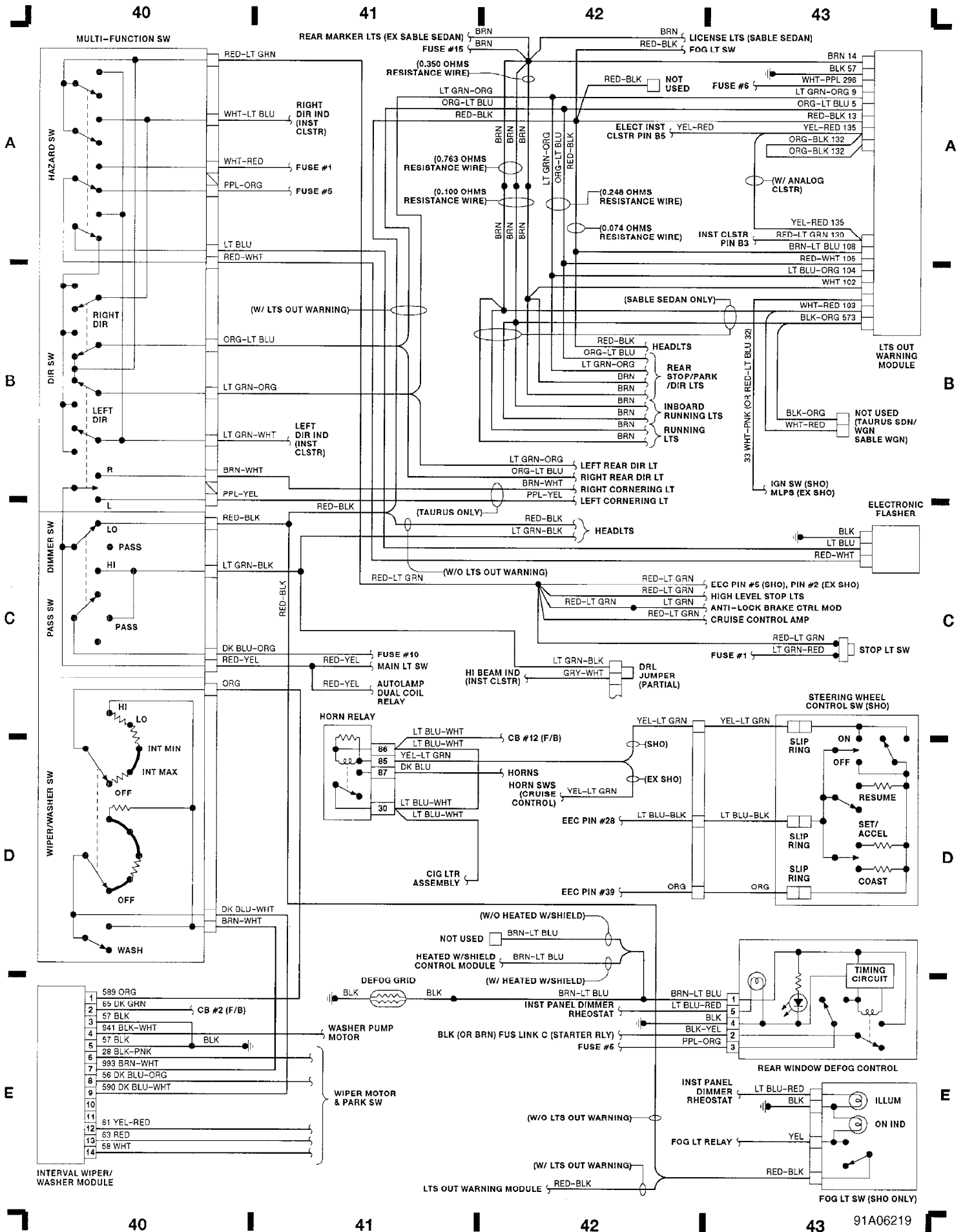
Fig. 11: Multi-Function Sw, Steering Wheel Ctrl Sw (Grid 40-43)
