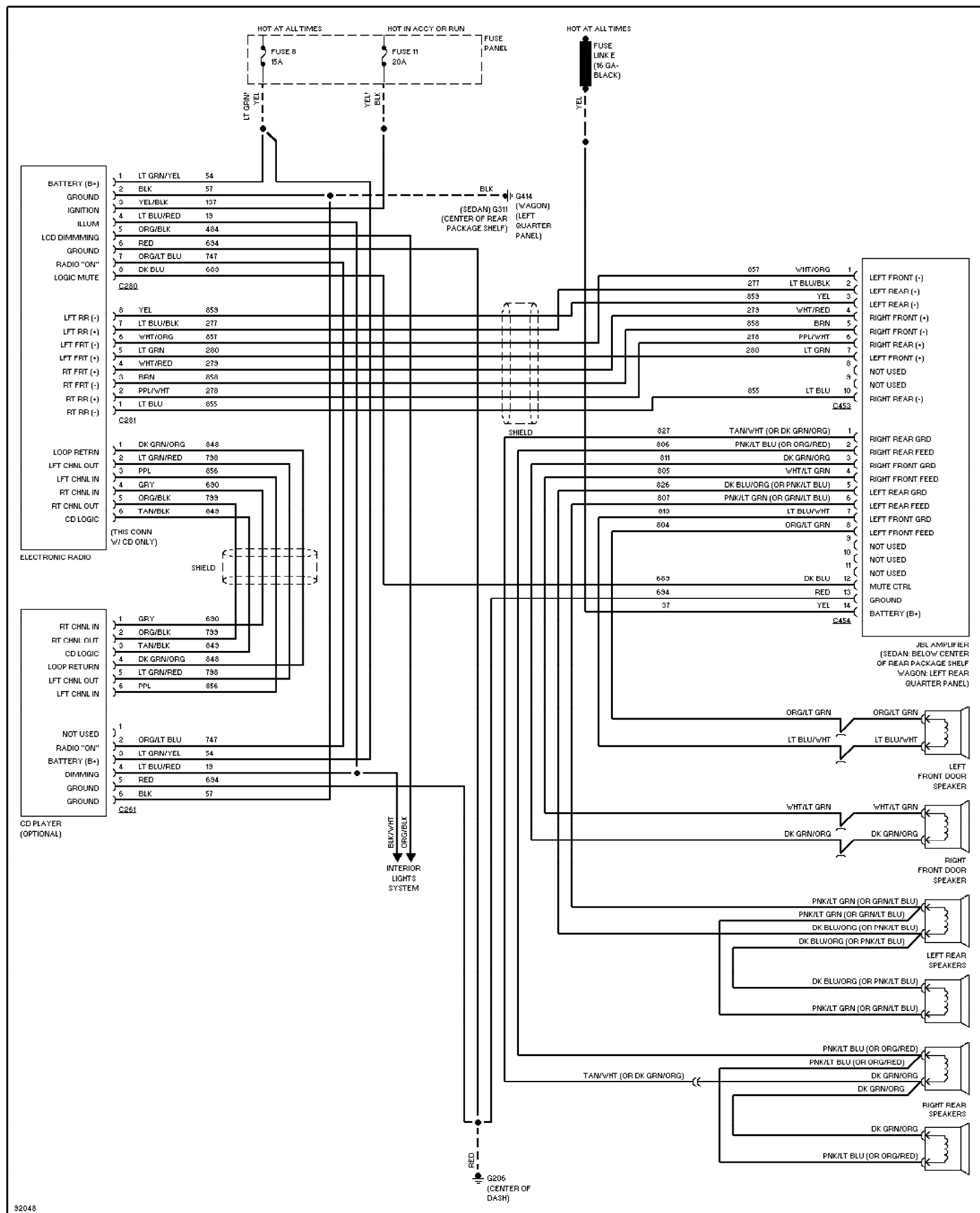
Fig. 15: Radio Circuits, JBL System 1991 Ford Taurus LX
