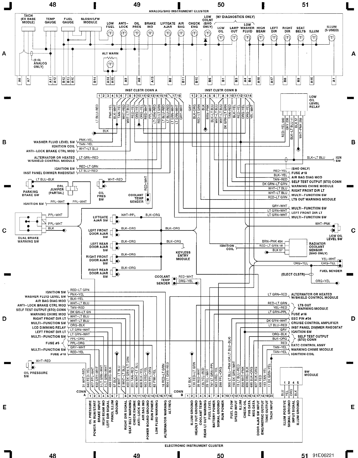
Fig. 13: Instrument Clusters (Grid 48-51) 1991 Ford Taurus LX
