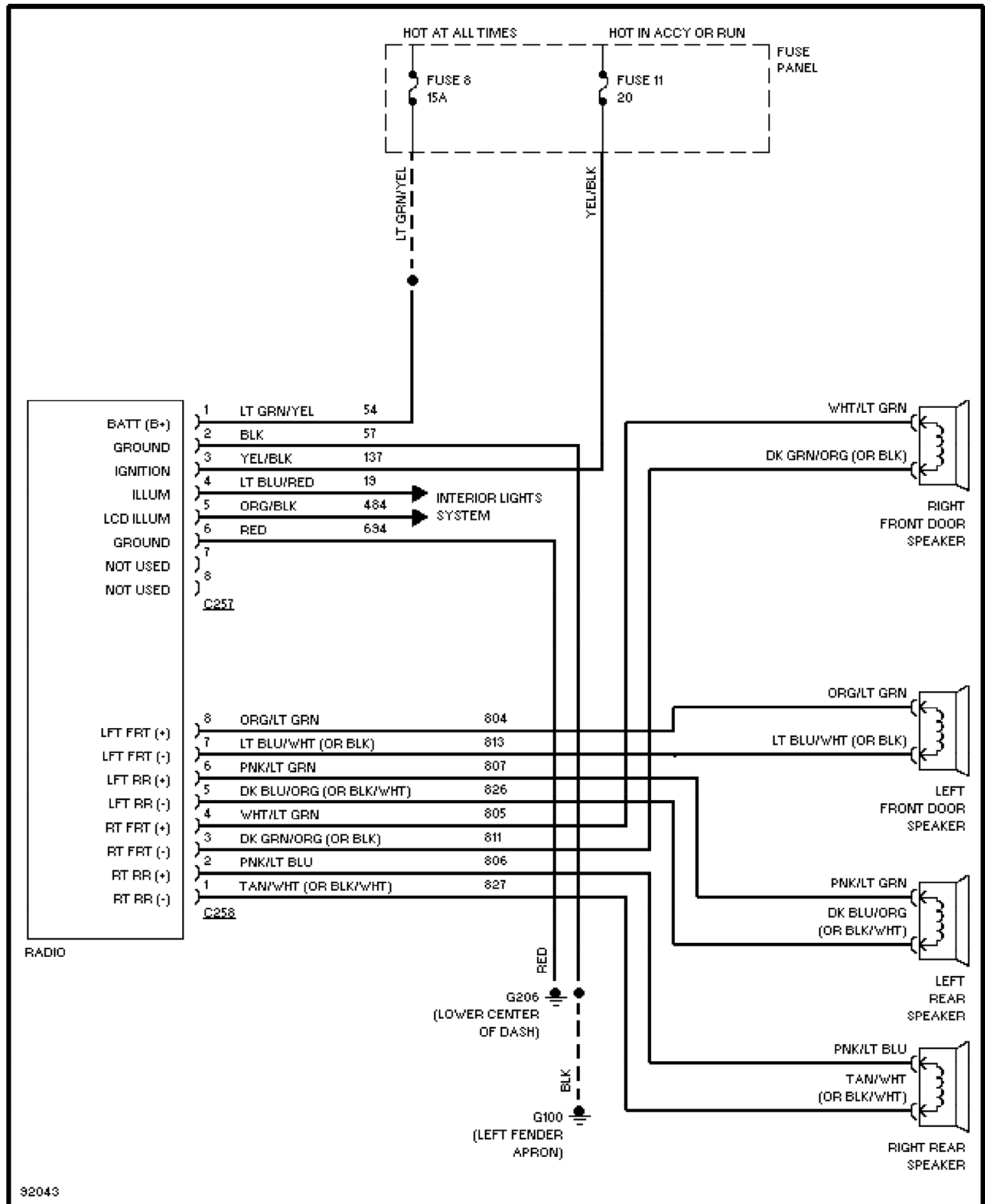
Fig. 14: Radio Circuits 1991 Ford Taurus LX
