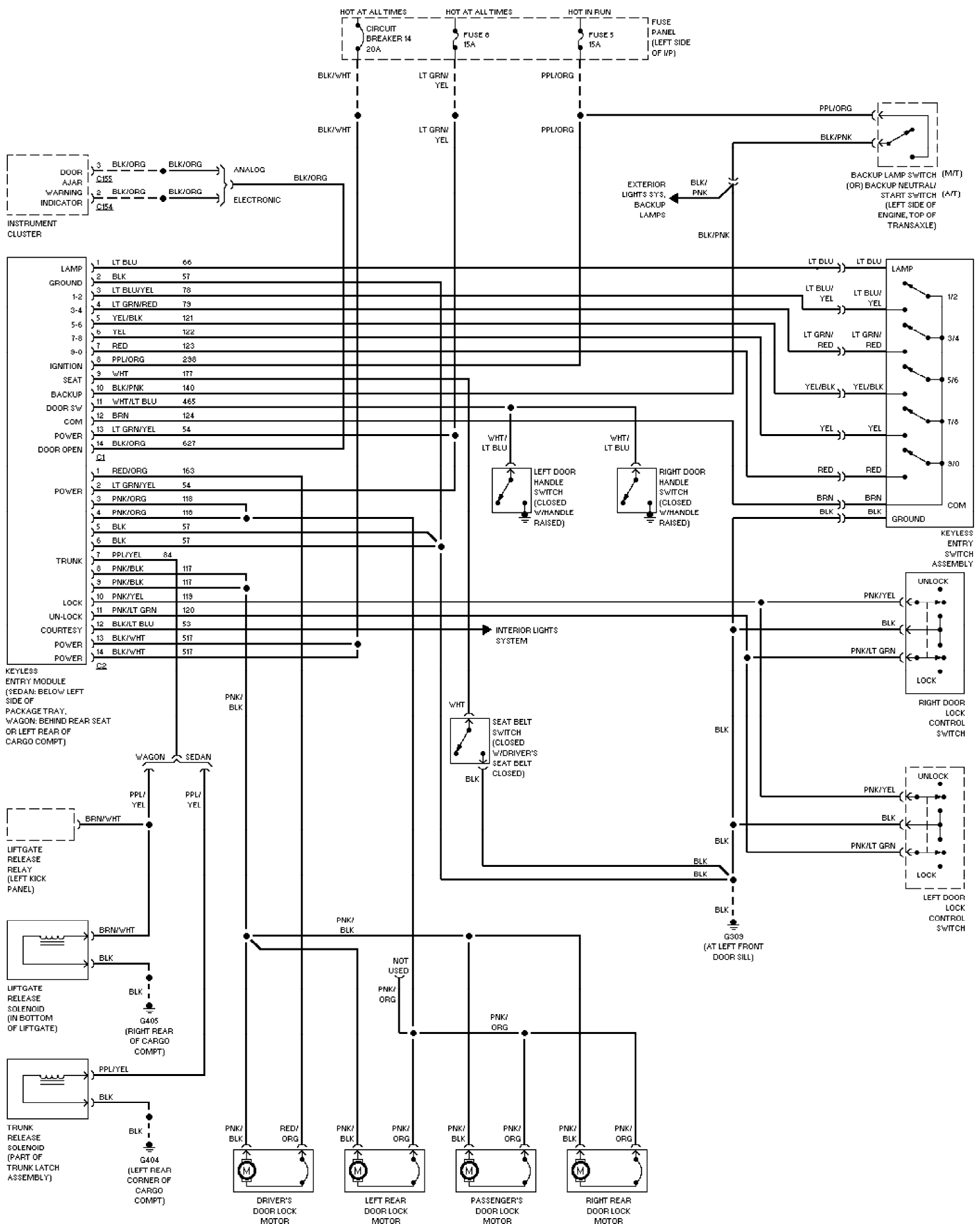
Fig. 9: Keyless Entry Circuit 1991 Ford Taurus LX
