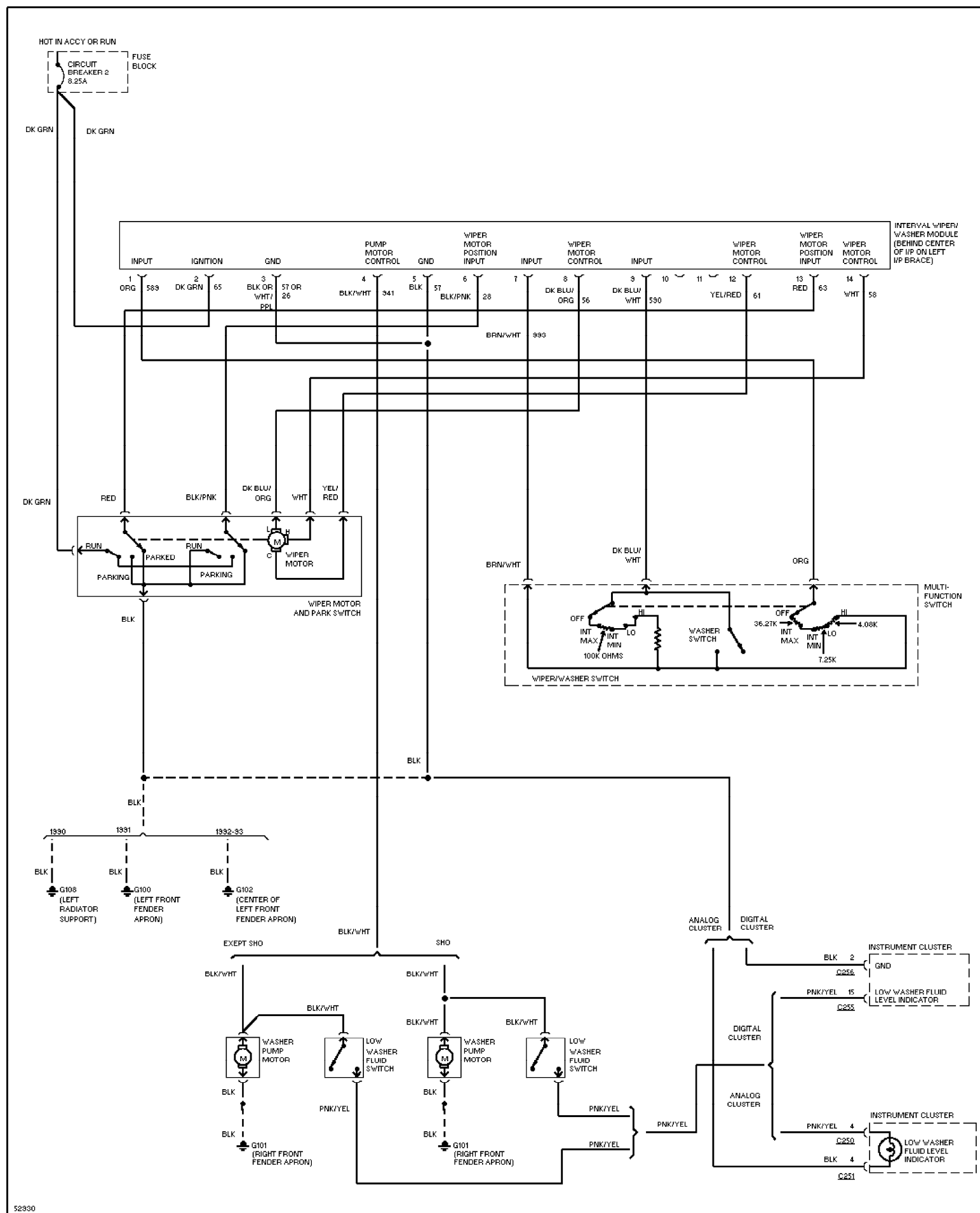
Fig. 21: Interval Wiper/Washer Circuit 1991 Ford Taurus LX
