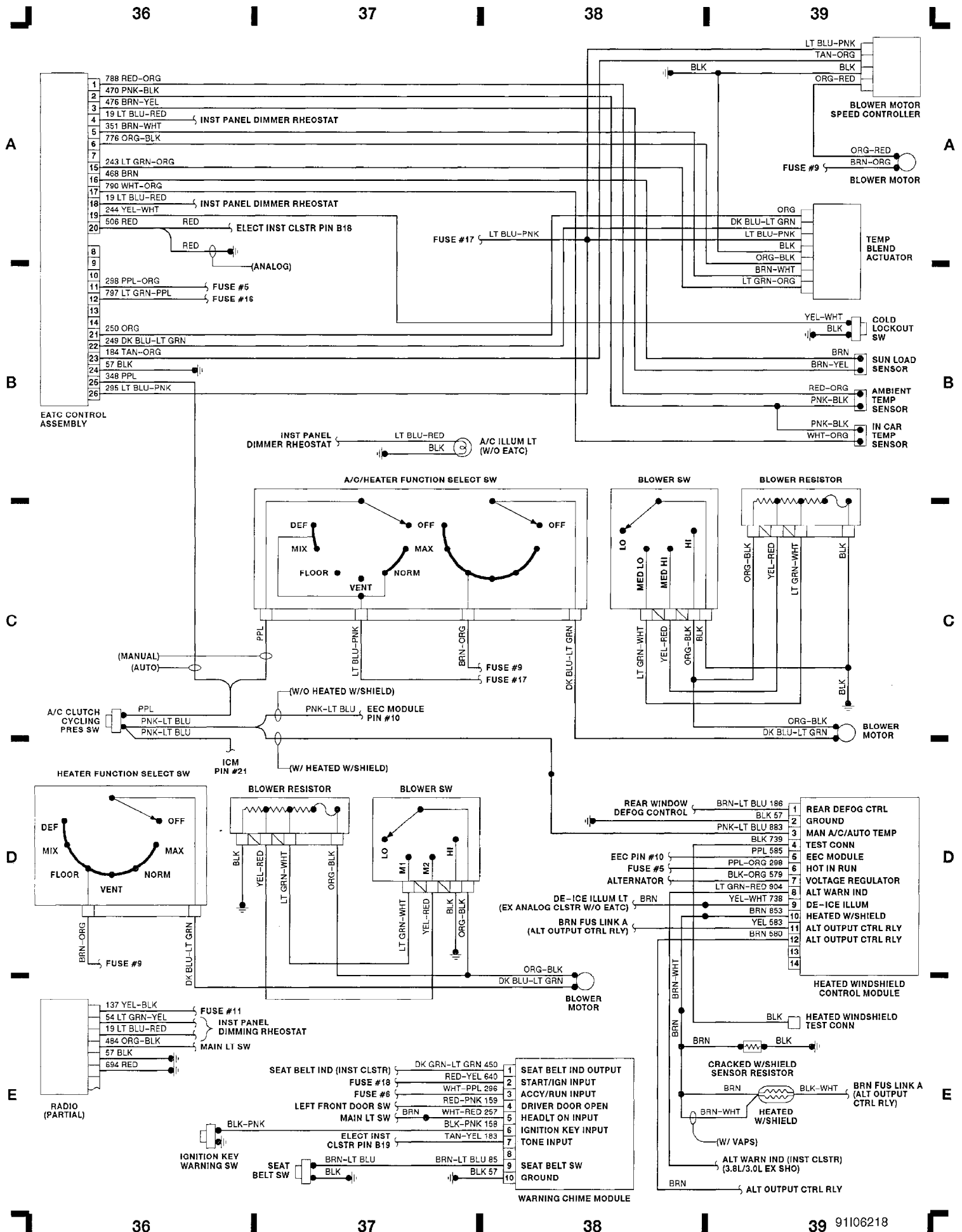
Fig. 10: EATC, A/C/Heater (Grid 36-39) 1991 Ford Taurus LX
