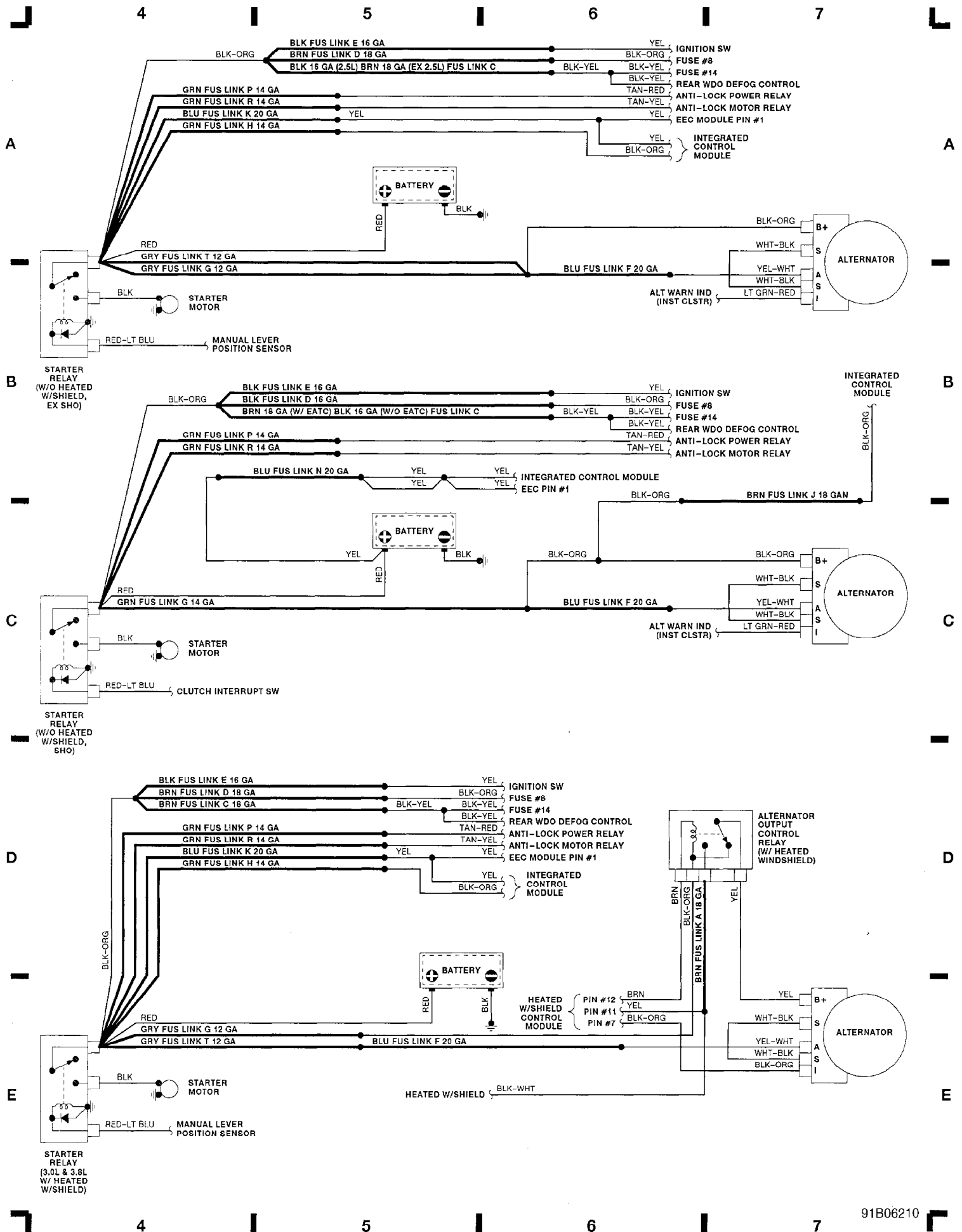
Fig. 2: Engine Compartment (Grid 4-7) 1991 Ford Taurus LX
