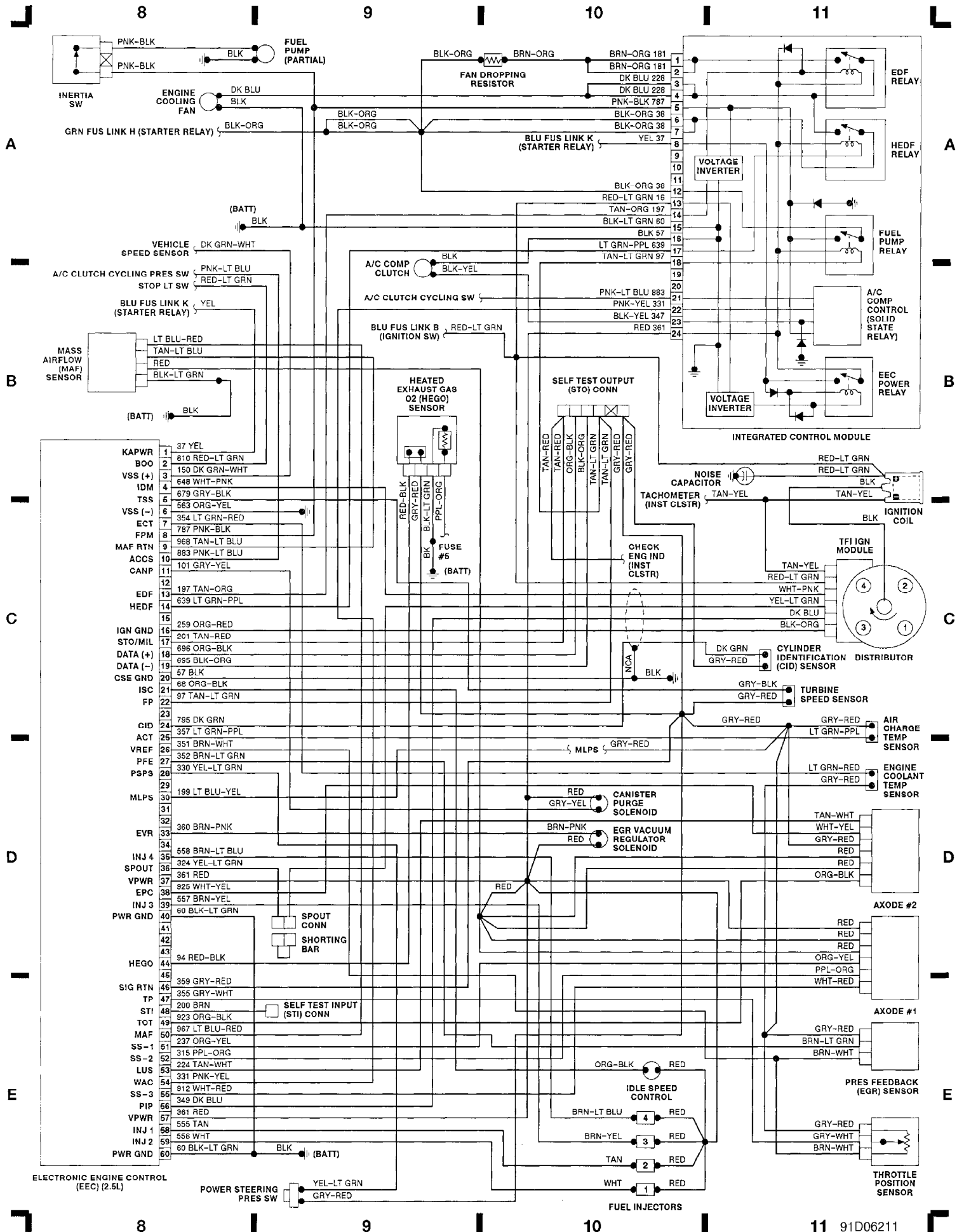
Fig. 3: Elect Engine Control (2.5L) (Grid 8-11) 1991 Ford Taurus LX
