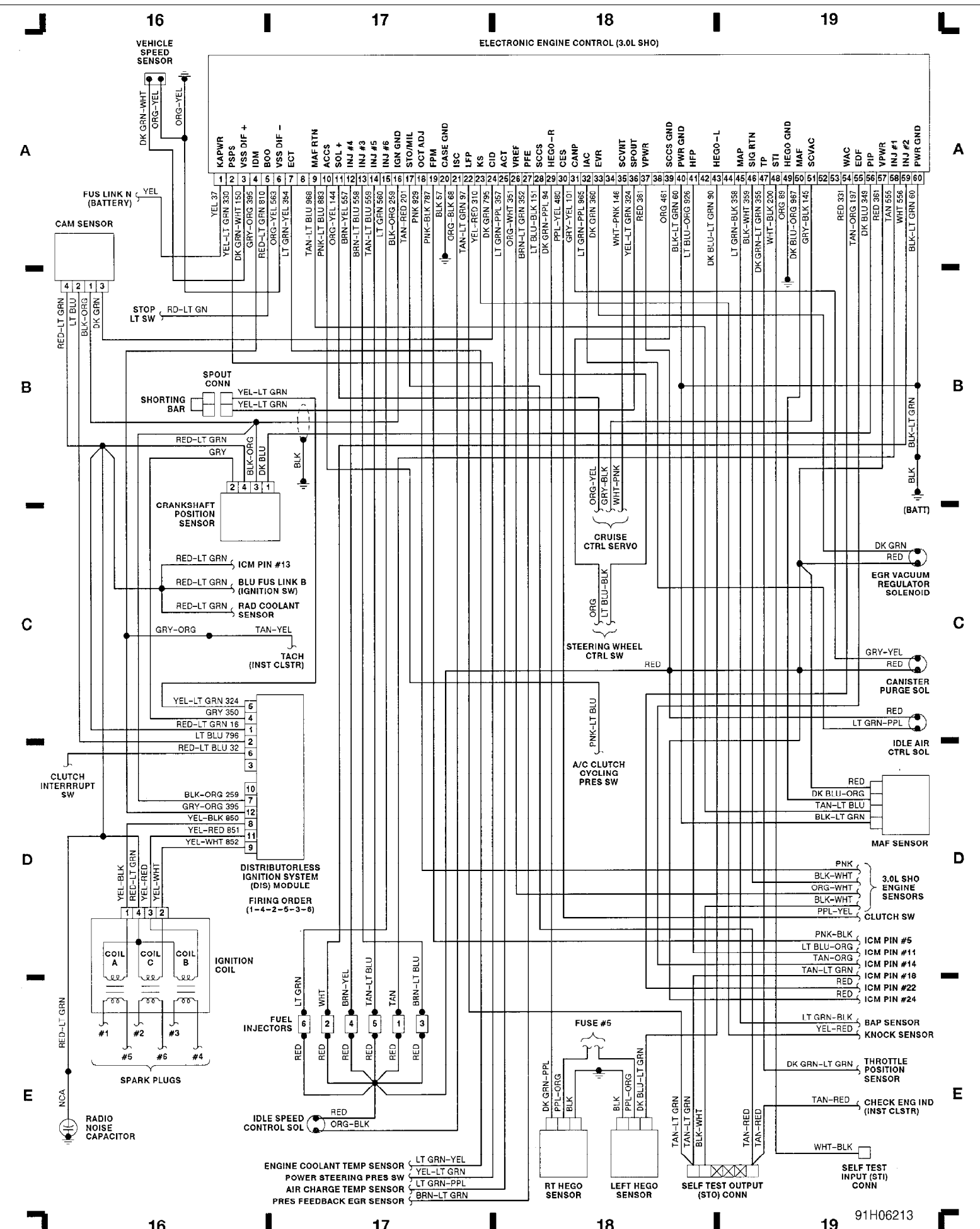
Fig. 5: Elect Engine Control (3.0L SHO) (Grid 16-19) 1991 Ford Taurus LX
