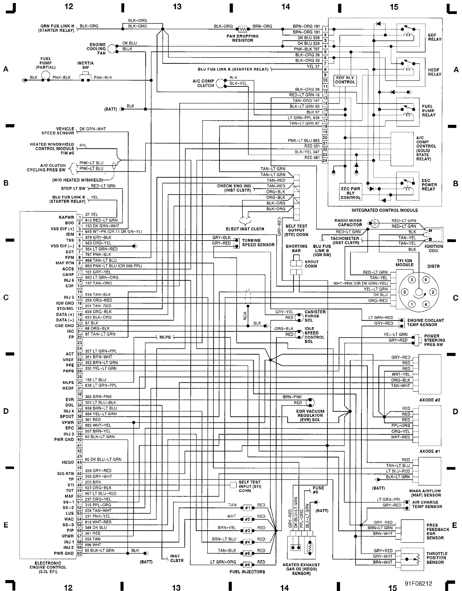
Fig. 4: Elect Engine Control (3.0L EFI) (Grid 12-15) 1991 Ford Taurus LX
