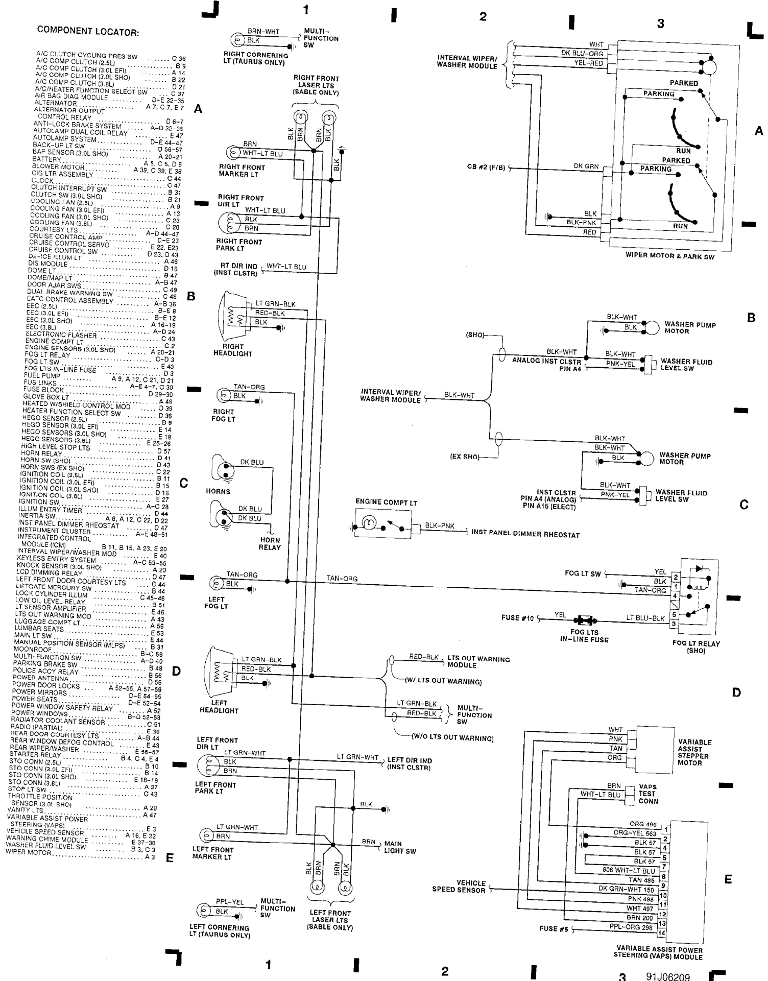
Fig. 1: Headlights & Washer/Wiper, VAPS (Grid 1-3) 1991 Ford Taurus LX
