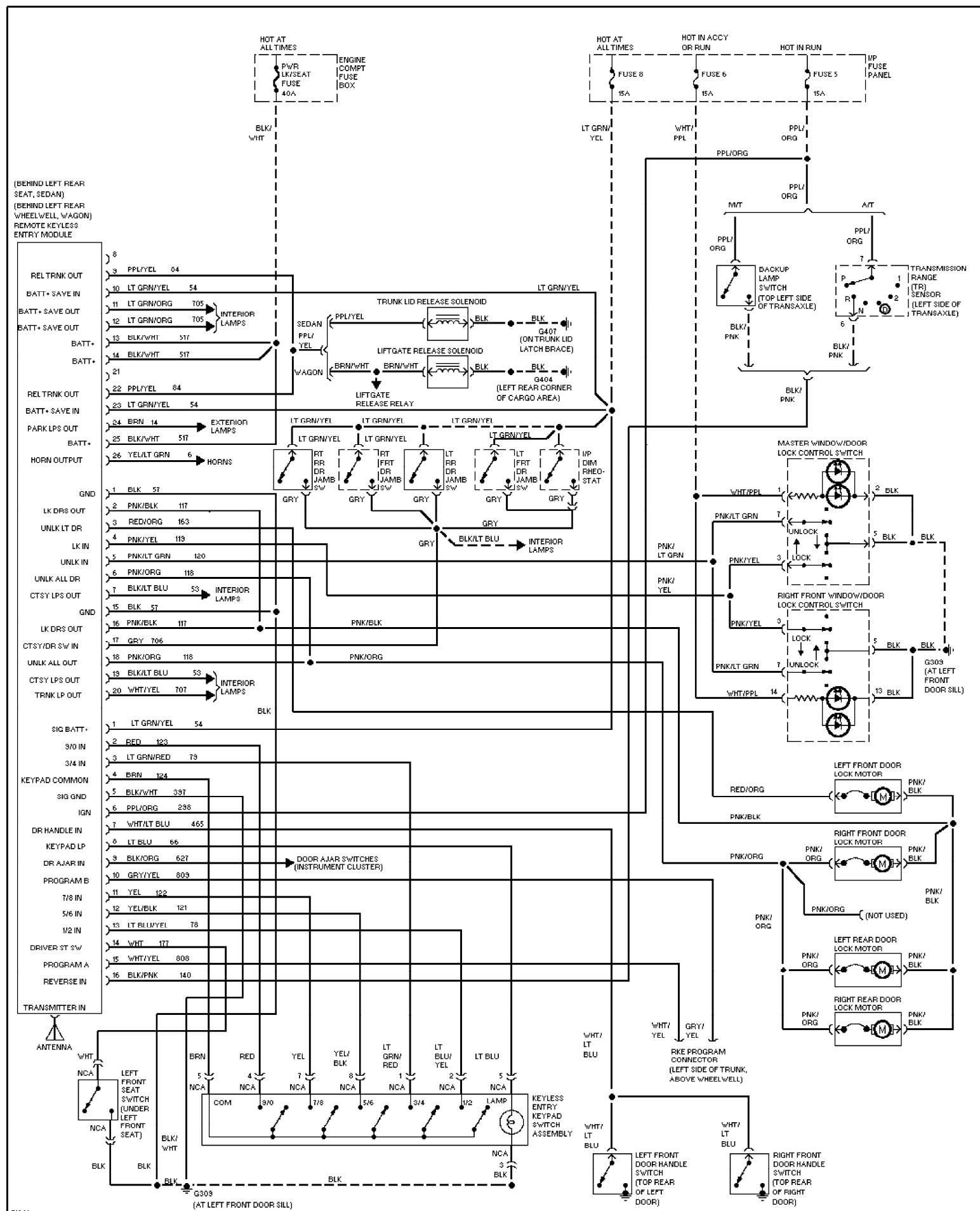
Fig. 91: Keyless Entry Circuit 1995 Ford Taurus LX
