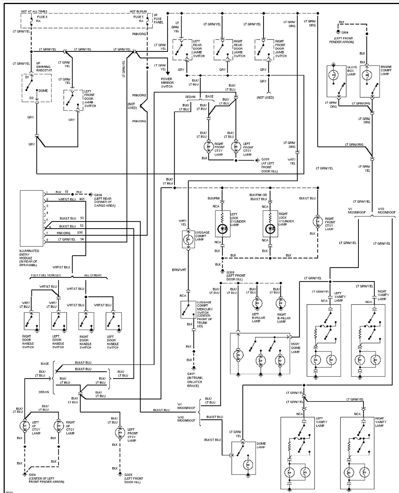
Fig. 79: Courtesy Lamps Circuit, Sedan W/O Remote/Keyless Entry 1995 Ford Taurus LX
