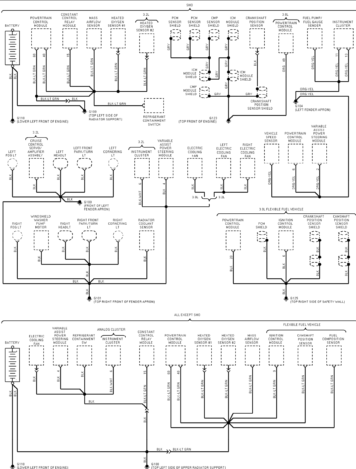
Fig. 46: Ground Distribution Circuit (1 of 5) 1995 Ford Taurus LX
