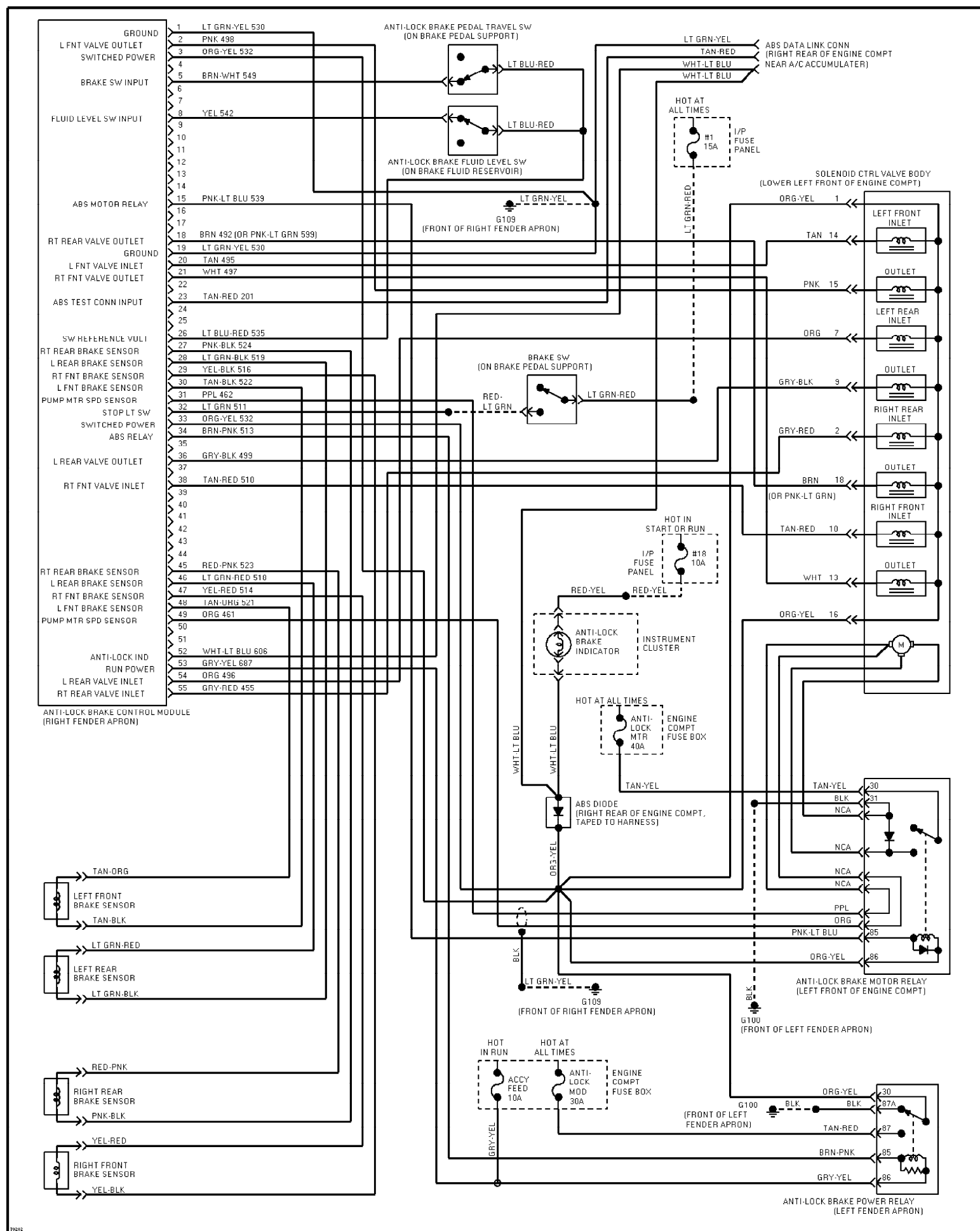
Fig. 15: 3.8L, Anti-lock Brake Circuits 1995 Ford Taurus LX
