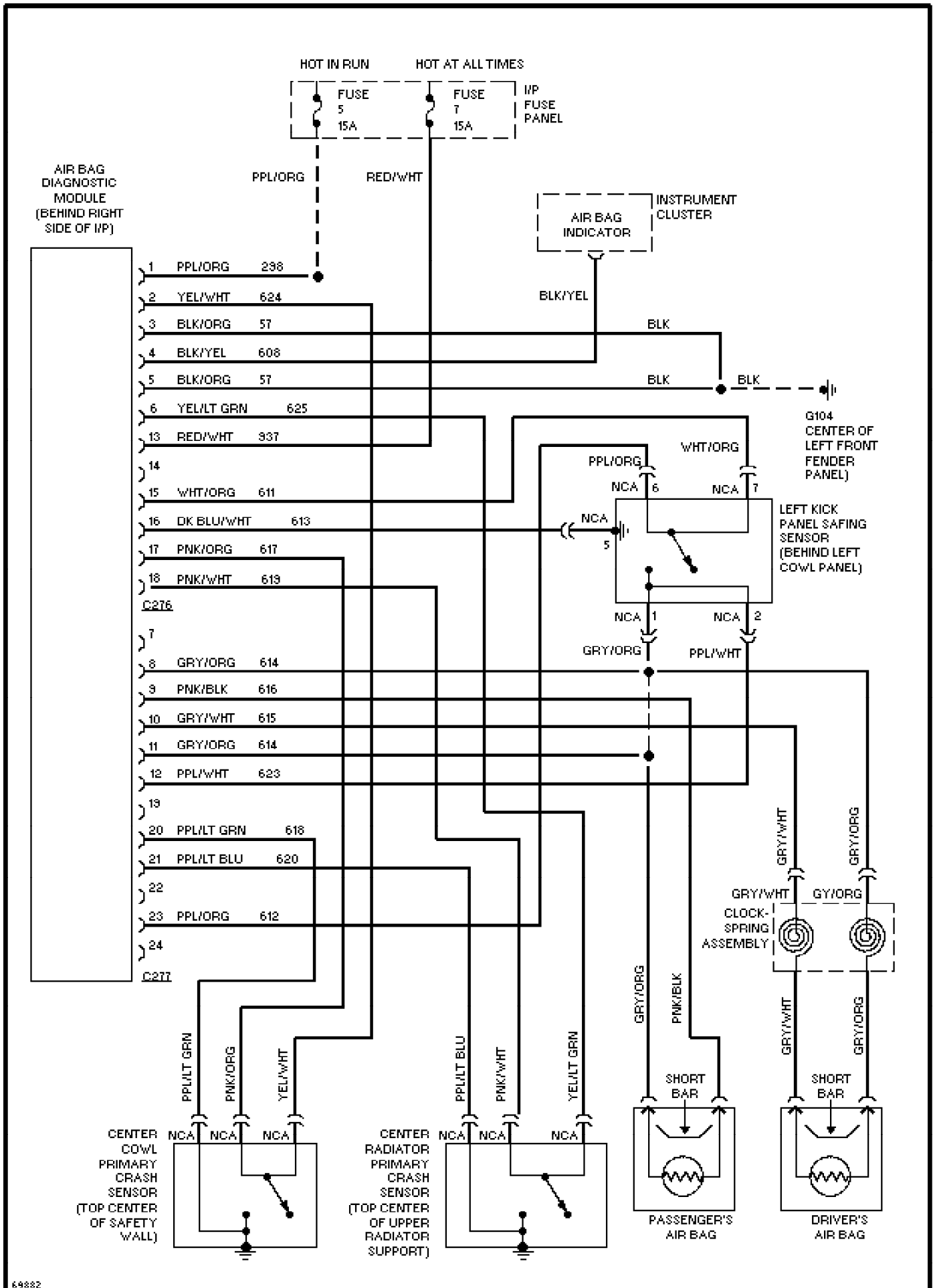
Fig. 110: Supplemental Restraint Circuit 1995 Ford Taurus LX
