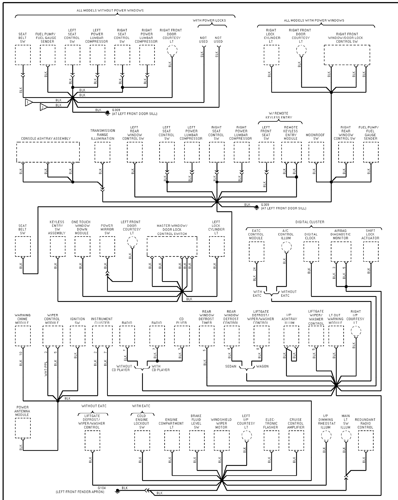
Fig. 48: Ground Distribution Circuit (3 of 5) 1995 Ford Taurus LX
