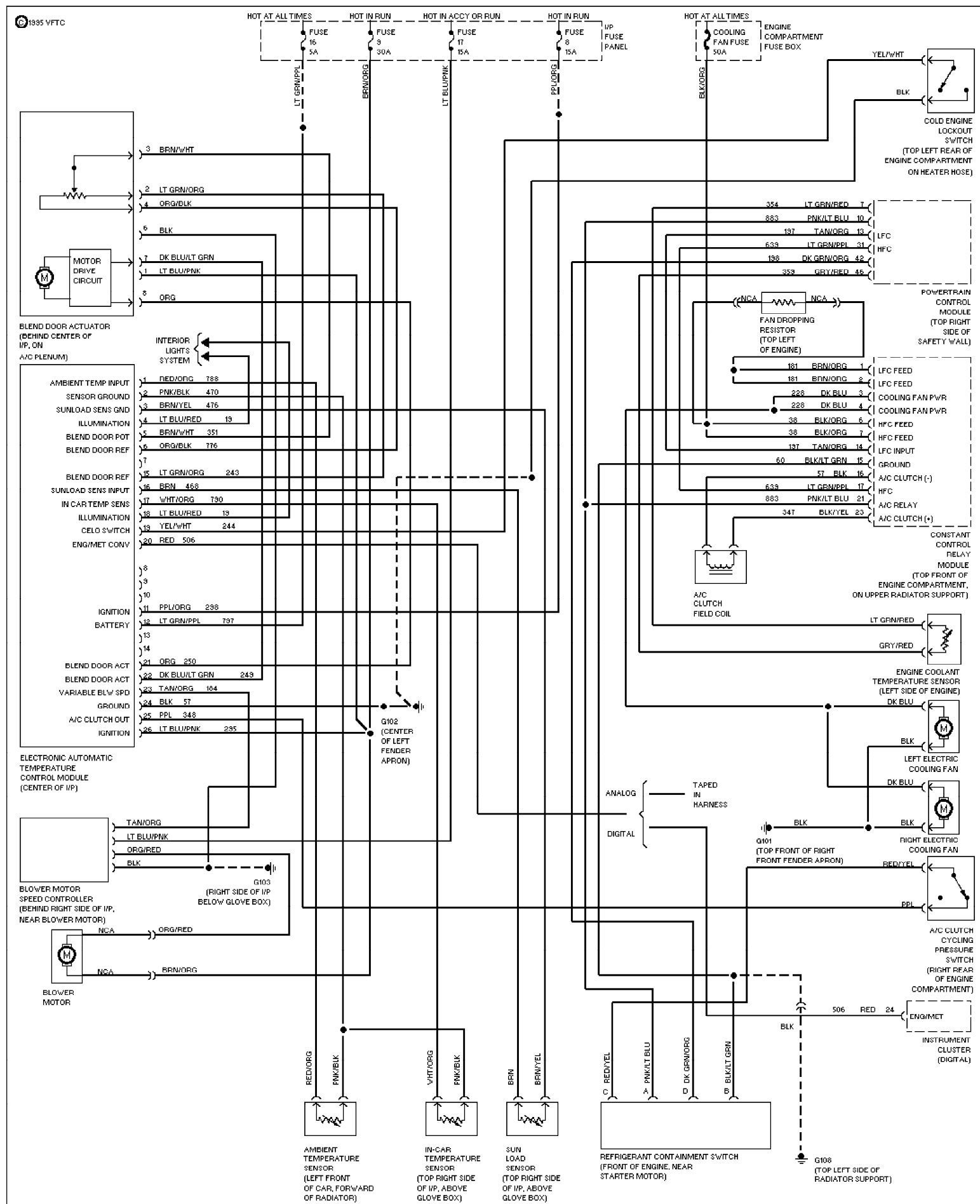
Fig. 7: 3.2L SHO, A/C Circuit, Auto A/C 1995 Ford Taurus LX
