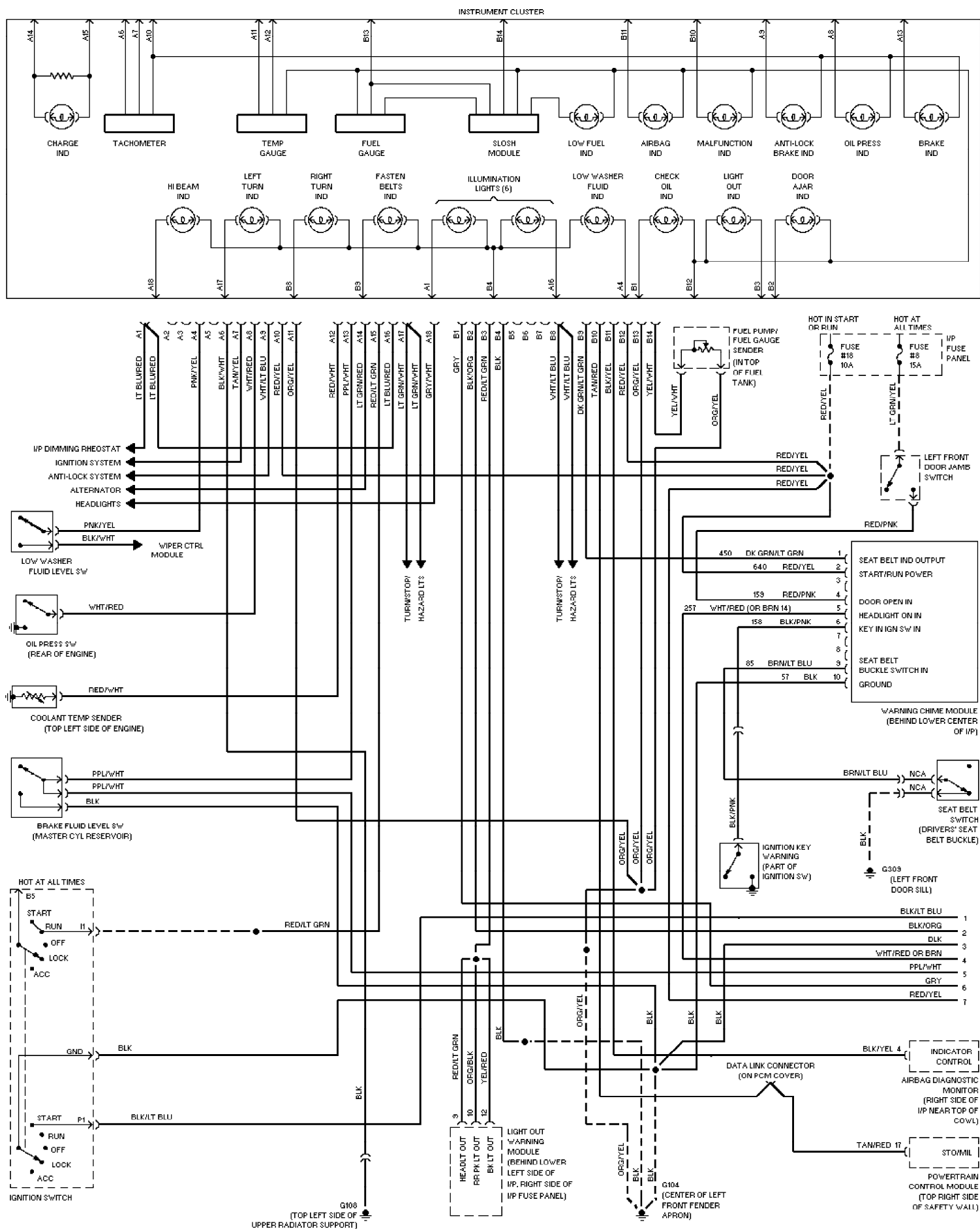
Fig. 73: 3.8L, Analog Cluster Circuit (1 of 2) 1995 Ford Taurus LX
