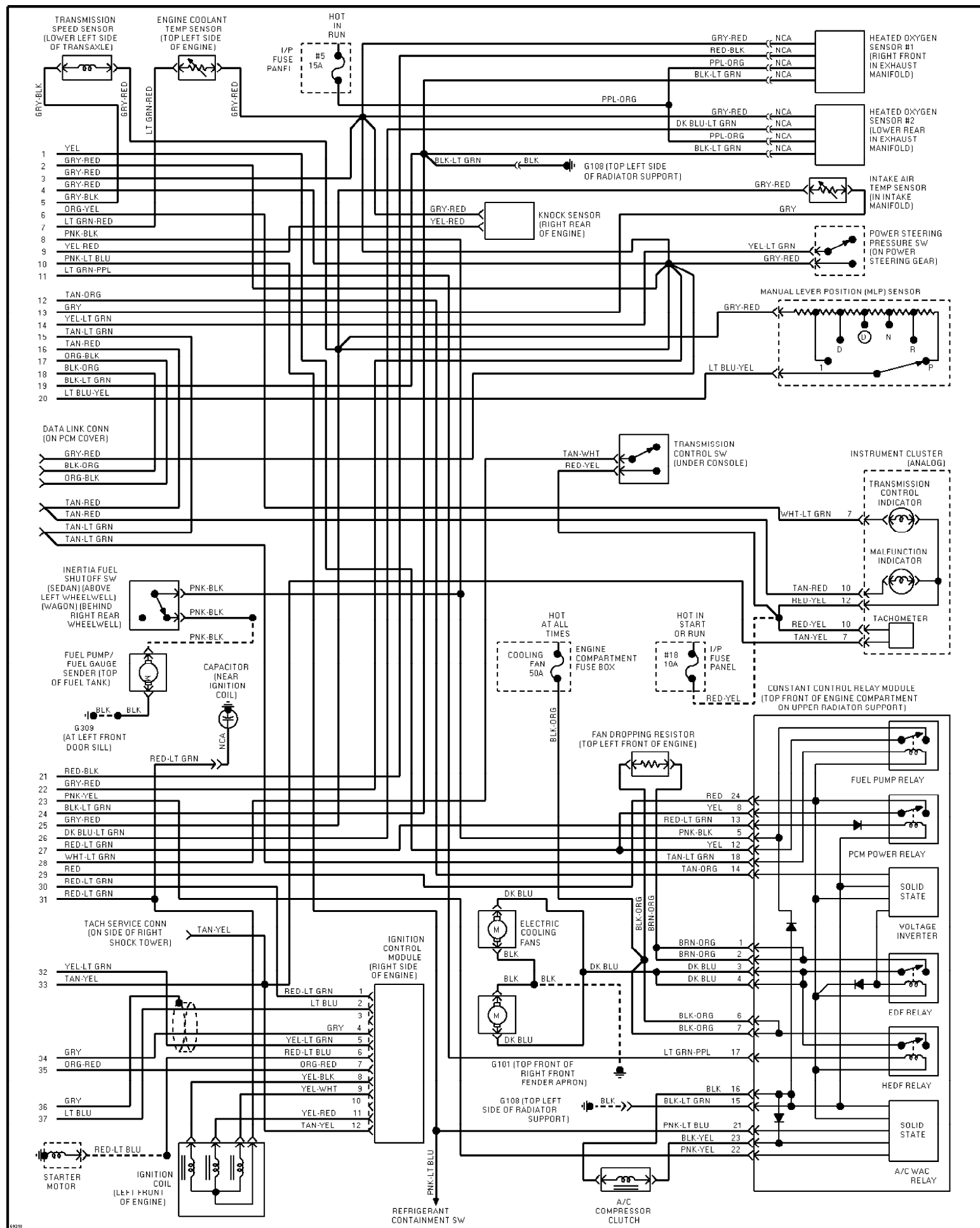
Fig. 40: 3.2L SHO, Engine Performance Circuits (2 of 2) 1995 Ford Taurus LX
