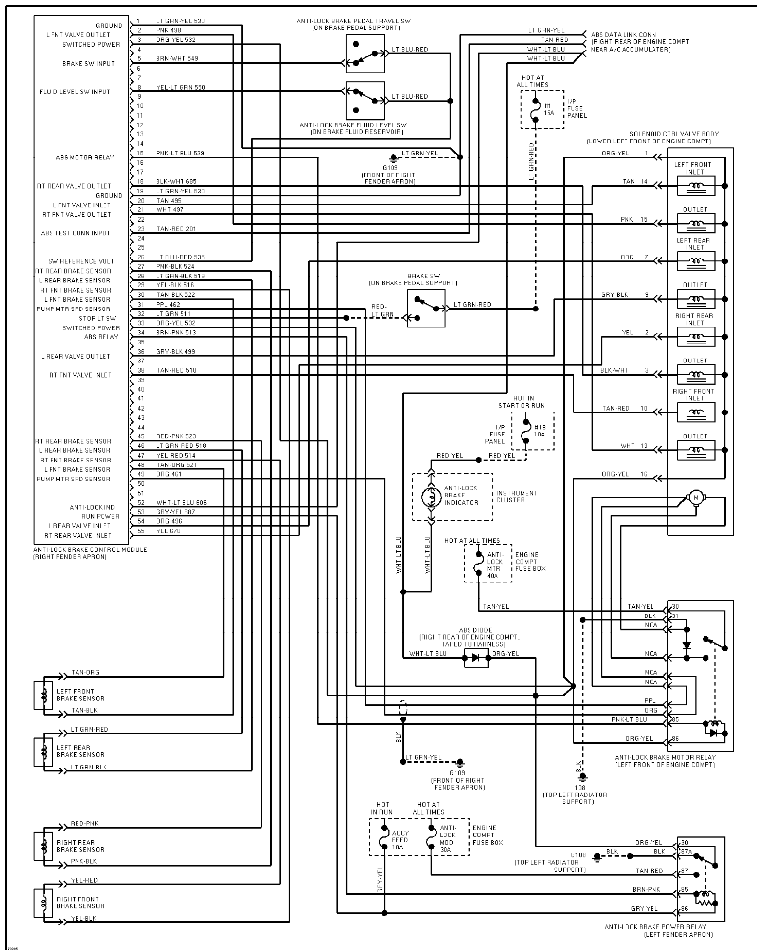
Fig. 14: 3.2L SHO, Anti-lock Brake Circuits 1995 Ford Taurus LX
