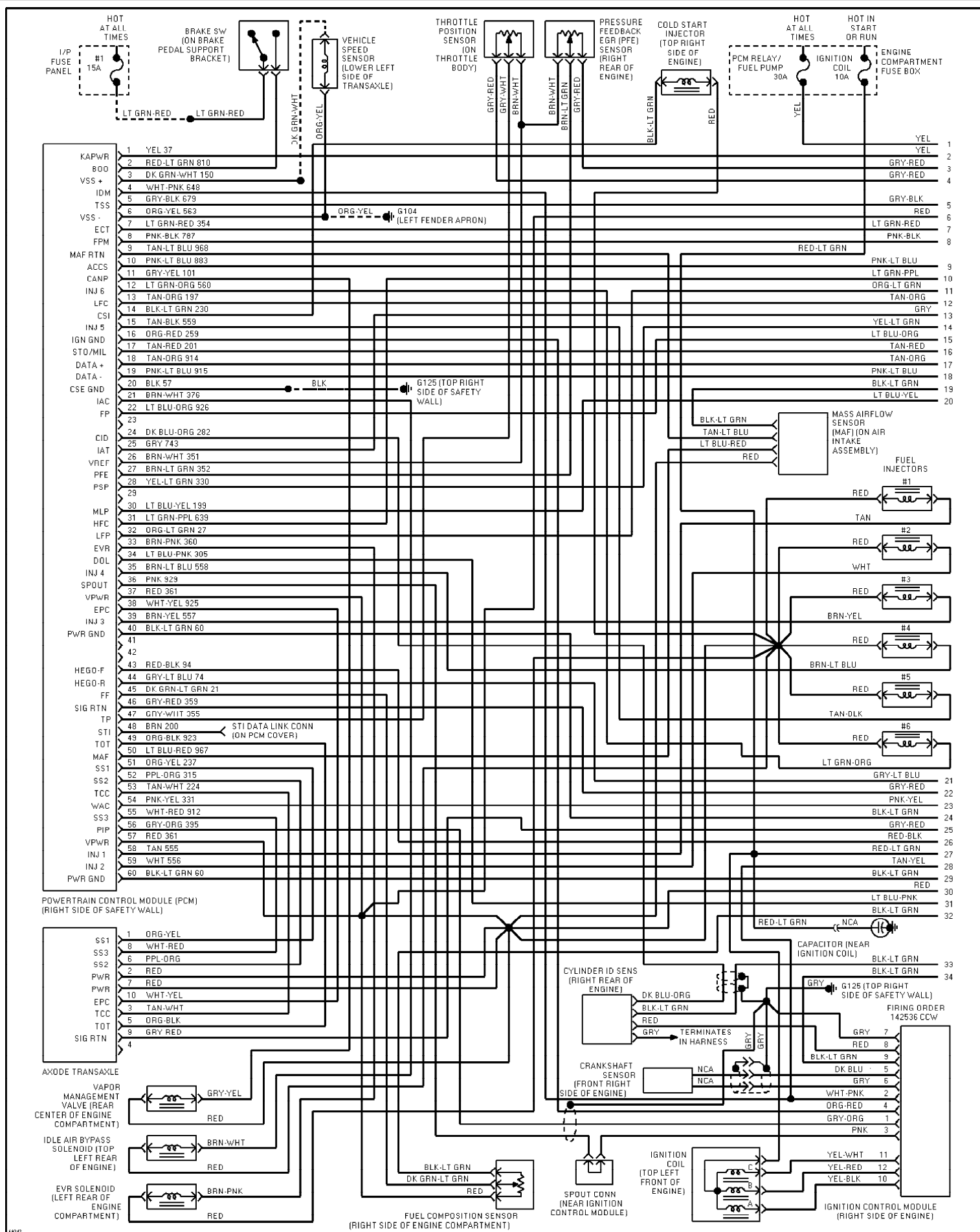
Fig. 33: 3.0L Flex Fuel, Engine Performance Circuits (1 of 2)
