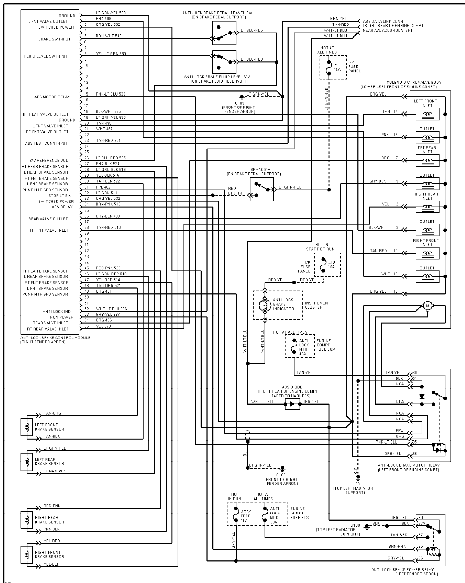
Fig. 12: 3.0L SHO, Anti-lock Brake Circuits 1995 Ford Taurus LX
