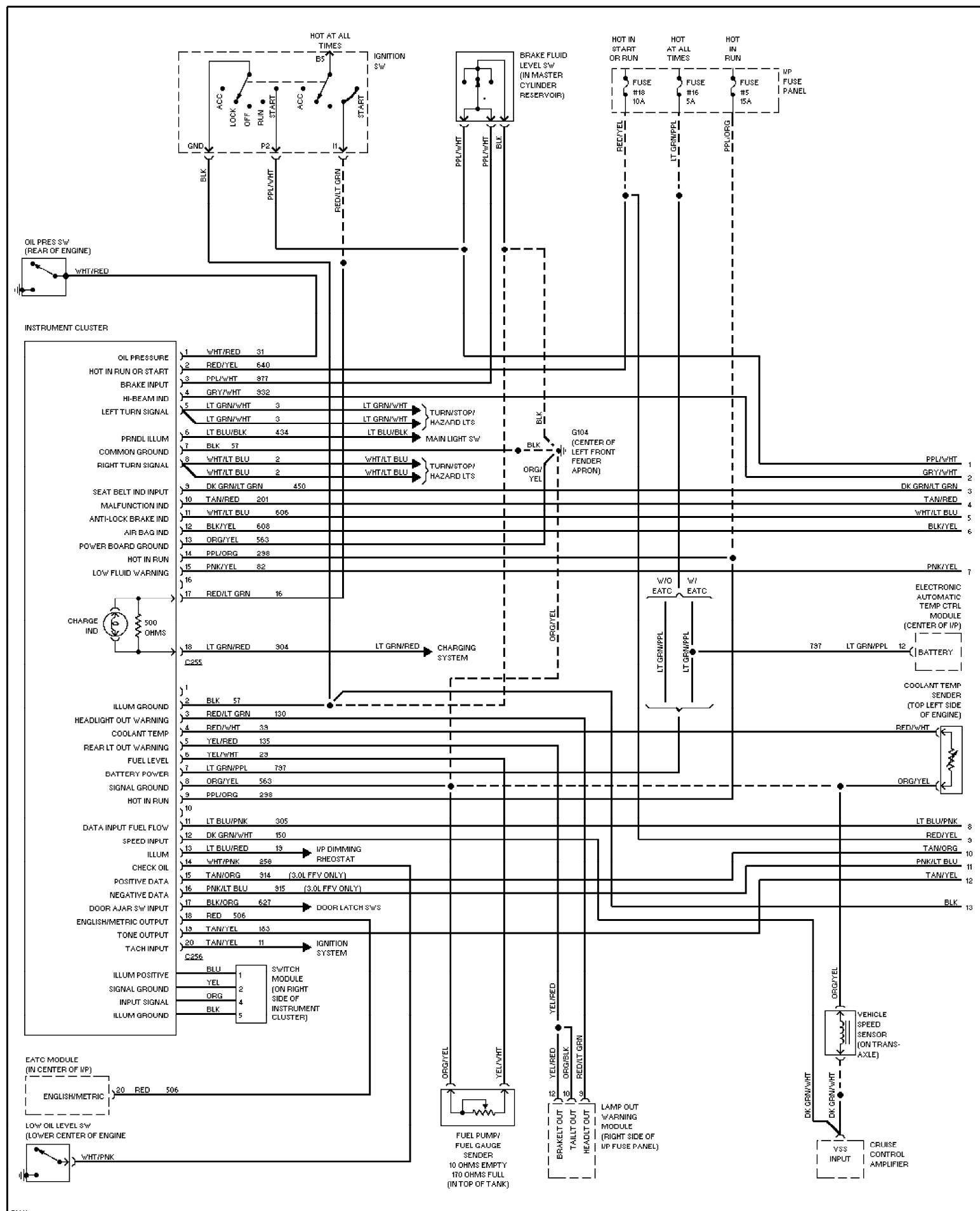
Fig. 59: 3.0L Flex Fuel, Electronic Cluster Circuit (1 of 2) 1995 Ford Taurus LX
