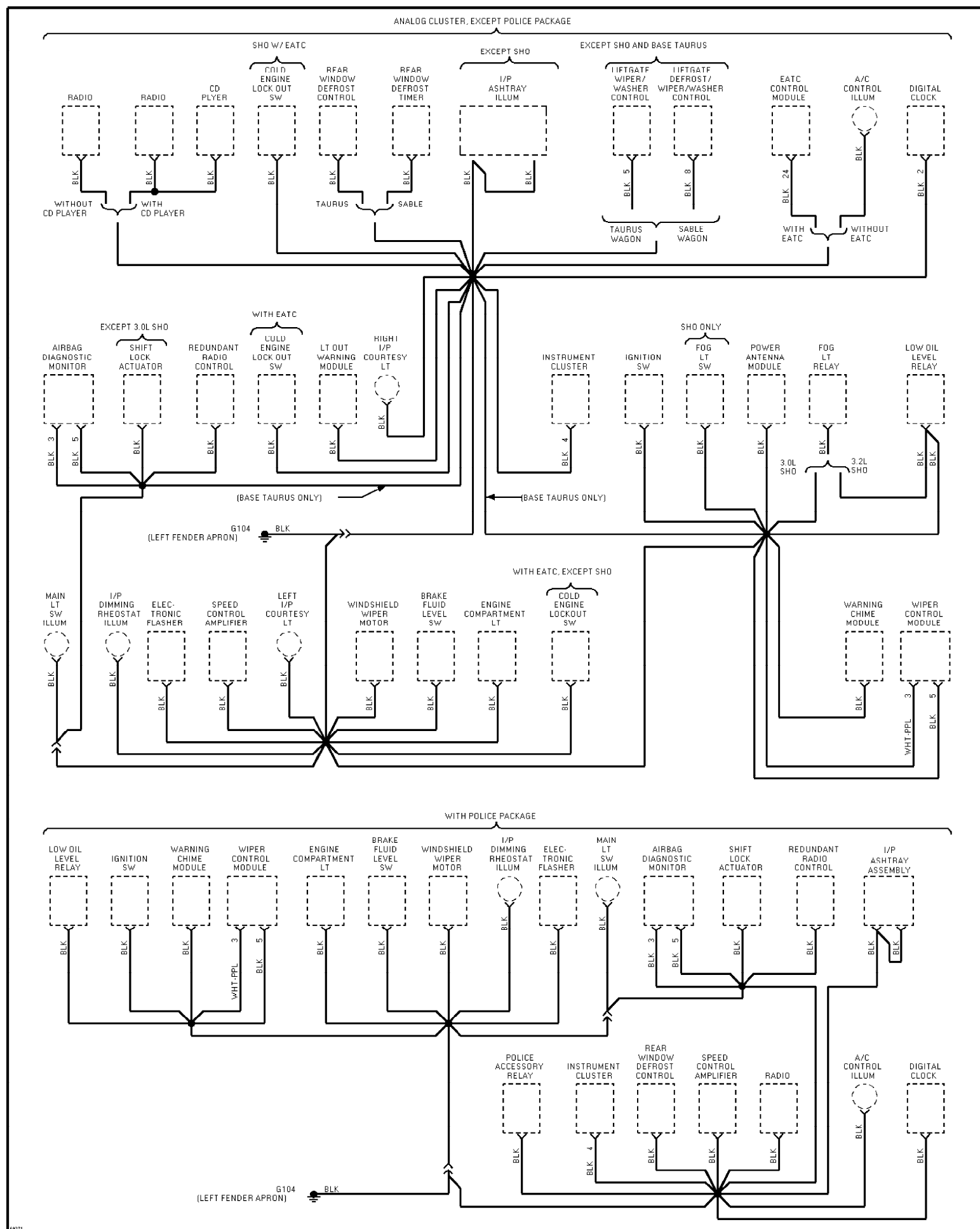
Fig. 49: Ground Distribution Circuit (4 of 5) 1995 Ford Taurus LX
