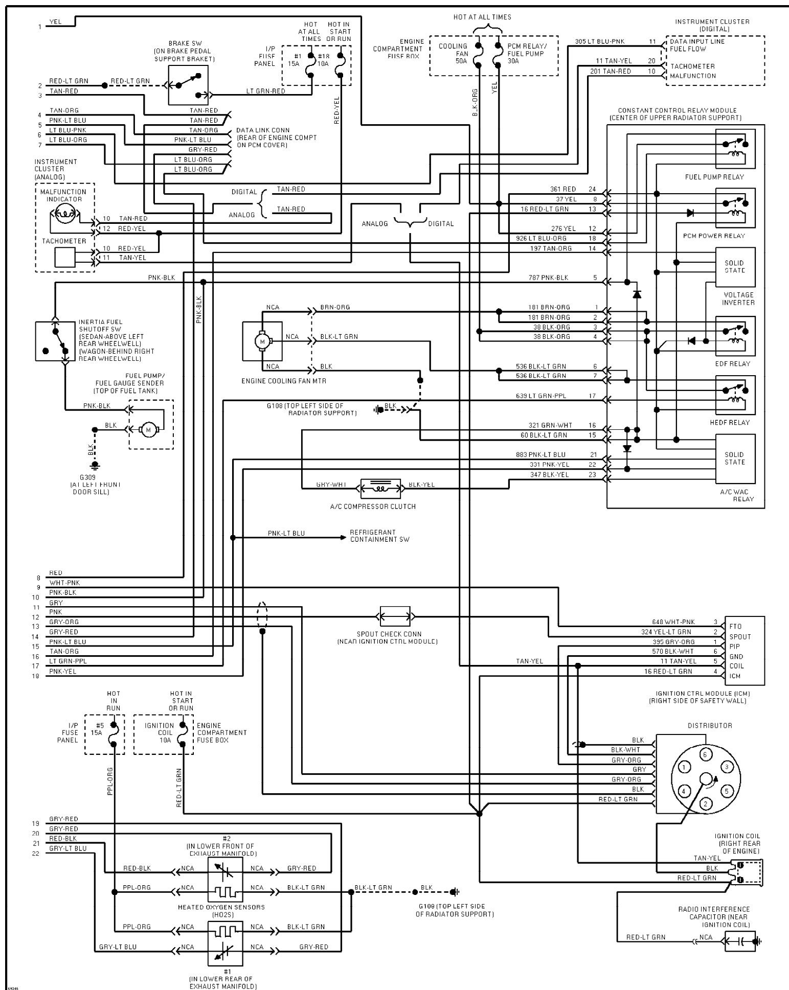
Fig. 42: 3.8L, Engine Performance Circuits (2 of 2) 1995 Ford Taurus LX
