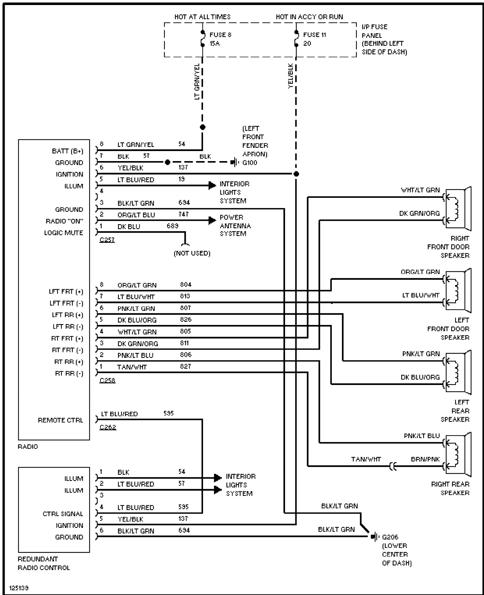
Fig. 97: Base Radio 1995 Ford Taurus LX
