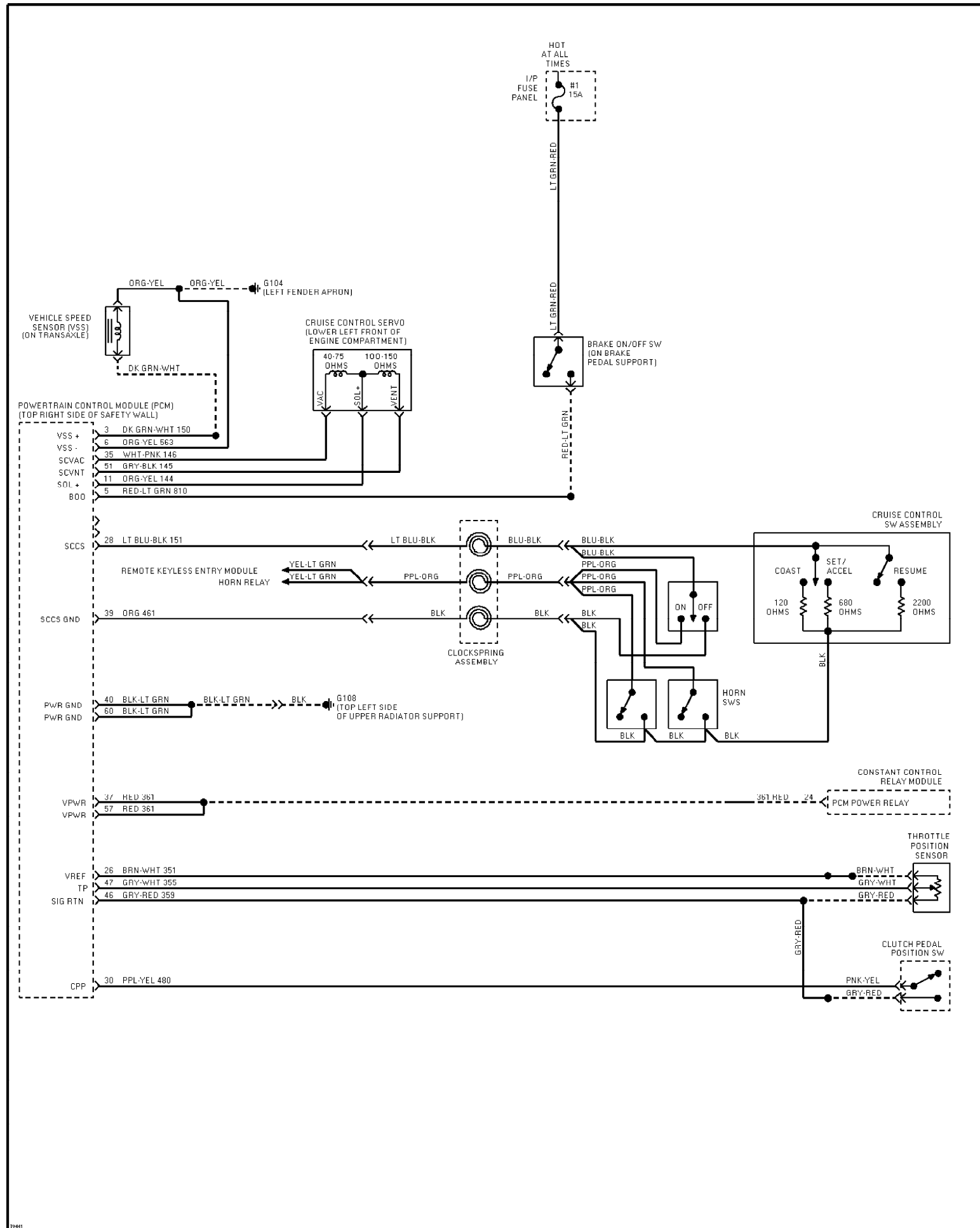
Fig. 27: 3.0L SHO, Cruise Control Circuit 1995 Ford Taurus LX
