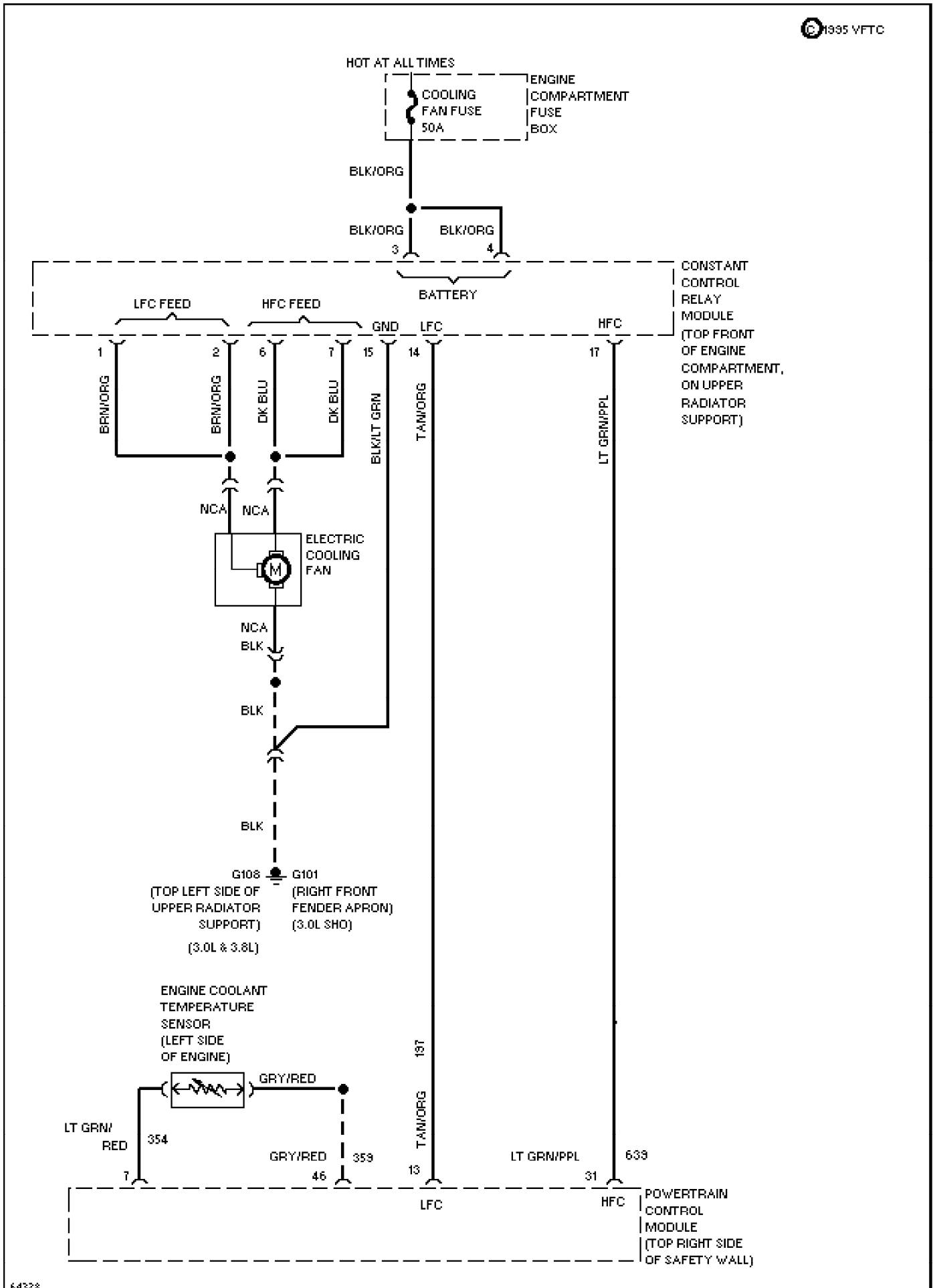
Fig. 23: 3.0L, Cooling Fan Circuit 1995 Ford Taurus LX
