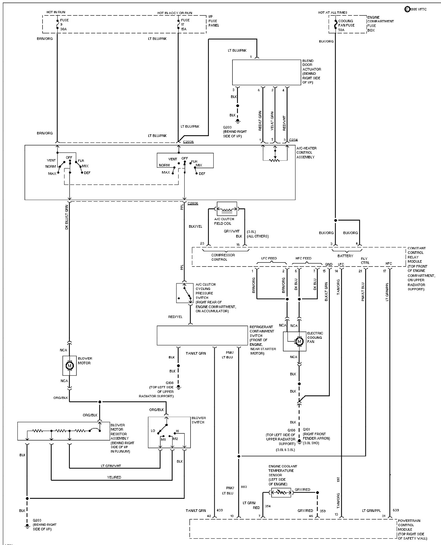
Fig. 6: 3.0L, A/C Circuit, Manual A/C 1995 Ford Taurus LX
