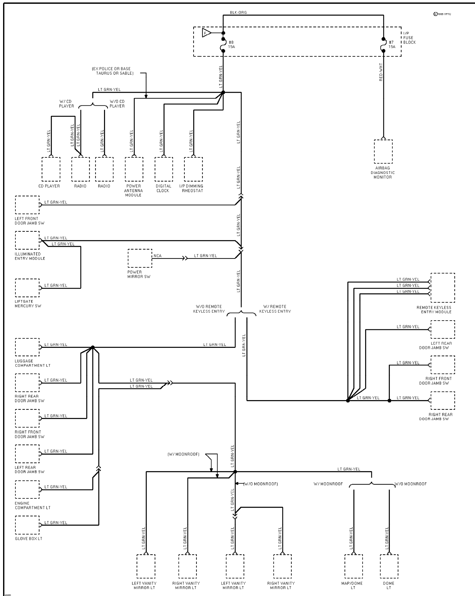
Fig. 85: Power Distribution Circuit (3 of 6) 1995 Ford Taurus LX
