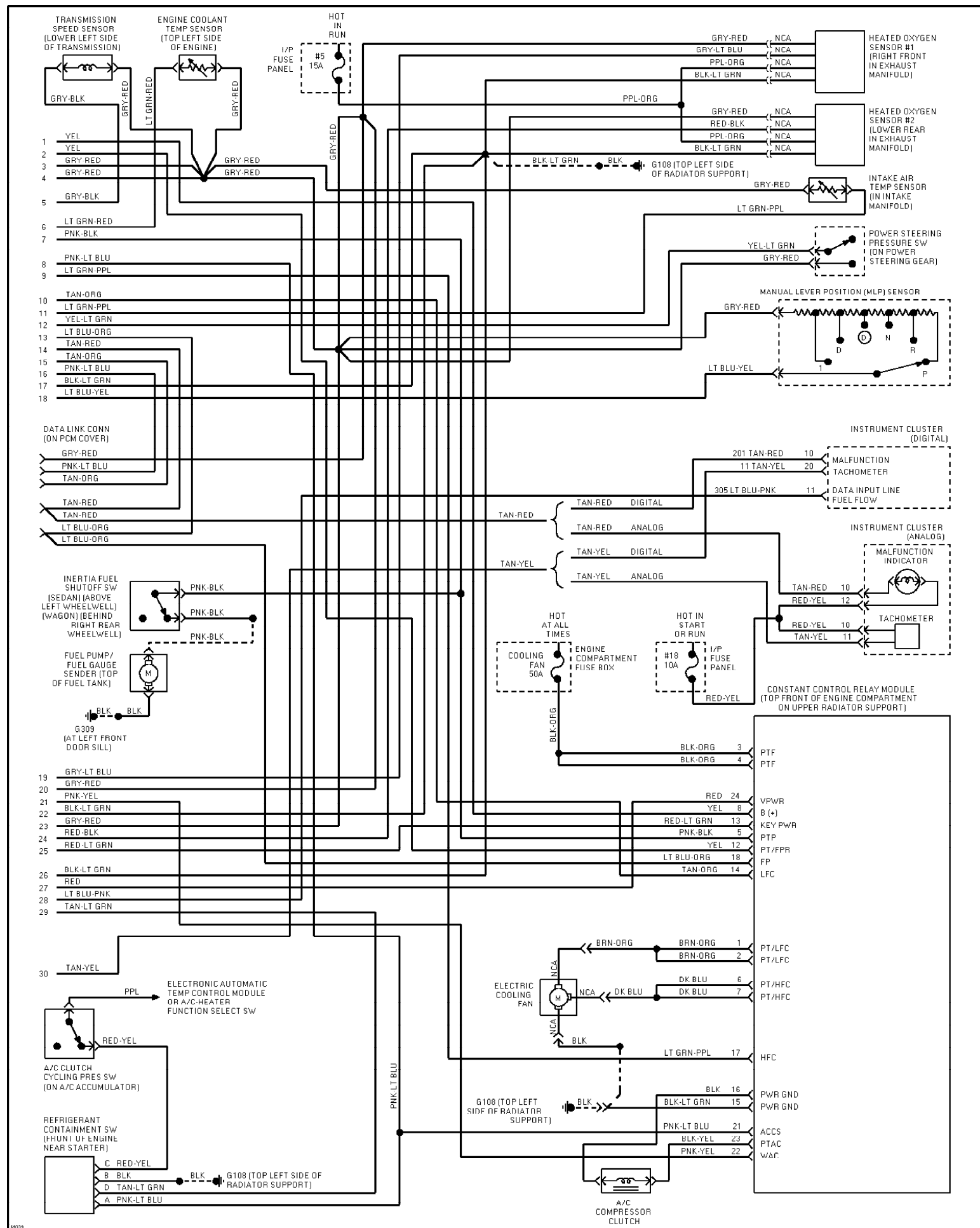
Fig. 38: 3.0L, Engine Performance Circuits (2 of 2) 1995 Ford Taurus LX
