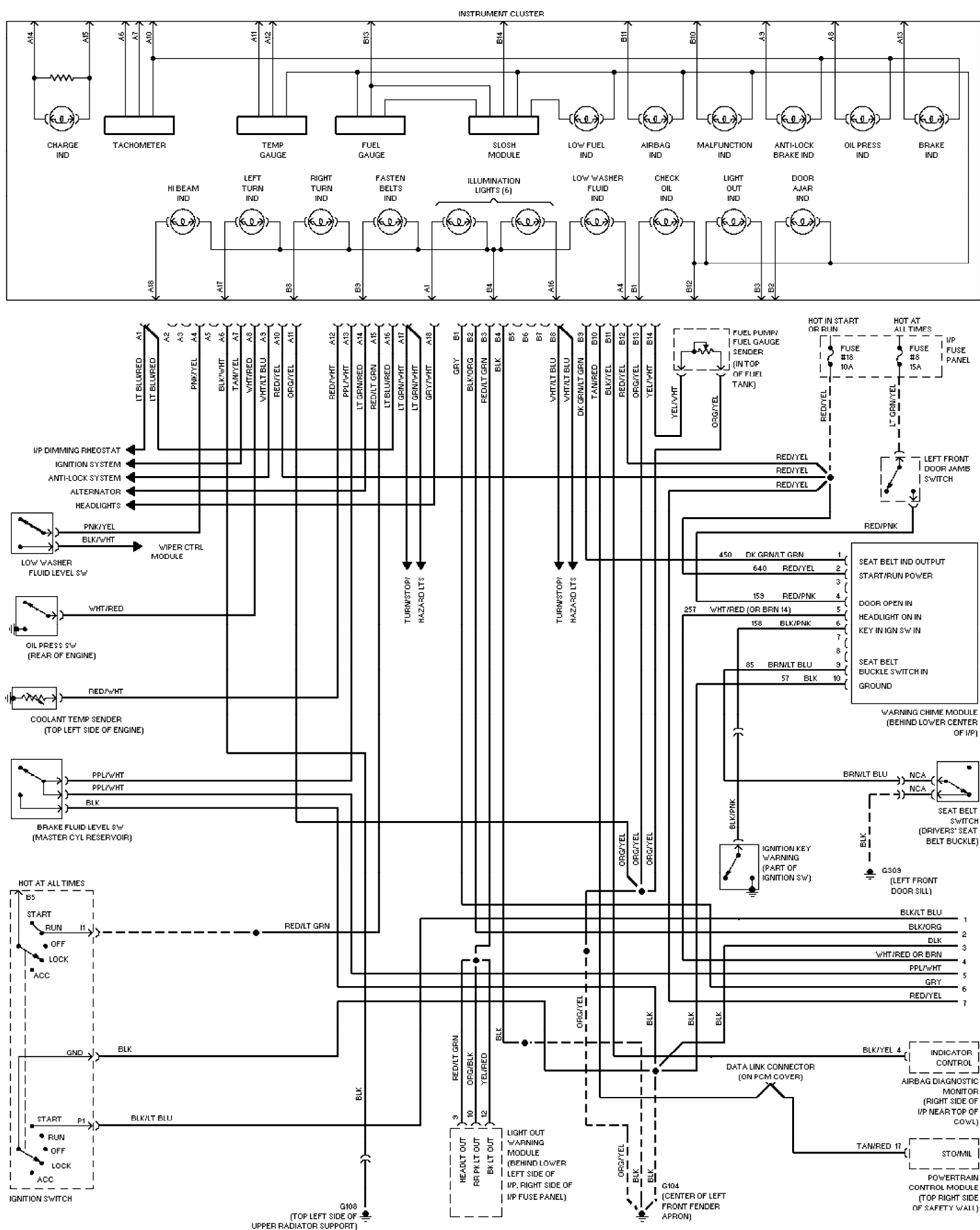
Fig. 65: 3.0L, Analog Cluster Circuit (1 of 2) 1995 Ford Taurus LX
