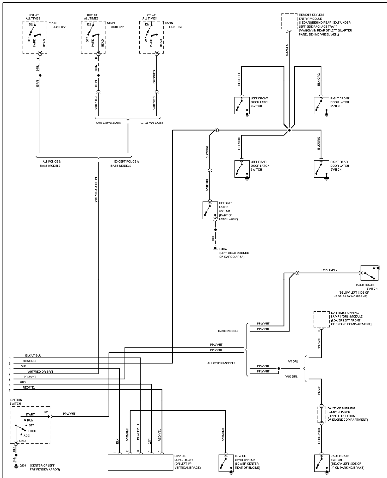
Fig. 58: 3.0L Flex Fuel, Analog Cluster Circuit (2 of 2) 1995 Ford Taurus LX
