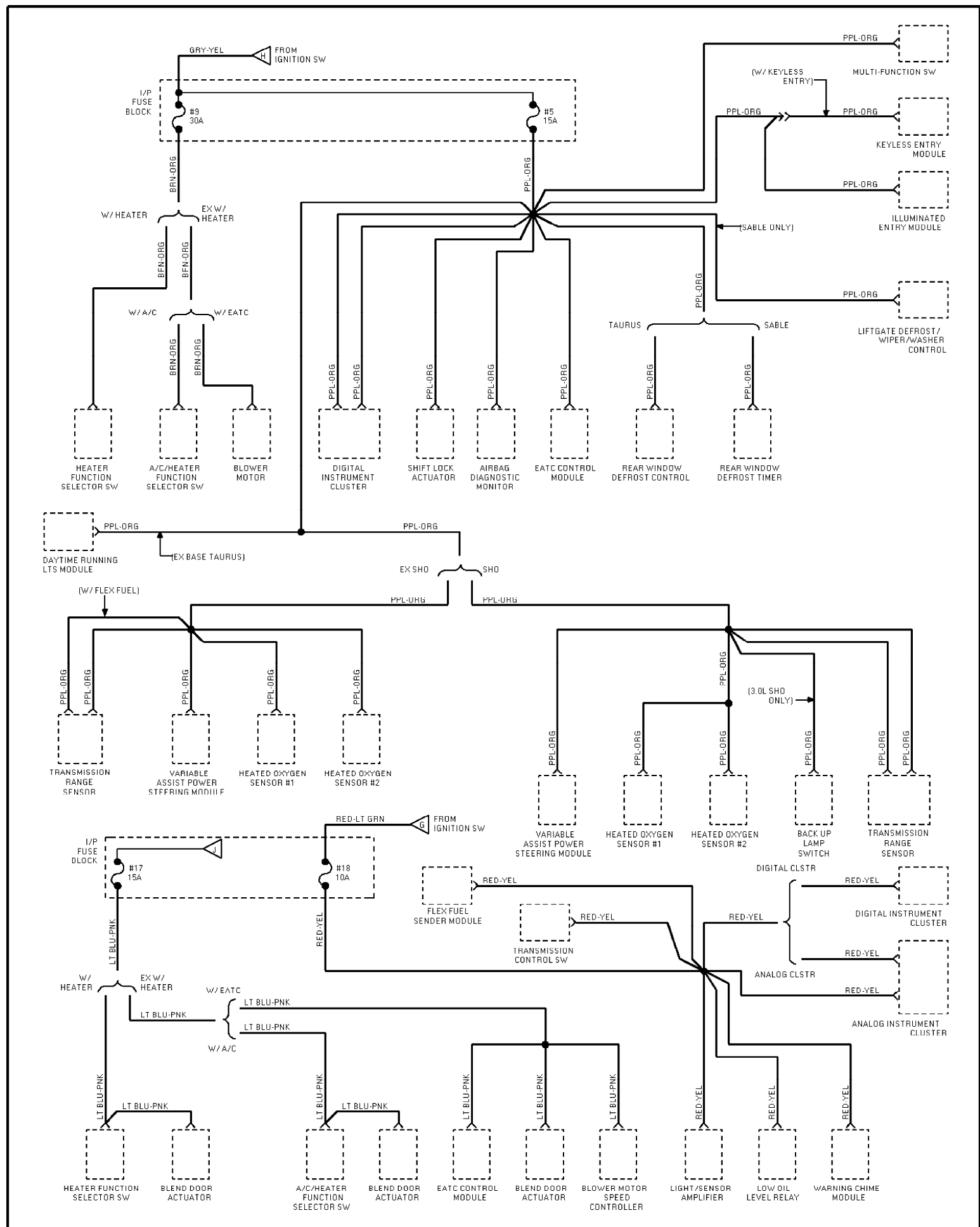
Fig. 86: Power Distribution Circuit (4 of 6) 1995 Ford Taurus LX
