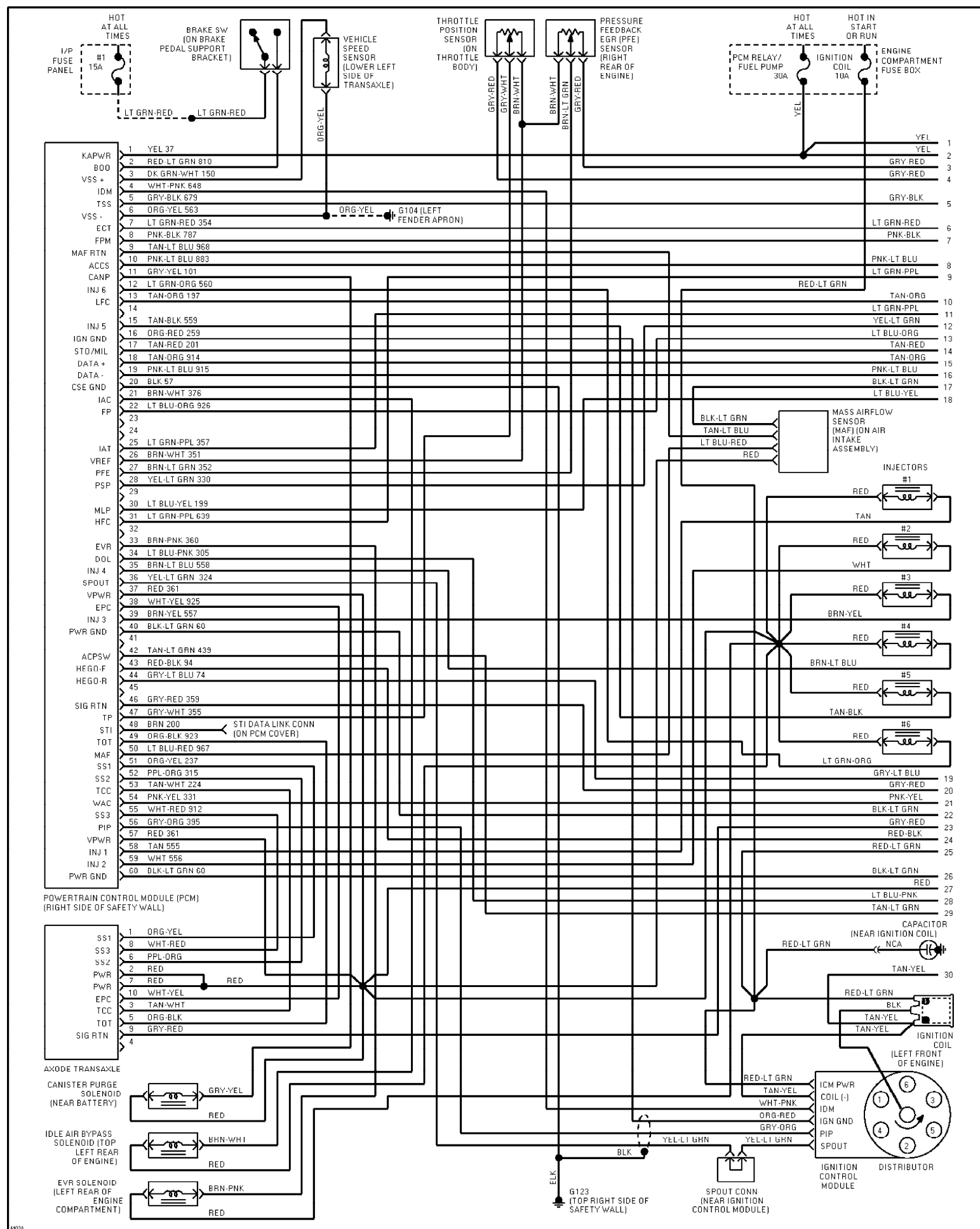
Fig. 37: 3.0L, Engine Performance Circuits (1 of 2) 1995 Ford Taurus LX
