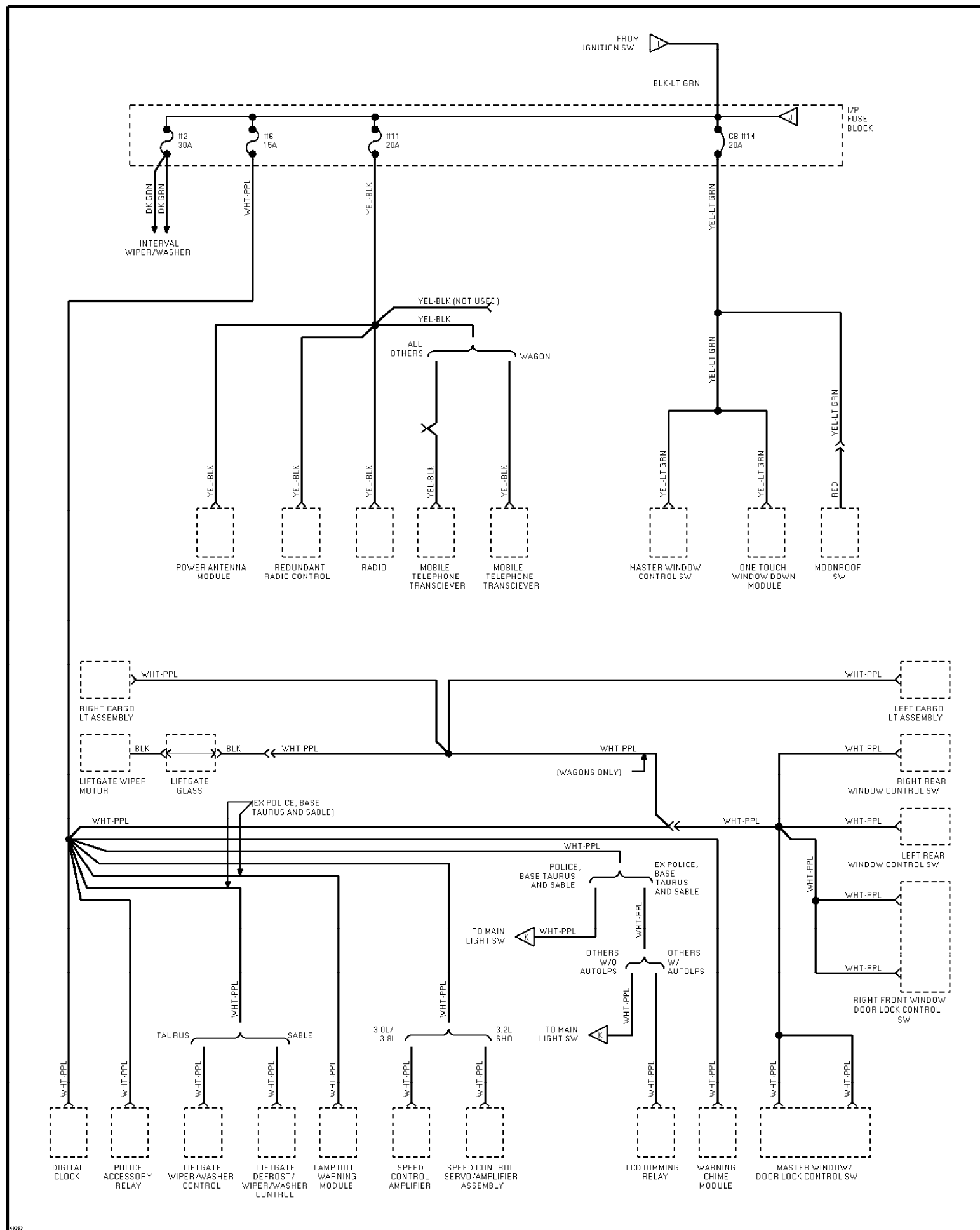
Fig. 87: Power Distribution Circuit (5 of 6) 1995 Ford Taurus LX
