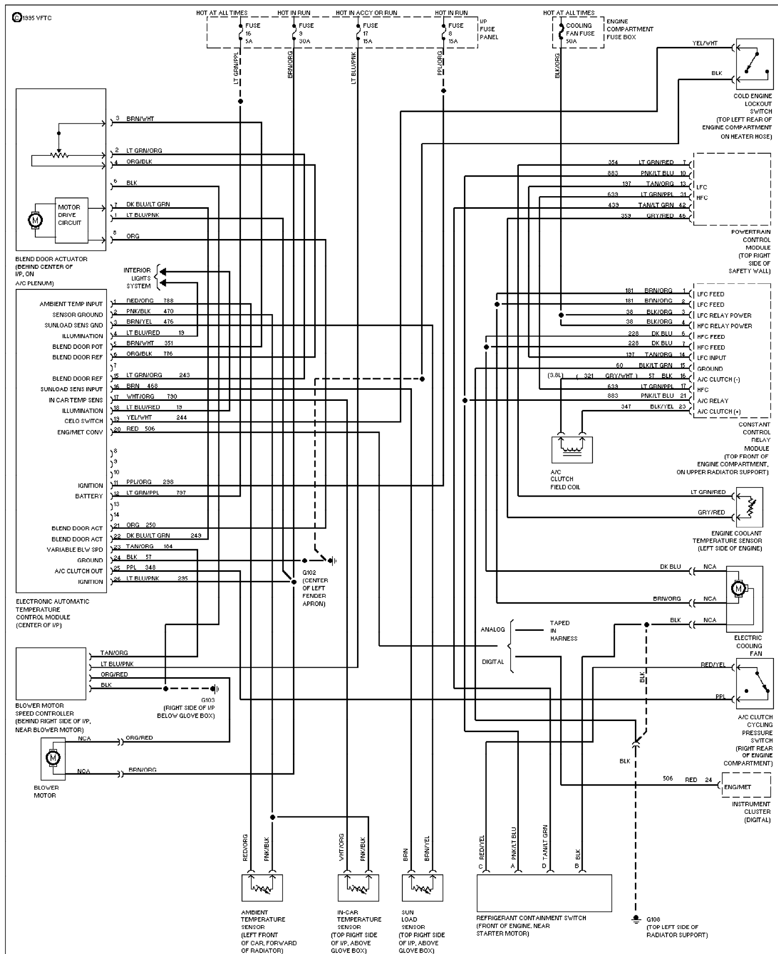
Fig. 5: 3.0L, A/C Circuit, Auto A/C 1995 Ford Taurus LX
