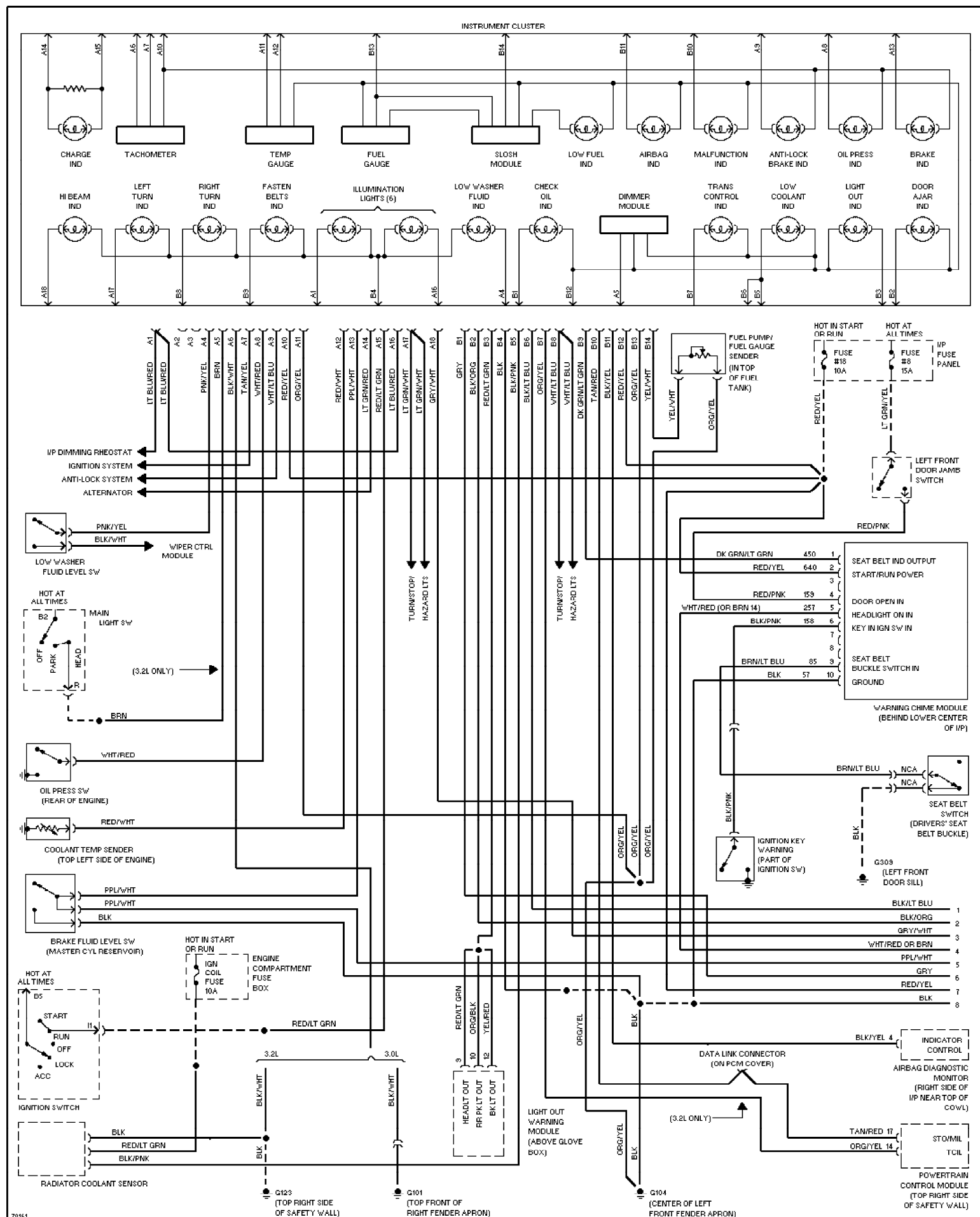
Fig. 62: 3.0L SHO, Instrument Cluster Circuit (1 of 2) 1995 Ford Taurus LX
