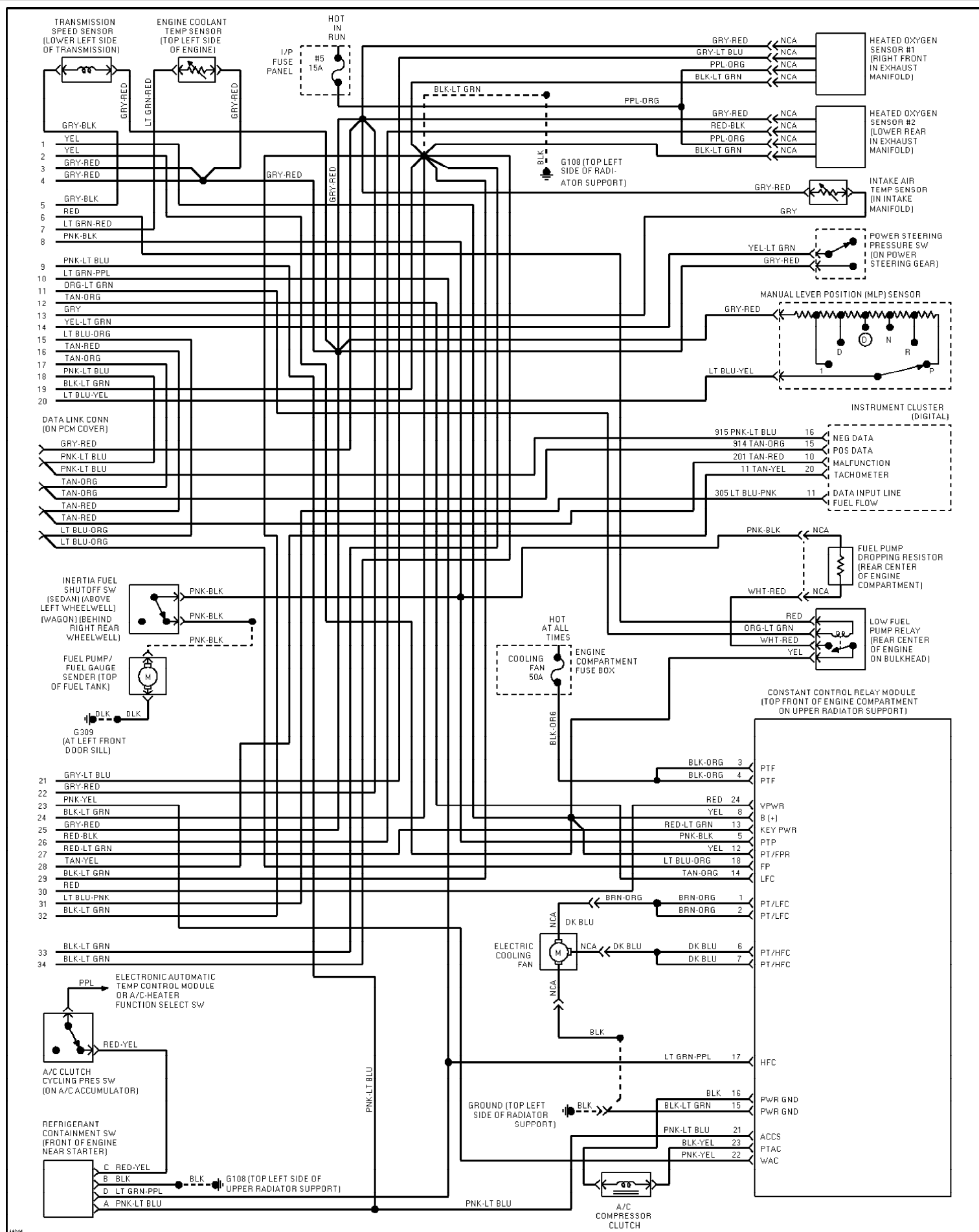
Fig. 34: 3.0L Flex Fuel, Engine Performance Circuits (2 of 2)
