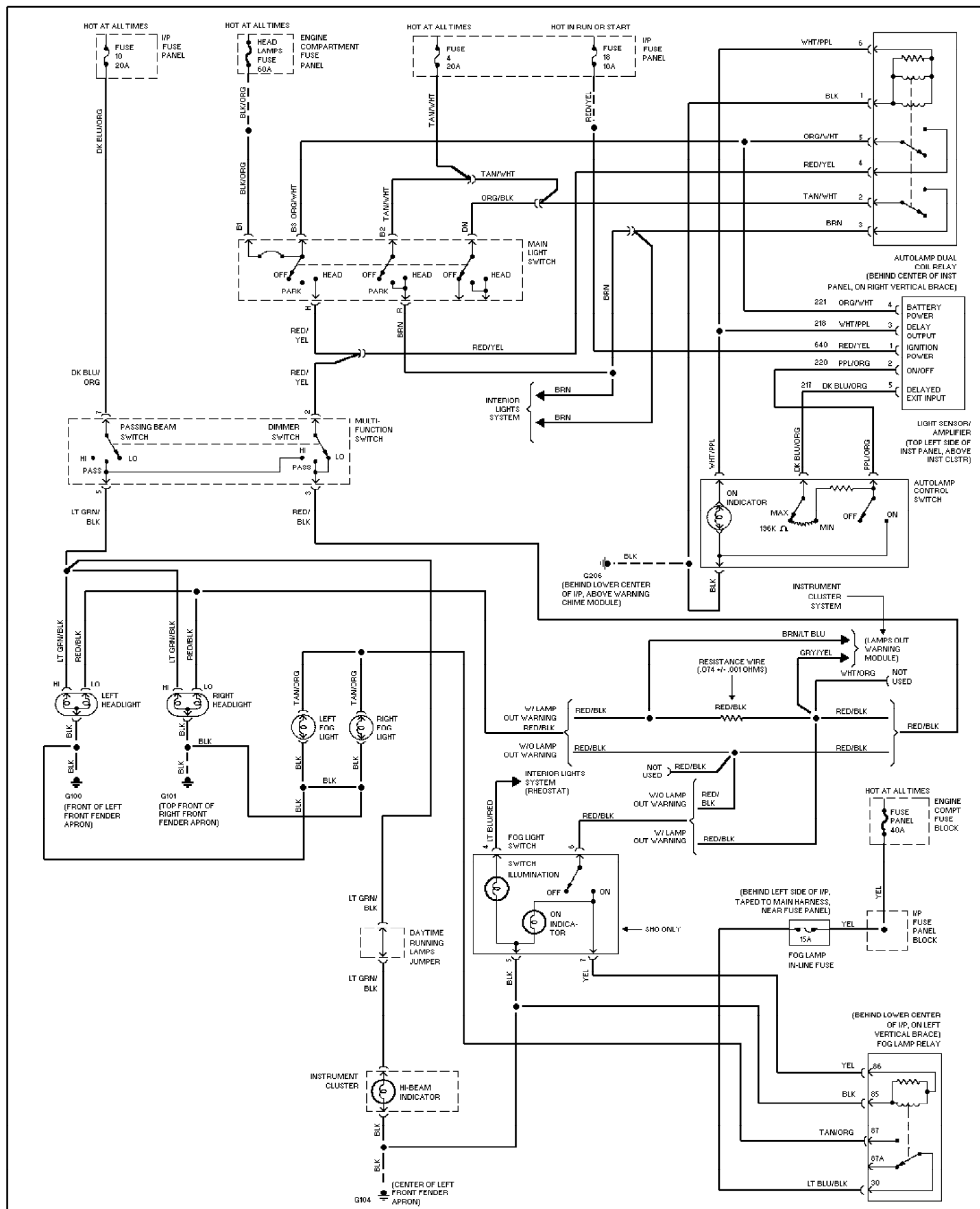
Fig. 52: Autolamps/Fog Lamps Circuit, W/O DRL 1995 Ford Taurus LX
