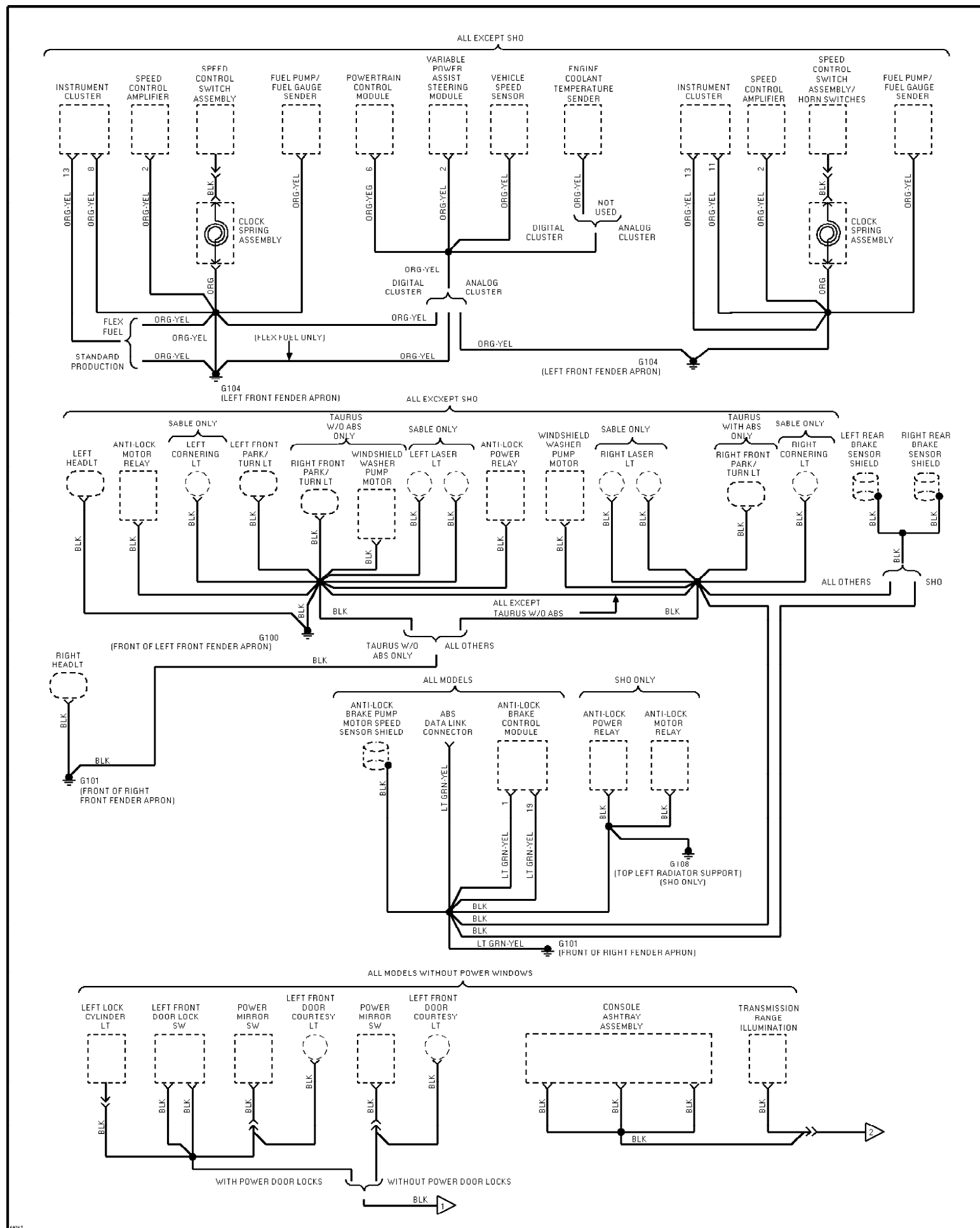
Fig. 47: Ground Distribution Circuit (2 of 5) 1995 Ford Taurus LX
