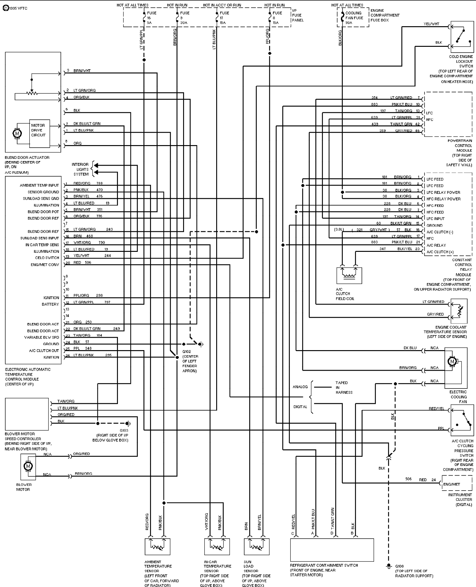
Fig. 9: 3.8L, A/C Circuit, Auto A/C 1995 Ford Taurus LX
