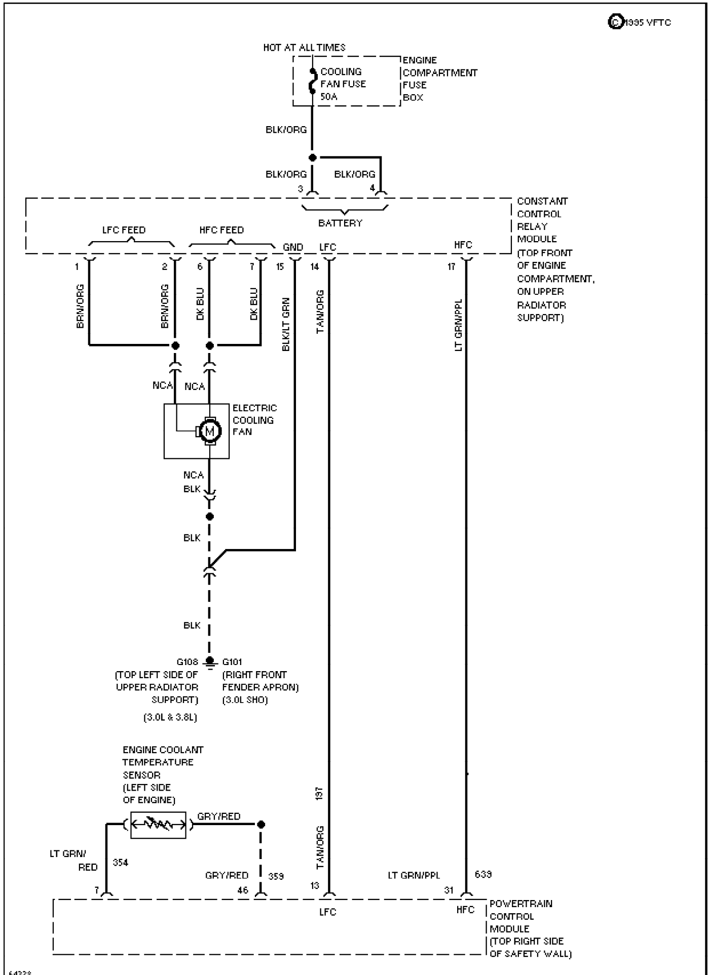
Fig. 21: 3.0L Flex Fuel, Cooling Fan Circuit 1995 Ford Taurus LX
