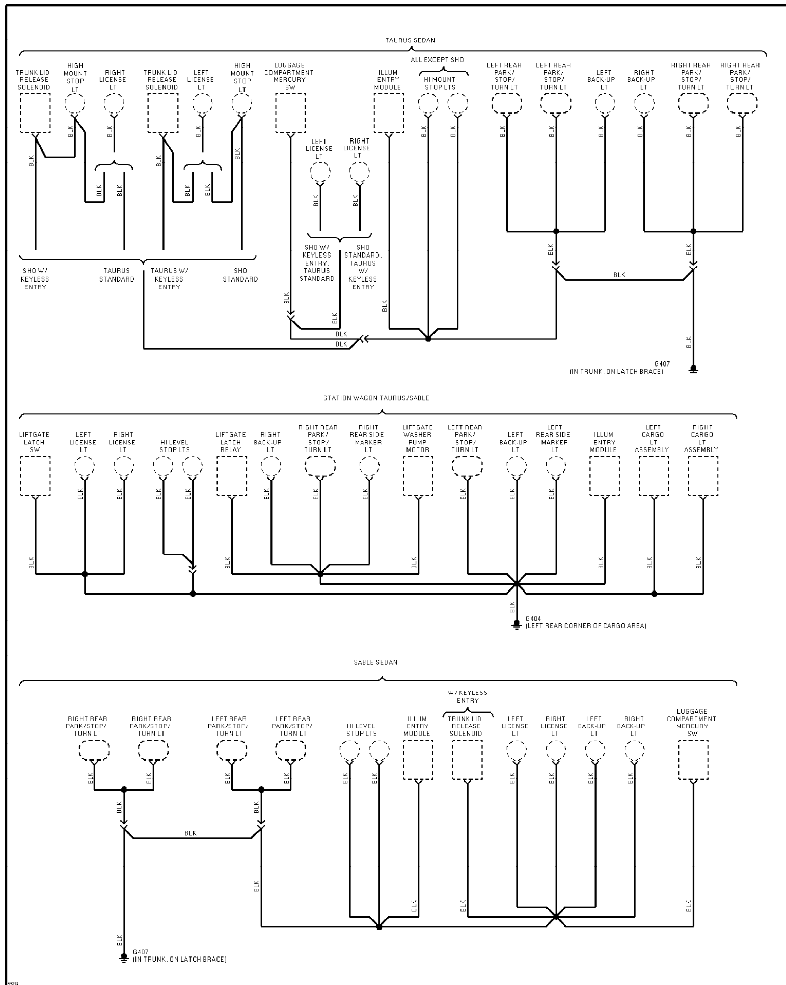
Fig. 50: Ground Distribution Circuit (5 of 5) 1995 Ford Taurus LX
