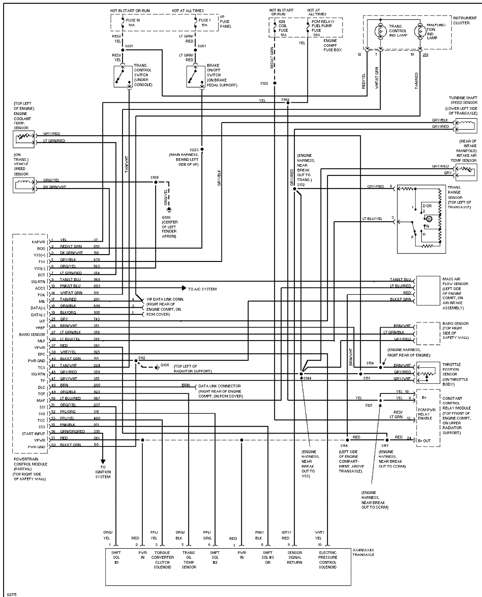
Fig. 113: 3.2L SHO, Transmission Circuit 1995 Ford Taurus LX
