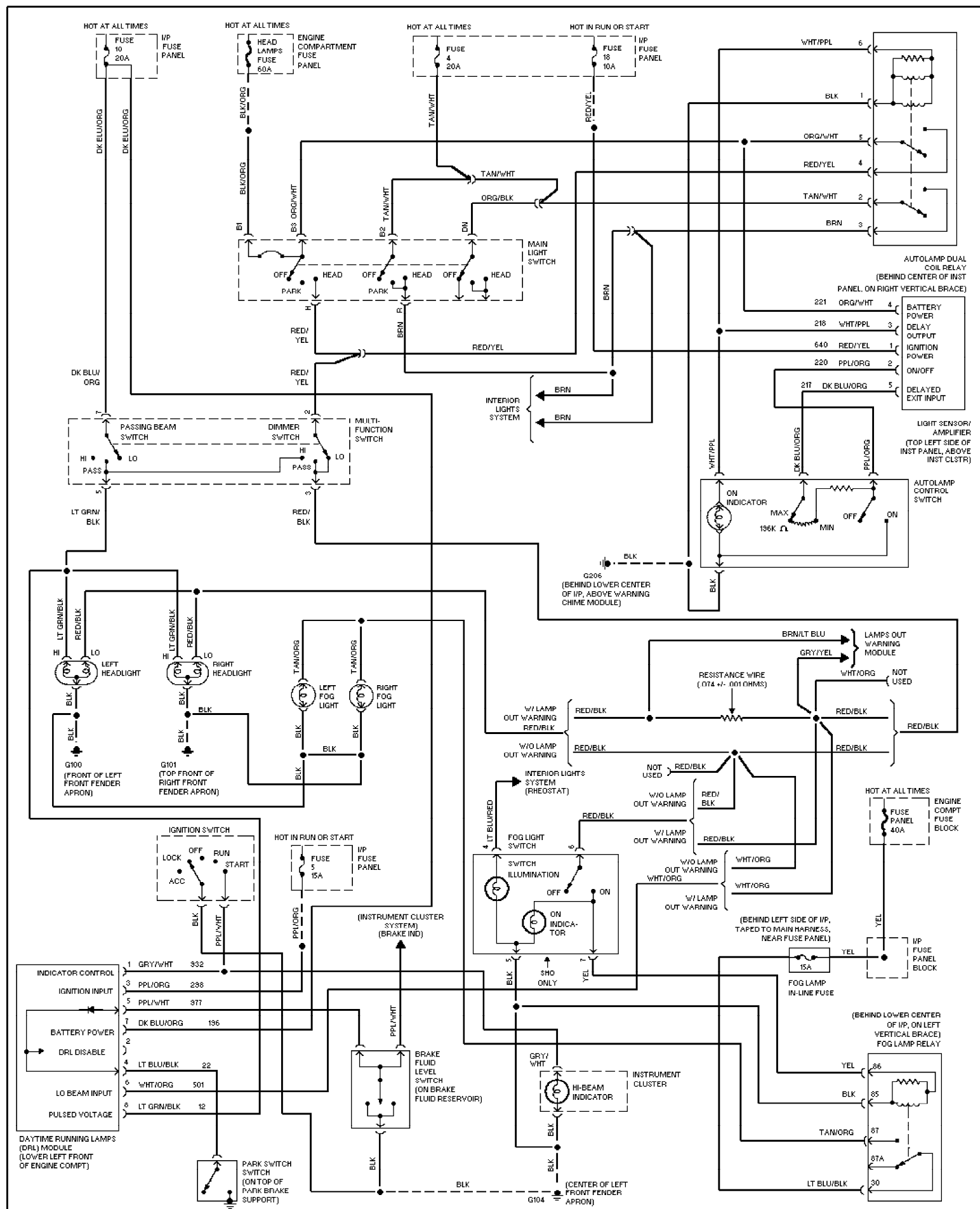
Fig. 51: Autolamps/Fog Lamps Circuit, W/ DRL 1995 Ford Taurus LX
