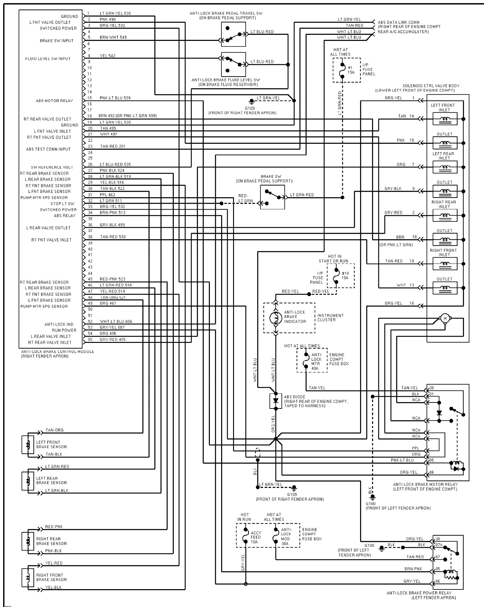
Fig. 11: 3.0L Flex Fuel, Anti-lock Brake Circuits 1995 Ford Taurus LX
