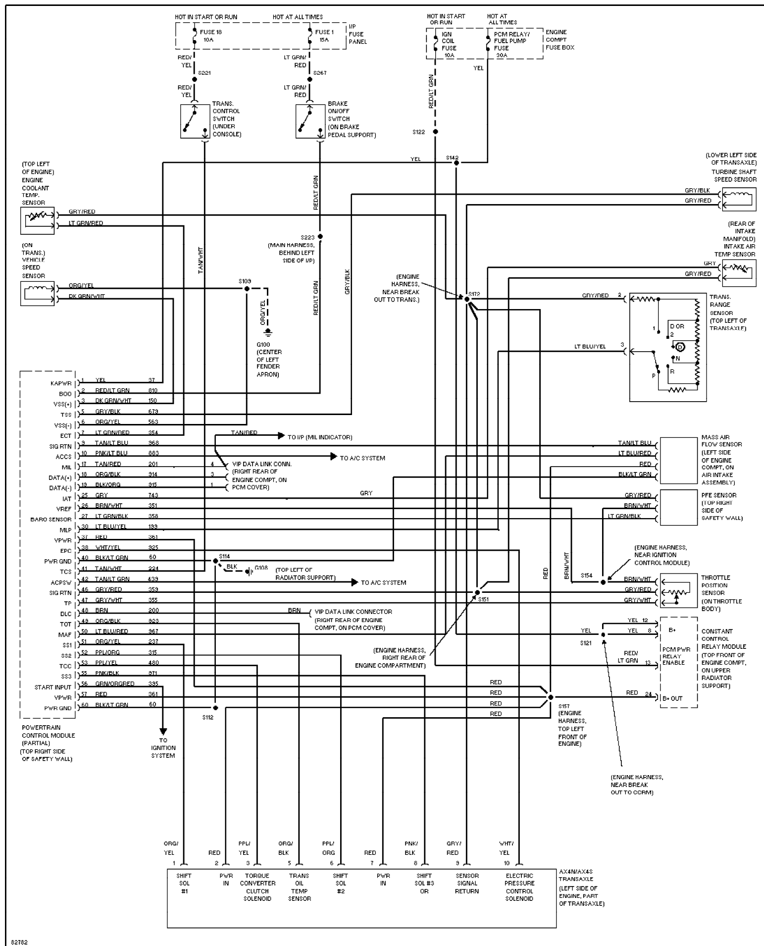
Fig. 114: 3.8L, Transmission Circuit 1995 Ford Taurus LX
