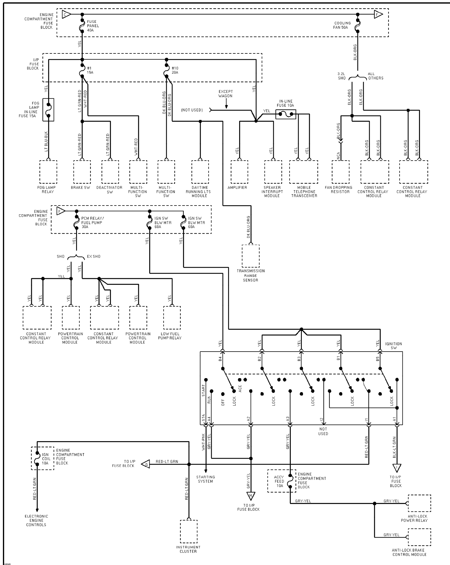
Fig. 84: Power Distribution Circuit (2 of 6) 1995 Ford Taurus LX
