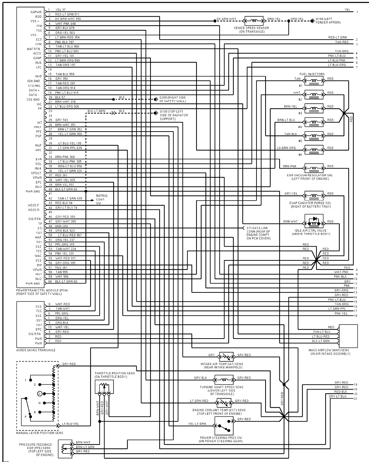
Fig. 41: 3.8L, Engine Performance Circuits (1 of 2) 1995 Ford Taurus LX
