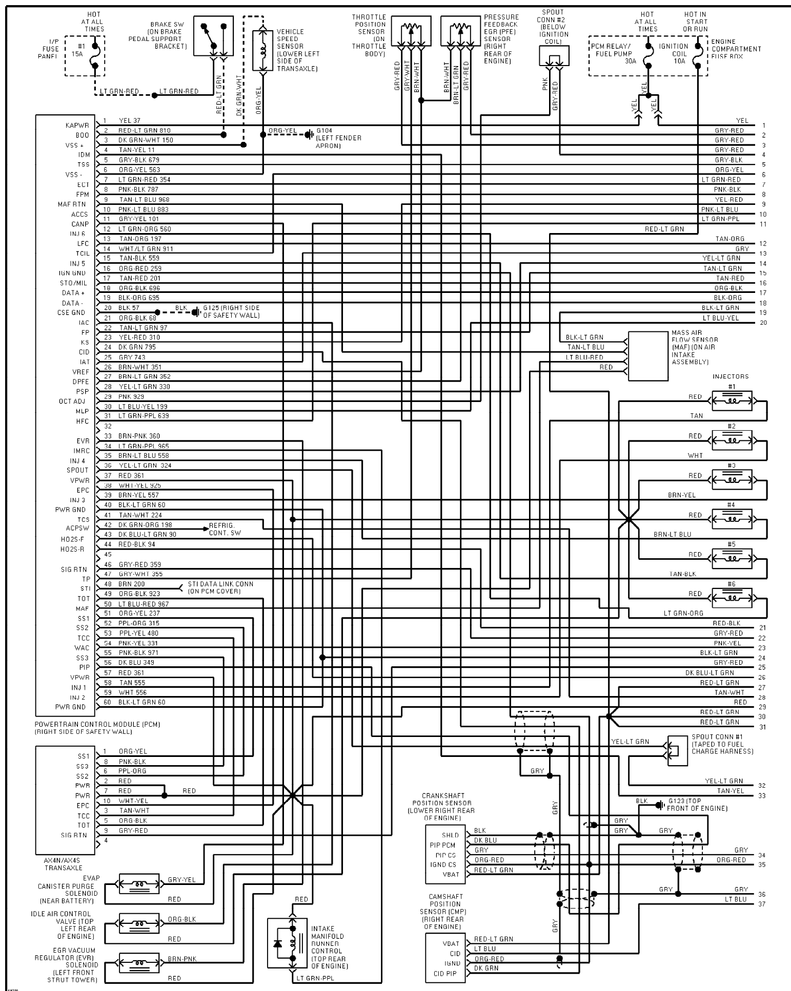
Fig. 39: 3.2L SHO, Engine Performance Circuits (1 of 2) 1995 Ford Taurus LX
