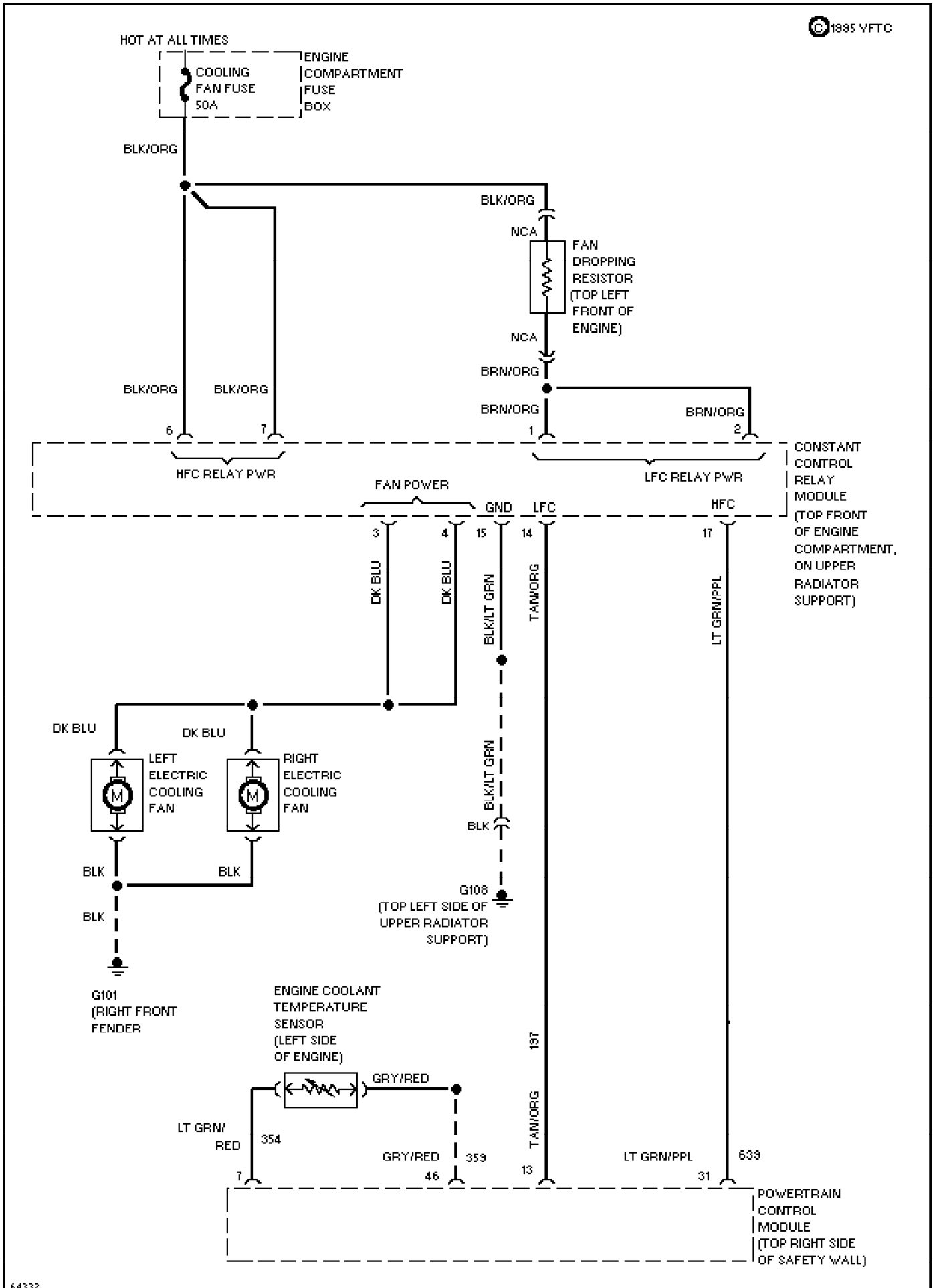
Fig. 24: 3.2L SHO, Cooling Fan Circuit 1995 Ford Taurus LX
