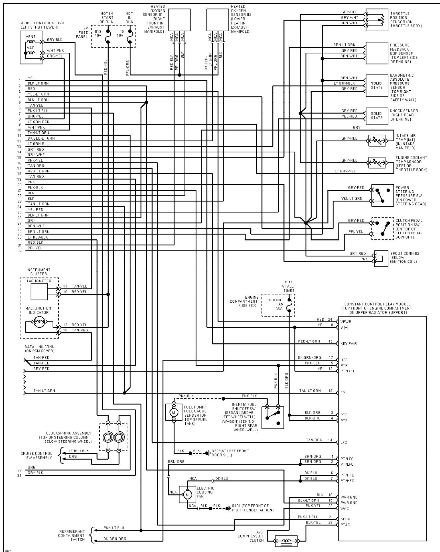
Fig. 36: 3.0L SHO, Engine Performance Circuits (2 of 2) 1995 Ford Taurus LX
