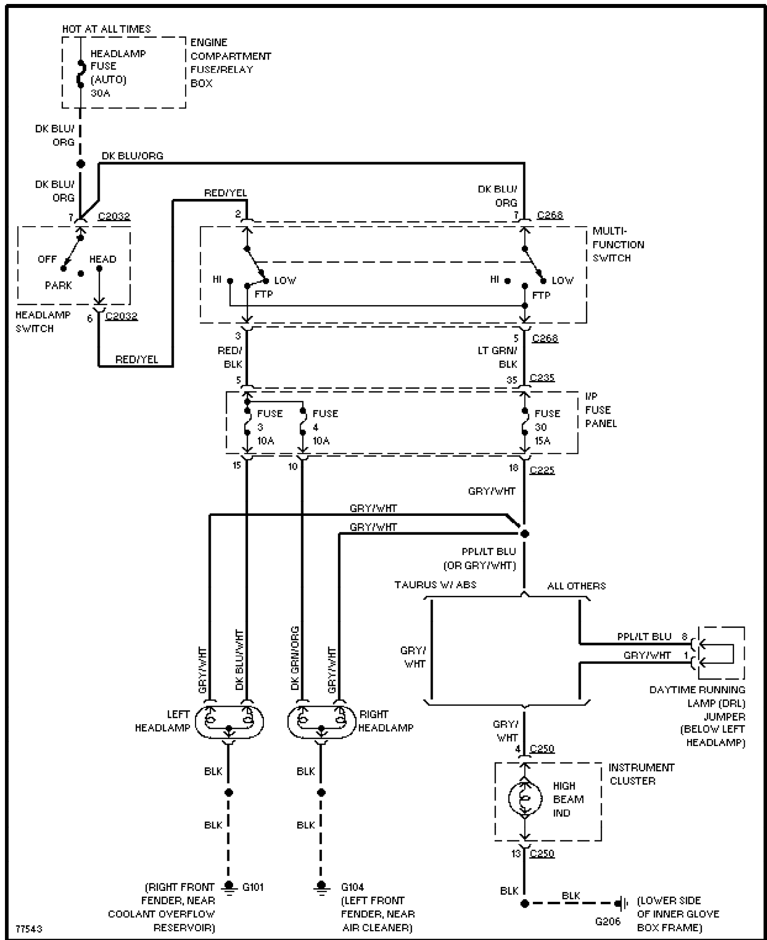
Fig. 44: Headlamps Circuit, W/O DRL 1996 Ford Taurus LX
