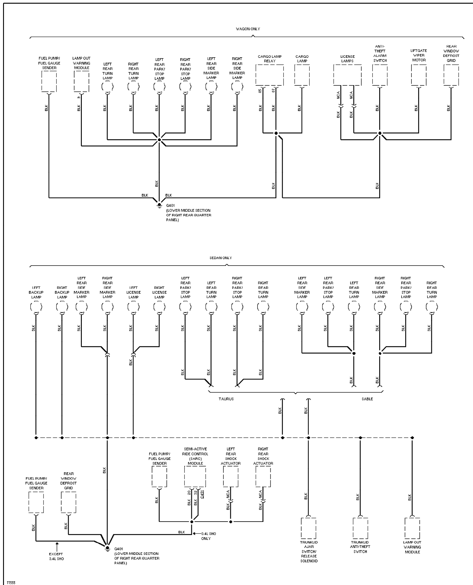
Fig. 40: Ground Distribution Circuit (3 of 3) 1996 Ford Taurus LX
