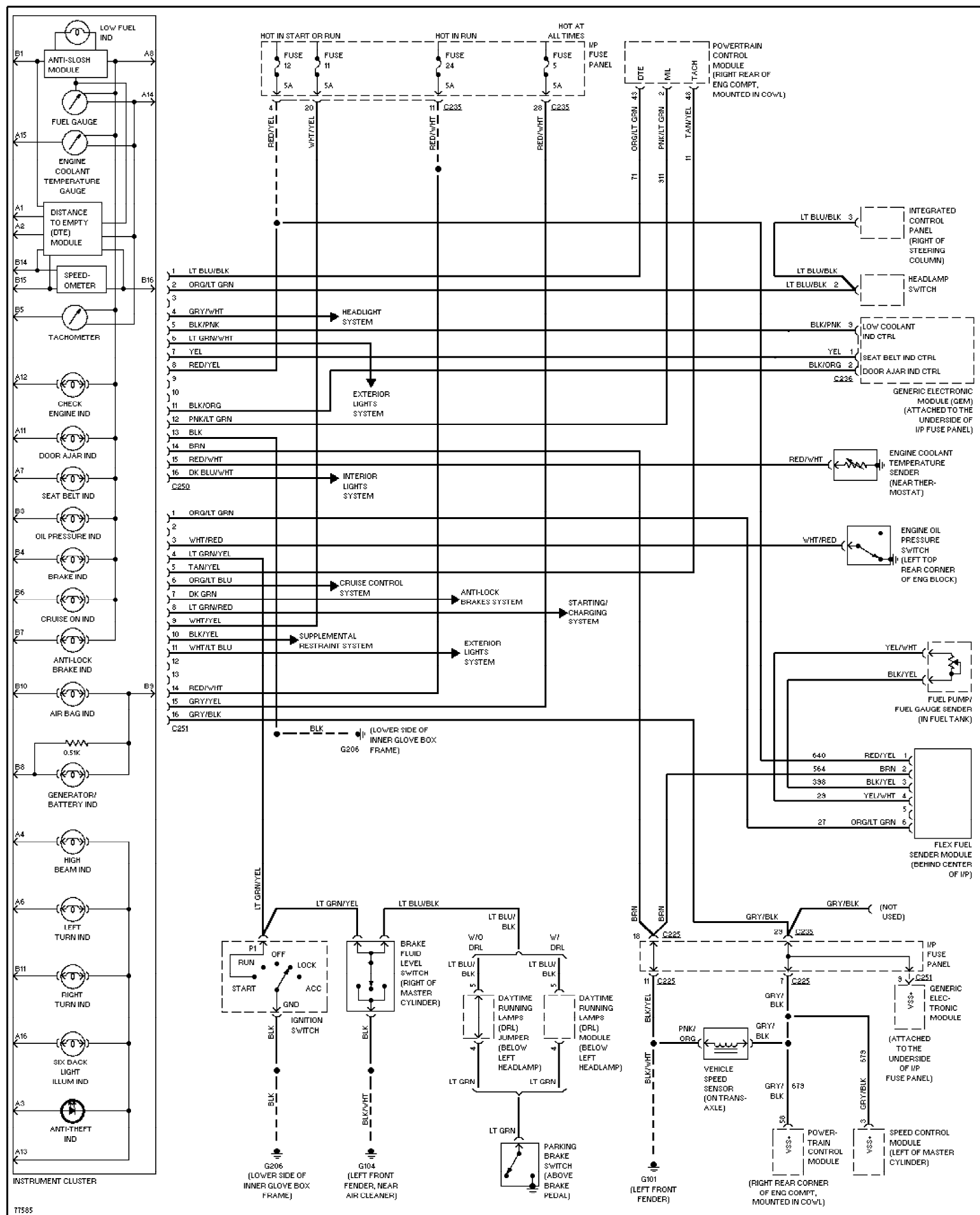
Fig. 46: 3.0L Flex Fuel, Instrument Cluster Circuit 1996 Ford Taurus LX
