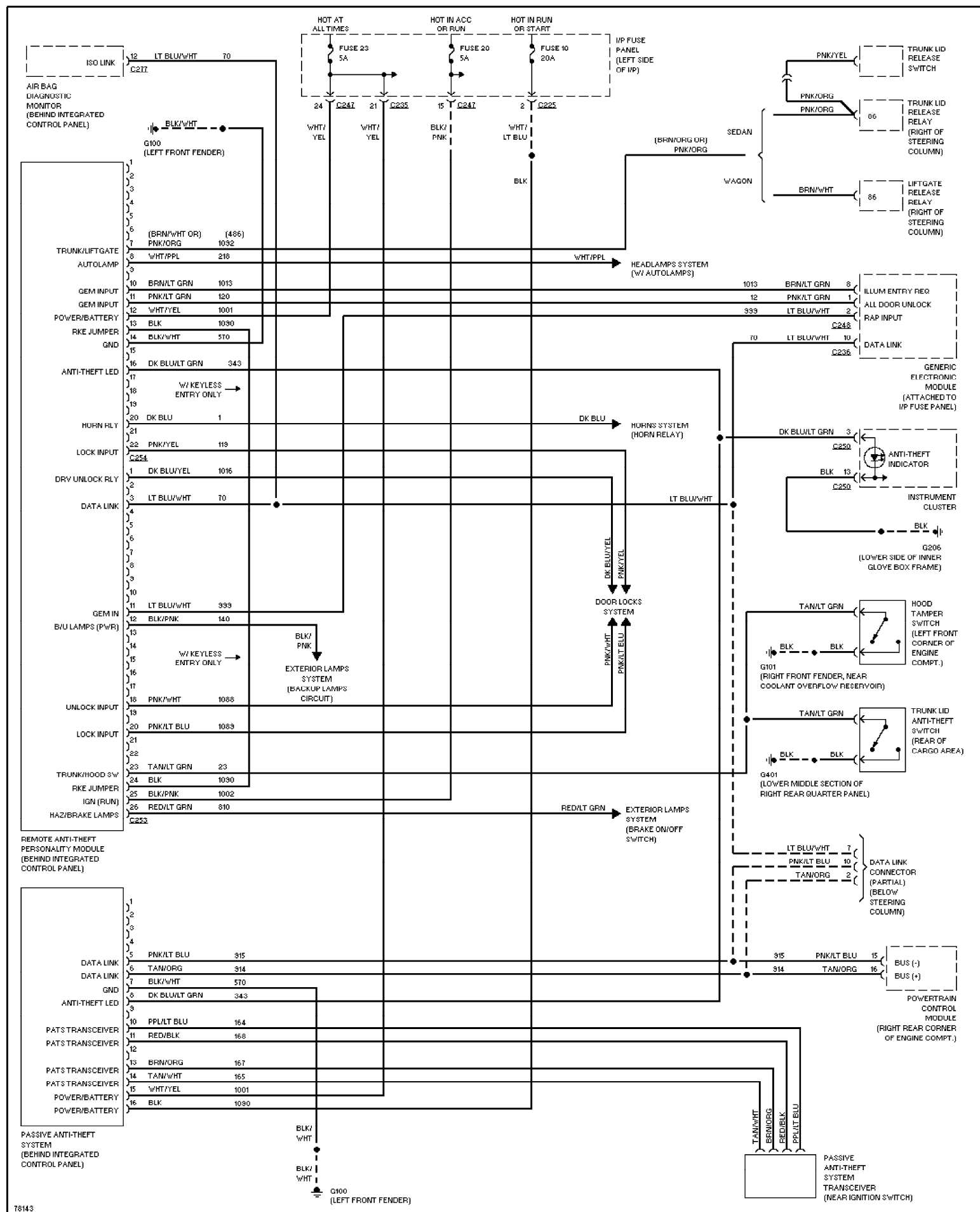
Fig. 4: Anti-theft Circuit 1996 Ford Taurus LX
