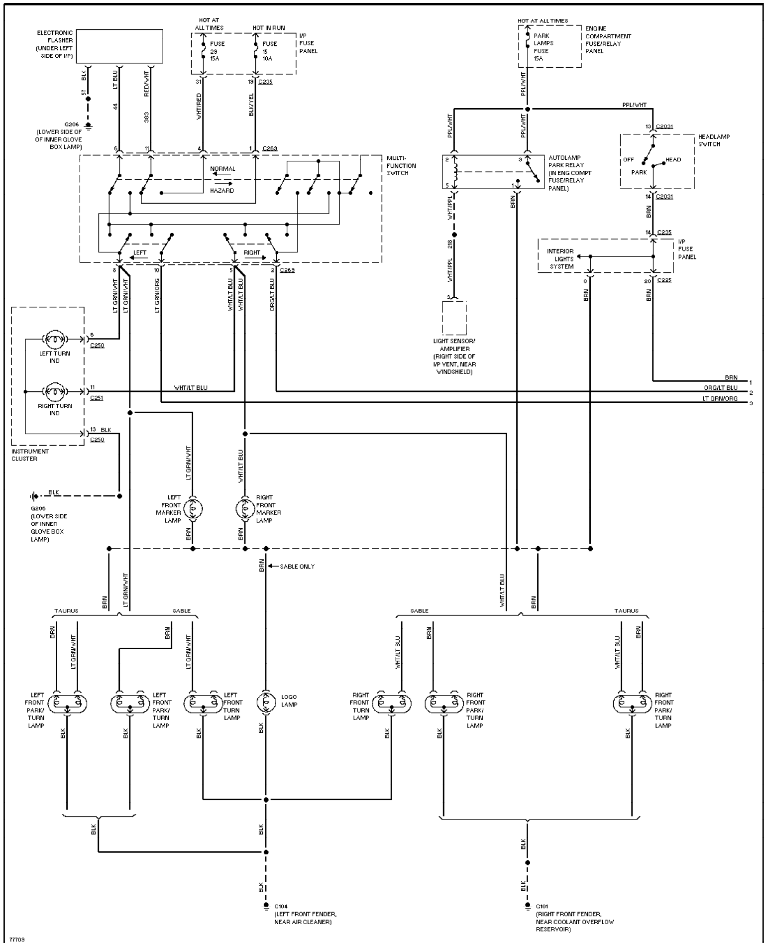
Fig. 35: Exterior Lamps Circuit, Wagon W/O Lamp Out Warning (1 of 2)
