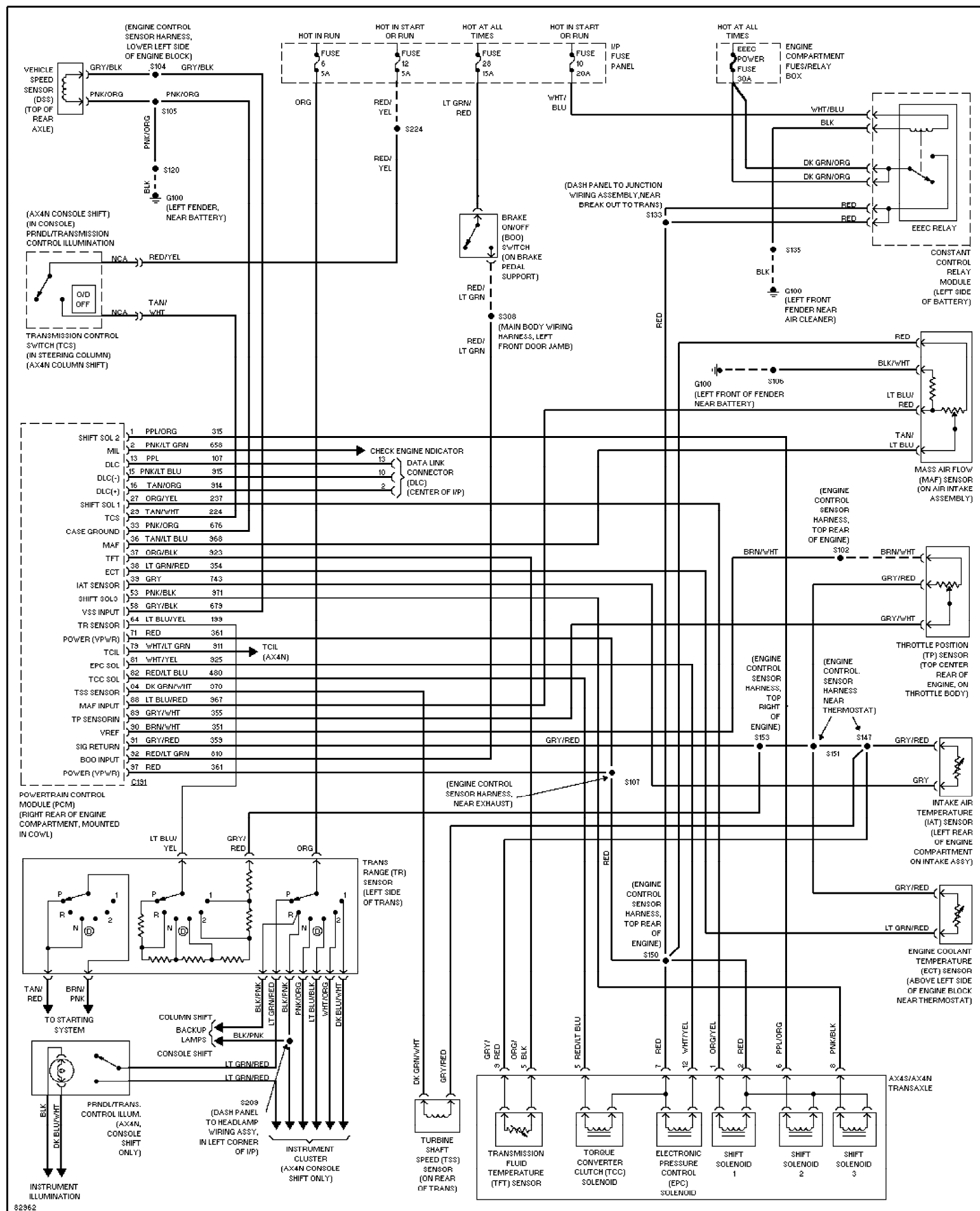
Fig. 73: 3.0L 24-Valve, Transmission Circuit 1996 Ford Taurus LX
