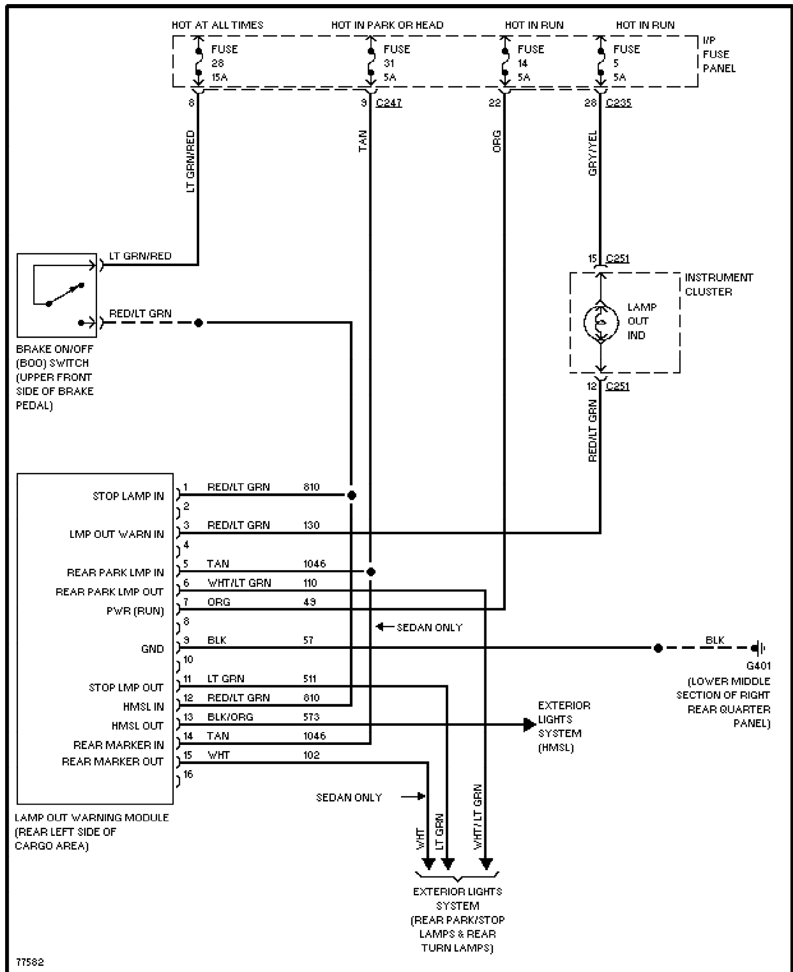
Fig. 50: Lamp Monitor Circuit 1996 Ford Taurus LX
