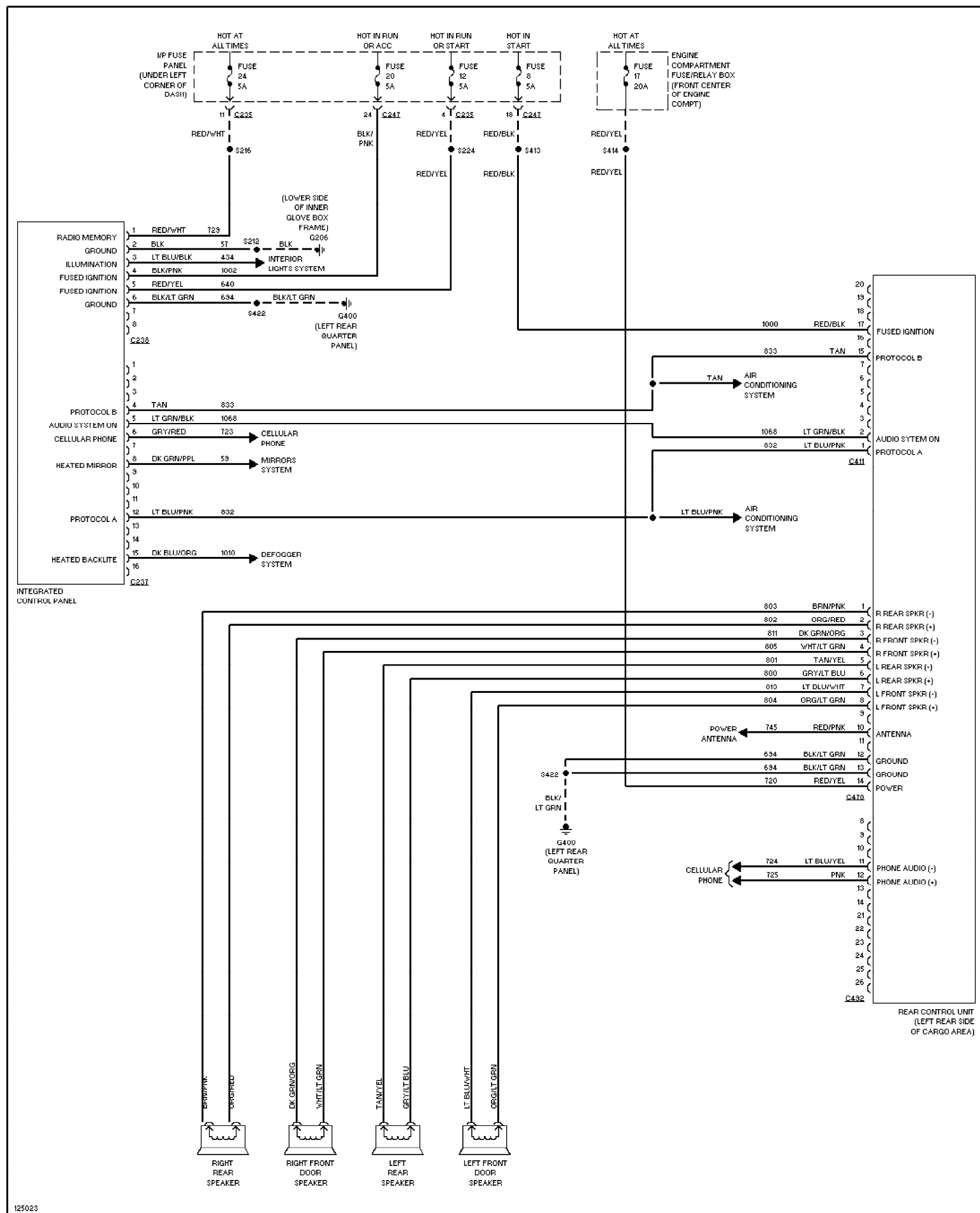
Fig. 63: Radio Circuits, W/O Cassette Deck 1996 Ford Taurus LX
