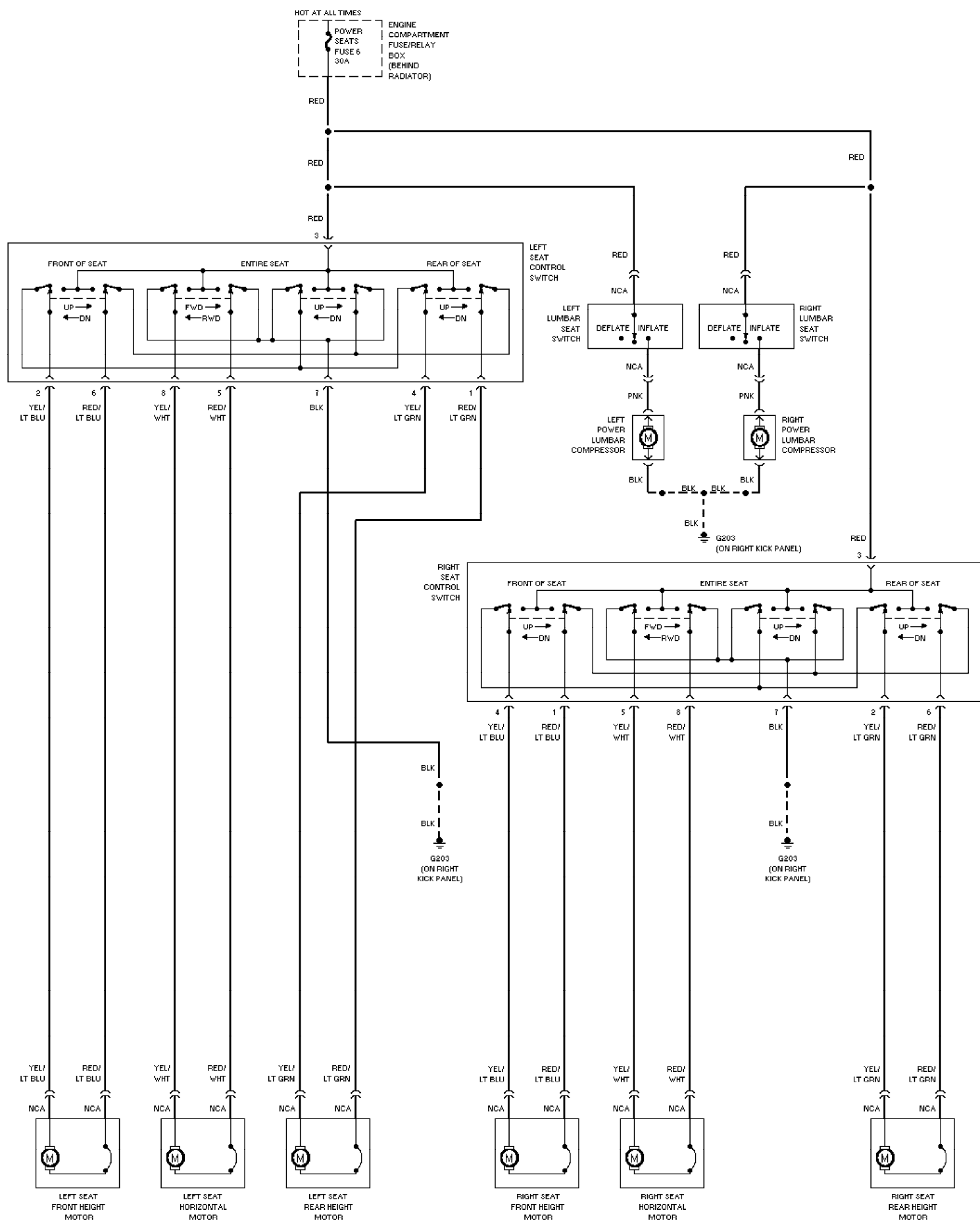
Fig. 59: Power & Lumbar Seat Circuit 1996 Ford Taurus LX
