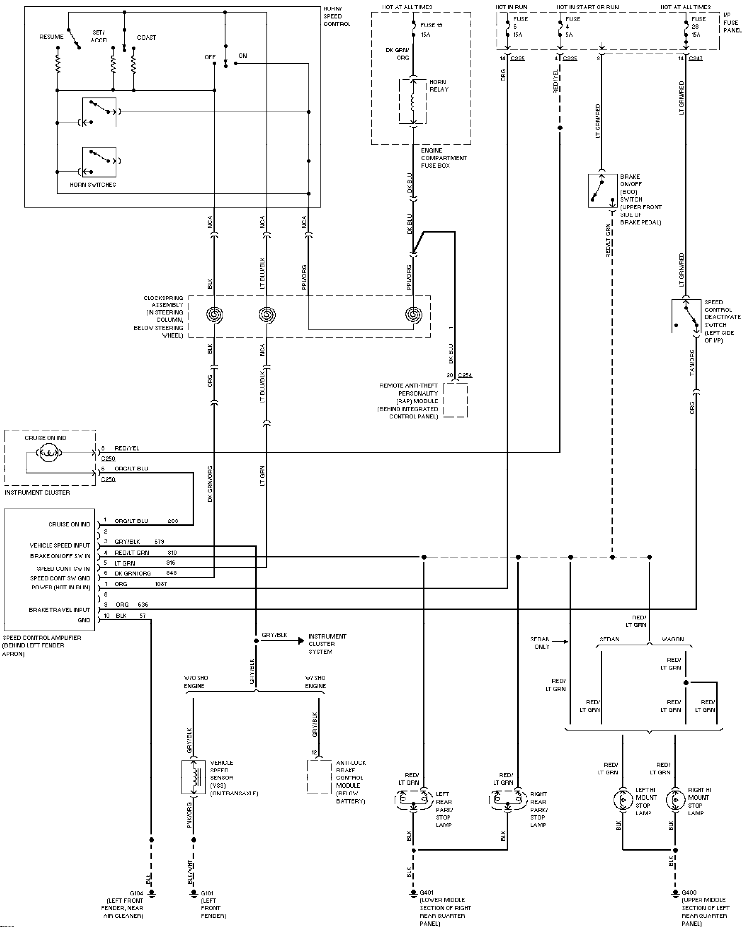
Fig. 8: Cruise Control Circuit 1996 Ford Taurus LX
