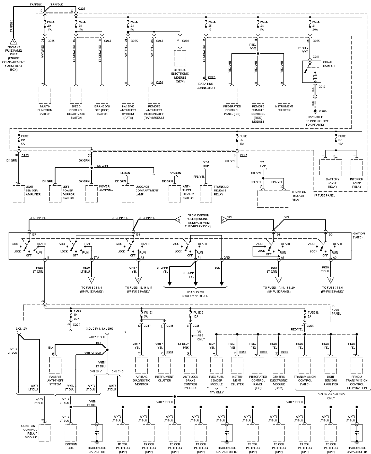
Fig. 55: Power Distribution Circuit (2 of 3) 1996 Ford Taurus LX
