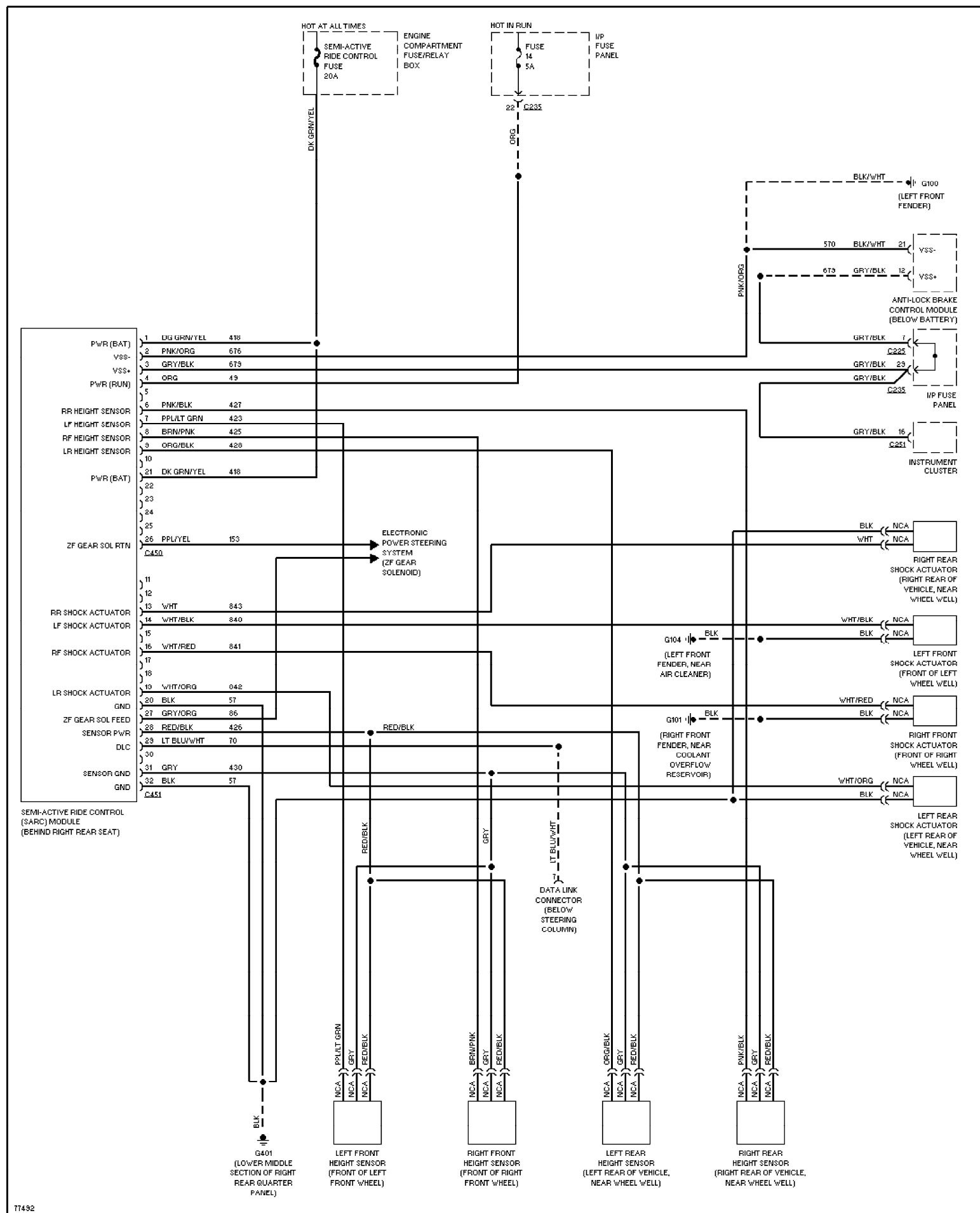
Fig. 14: Electronic Suspension Circuit 1996 Ford Taurus LX
