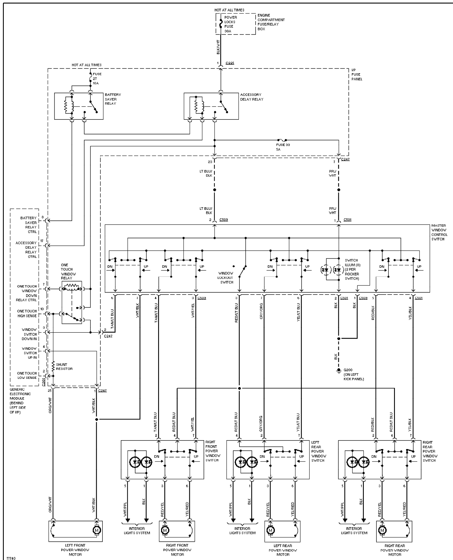
Fig. 61: Power Window Circuit 1996 Ford Taurus LX
