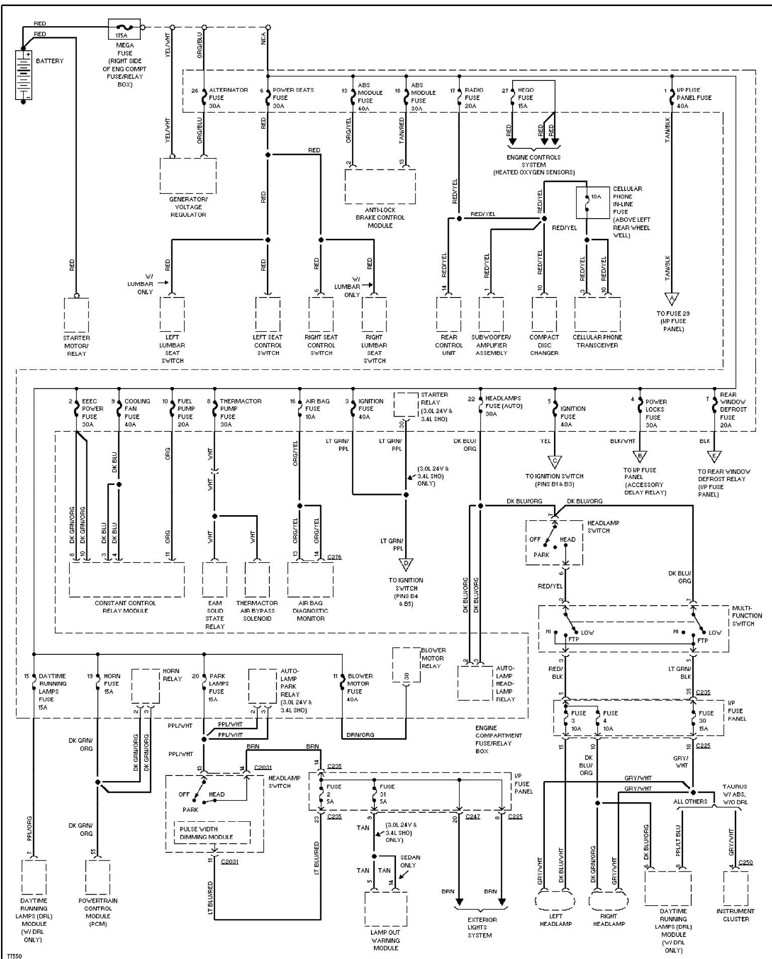
Fig. 54: Power Distribution Circuit (1 of 3) 1996 Ford Taurus LX
