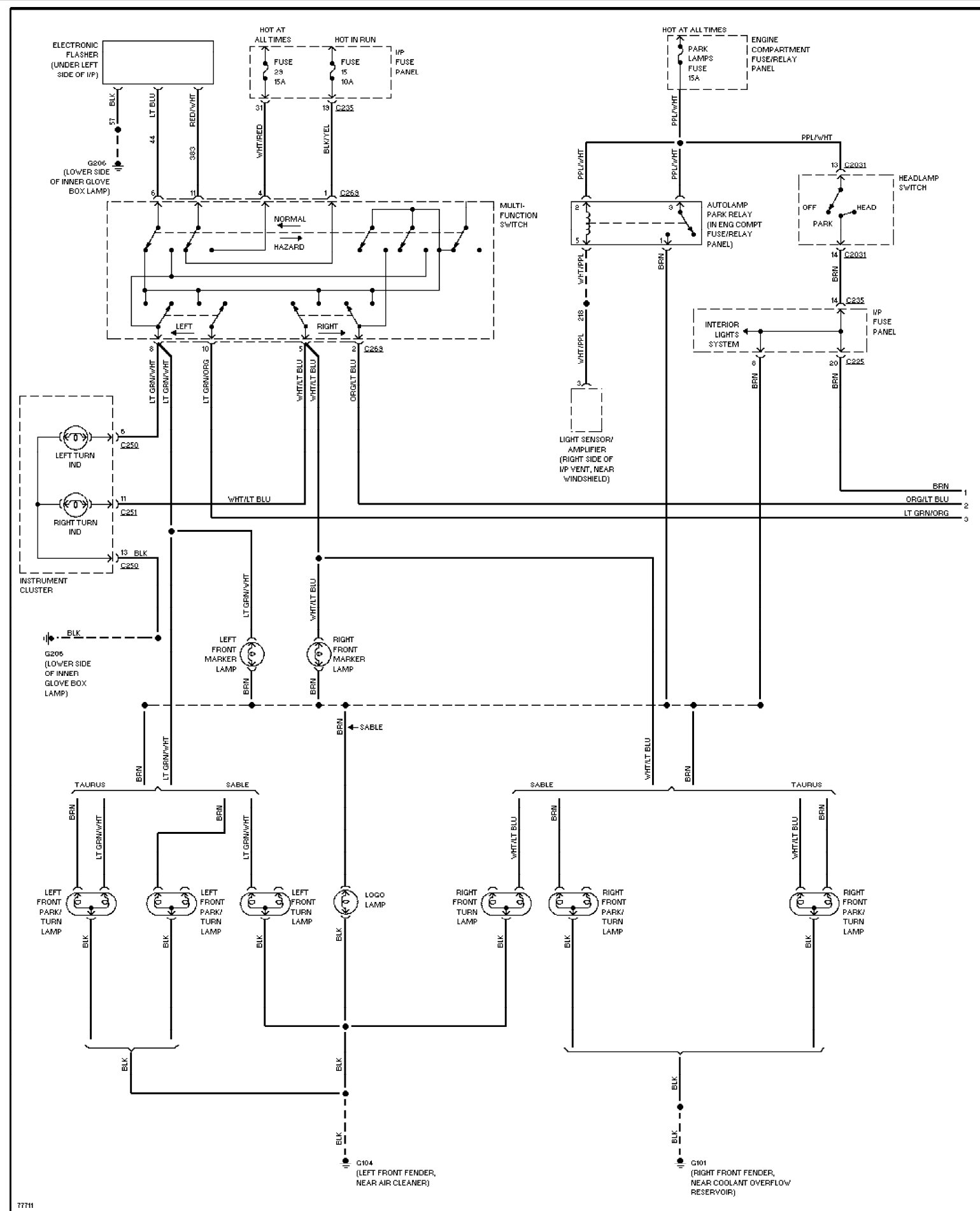
Fig. 33: Exterior Lamps Circuit, Wagon W/ Lamp Out Warning (1 of 2)
