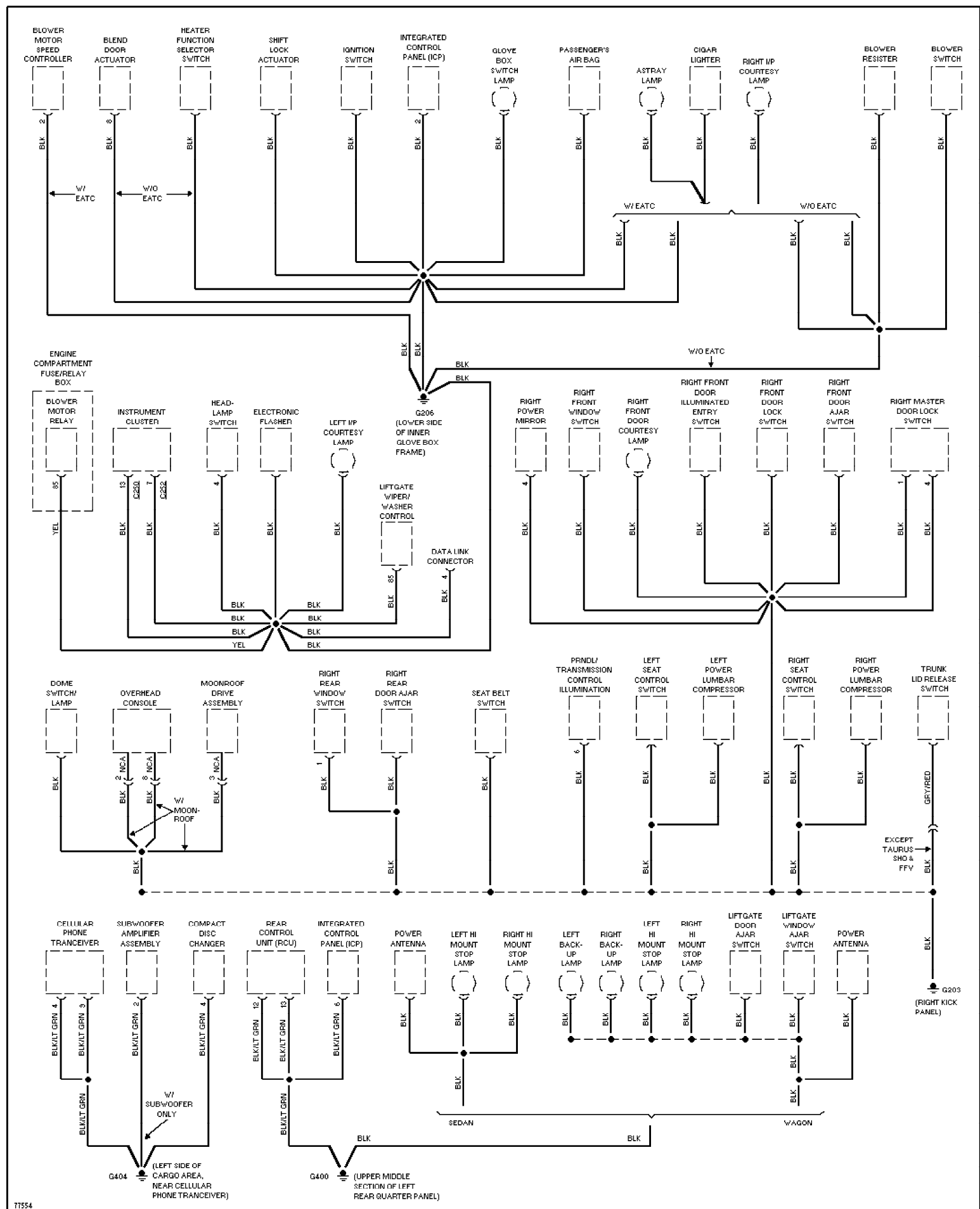
Fig. 39: Ground Distribution Circuit (2 of 3) 1996 Ford Taurus LX
