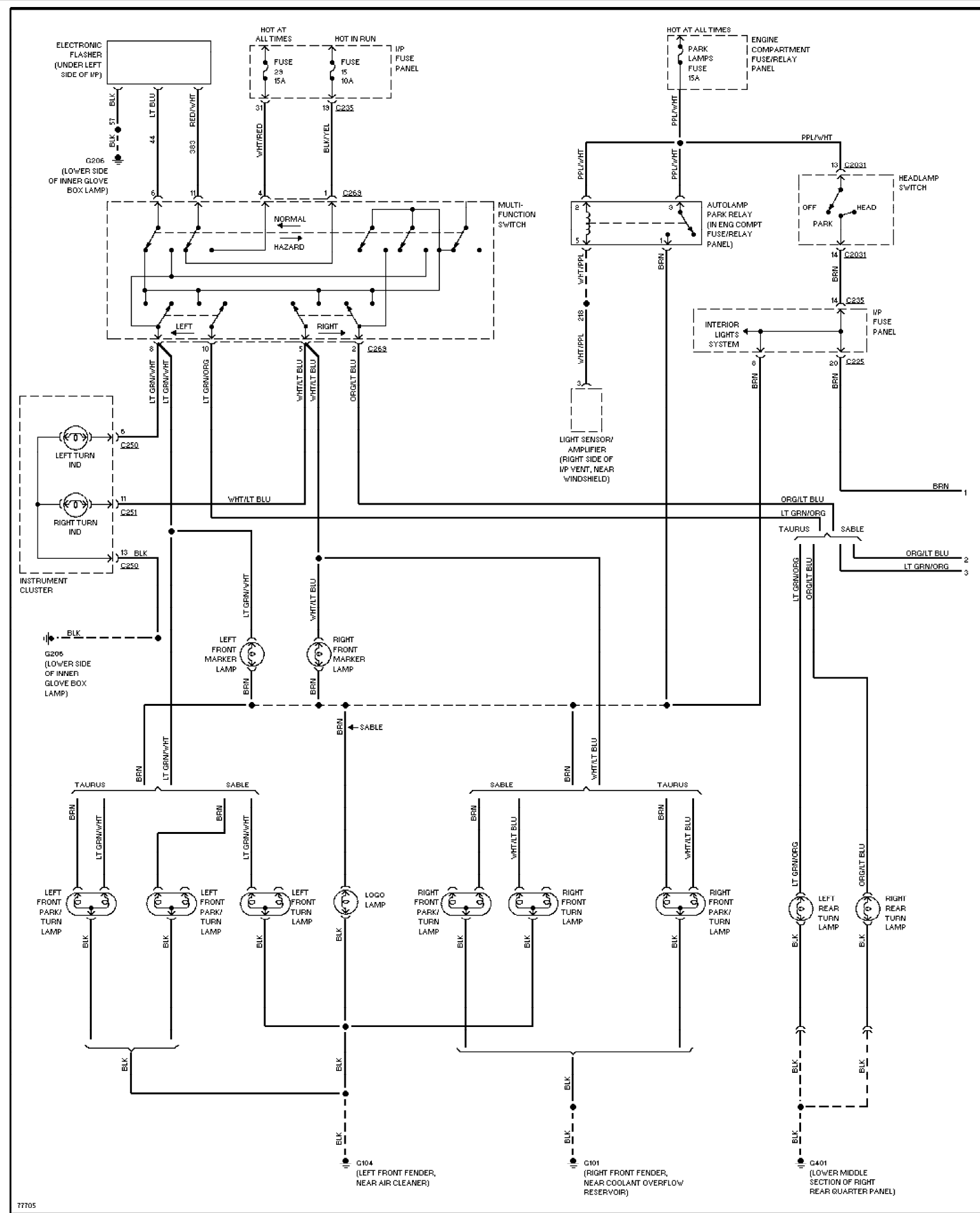
Fig. 31: Exterior Lamps Circuit, Sedan W/O Lamp Out Warning (1 of 2)
