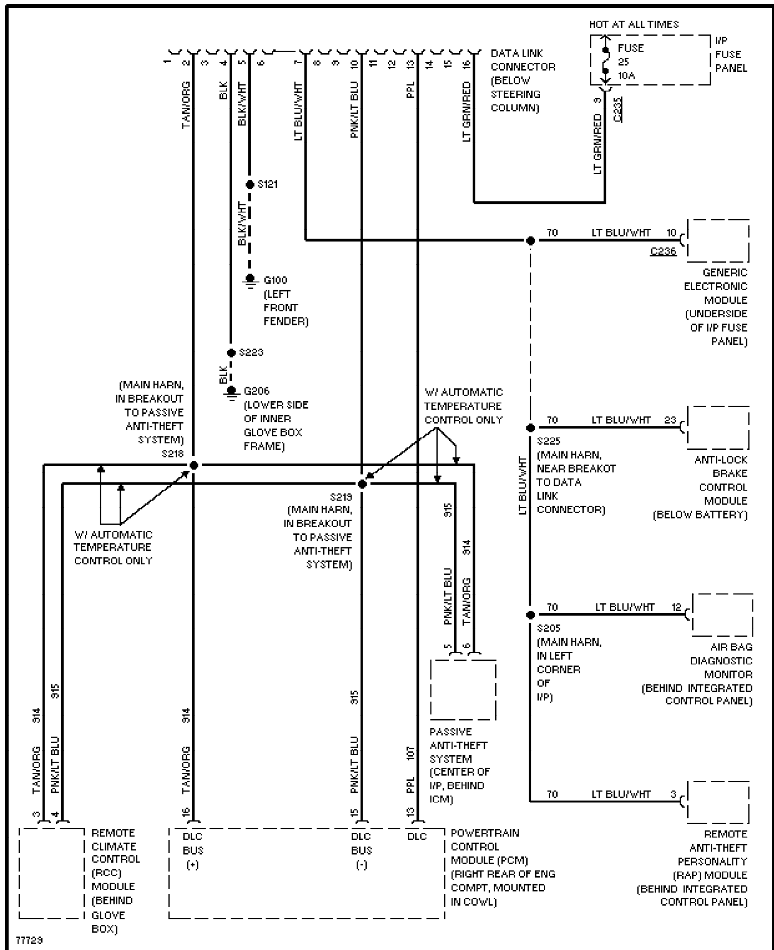
Fig. 6: Computer Data Lines 1996 Ford Taurus LX
