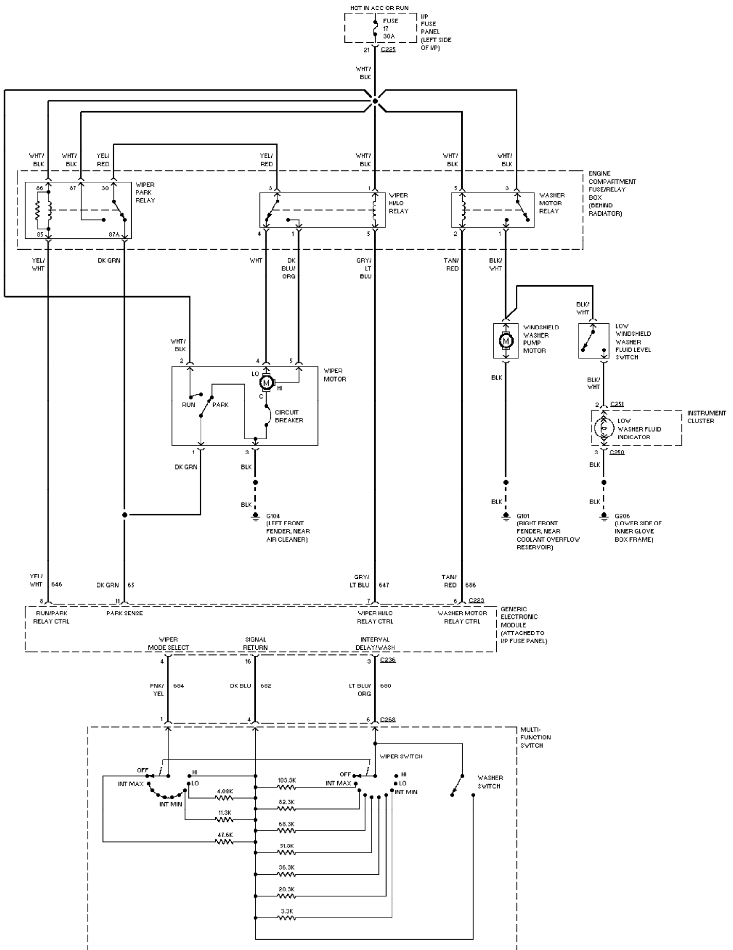
Fig. 78: Front Wiper/Washer Circuit 1996 Ford Taurus LX
