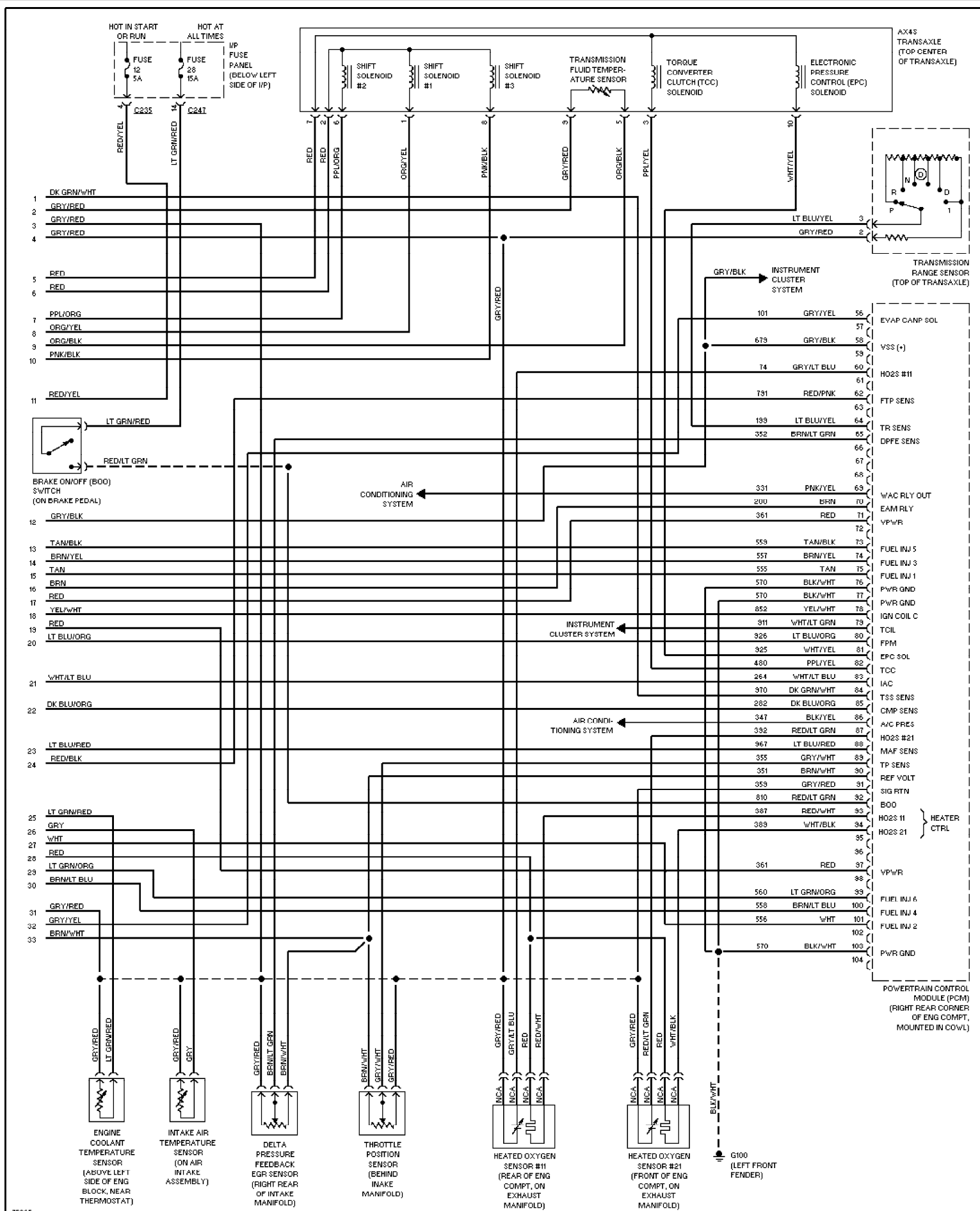
Fig. 23: 3.0L Flex Fuel, Engine Performance Circuits (3 of 3)
