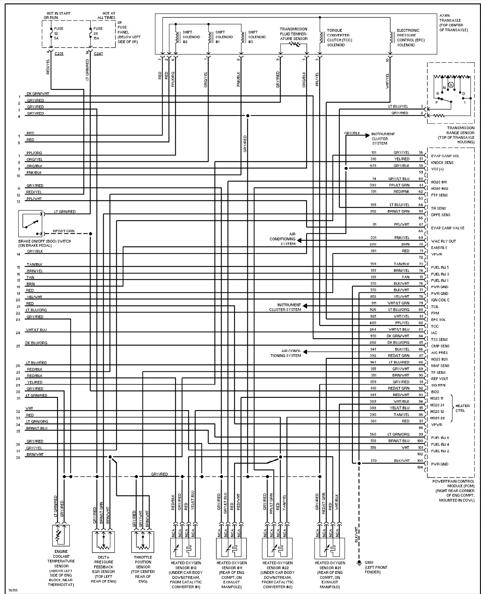
Fig. 20: 3.0L 24-Valve, Engine Performance Circuits (3 of 3)
