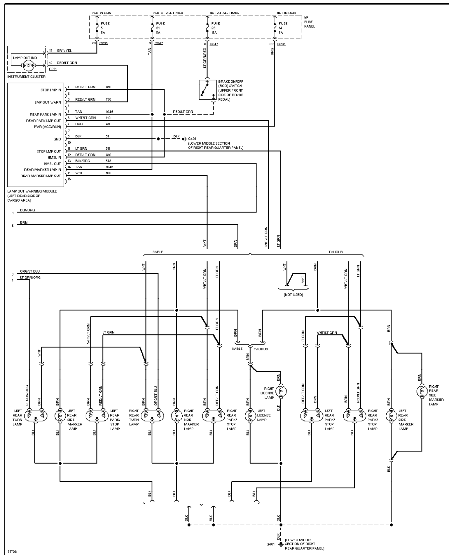
Fig. 30: Exterior Lamps Circuit, Sedan W/ Lamp Out Warning (2 of 2)
