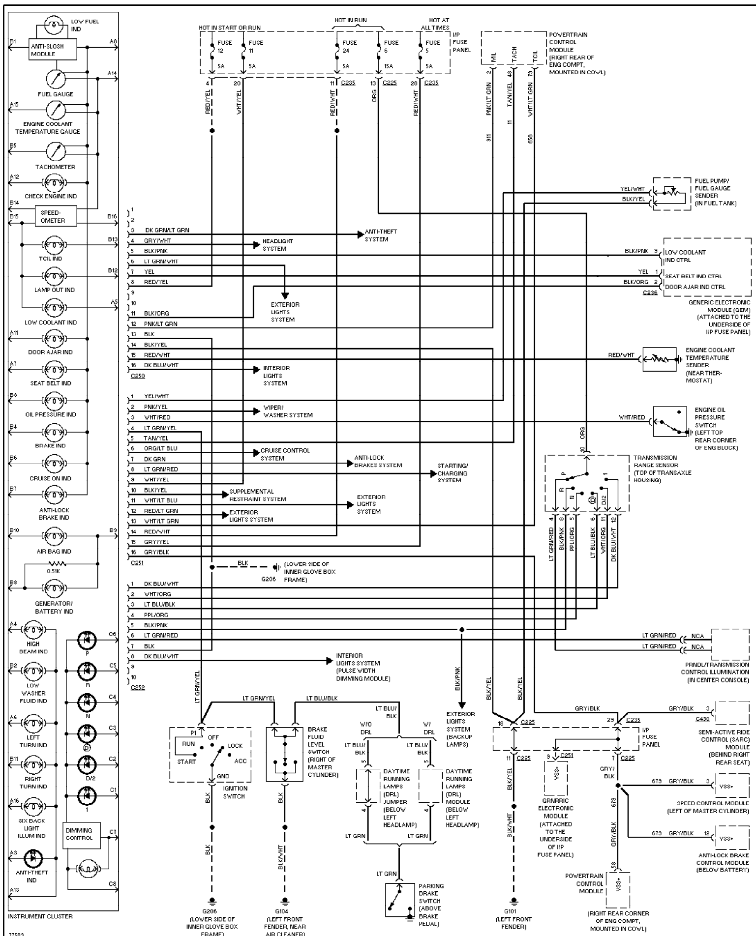
Fig. 47: 3.0L, Instrument Cluster Circuit 1996 Ford Taurus LX
