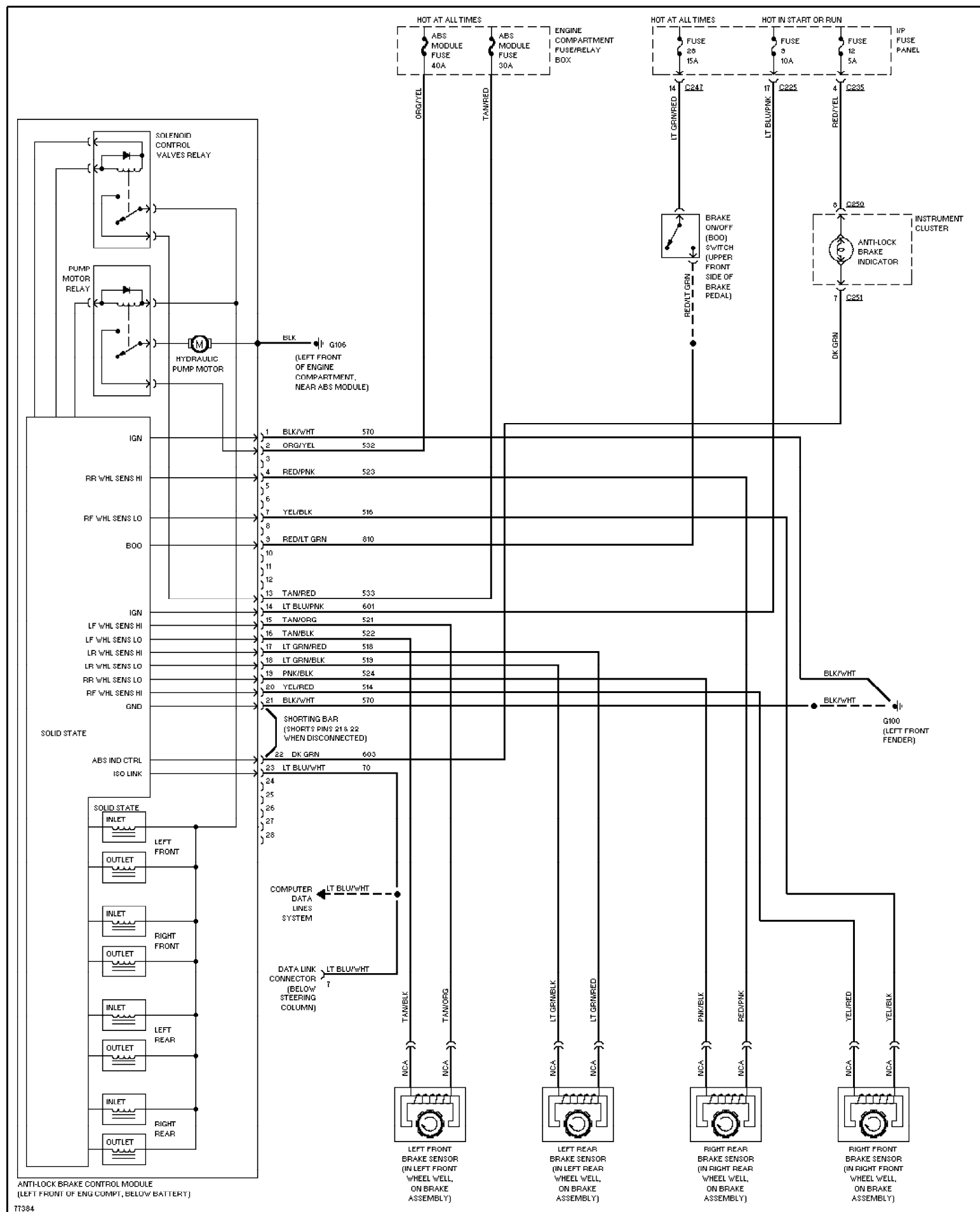
Fig. 3: Anti-lock Brake Circuits 1996 Ford Taurus LX
