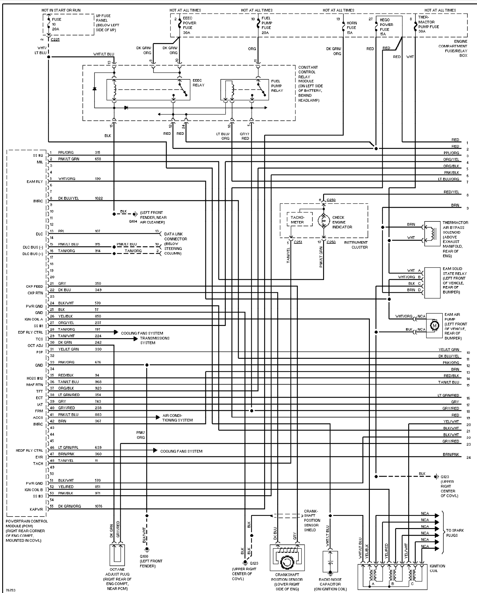
Fig. 18: 3.0L 24-Valve, Engine Performance Circuits (1 of 3)
