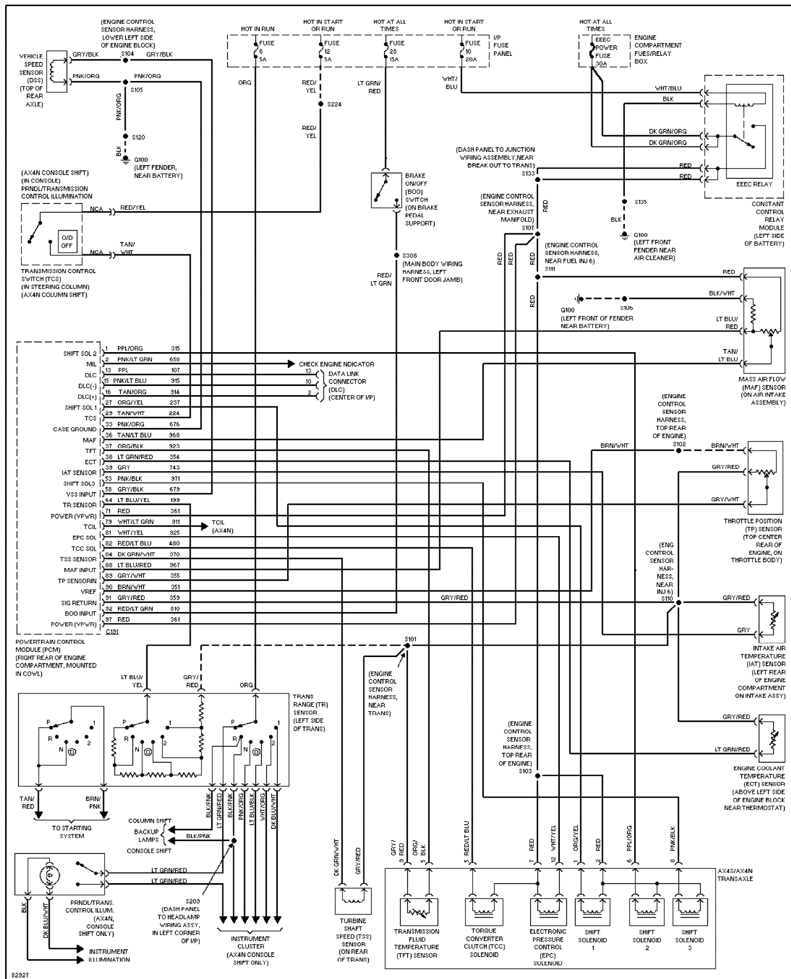
Fig. 72: 3.0L 12-Valve, Transmission Circuit 1996 Ford Taurus LX
