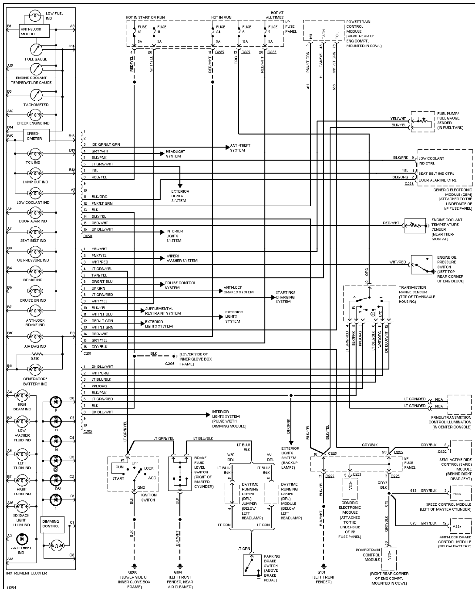
Fig. 49: 3.4L SHO, Instrument Cluster Circuit 1996 Ford Taurus LX
