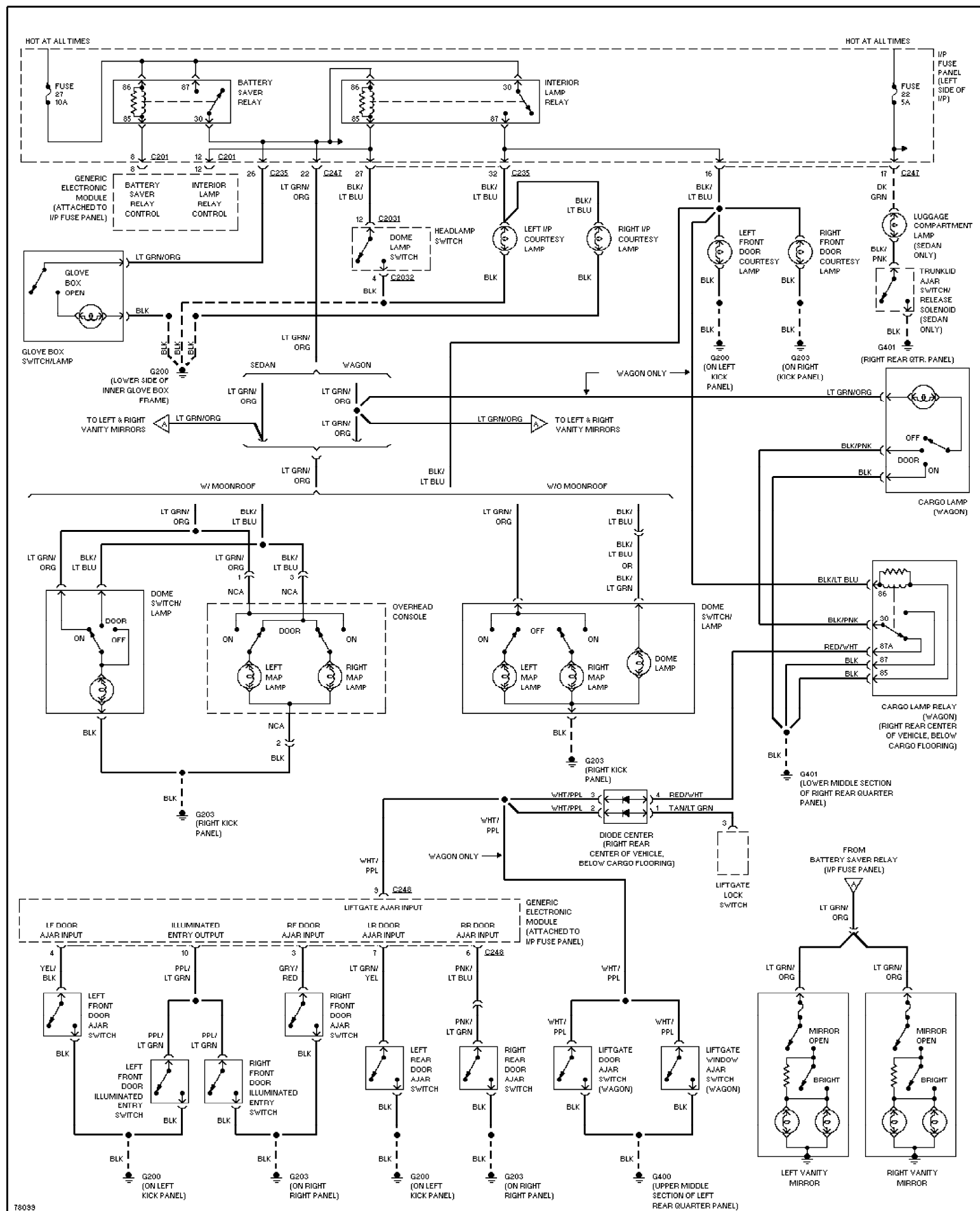
Fig. 51: Courtesy Lamps Circuit 1996 Ford Taurus LX
