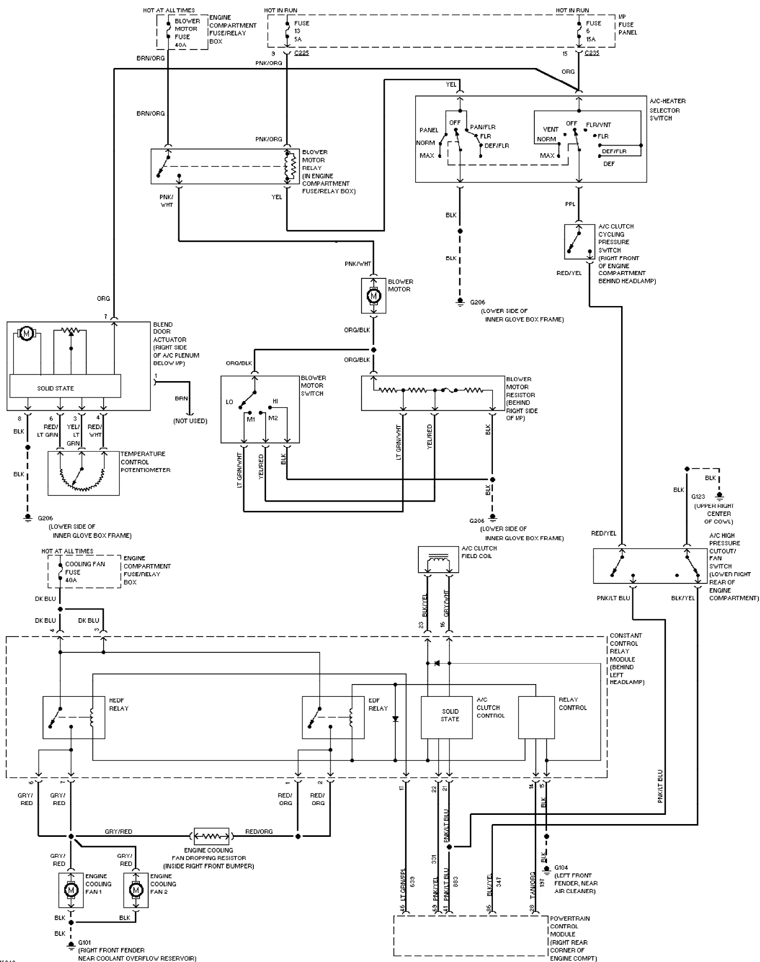
Fig. 2: A/C Circuit, Manual A/C 1996 Ford Taurus LX
