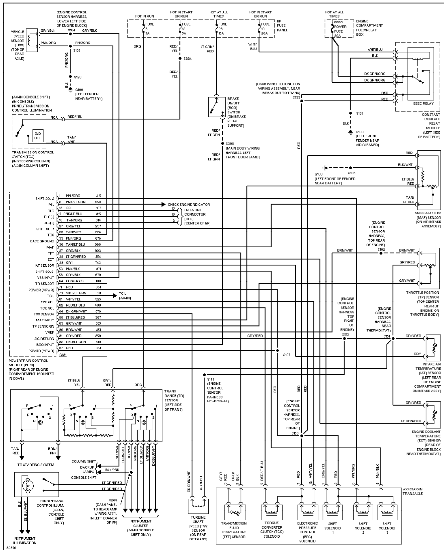
Fig. 75: 3.4L SHO, Transmission Circuit 1996 Ford Taurus LX
