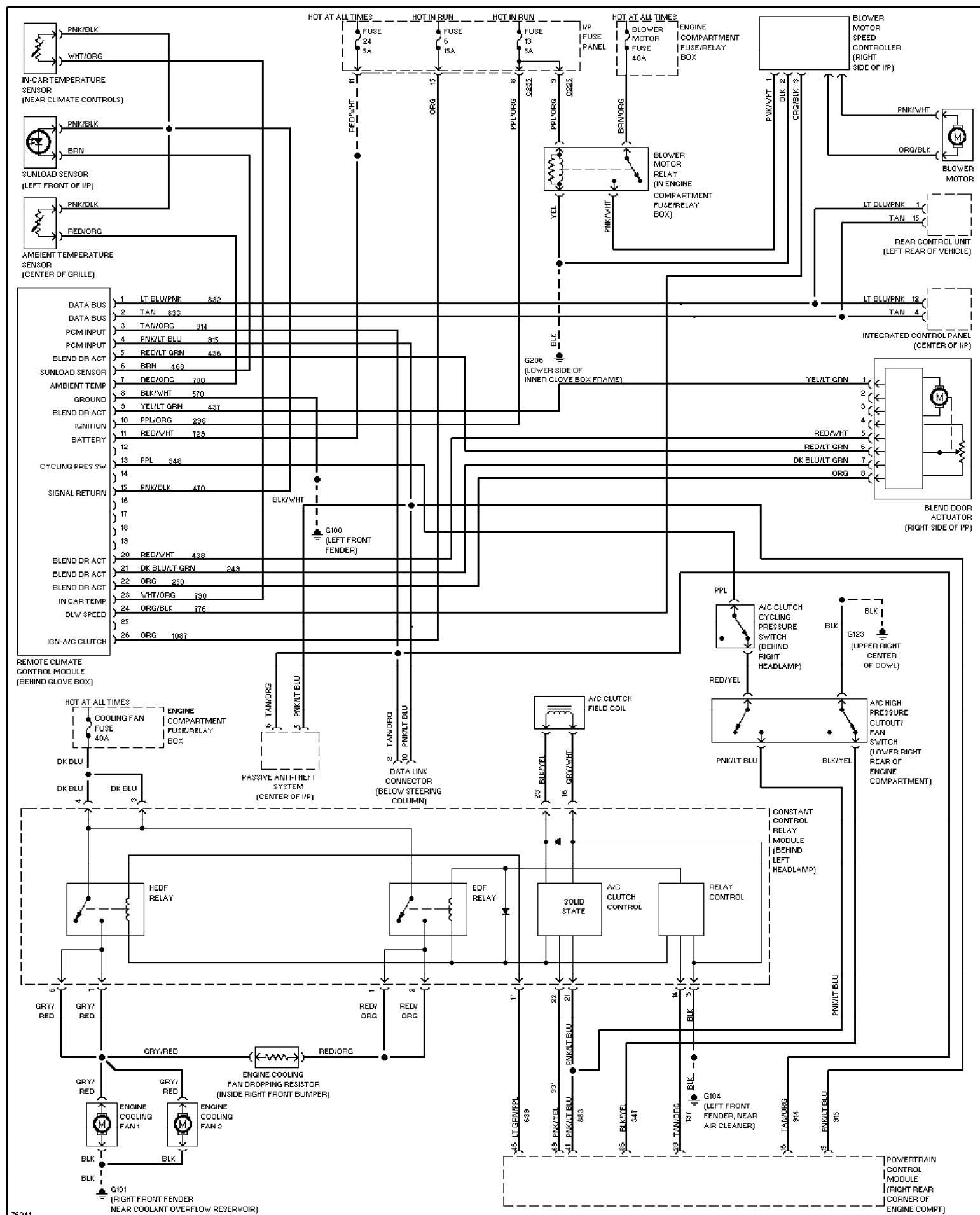
Fig. 1: A/C Circuit, Auto A/C 1996 Ford Taurus LX
