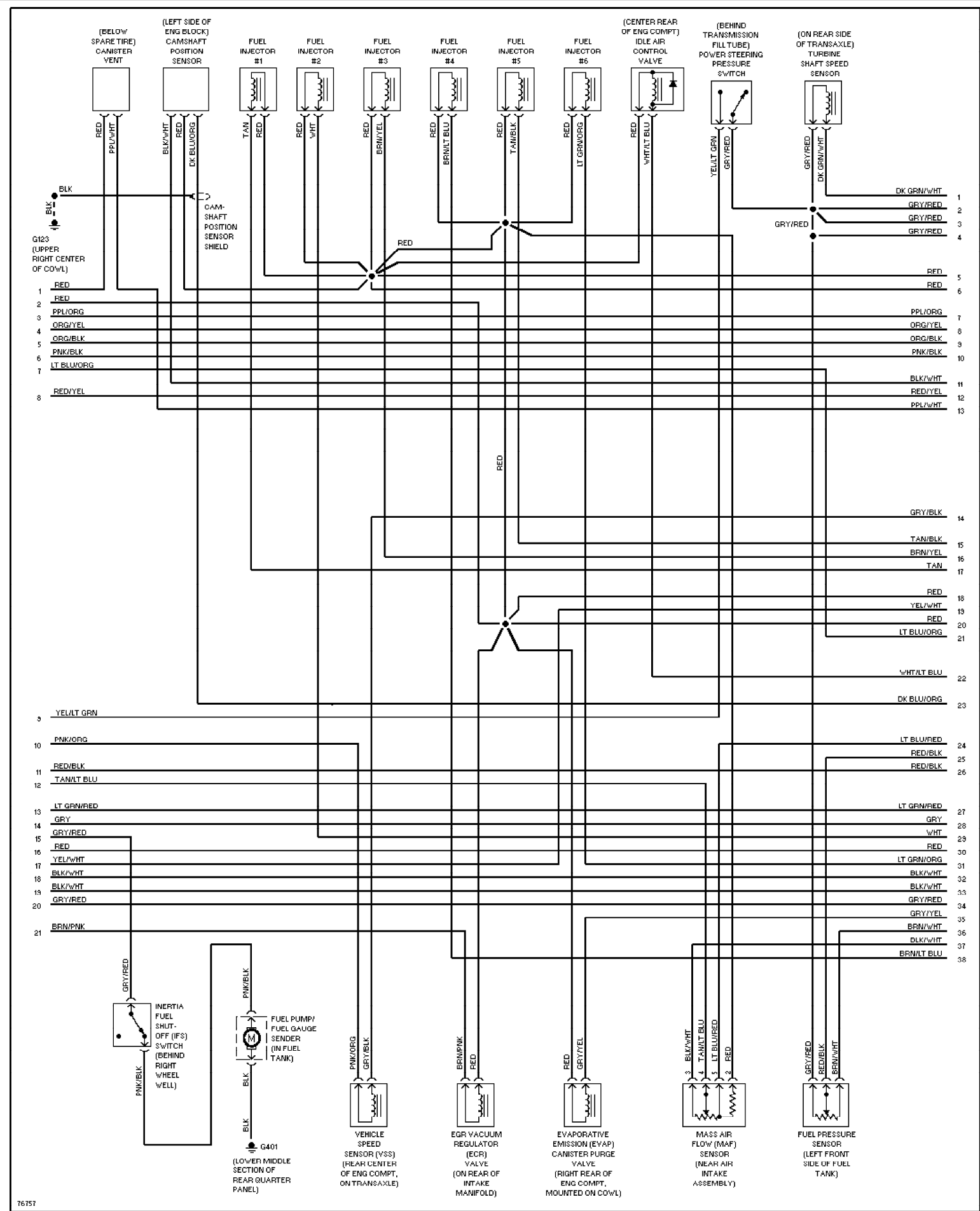
Fig. 16: 3.0L 12-Valve, Engine Performance Circuits (2 of 3)
