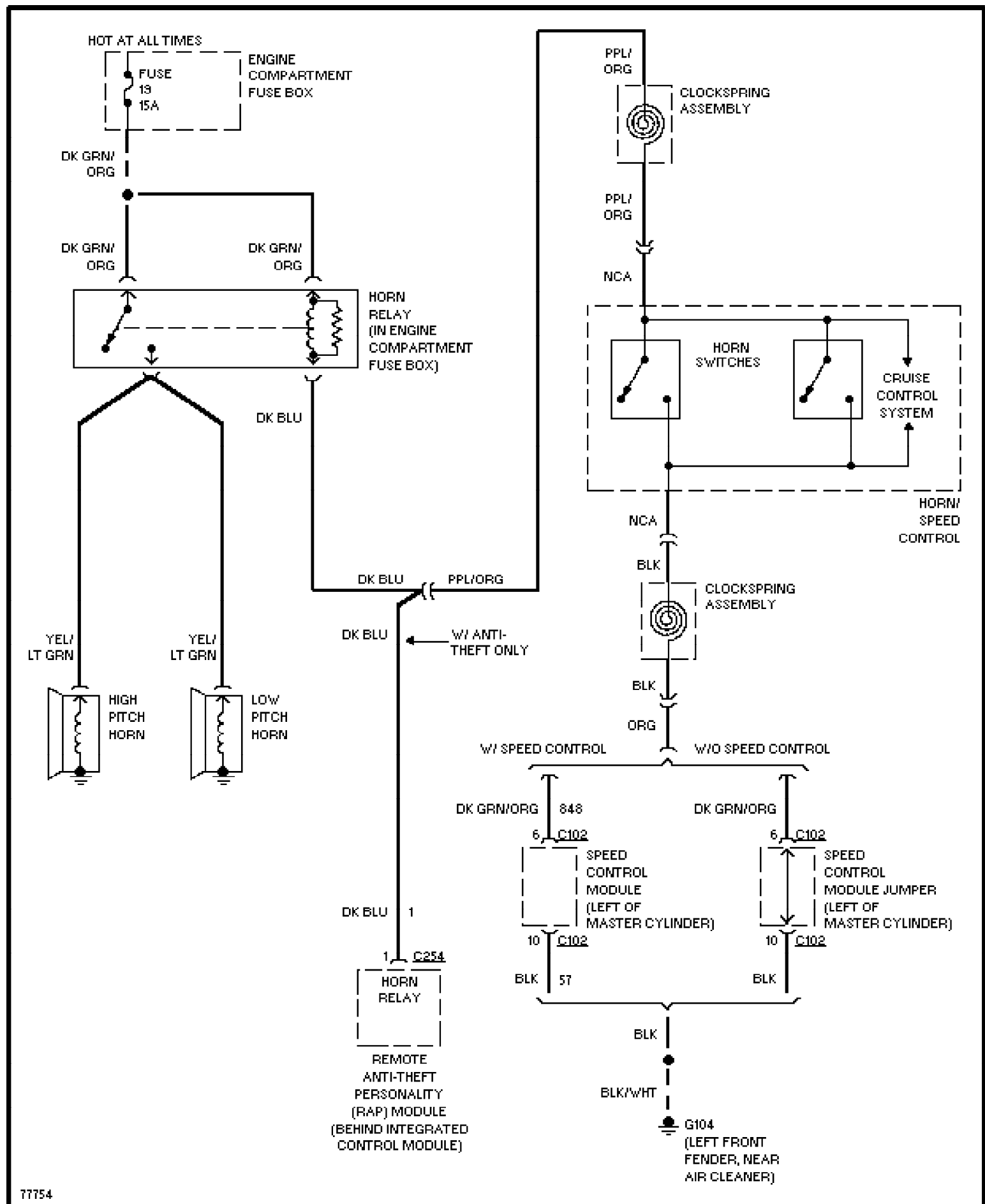
Fig. 45: Horn Circuit 1996 Ford Taurus LX
