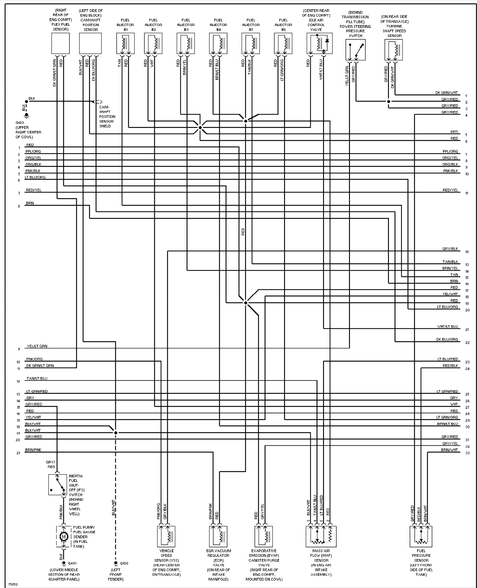
Fig. 22: 3.0L Flex Fuel, Engine Performance Circuits (2 of 3)
