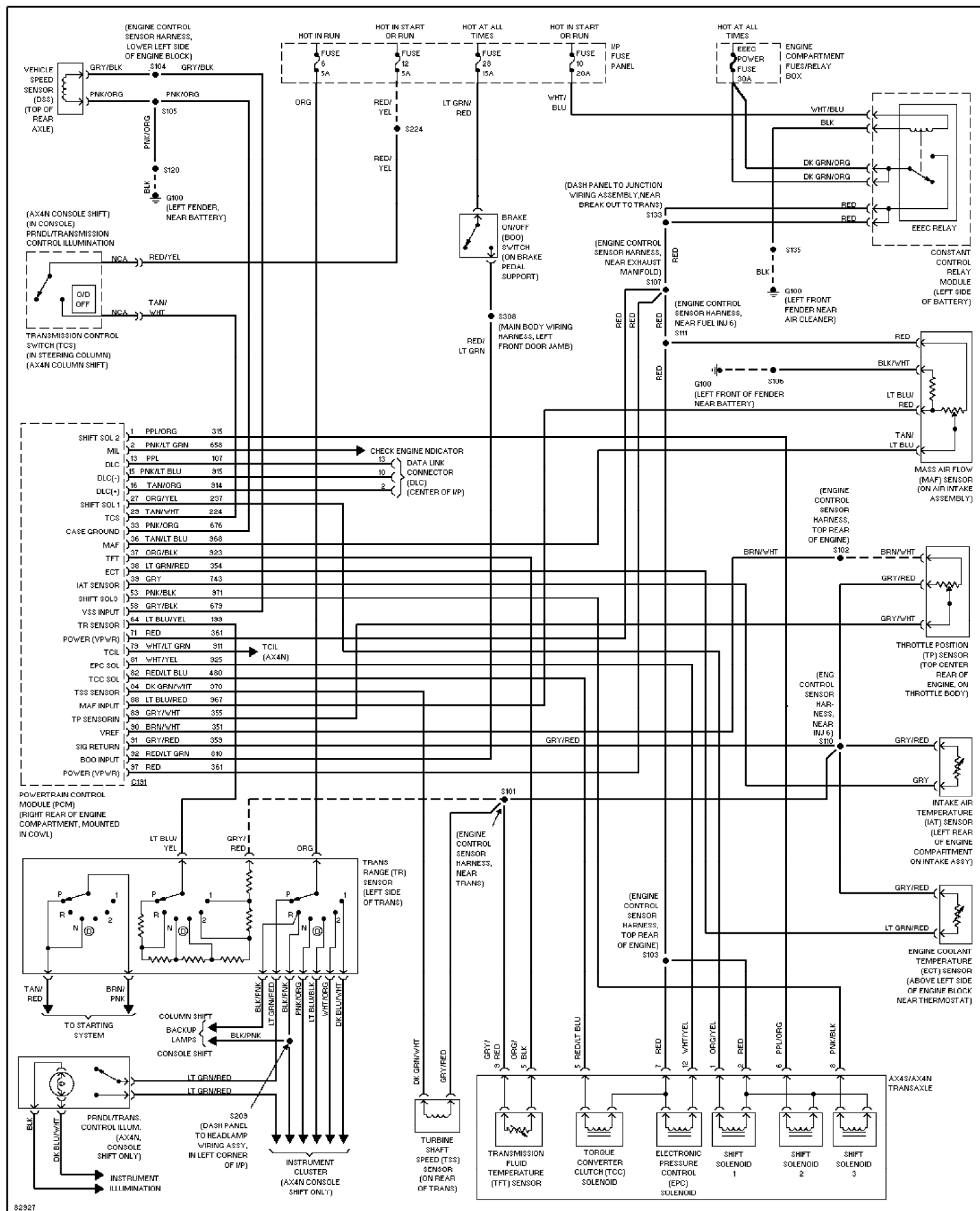
Fig. 74: 3.0L Flex Fuel, Transmission Circuit 1996 Ford Taurus LX
