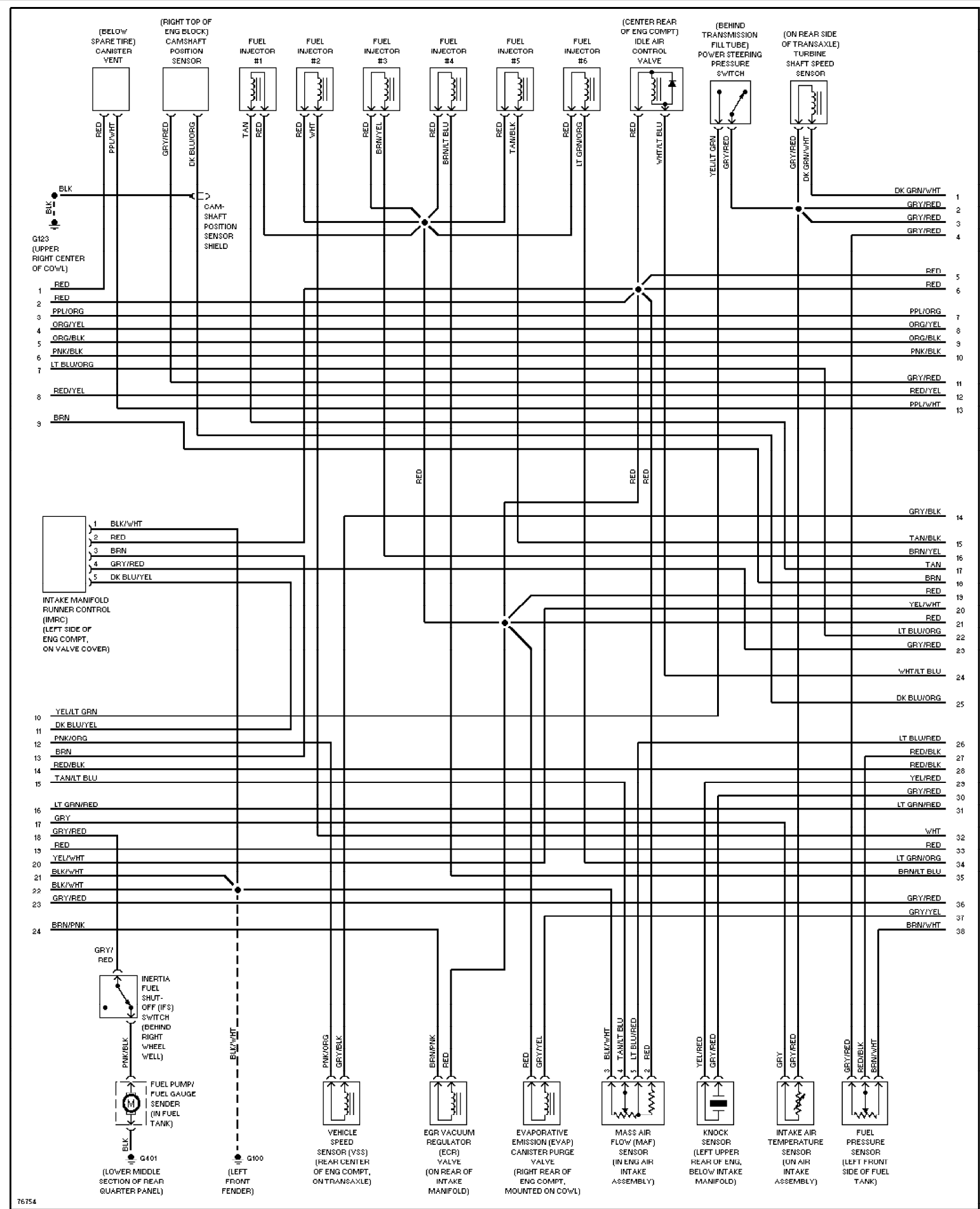
Fig. 19: 3.0L 24-Valve, Engine Performance Circuits (2 of 3)
