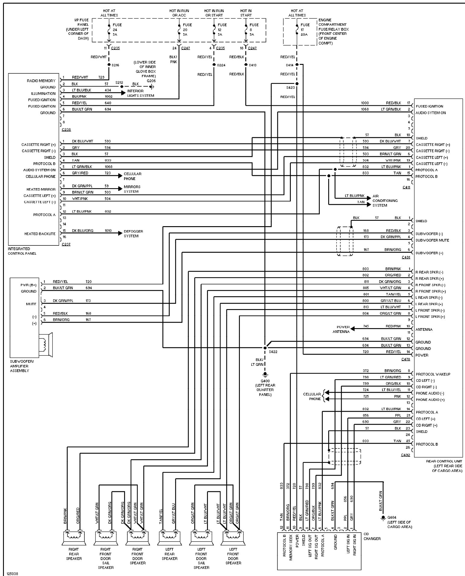
Fig. 62: Radio Circuits, W/ Cassette Deck 1996 Ford Taurus LX
