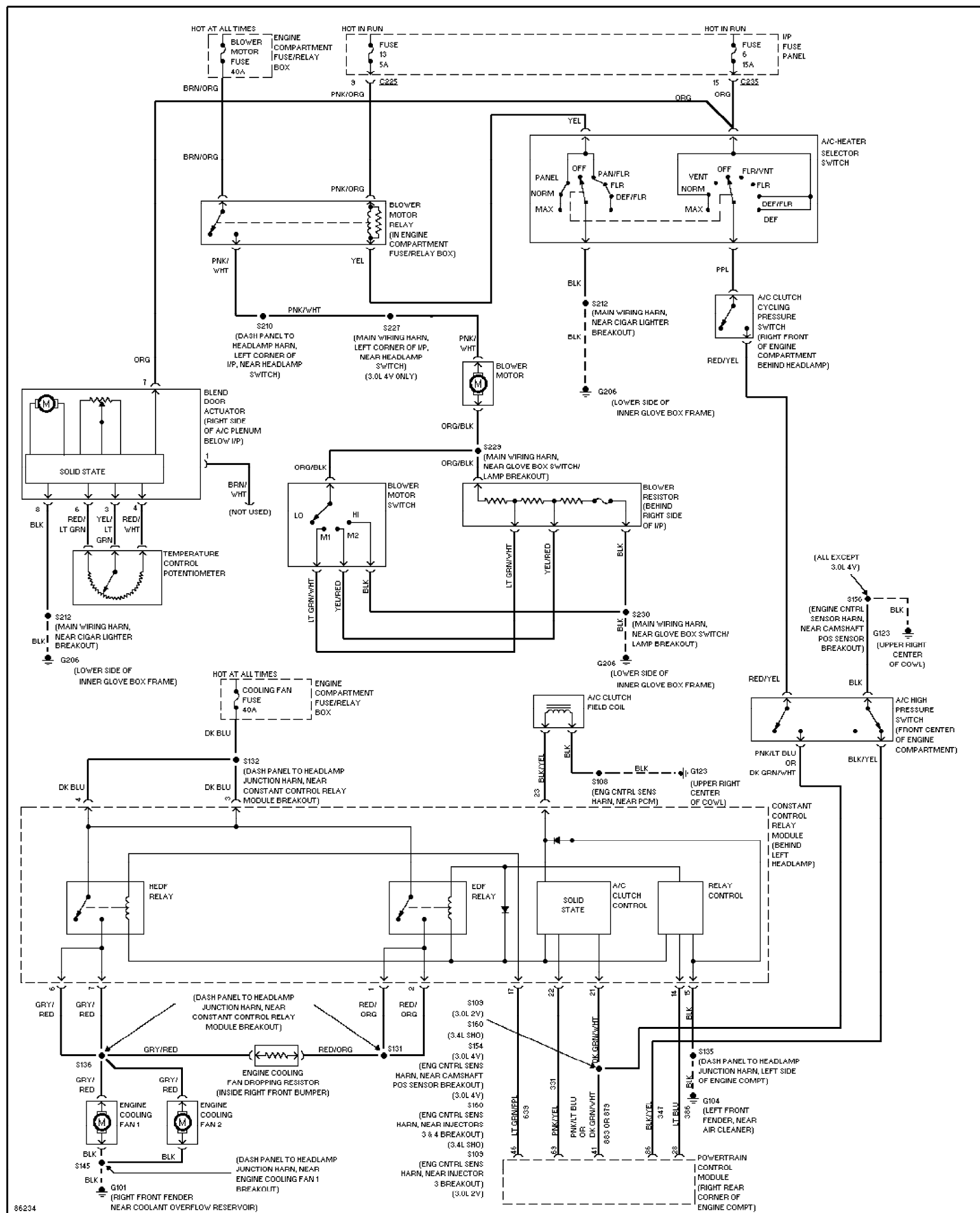
Fig. 2: A/C Circuit, Manual A/C 1997 Ford Taurus LX
