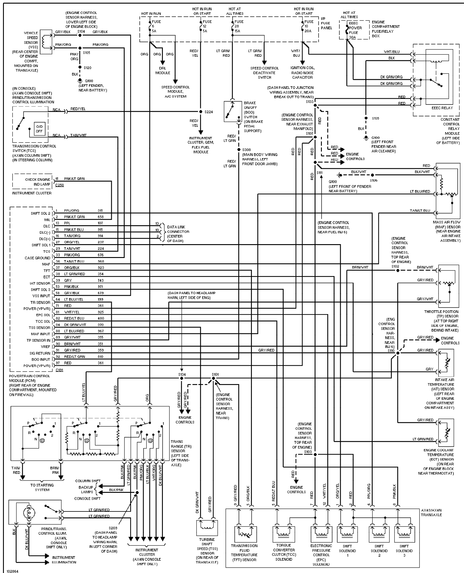
Fig. 71: 3.0L Flex Fuel, Transmission Circuit 1997 Ford Taurus LX
