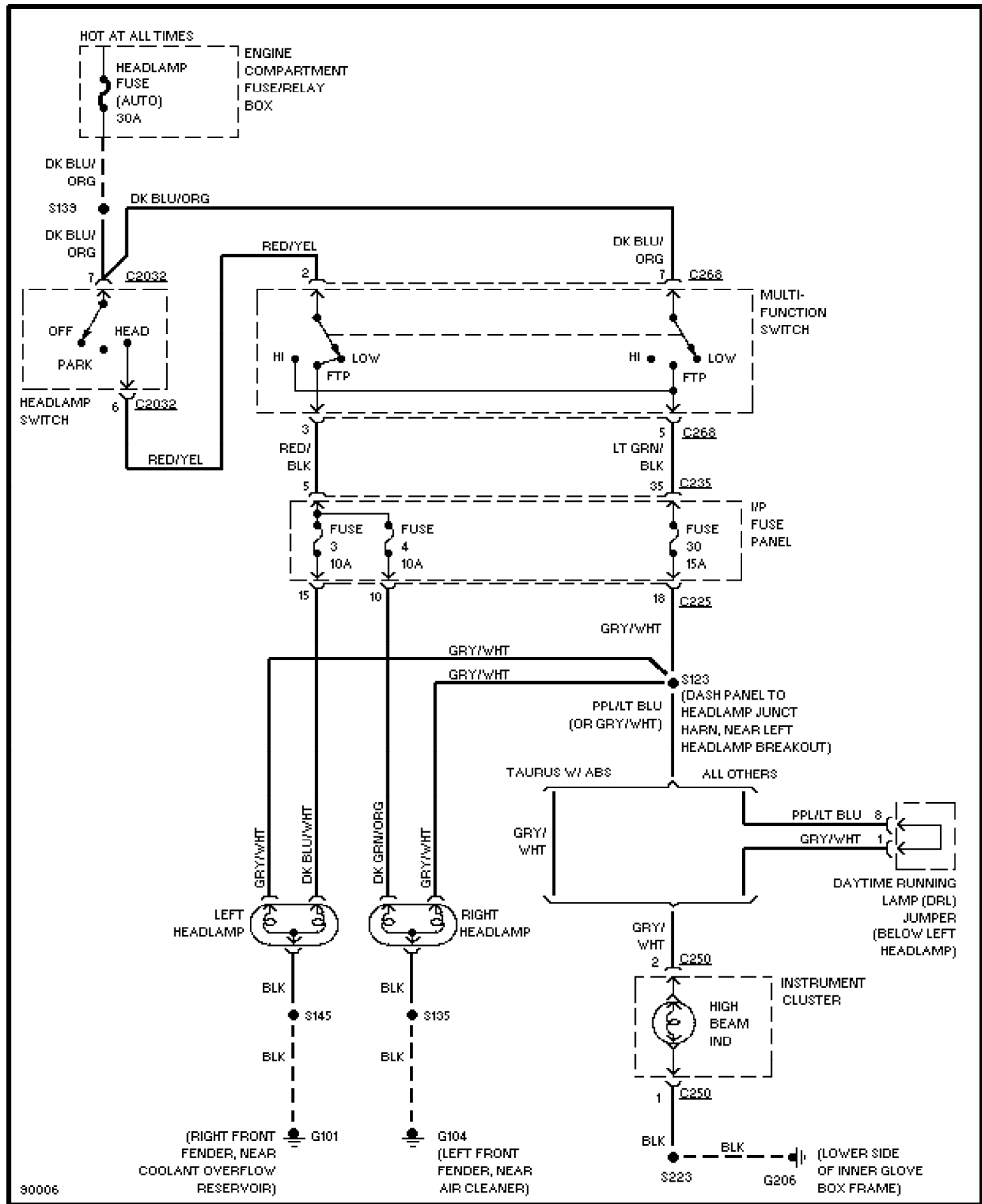
Fig. 41: Headlamps Circuit, W/O DRL 1997 Ford Taurus LX
