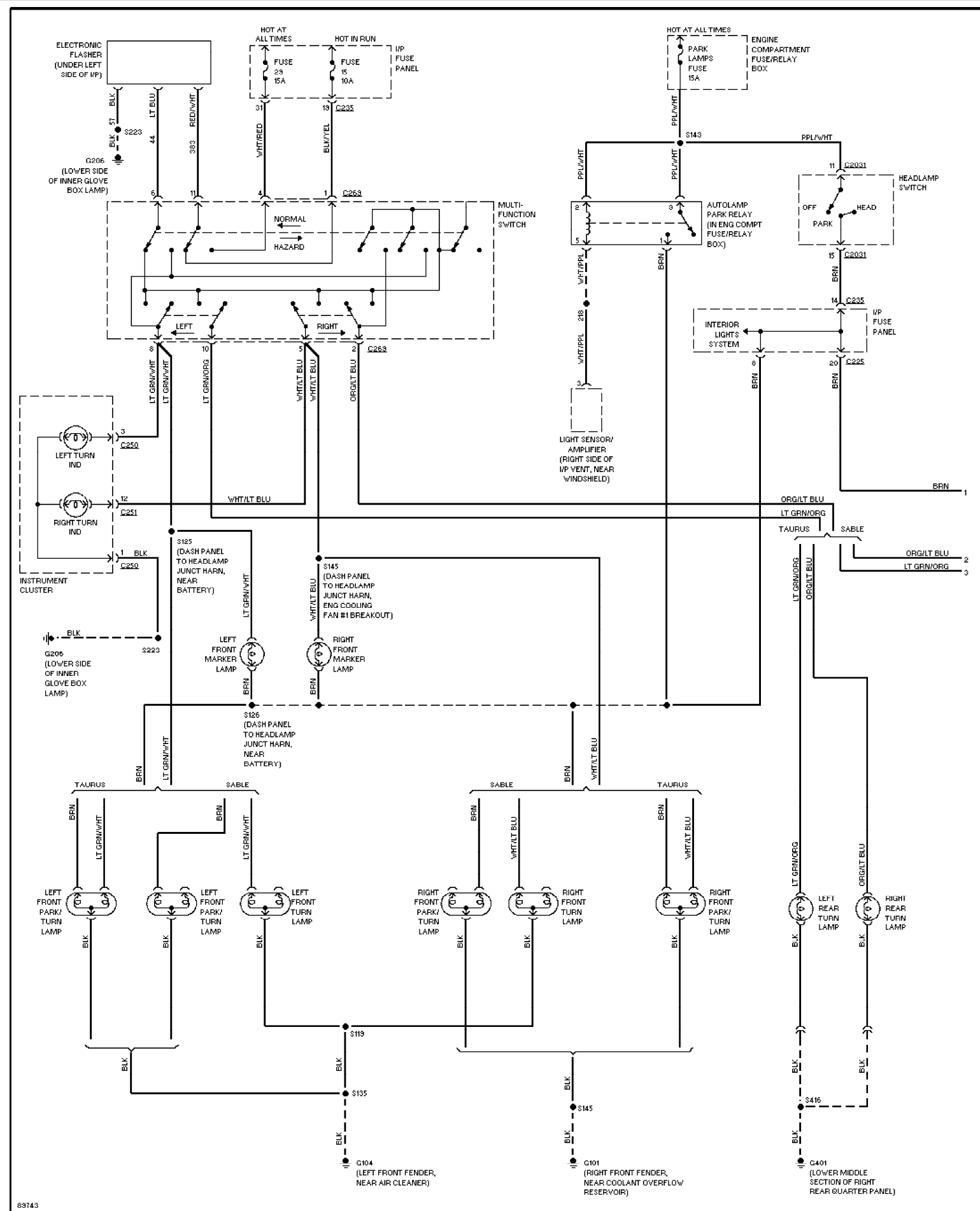
Fig. 28: Exterior Lamps Circuit, Sedan W/O Lamp Out Warning (1 of 2)
