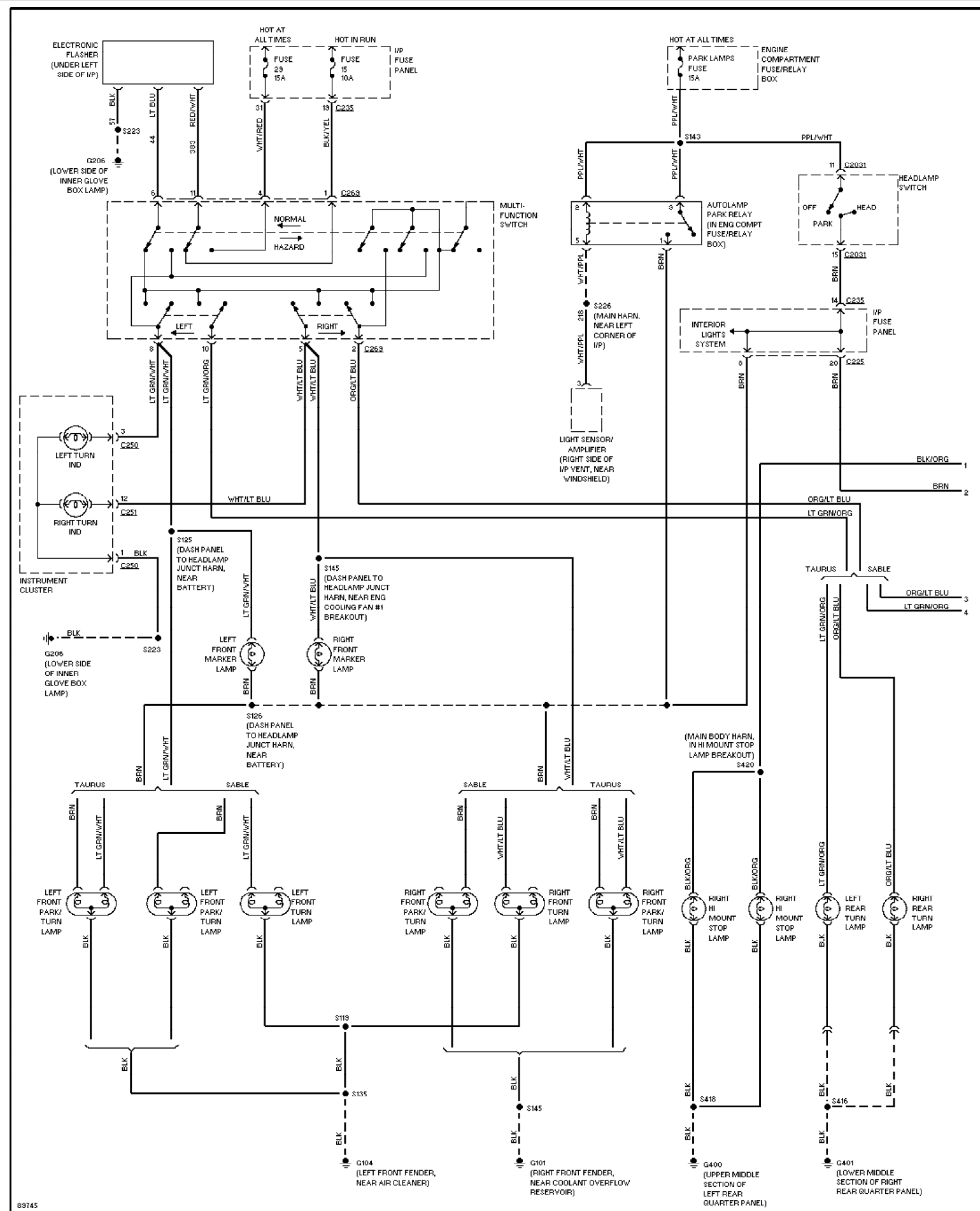
Fig. 26: Exterior Lamps Circuit, Sedan W/ Lamp Out Warning (1 of 2)
