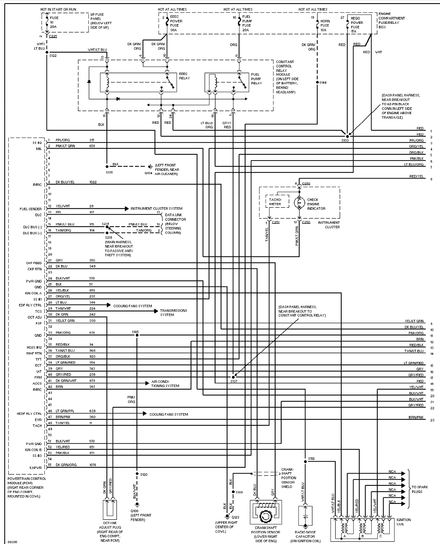
Fig. 15: 3.0L 24-Valve, Engine Performance Circuits (1 of 3)
