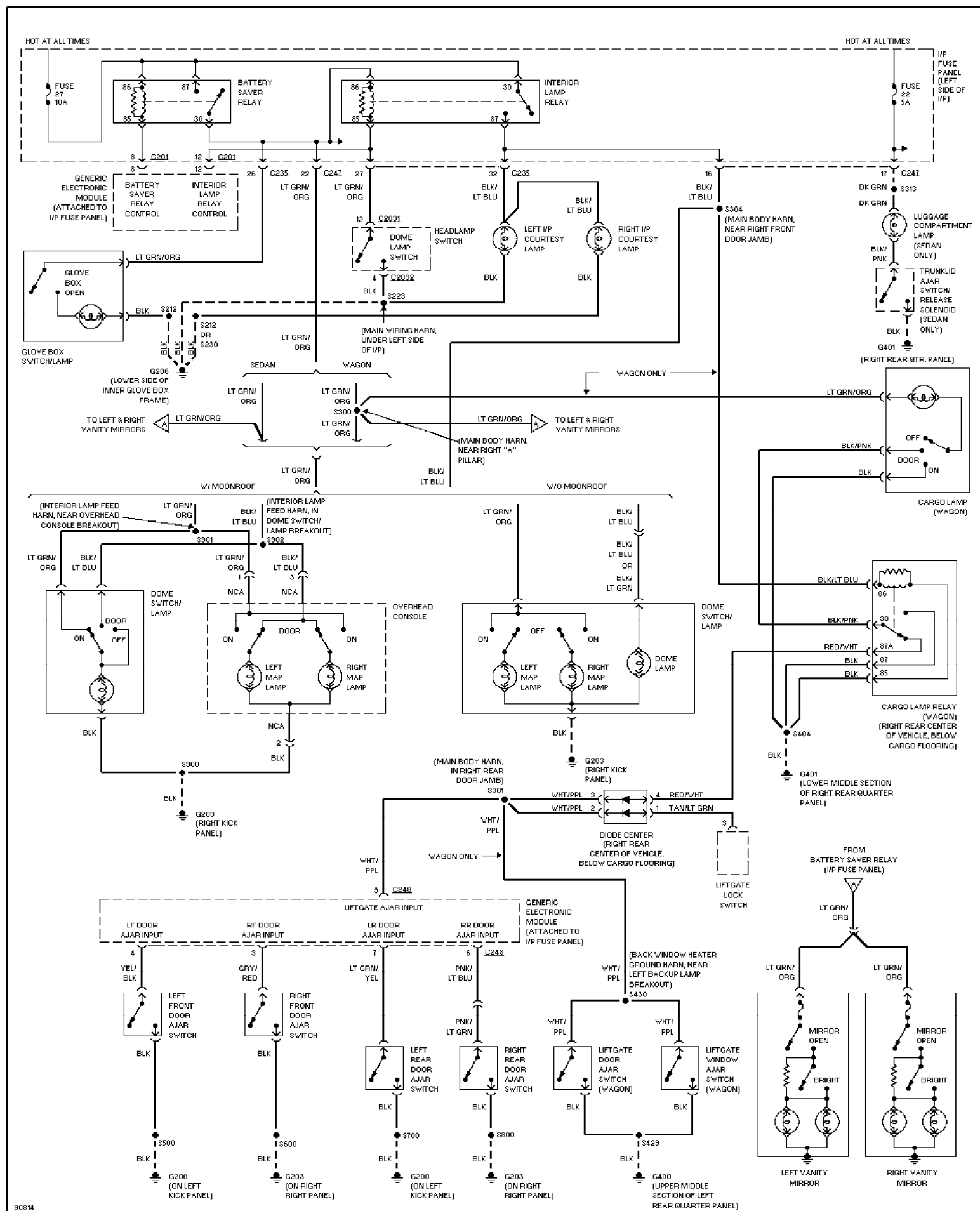
Fig. 48: Courtesy Lamps Circuit 1997 Ford Taurus LX
