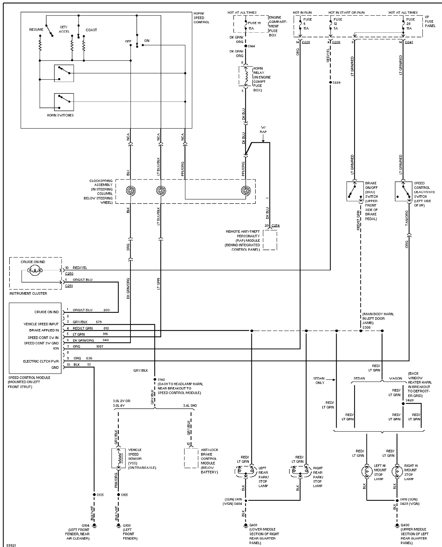
Fig. 8: Cruise Control Circuit 1997 Ford Taurus LX
