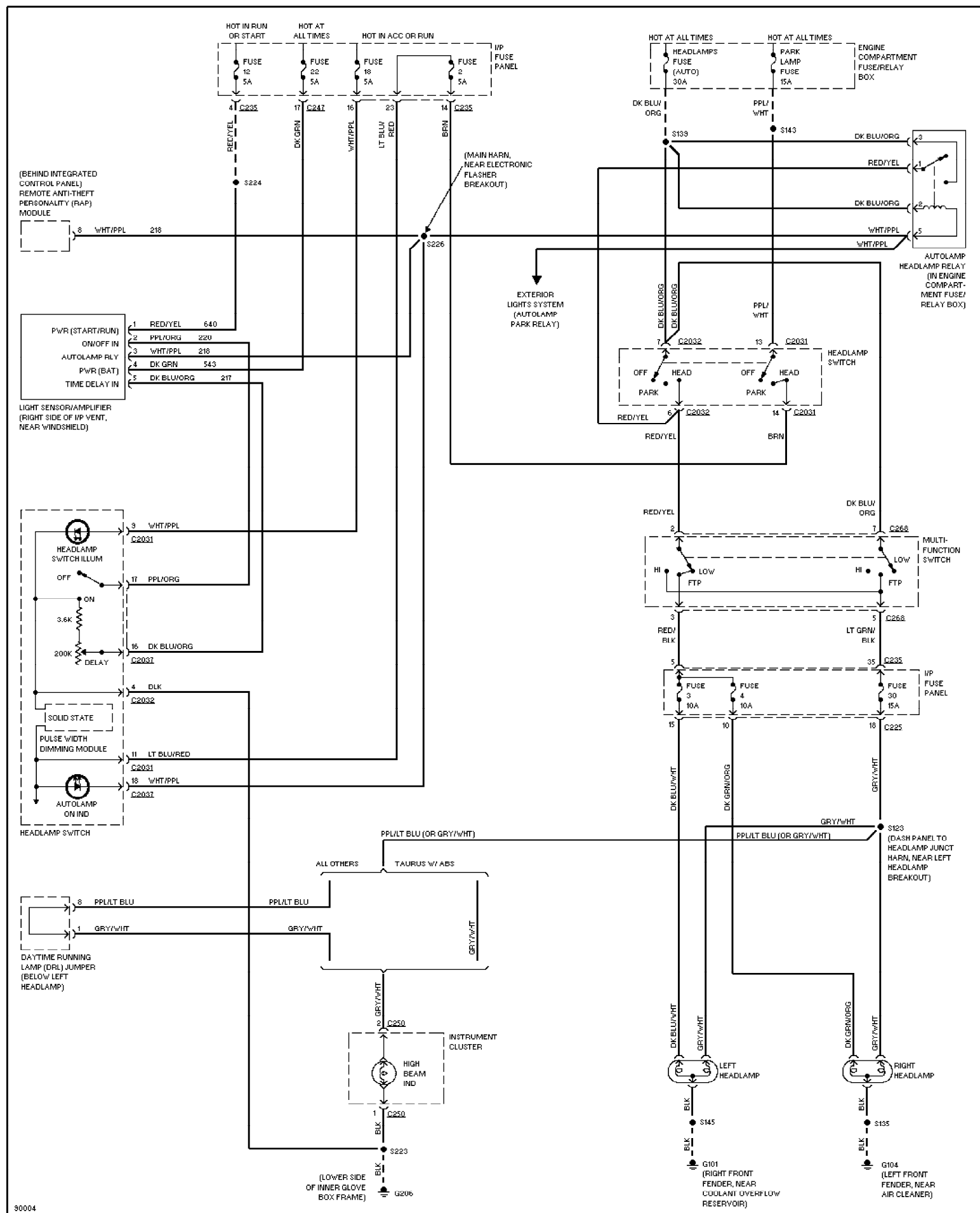
Fig. 39: Autolamps Circuit, W/O DRL 1997 Ford Taurus LX
