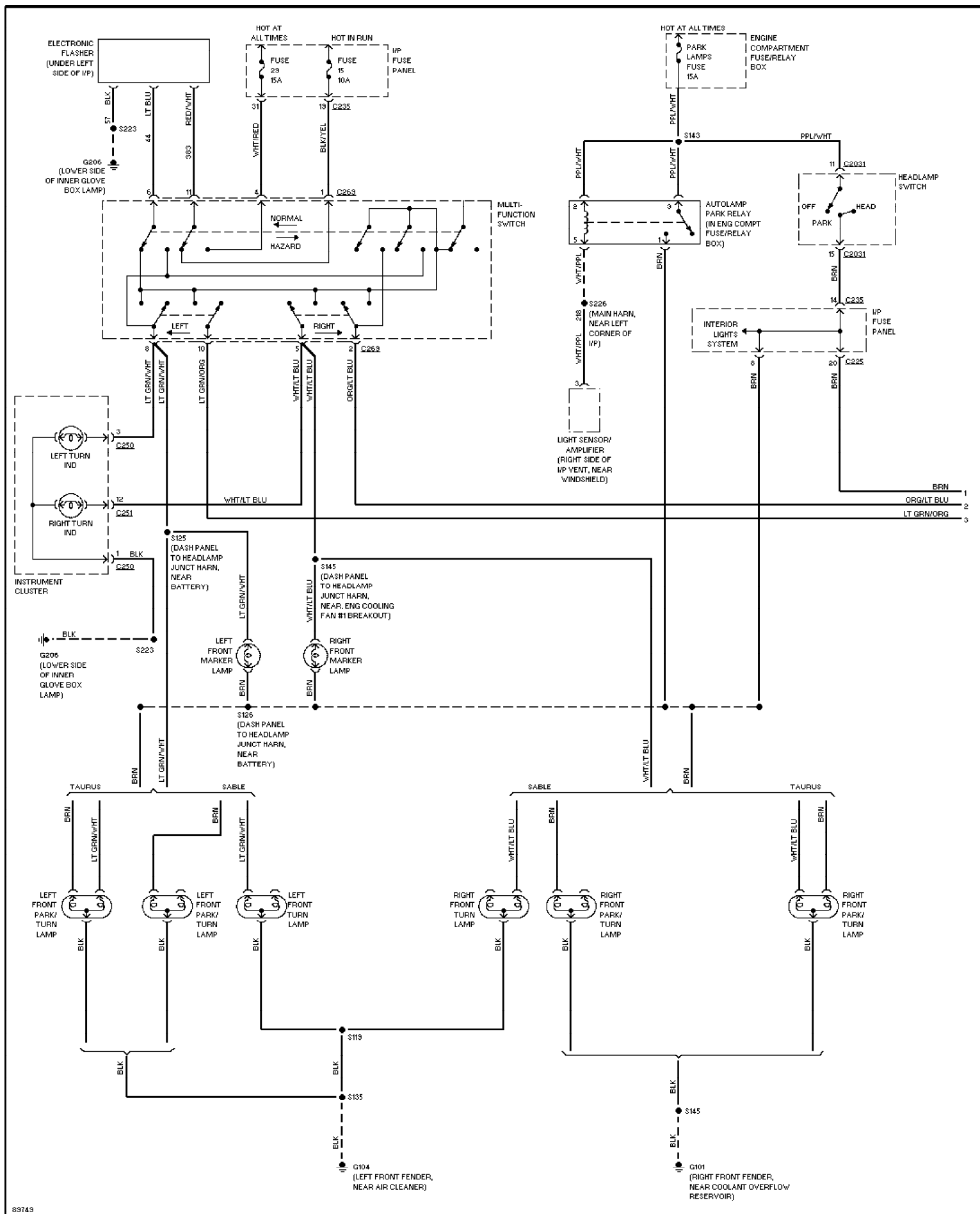
Fig. 30: Exterior Lamps Circuit, Wagon W/ Lamp Out Warning (1 of 2)
