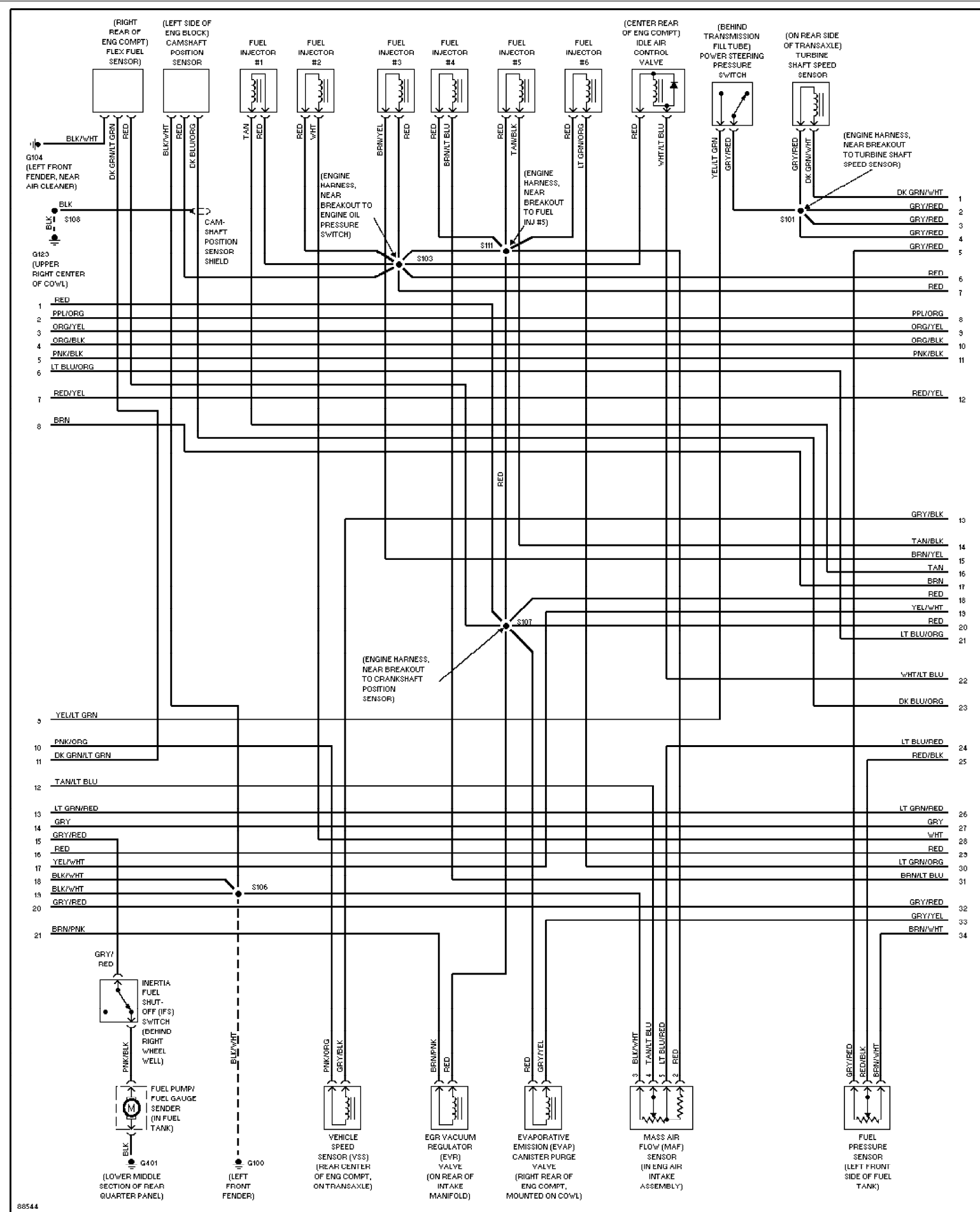
Fig. 19: 3.0L Flex Fuel, Engine Performance Circuits (2 of 3)
