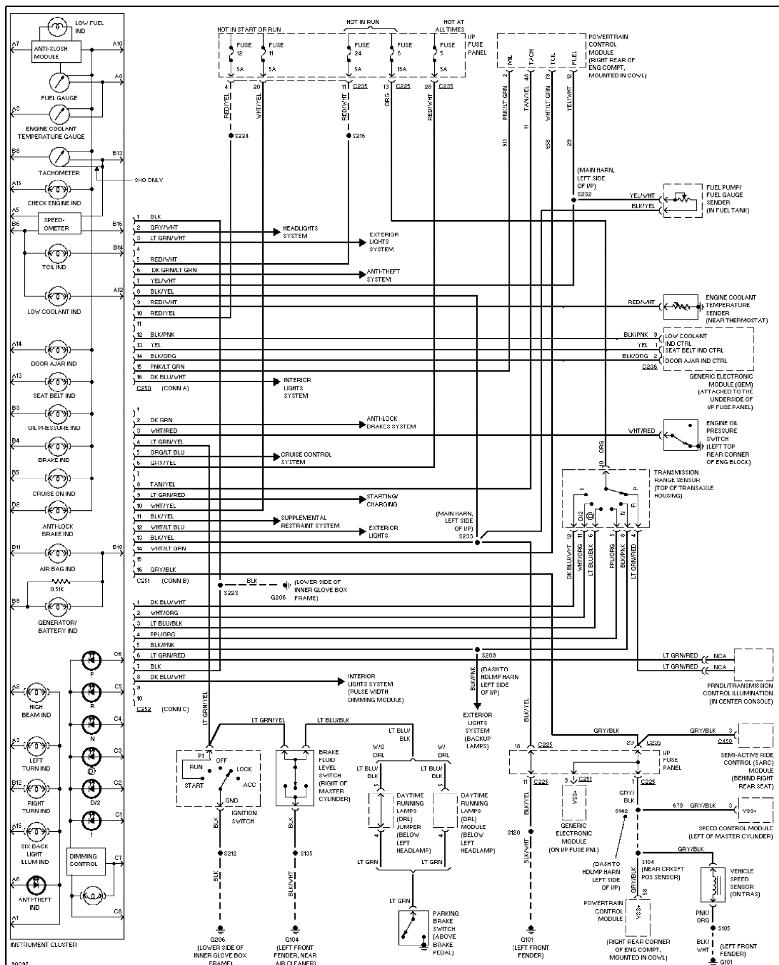
Fig. 46: 3.4L SHO, Instrument Cluster Circuit 1997 Ford Taurus LX
