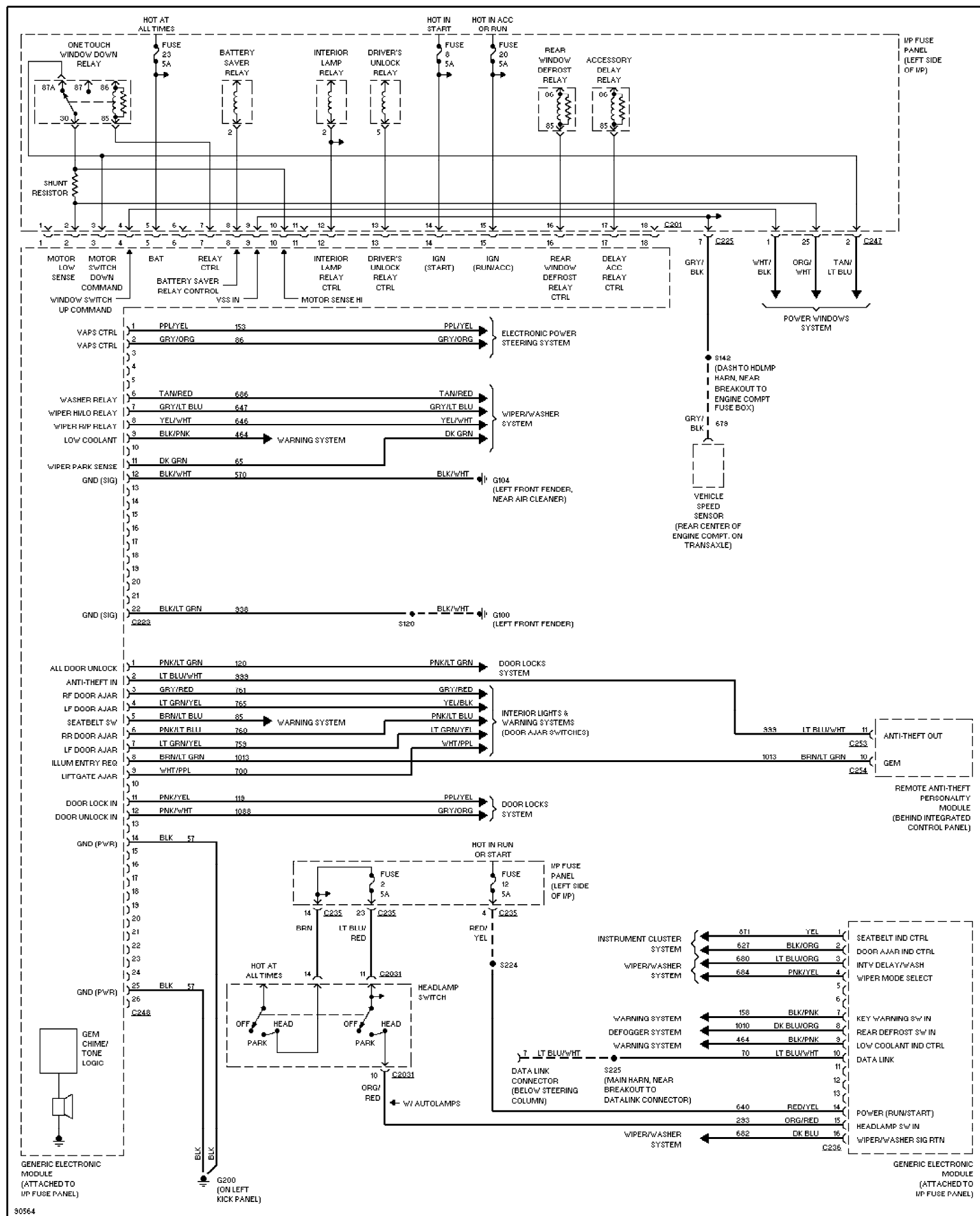
Fig. 5: Body Computer Circuits 1997 Ford Taurus LX
