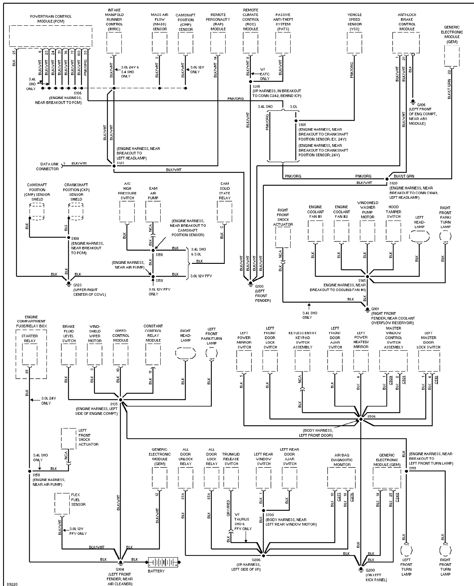
Fig. 35: Ground Distribution Circuit (1 of 3) 1997 Ford Taurus LX
