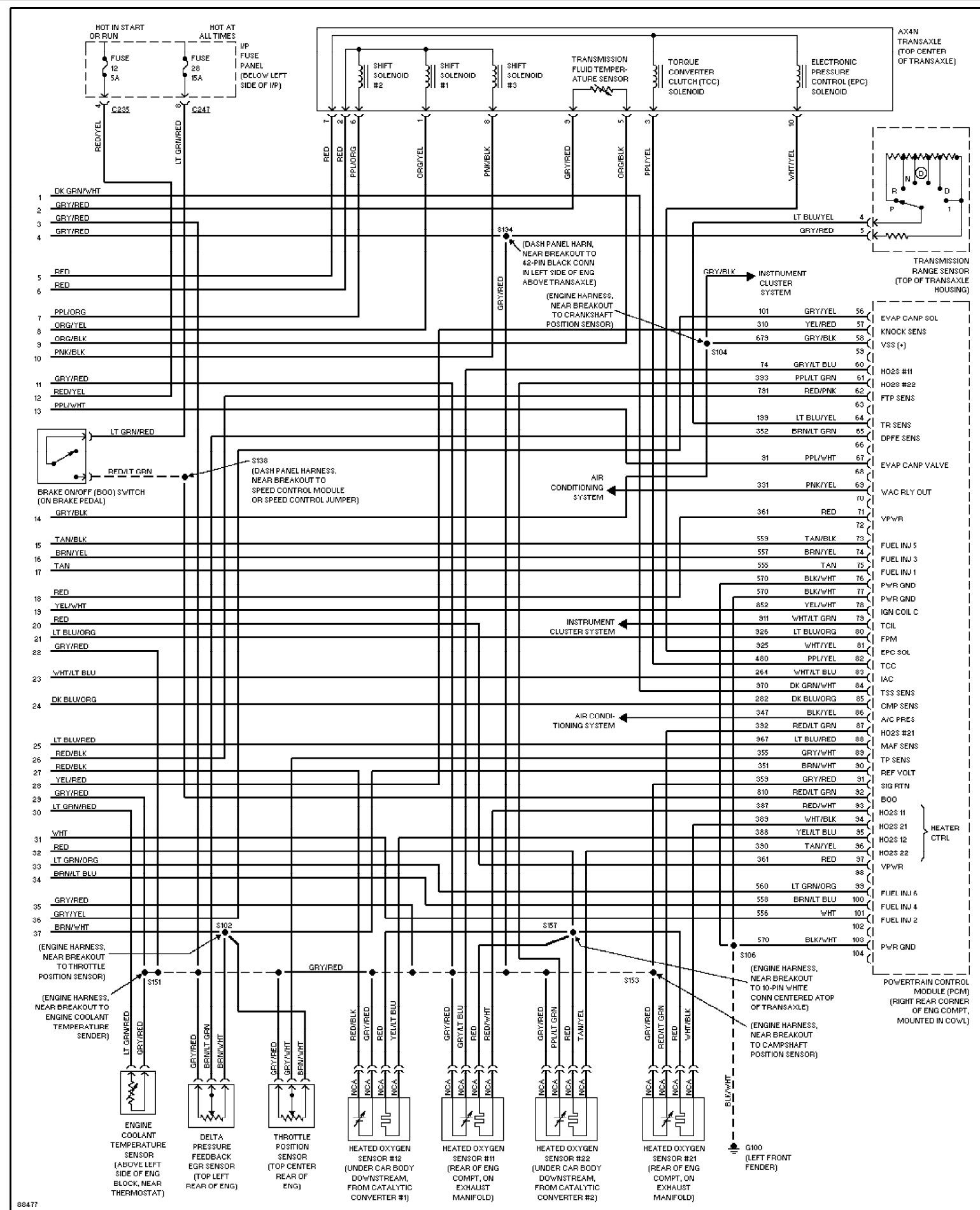
Fig. 17: 3.0L 24-Valve, Engine Performance Circuits (3 of 3)
