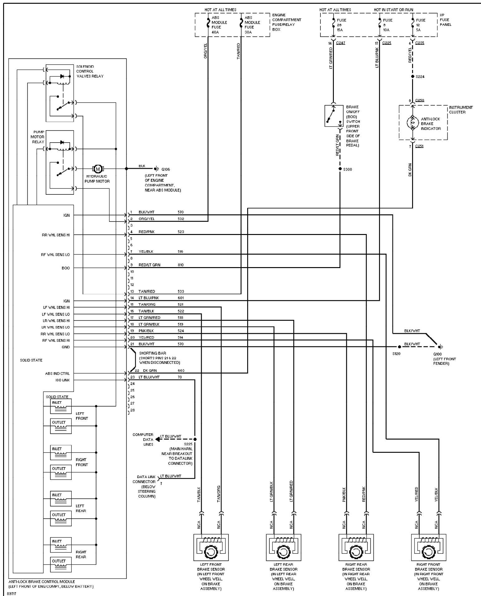
Fig. 3: Anti-lock Brake Circuits 1997 Ford Taurus LX
