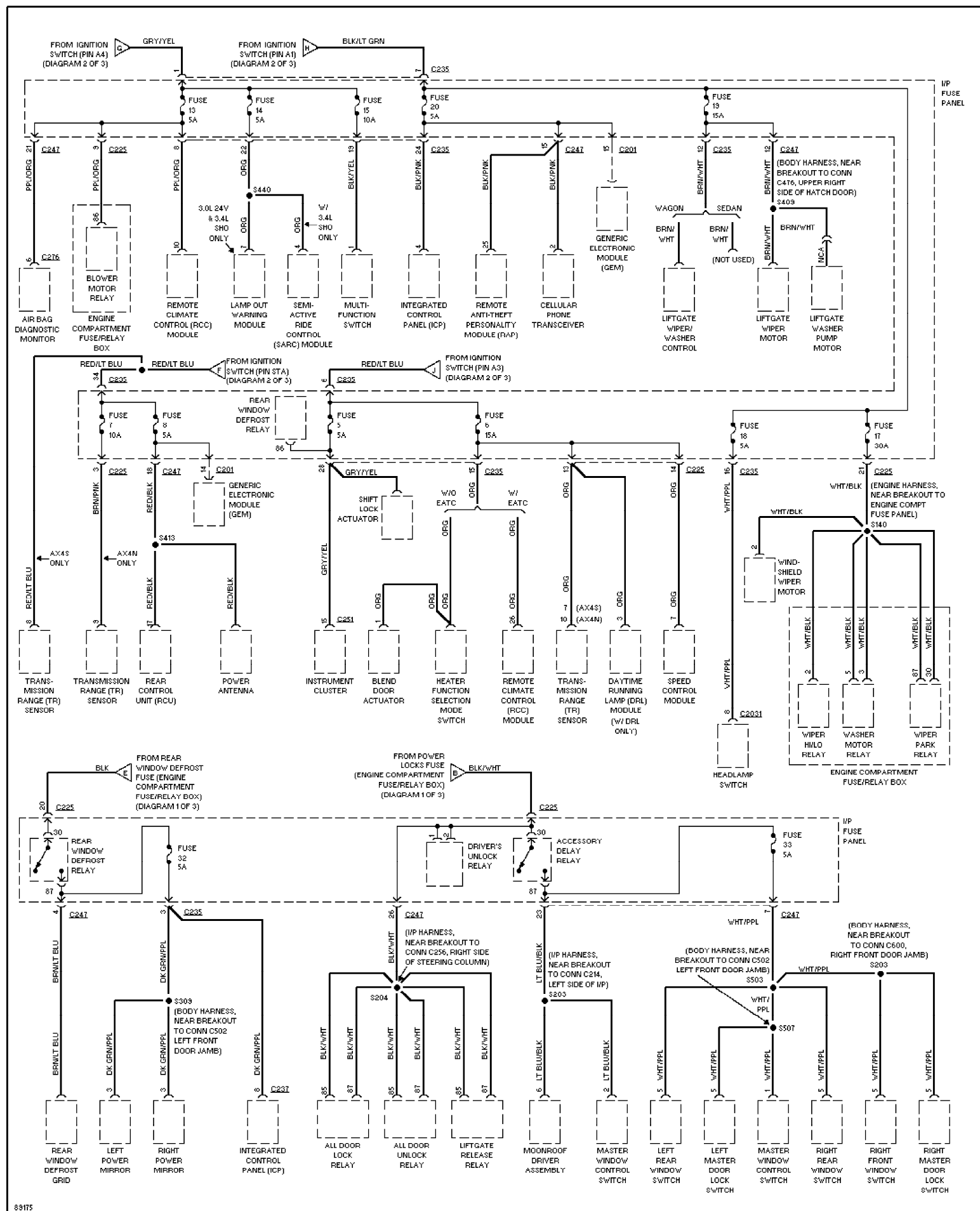
Fig. 53: Power Distribution Circuit (3 of 3) 1997 Ford Taurus LX
