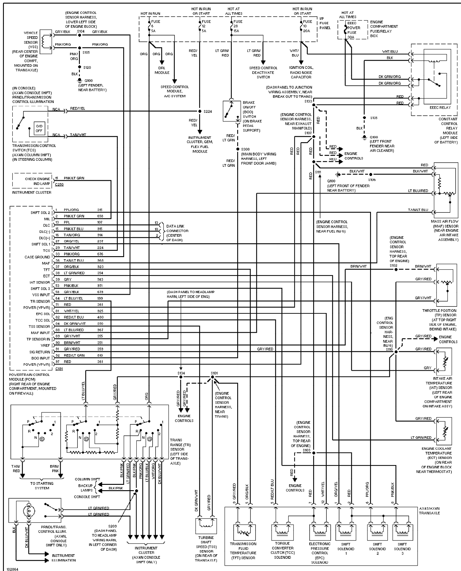
Fig. 69: 3.0L 12-Valve, Transmission Circuit 1997 Ford Taurus LX
