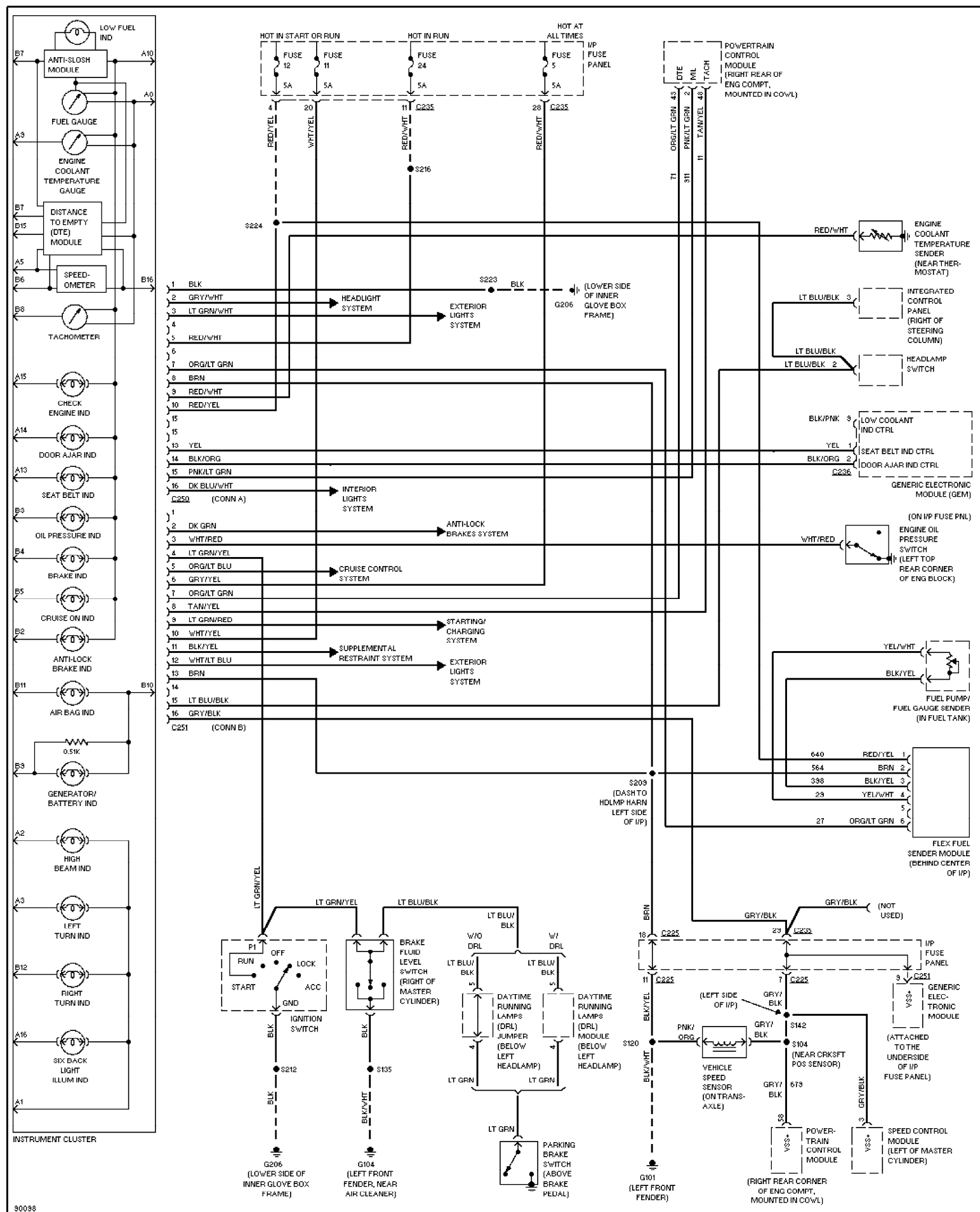
Fig. 43: 3.0L Flex Fuel, Instrument Cluster Circuit 1997 Ford Taurus LX
