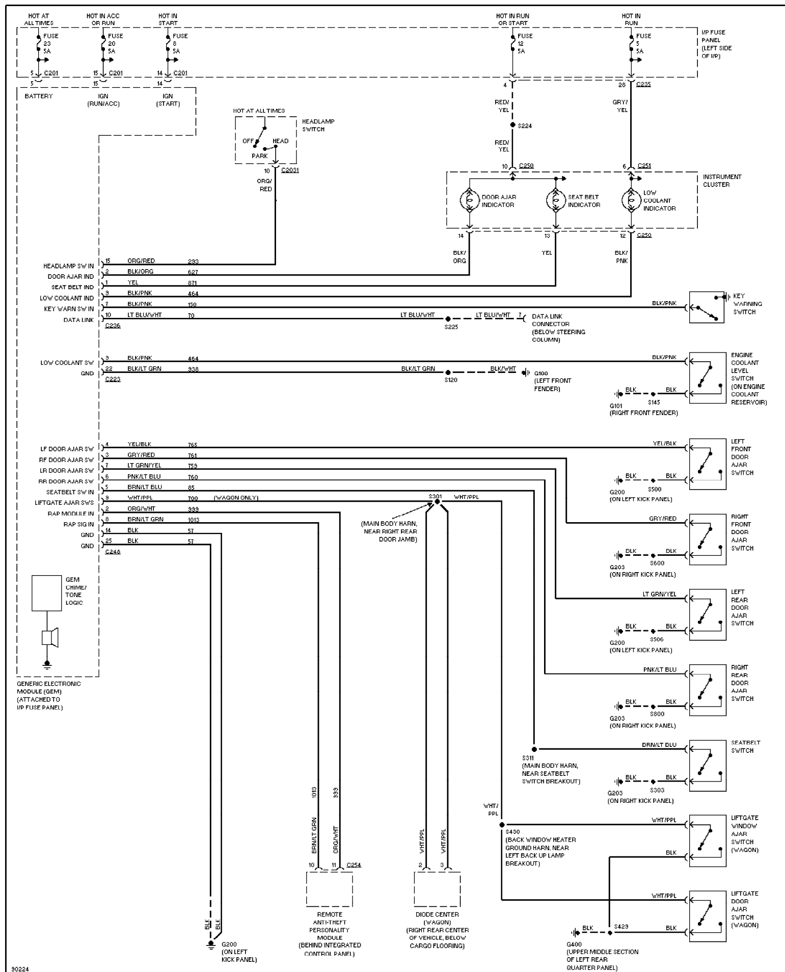
Fig. 74: Warning System Circuits 1997 Ford Taurus LX
