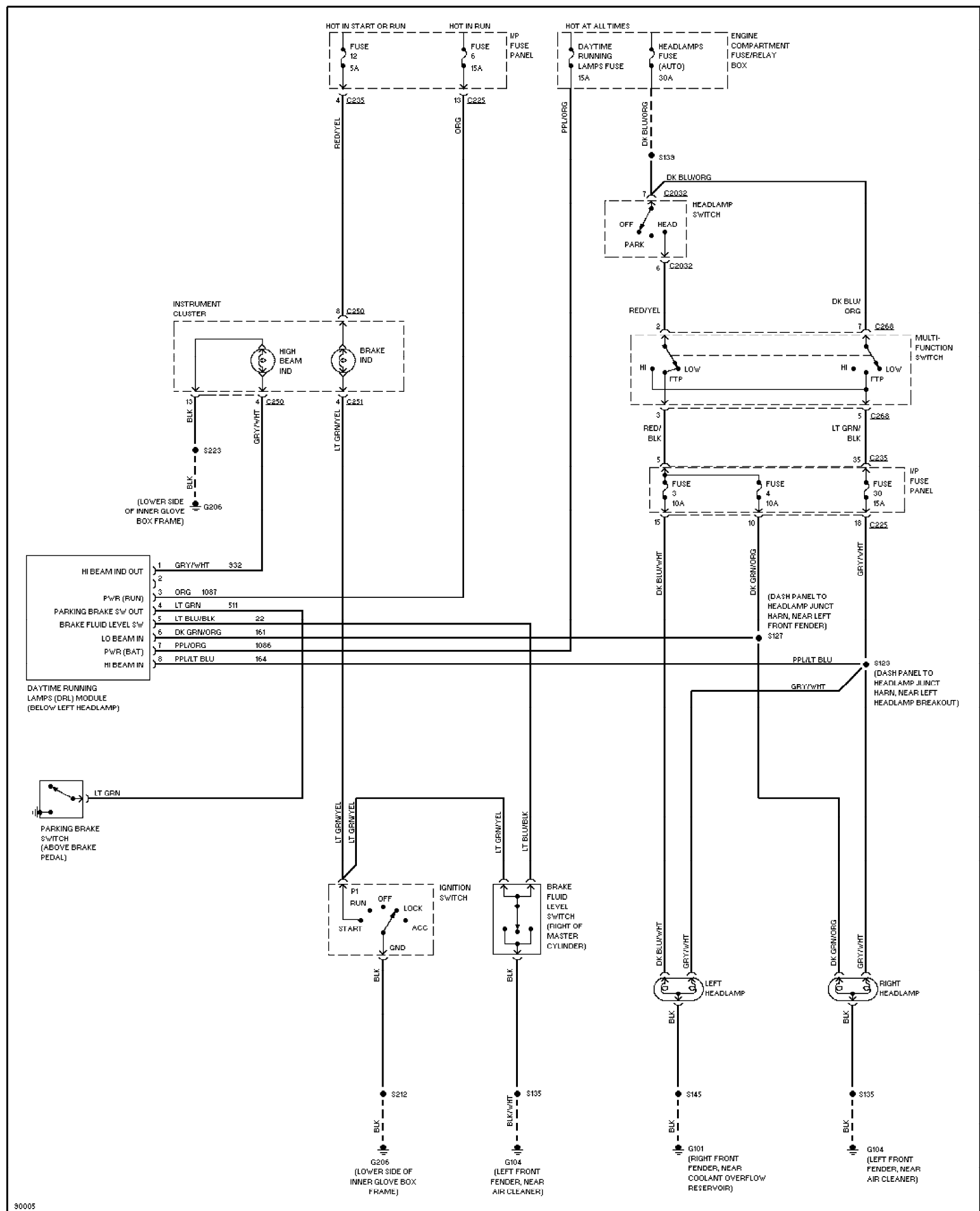
Fig. 40: Headlamps Circuit, W/ DRL 1997 Ford Taurus LX
