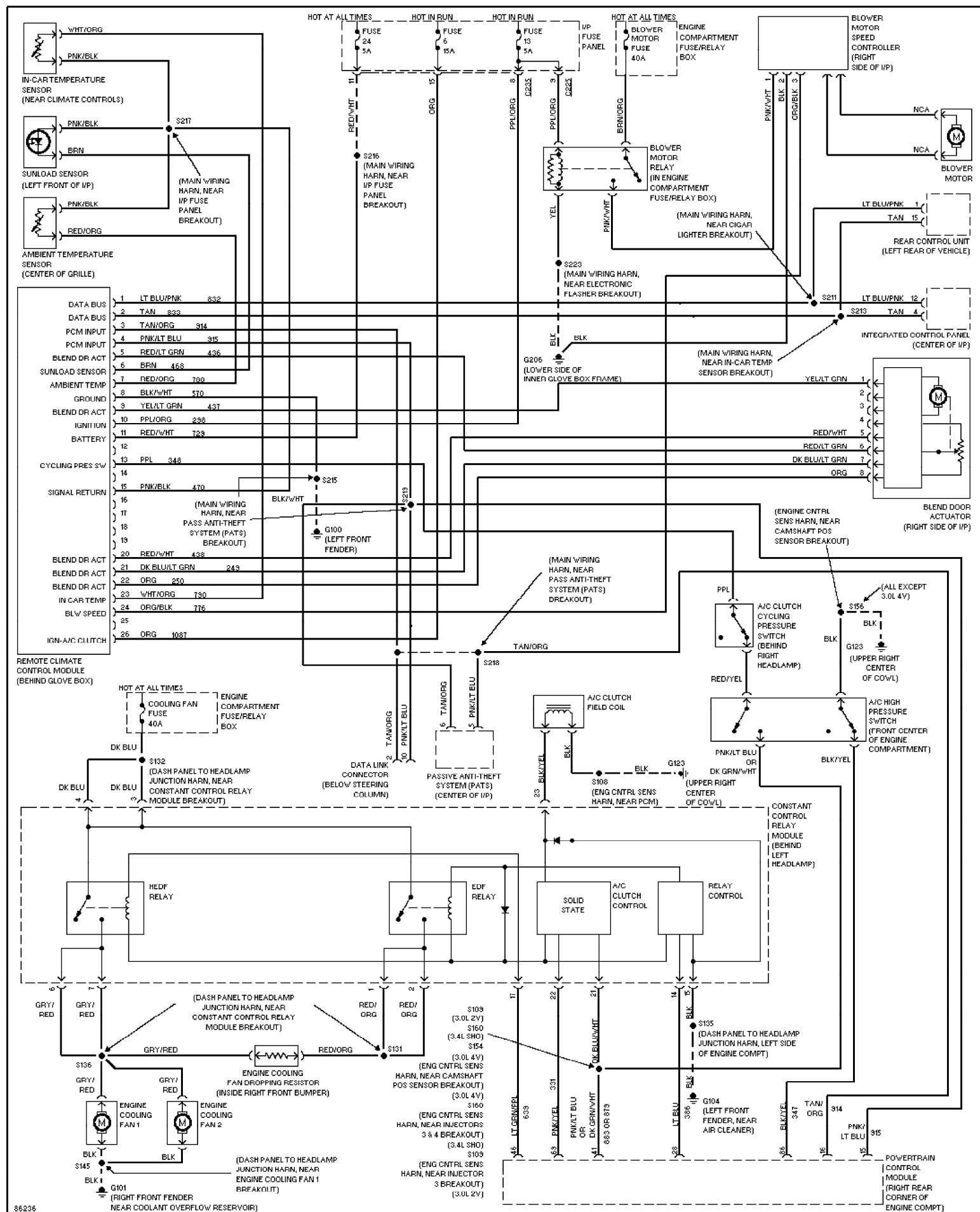
Fig. 1: A/C Circuit, Auto A/C 1997 Ford Taurus LX
