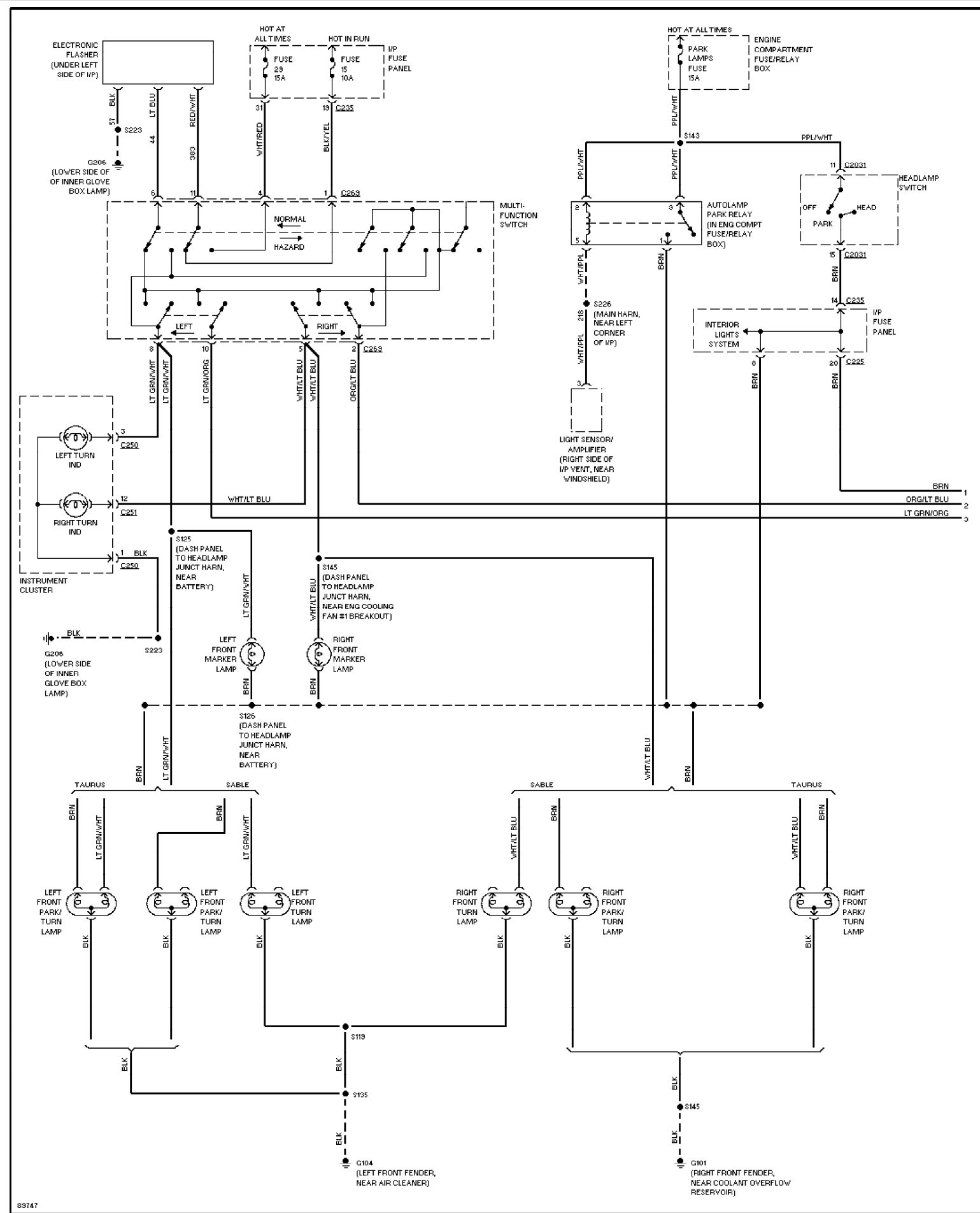
Fig. 32: Exterior Lamps Circuit, Wagon W/O Lamp Out Warning (1 of 2)
