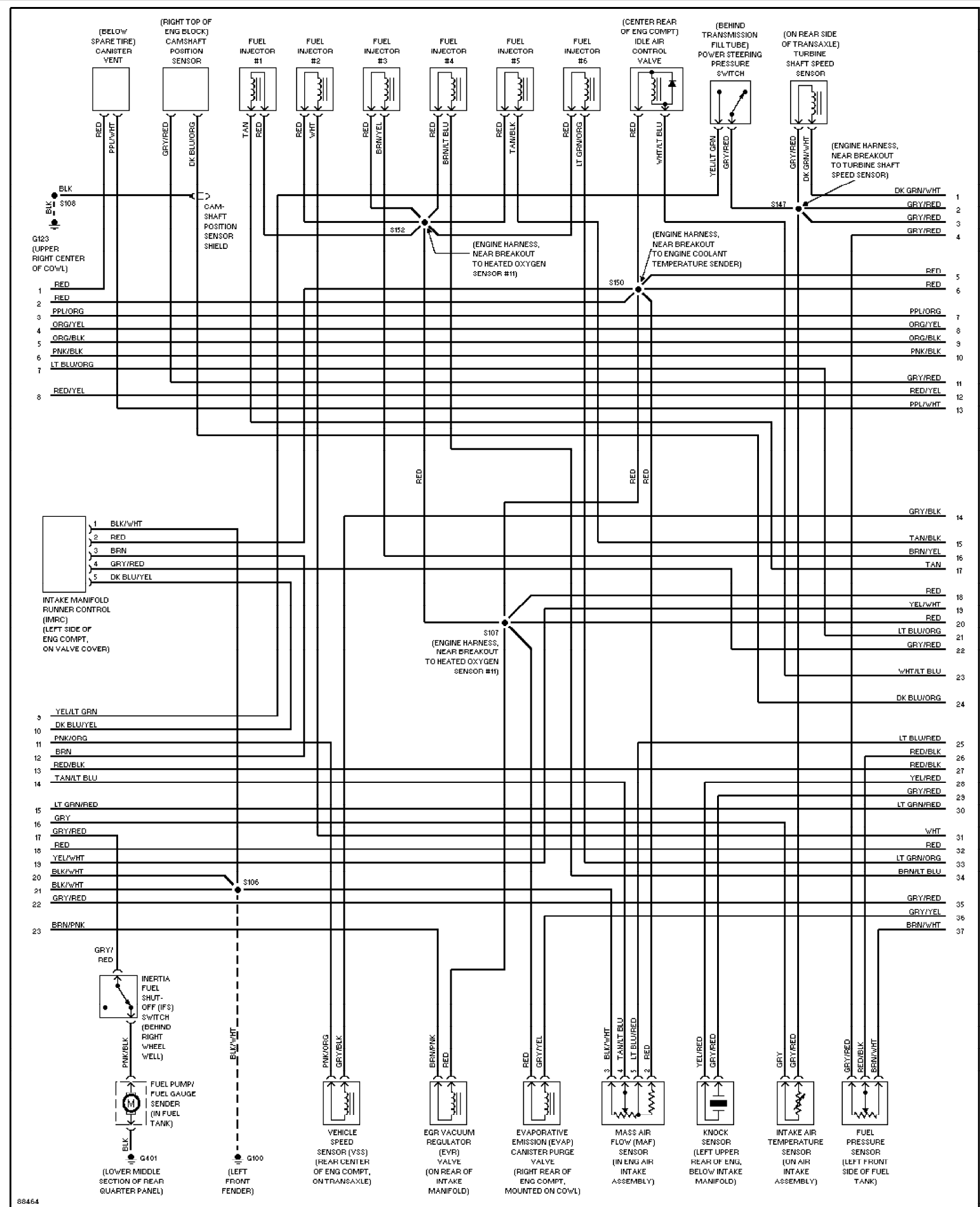
Fig. 16: 3.0L 24-Valve, Engine Performance Circuits (2 of 3)
