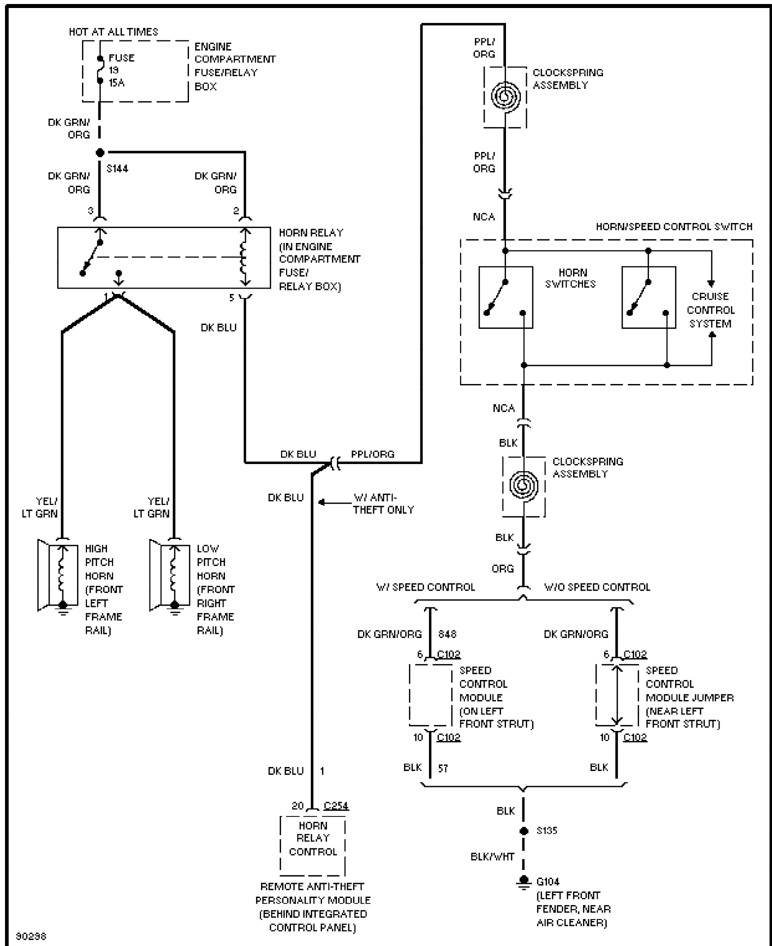
Fig. 42: Horn Circuit 1997 Ford Taurus LX
