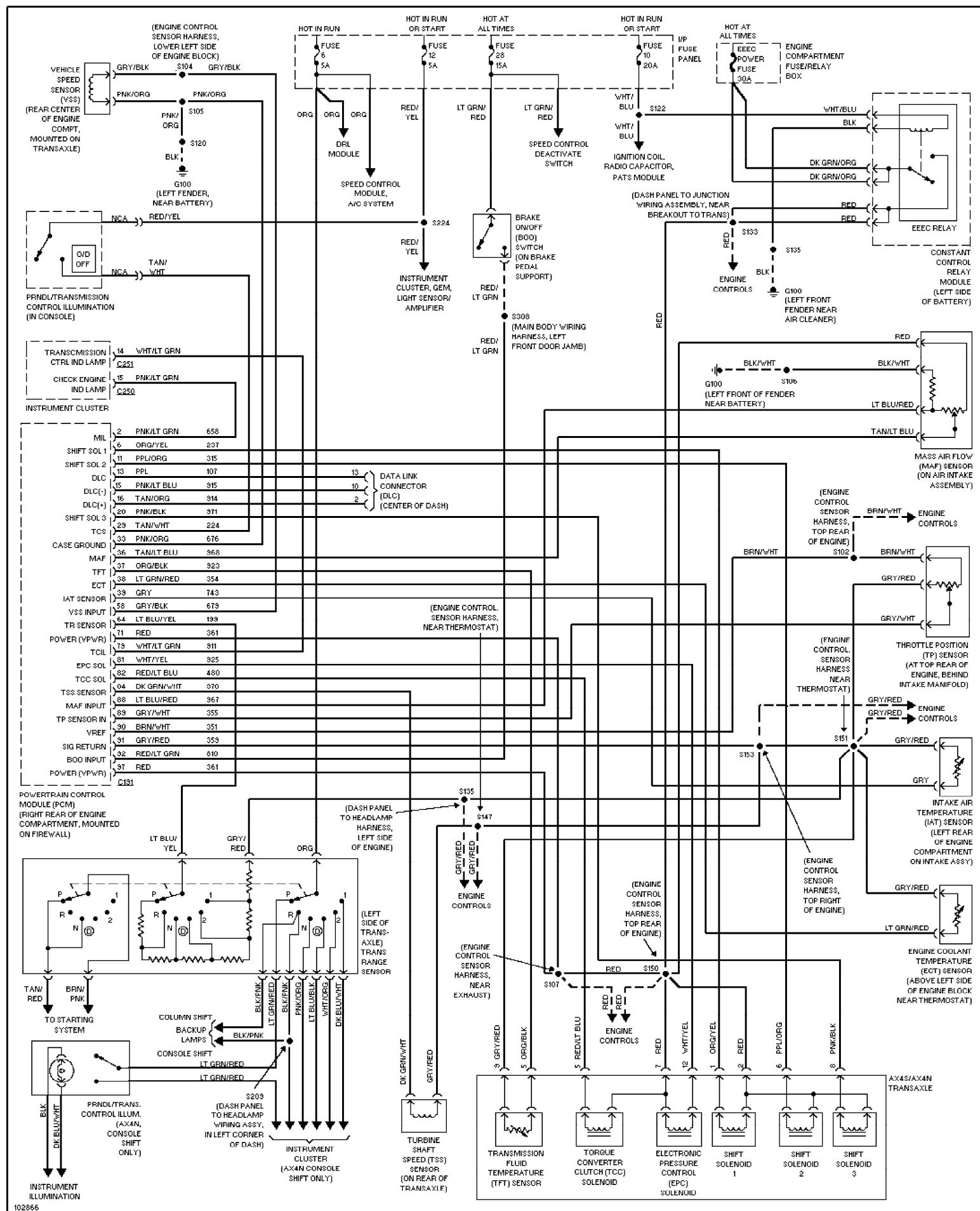
Fig. 72: 3.4L SHO, Transmission Circuit 1997 Ford Taurus LX
