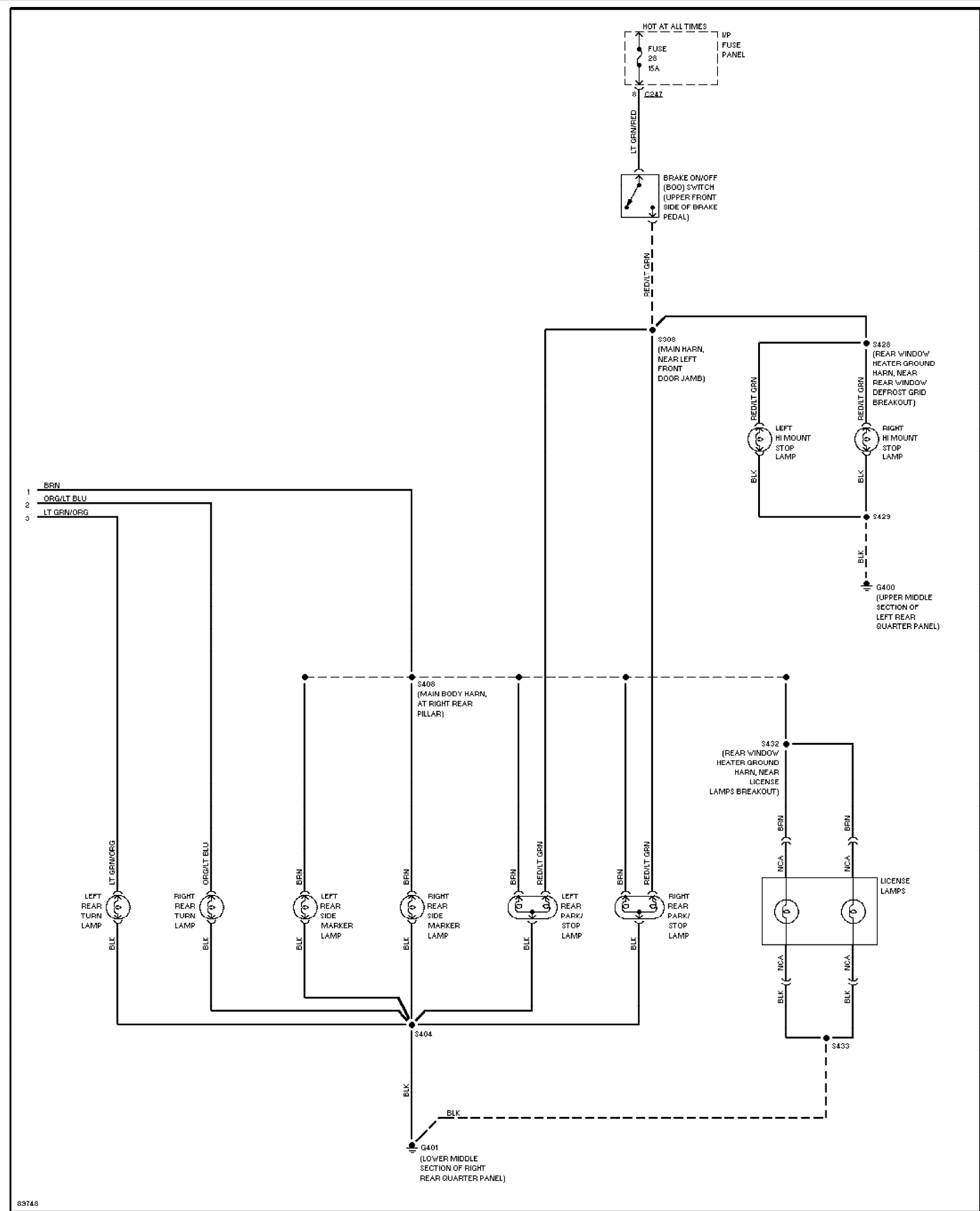
Fig. 33: Exterior Lamps Circuit, Wagon W/O Lamp Out Warning (2 of 2)
