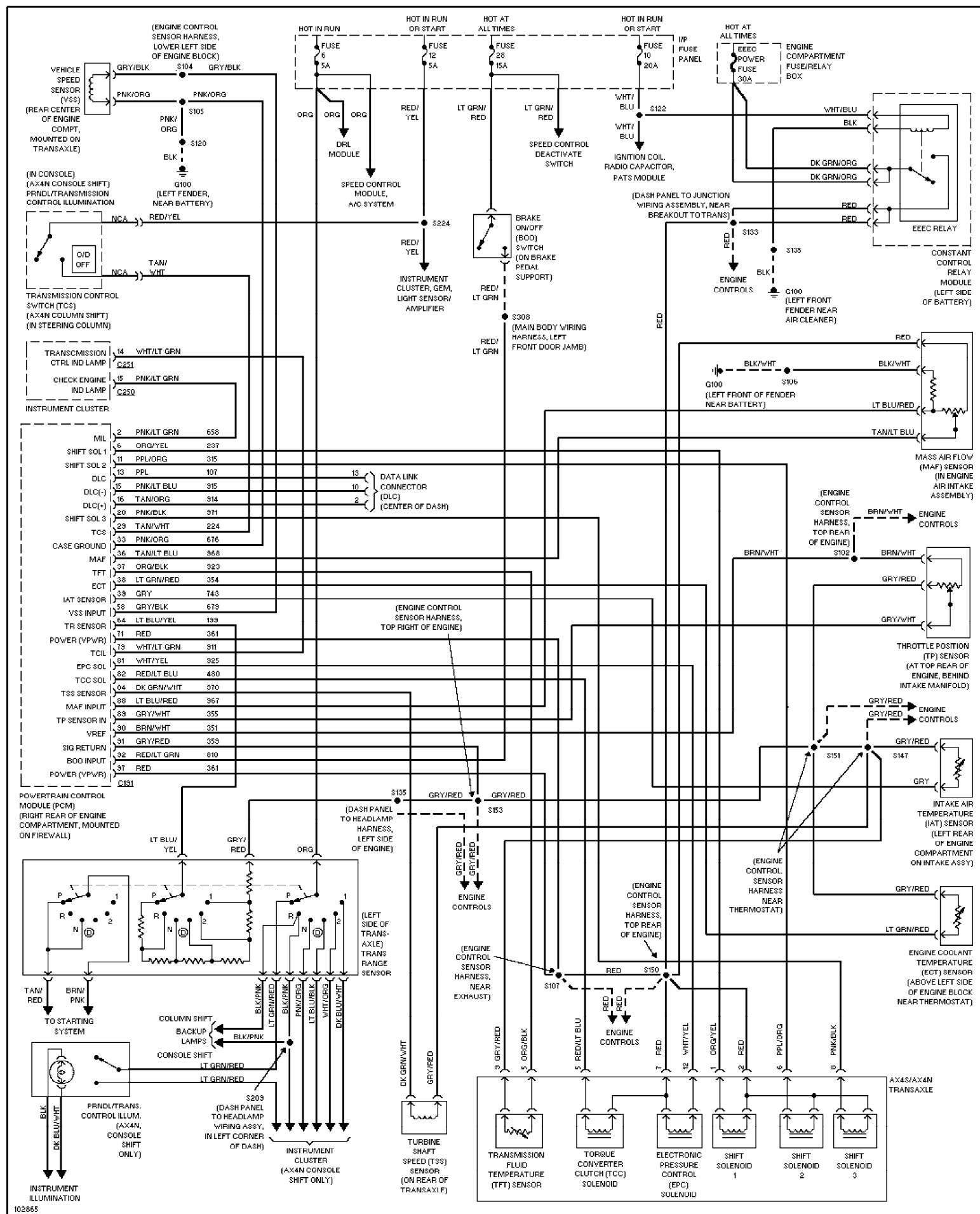
Fig. 70: 3.0L 24-Valve, Transmission Circuit 1997 Ford Taurus LX
