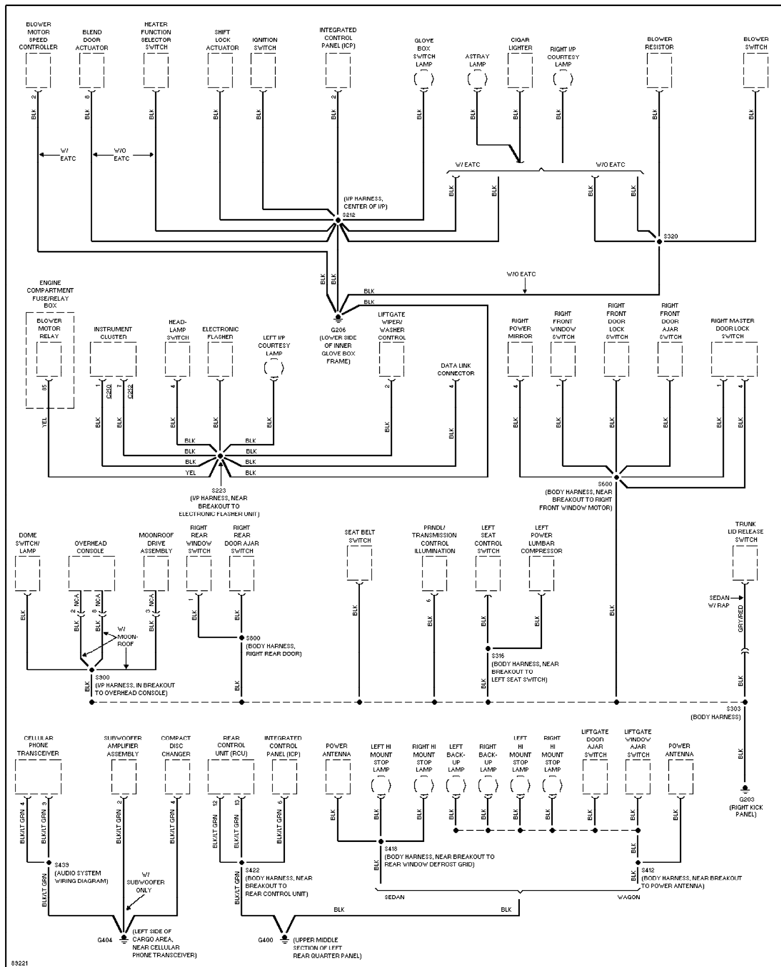
Fig. 36: Ground Distribution Circuit (2 of 3) 1997 Ford Taurus LX
