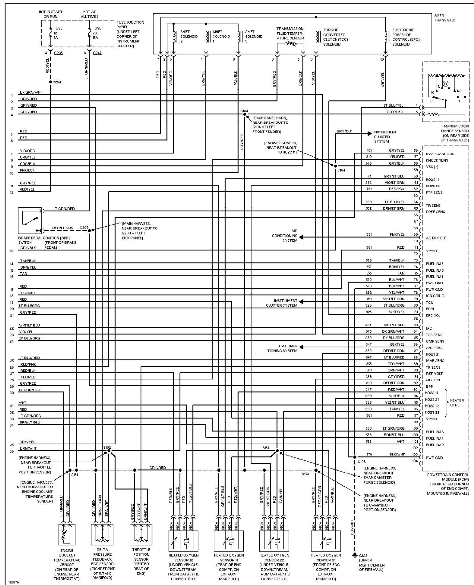
Fig. 19: 3.0L 24-Valve, Engine Performance Circuits (3 of 3)
