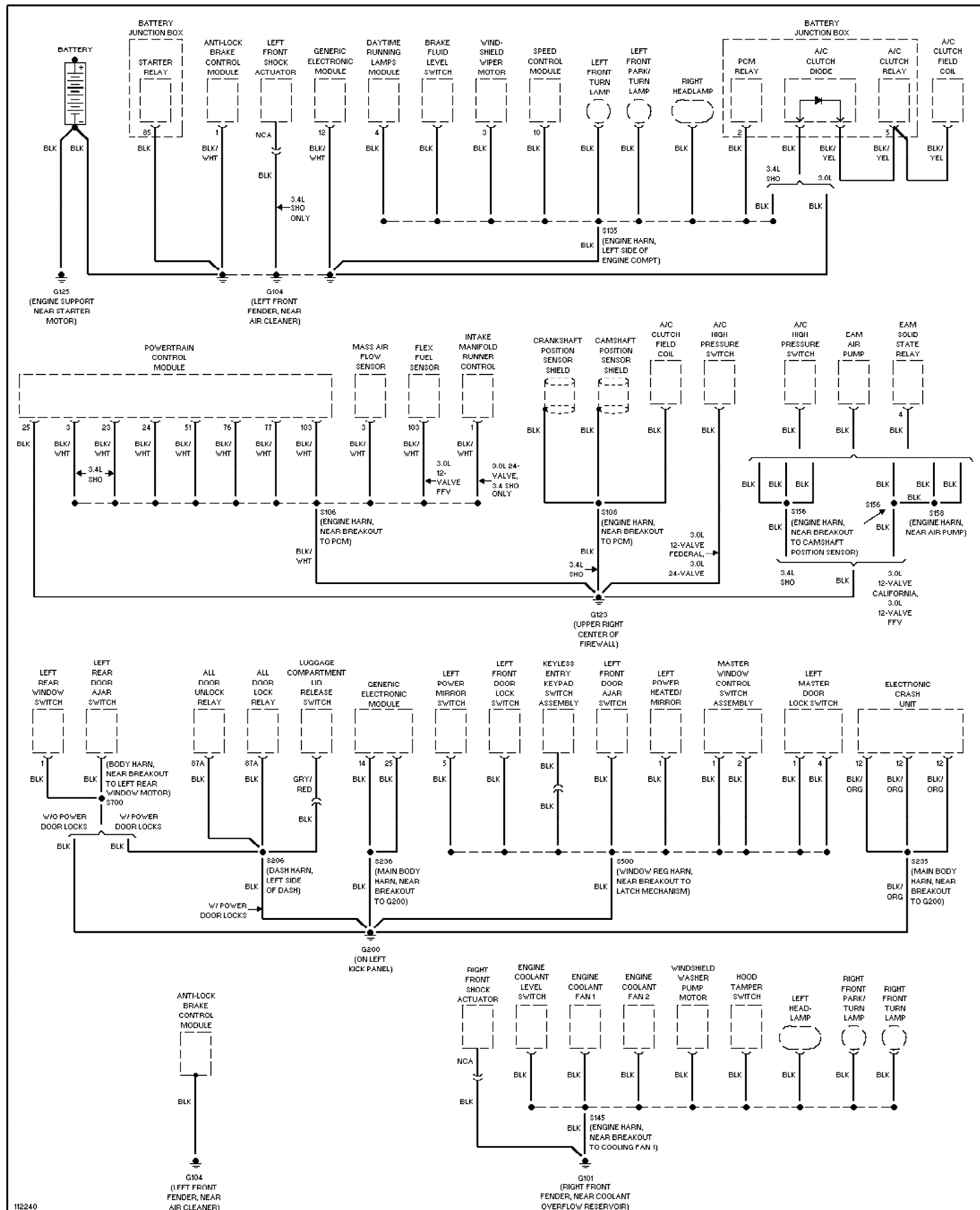
Fig. 31: Ground Distribution Circuit (1 of 3) 1999 Ford Taurus LX
