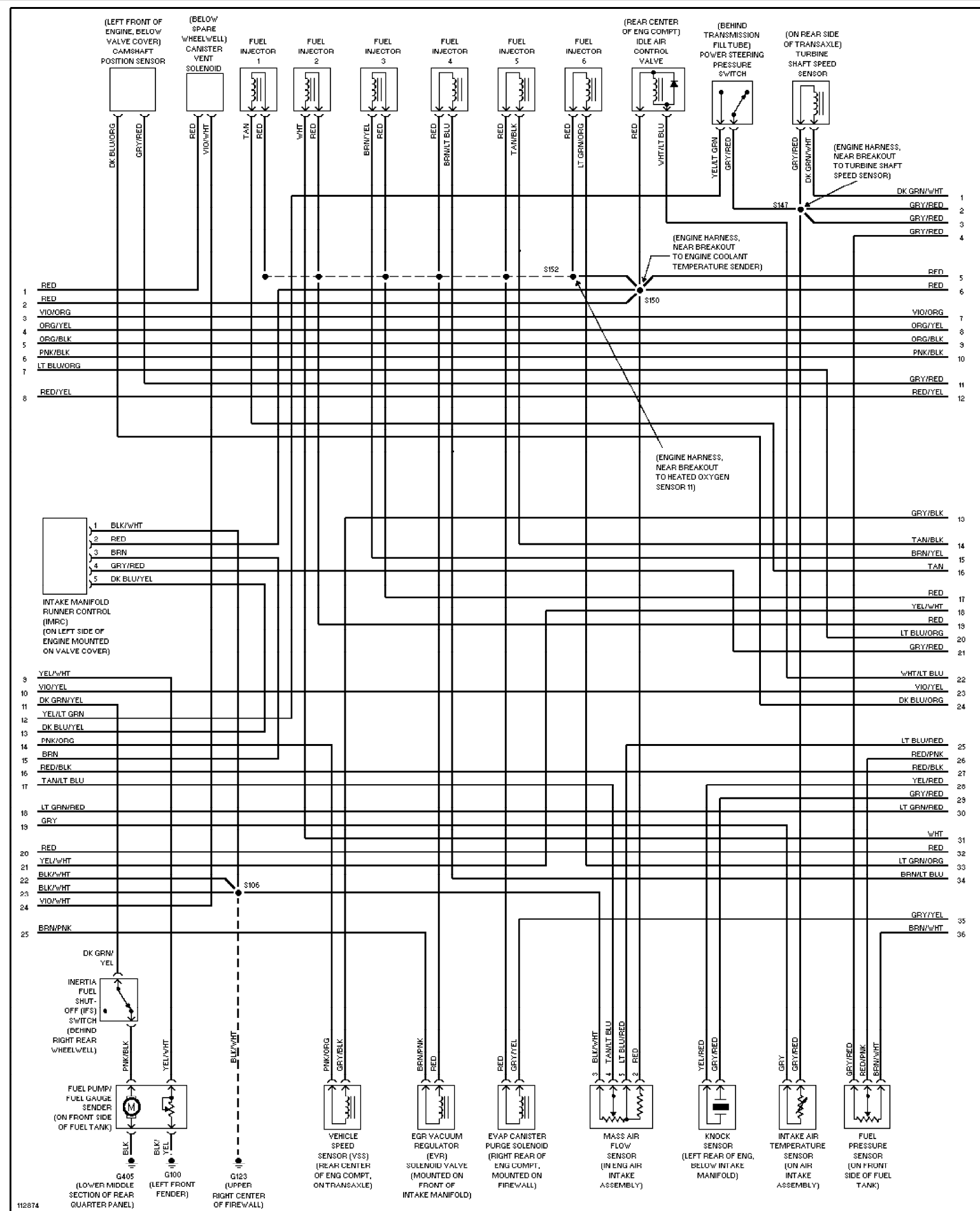
Fig. 18: 3.0L 24-Valve, Engine Performance Circuits (2 of 3)
