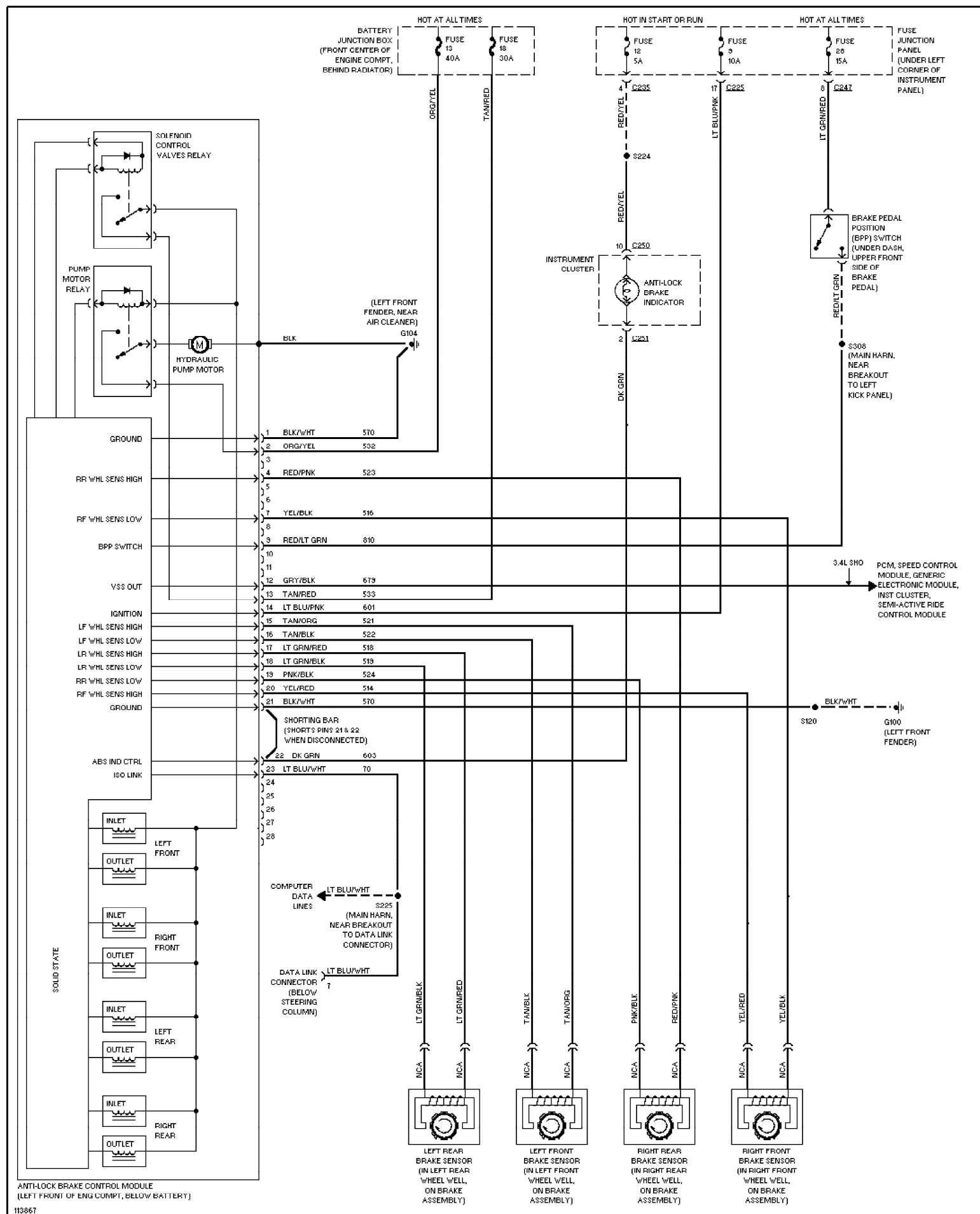
Fig. 4: Anti-lock Brake Circuits 1999 Ford Taurus LX
