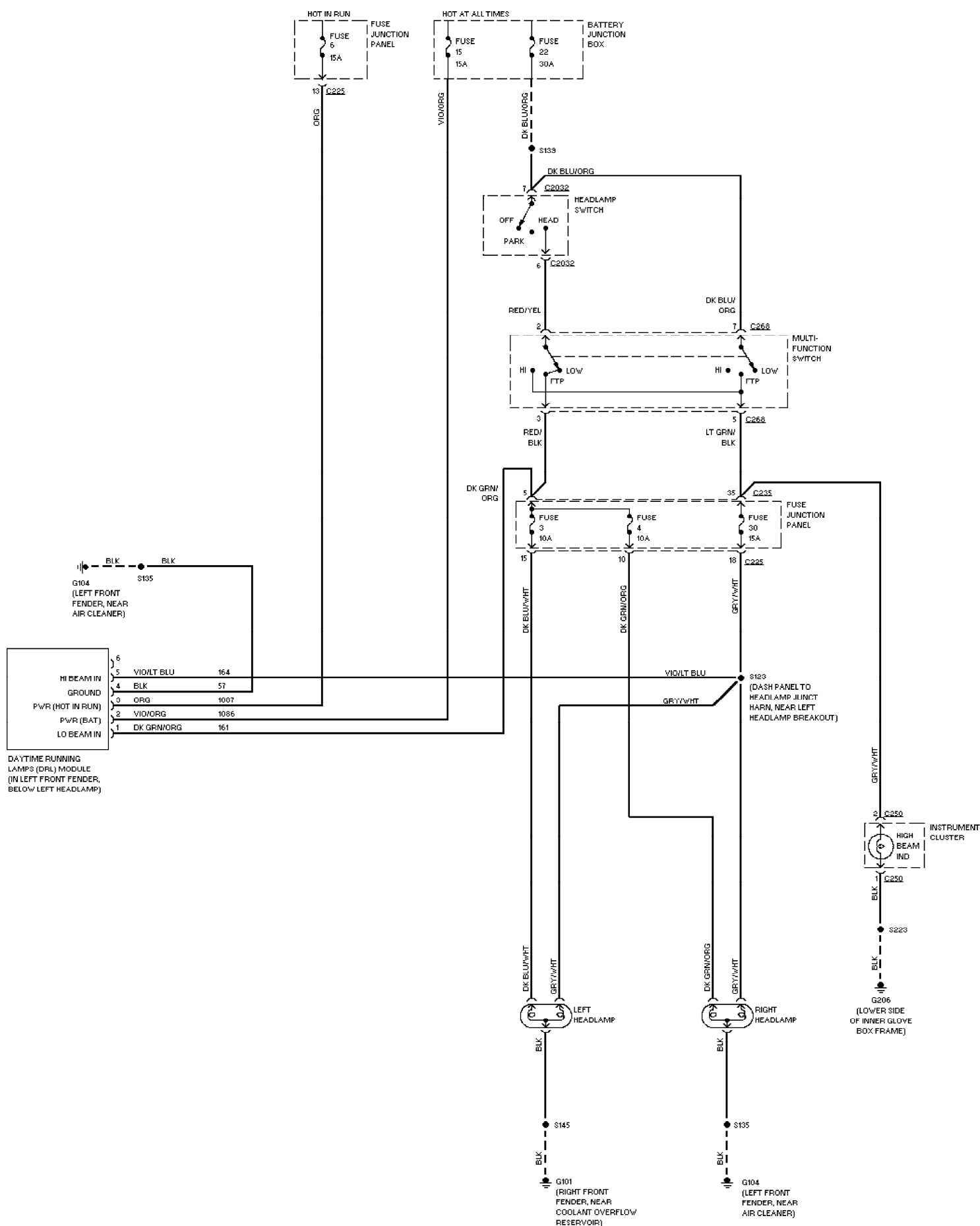
Fig. 36: Headlamps Circuit, W/ DRL 1999 Ford Taurus LX
