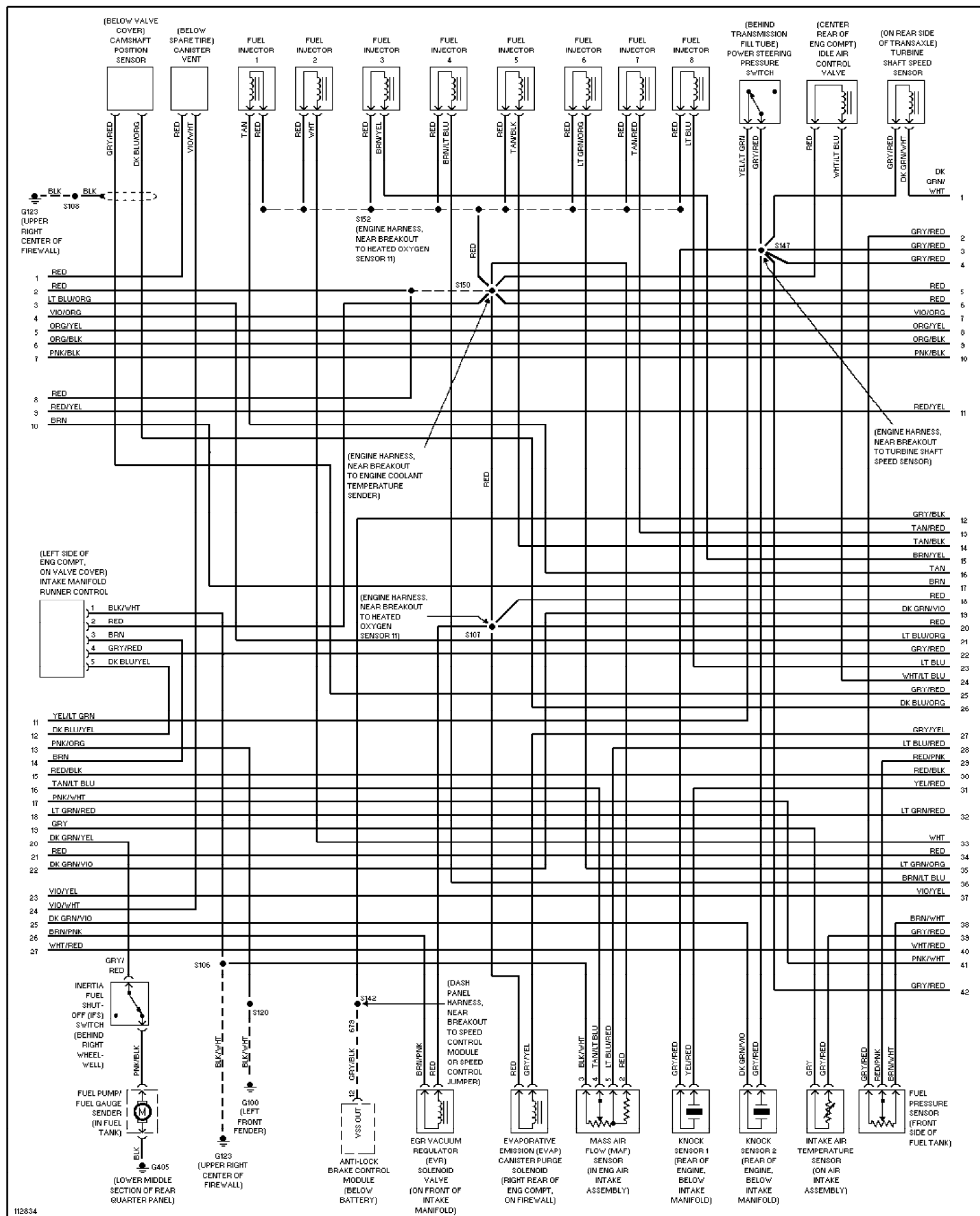
Fig. 24: 3.4L SHO, Engine Performance Circuits (2 of 3) 1999 Ford Taurus LX
