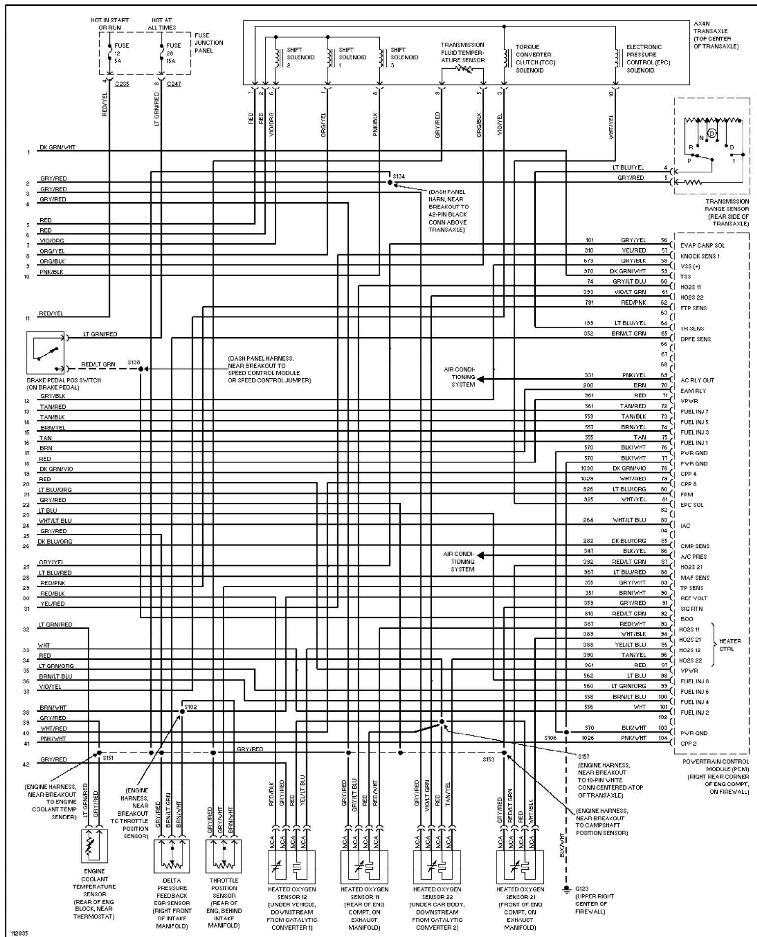
Fig. 25: 3.4L SHO, Engine Performance Circuits (3 of 3) 1999 Ford Taurus LX
