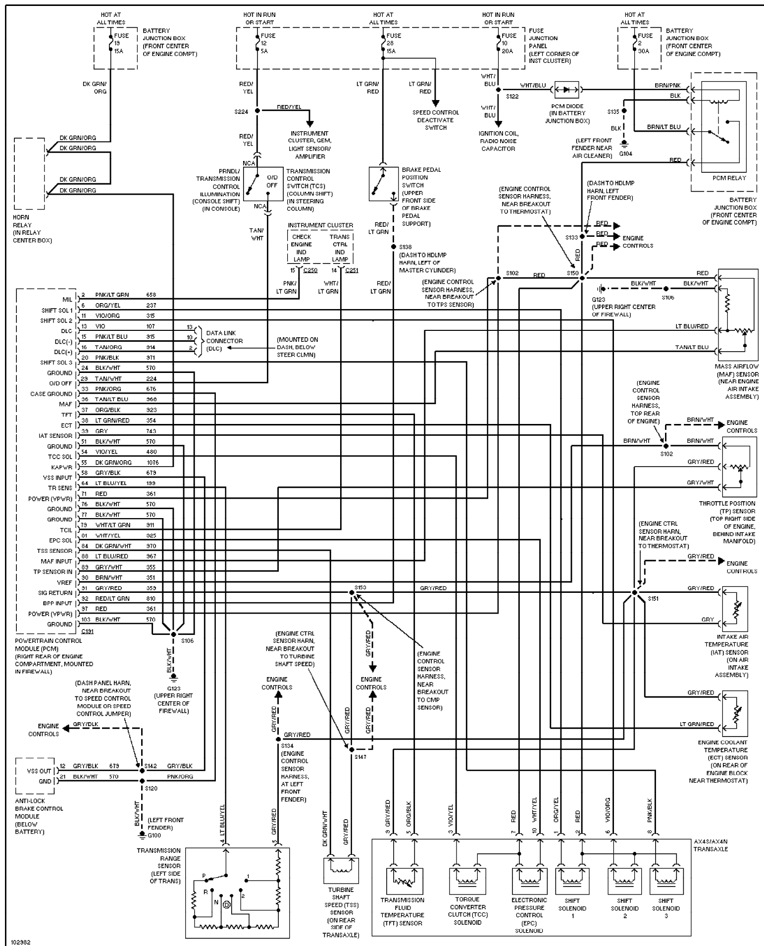
Fig. 64: 3.4L SHO, A/T Circuit 1999 Ford Taurus LX
