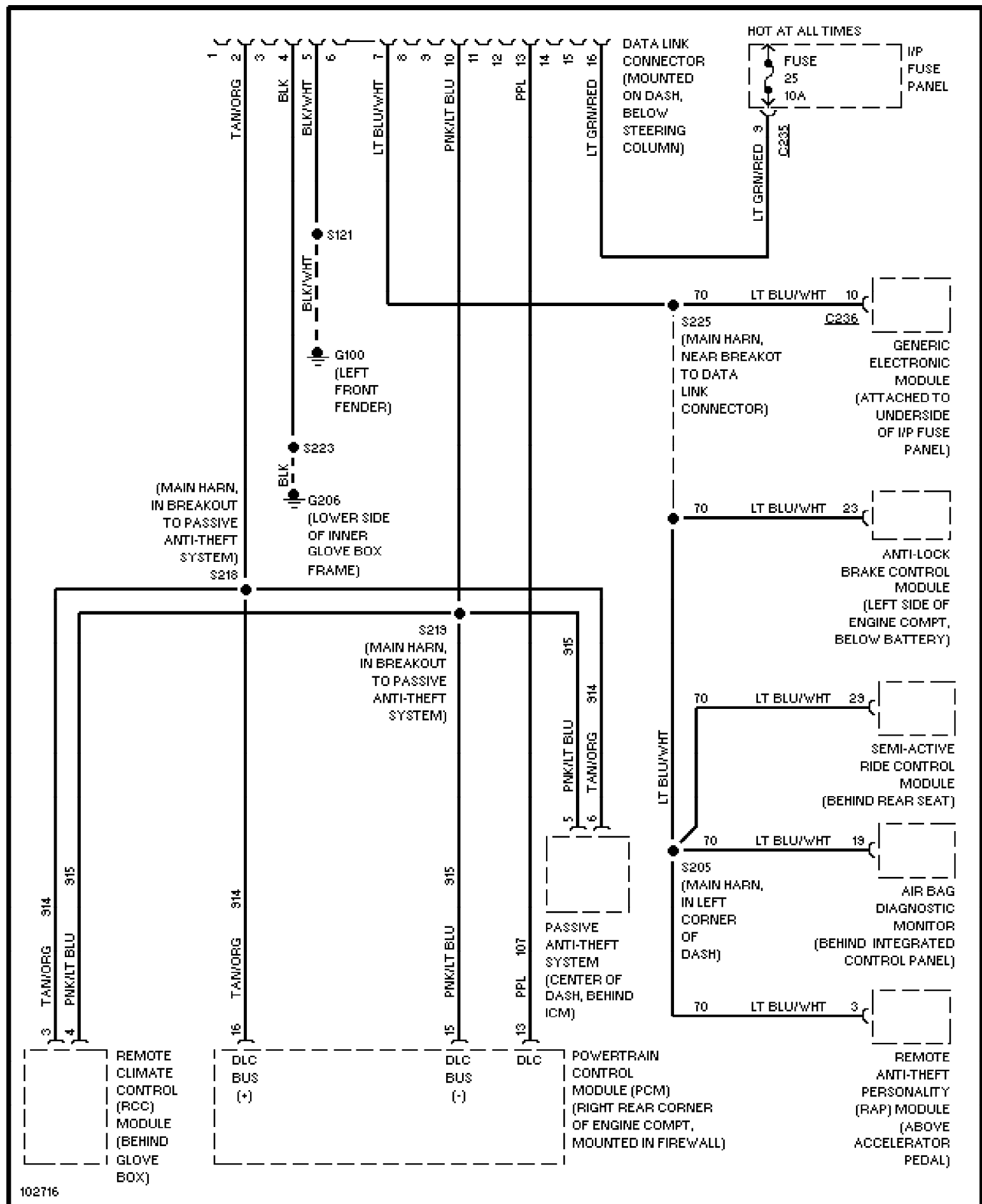
Fig. 8: Computer Data Lines 1999 Ford Taurus LX
