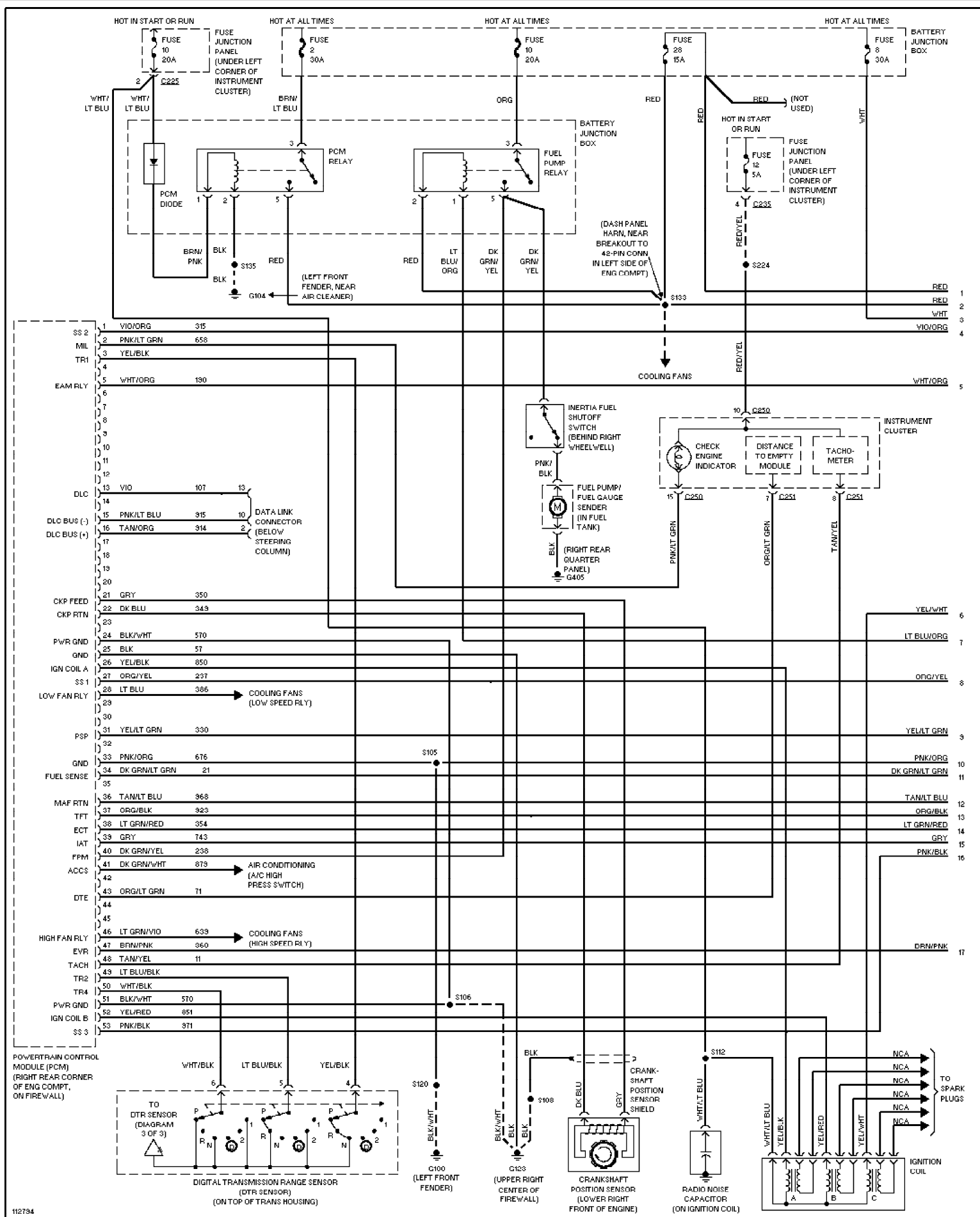
Fig. 20: 3.0L Flex Fuel, Engine Performance Circuits (1 of 3)
