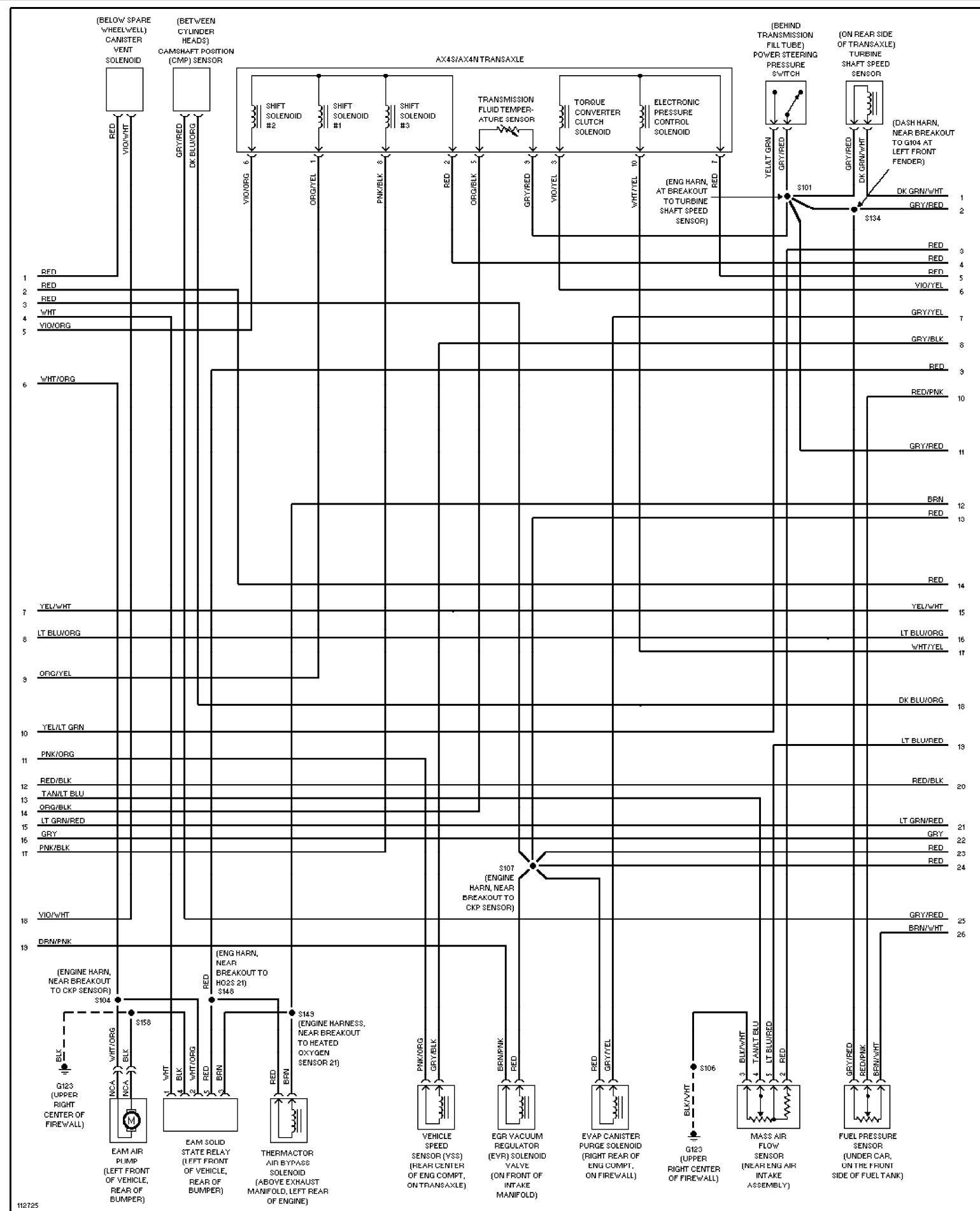
Fig. 15: 3.0L 12-Valve, Engine Performance Circuits (2 of 3)
