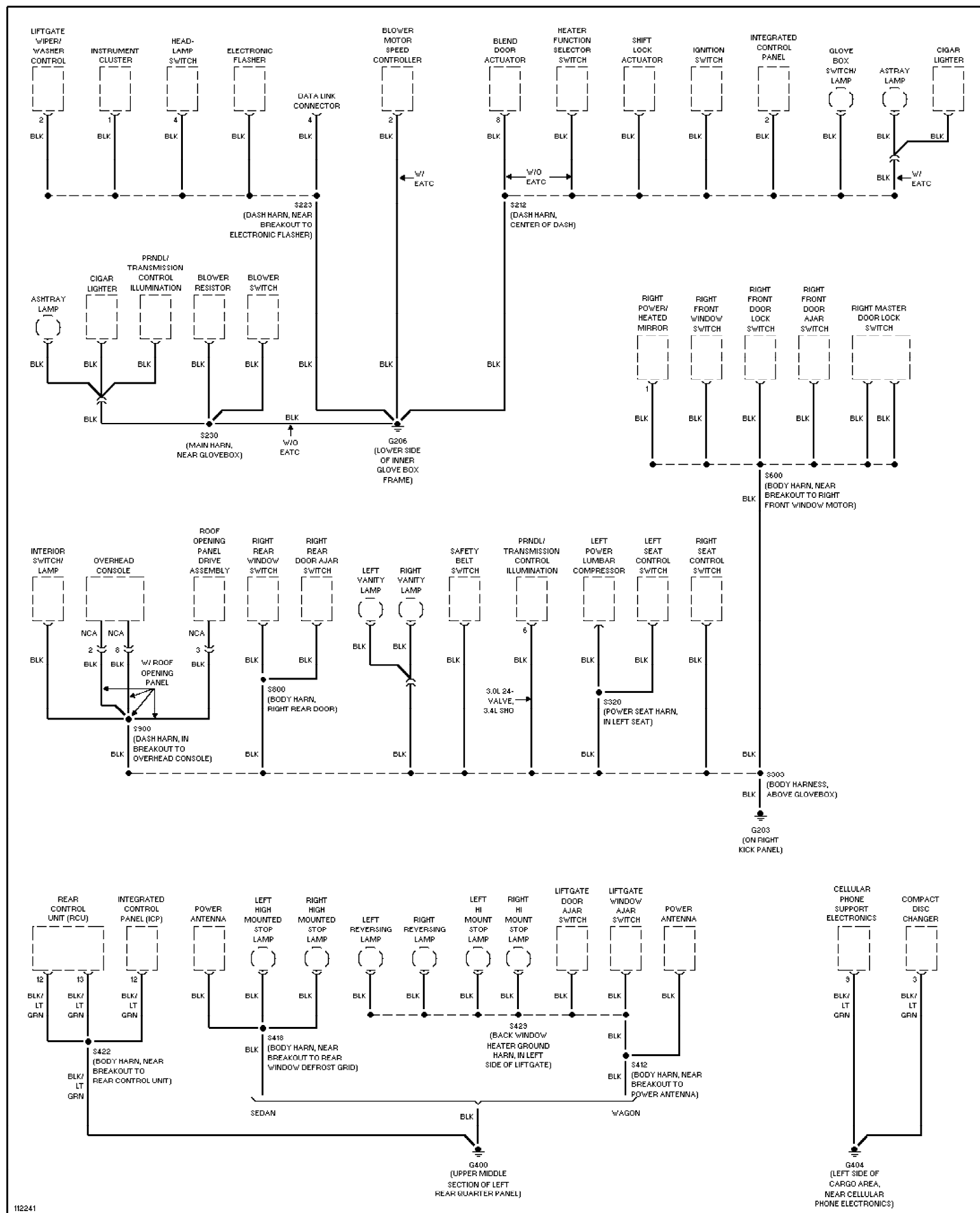
Fig. 32: Ground Distribution Circuit (2 of 3) 1999 Ford Taurus LX
