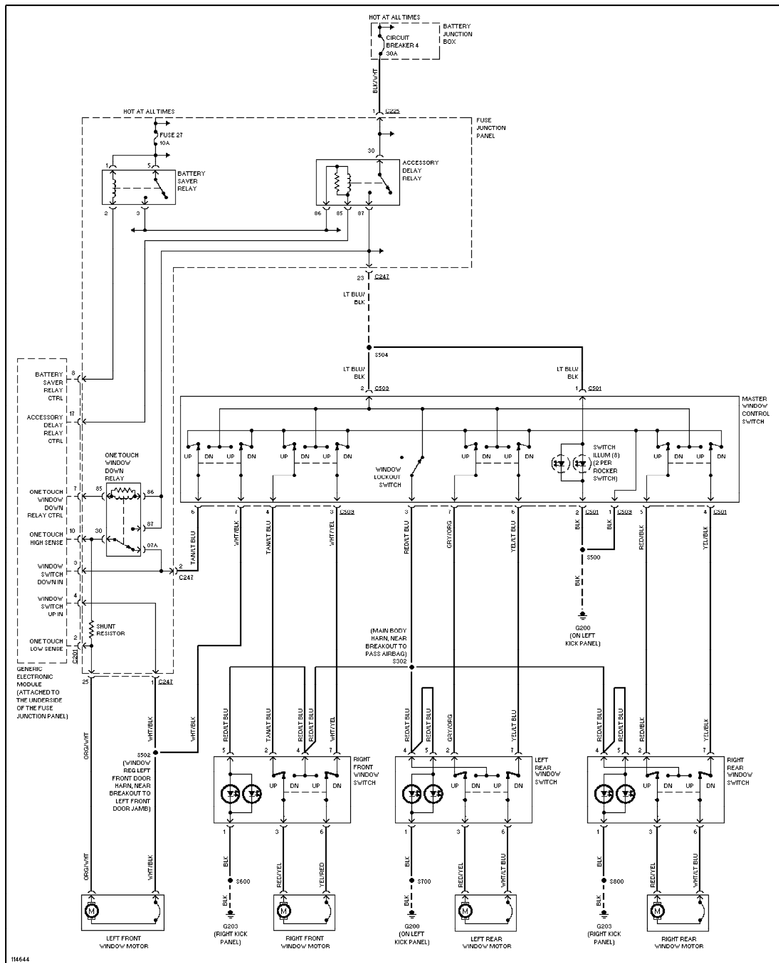
Fig. 54: Power Window Circuit 1999 Ford Taurus LX
