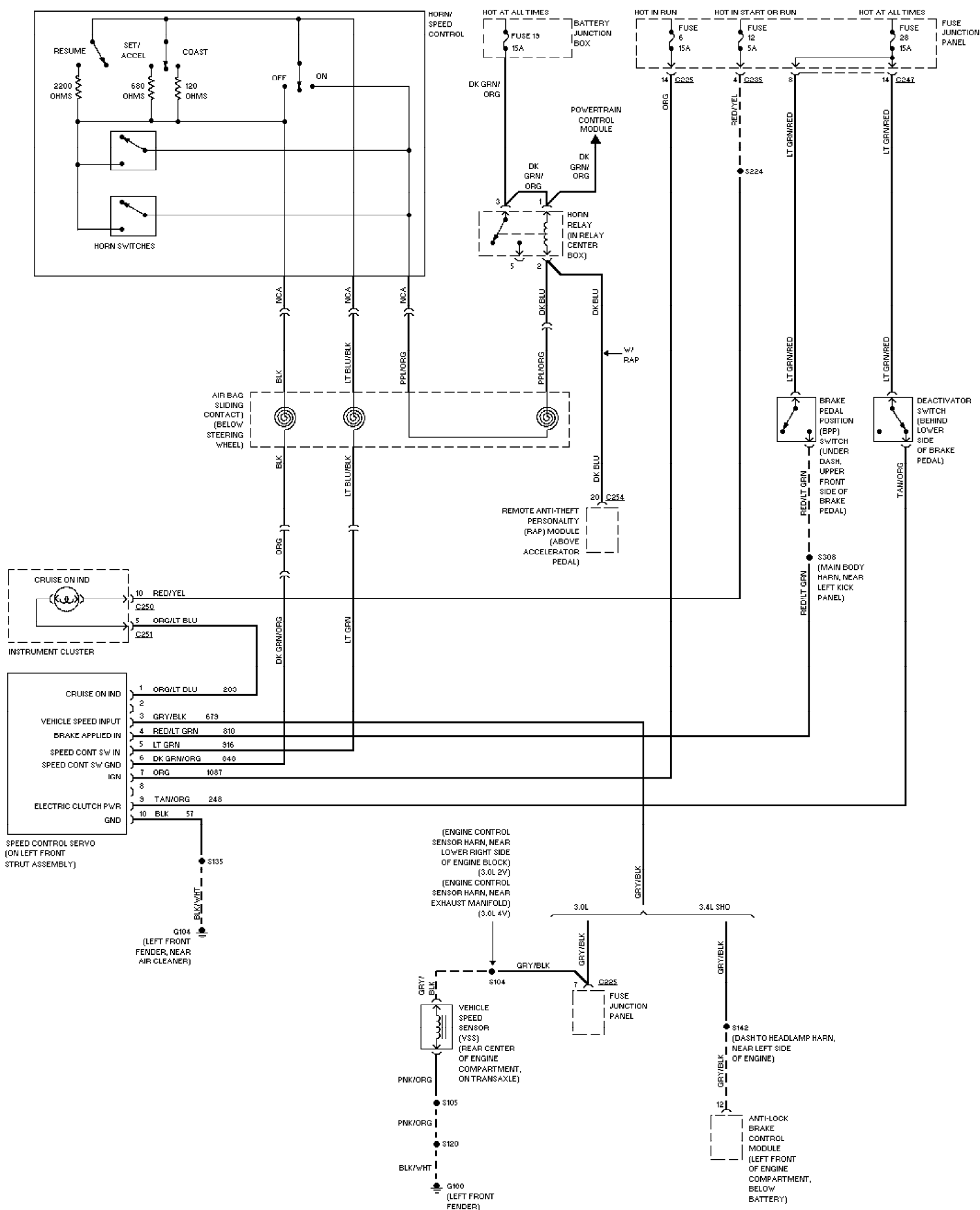
Fig. 10: Cruise Control Circuit 1999 Ford Taurus LX
