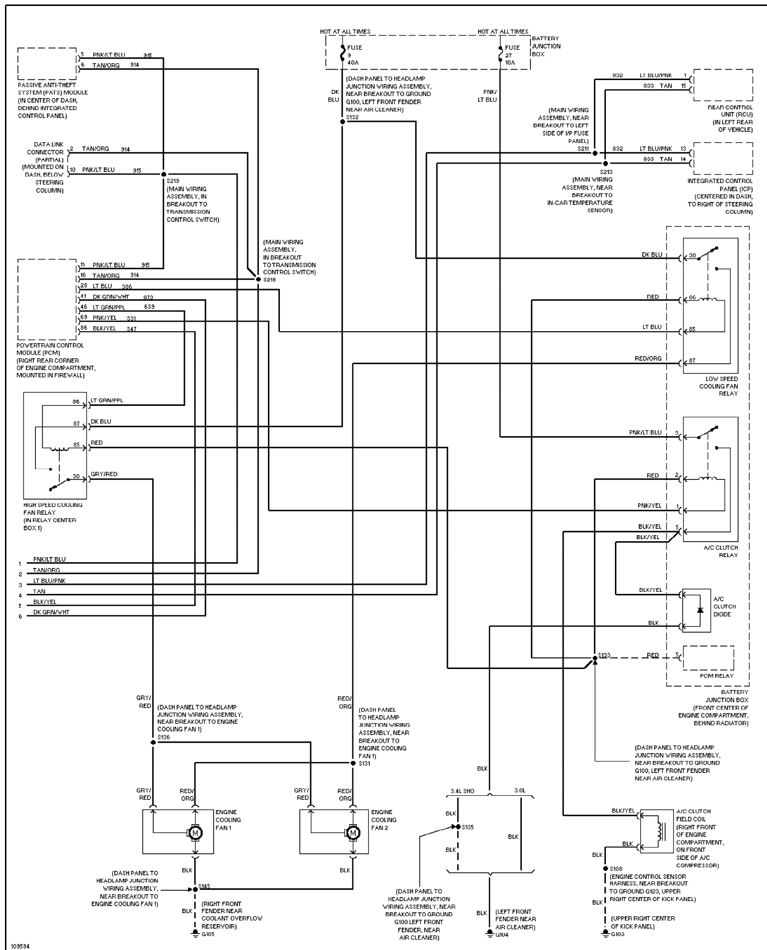
Fig. 2: Automatic A/C Circuit (2 of 2) 1999 Ford Taurus LX
