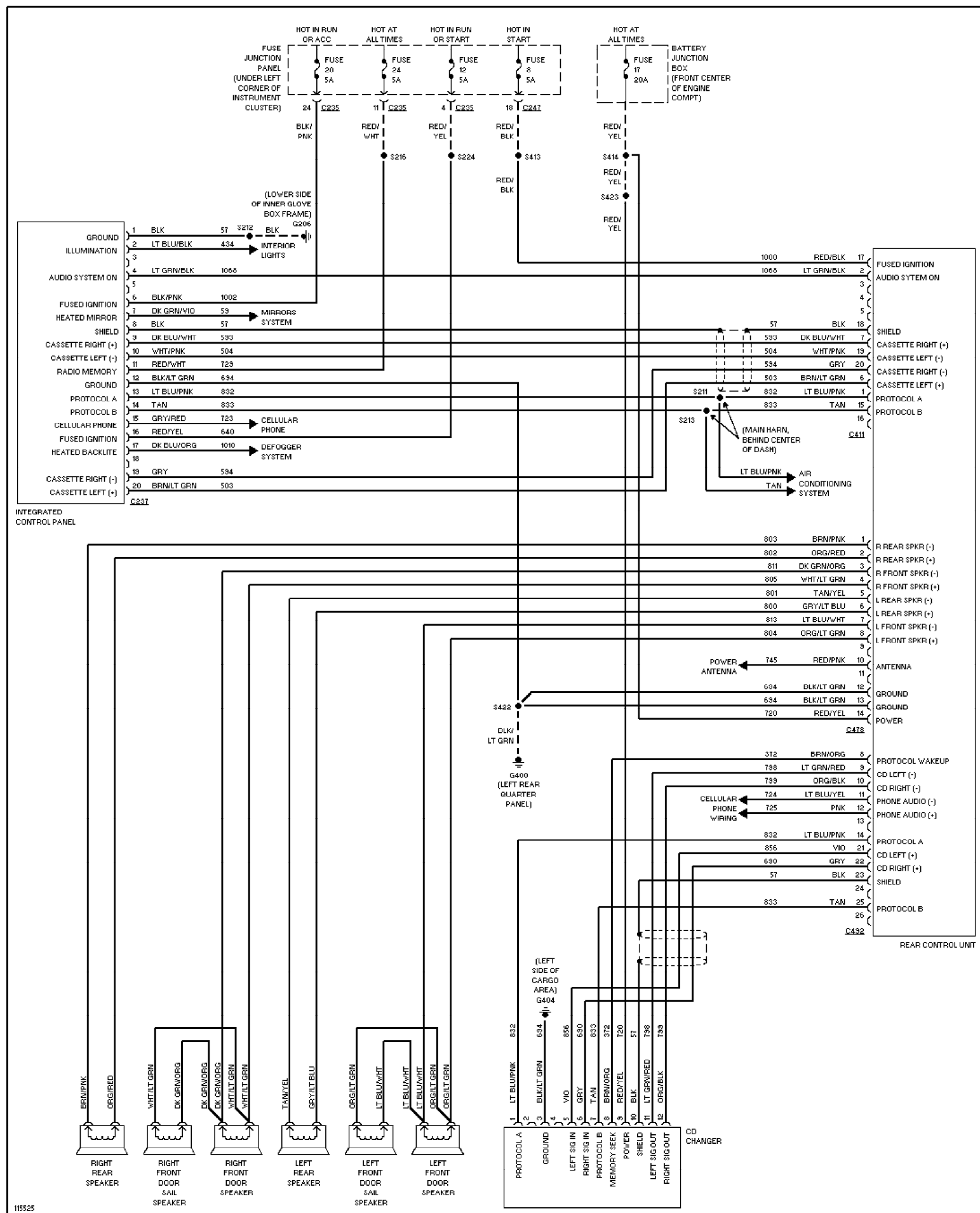
Fig. 55: Radio Circuits, W/ Cassette Deck 1999 Ford Taurus LX
