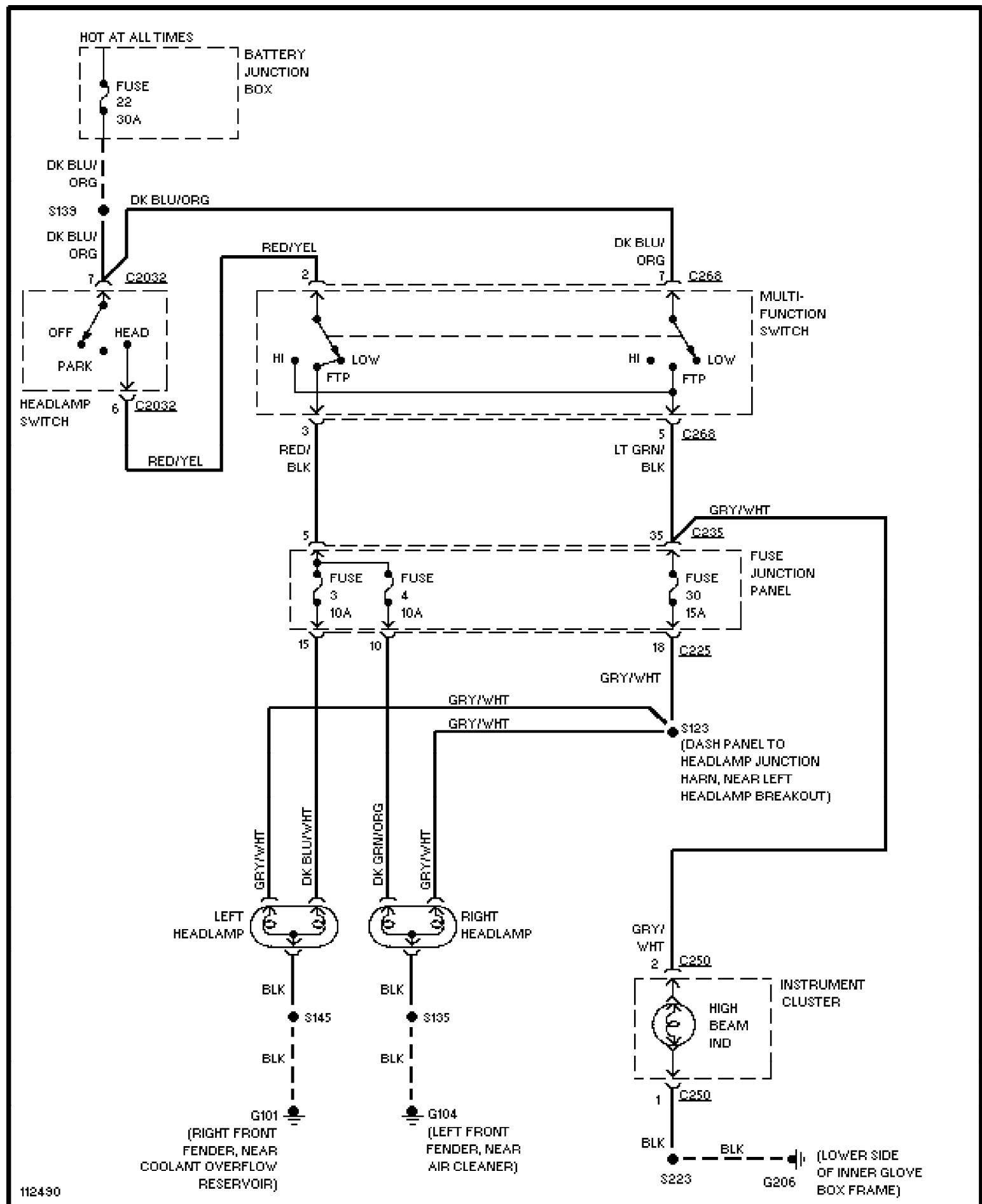
Fig. 37: Headlamps Circuit, W/O DRL 1999 Ford Taurus LX
