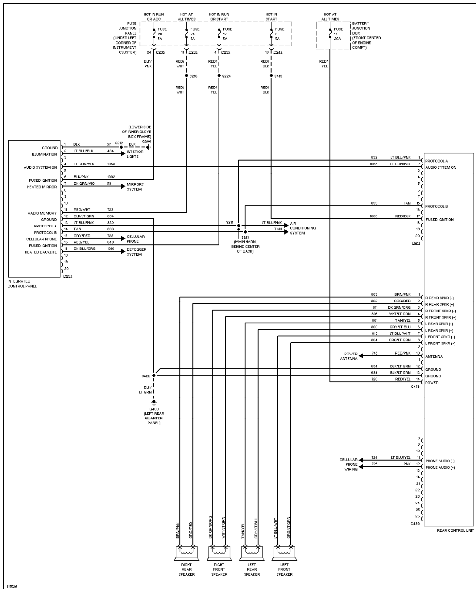
Fig. 56: Radio Circuits, W/O Cassette Deck 1999 Ford Taurus LX
