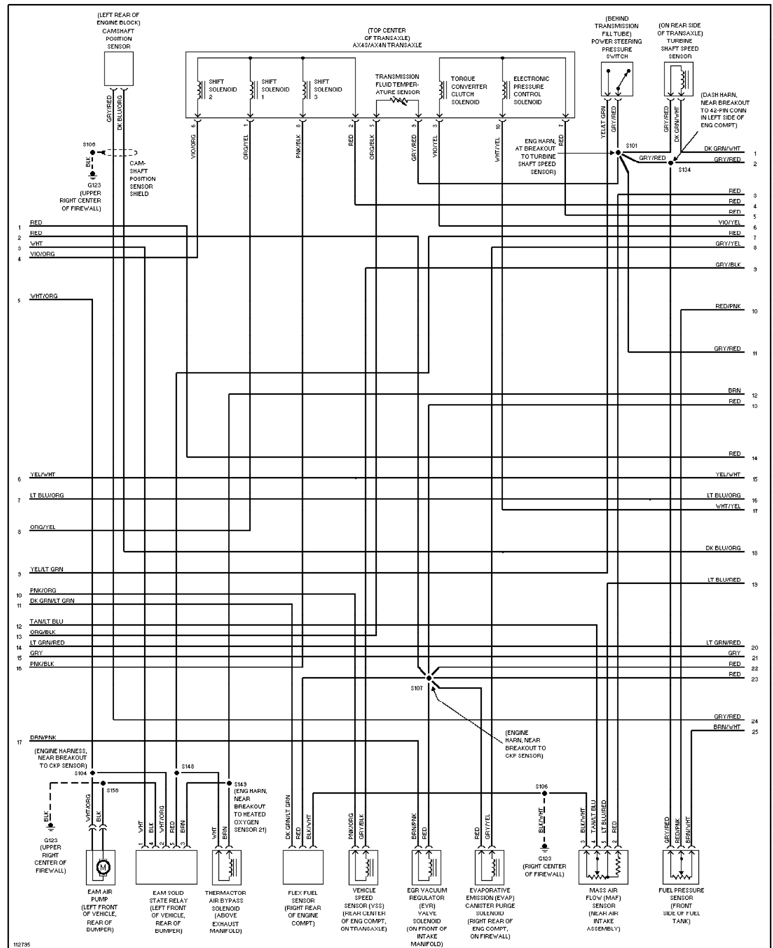
Fig. 21: 3.0L Flex Fuel, Engine Performance Circuits (2 of 3) 1999 Ford Taurus LX
