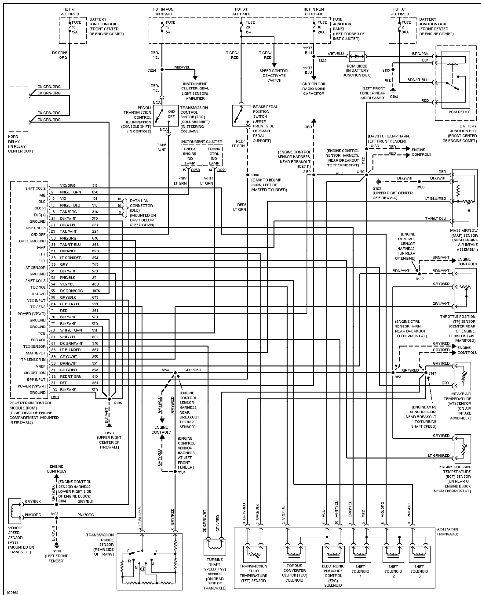
Fig. 62: 3.0L 24-Valve, A/T Circuit 1999 Ford Taurus LX
