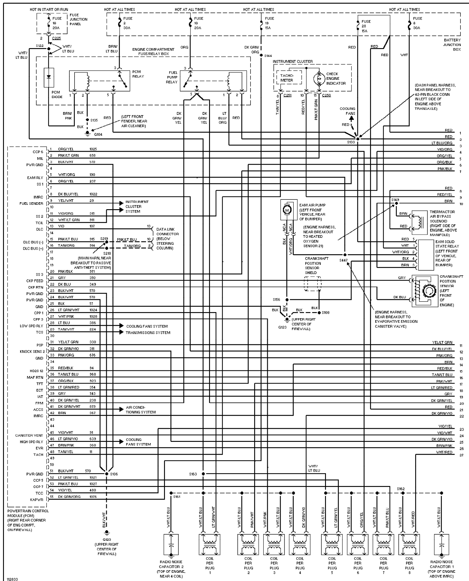
Fig. 23: 3.4L SHO, Engine Performance Circuits (1 of 3) 1999 Ford Taurus LX
