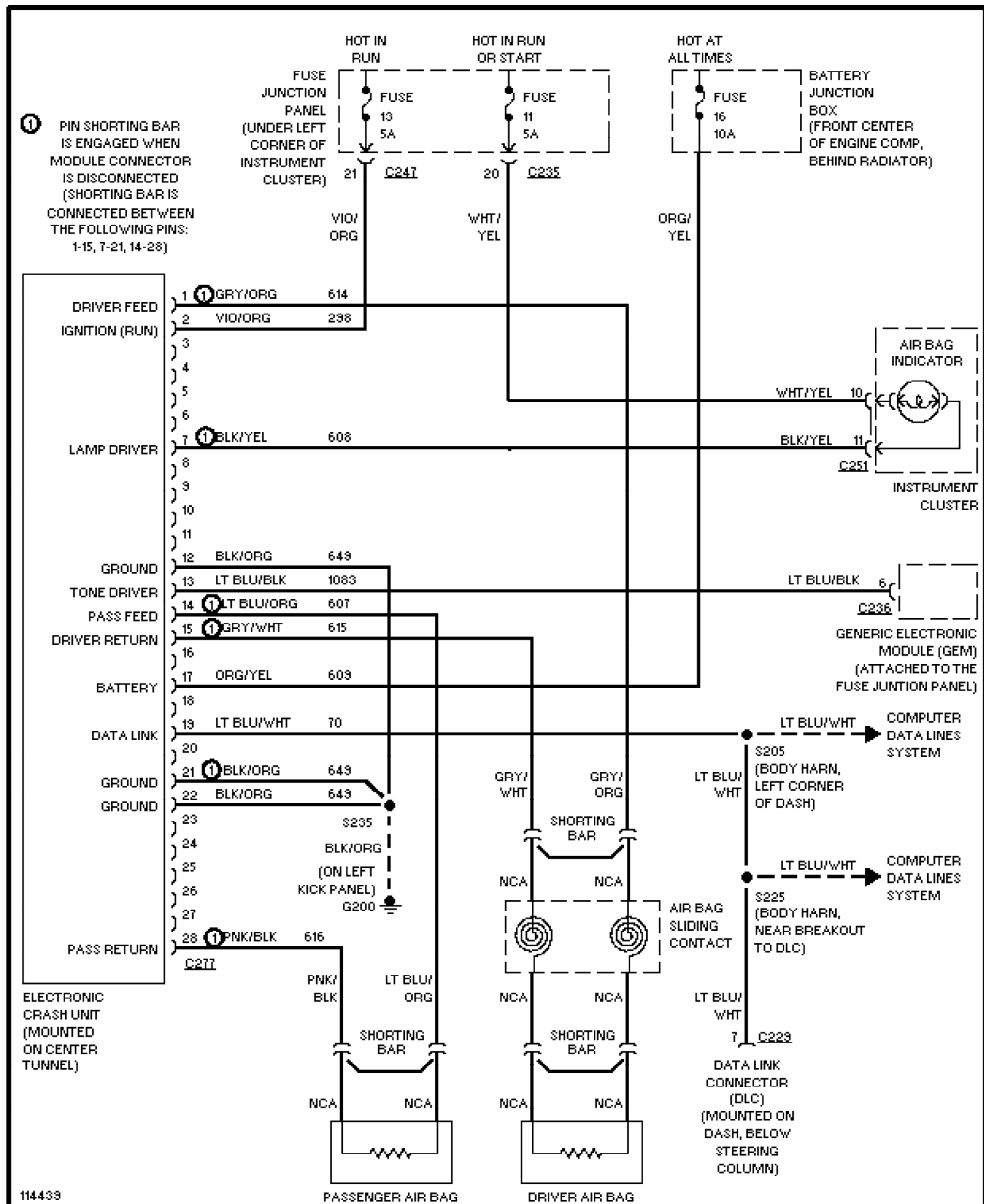
Fig. 60: Supplemental Restraint Circuit 1999 Ford Taurus LX
