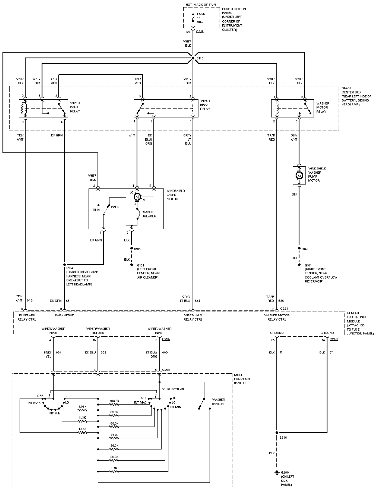
Fig. 67: Front Wiper/Washer Circuit 1999 Ford Taurus LX
