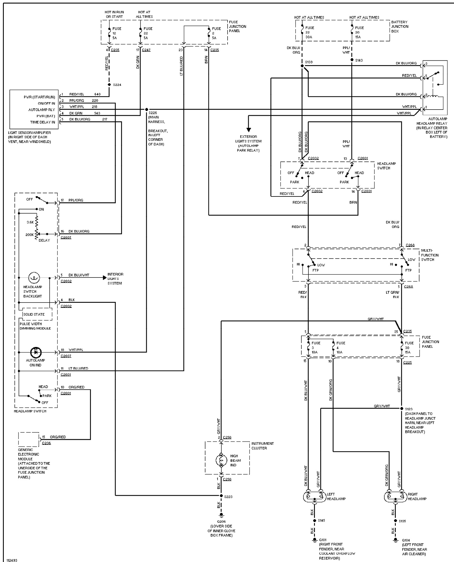
Fig. 35: Autolamps Circuit, W/O DRL 1999 Ford Taurus LX
