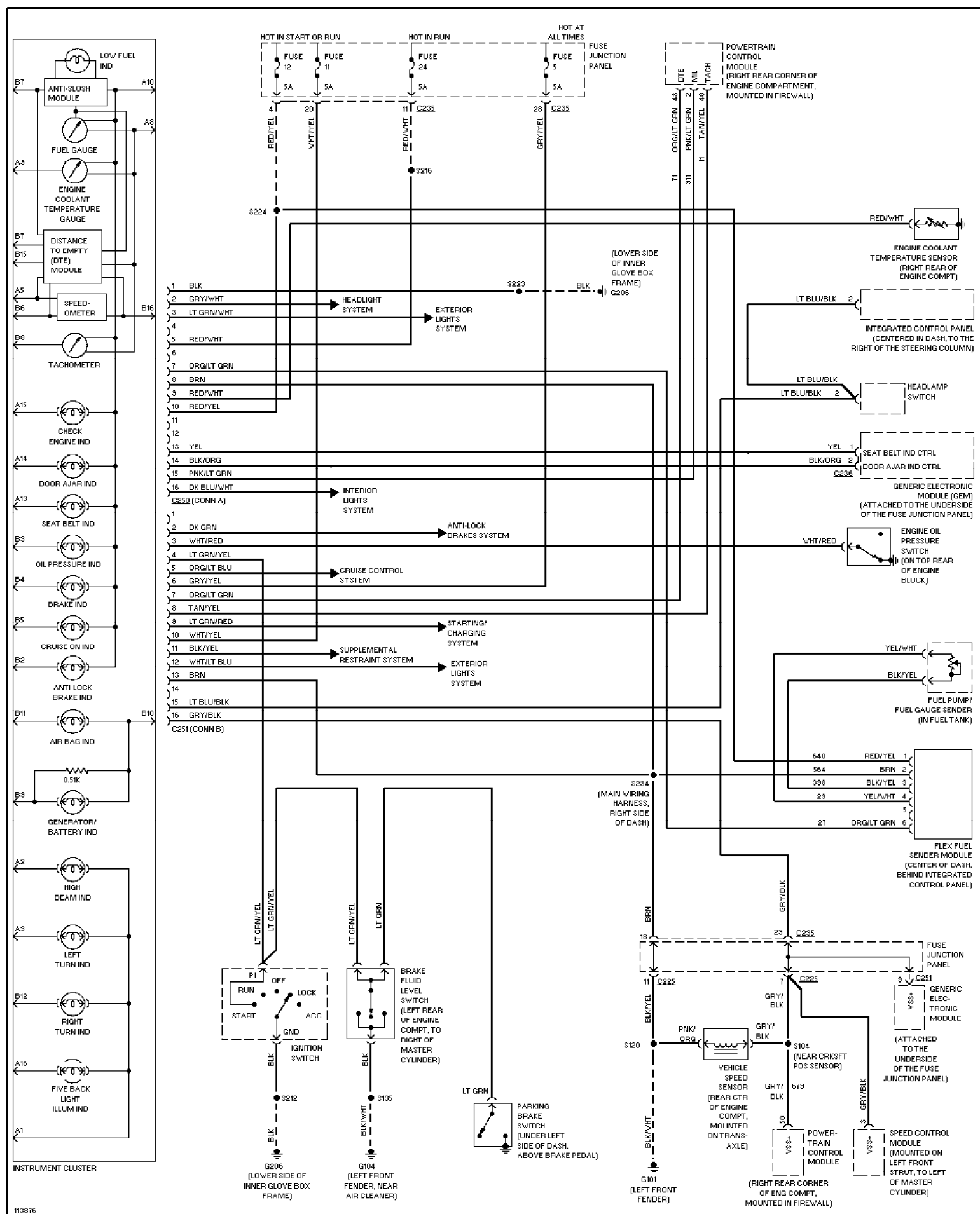
Fig. 39: 3.0L Flex Fuel, Instrument Cluster Circuit 1999 Ford Taurus LX
