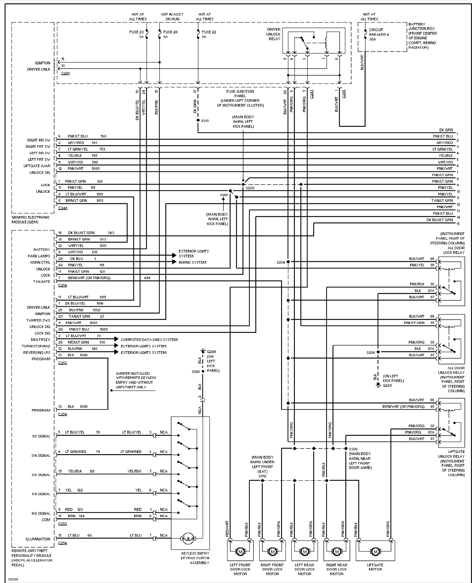
Fig. 48: Power Door Lock Circuit, W/ Keyless Entry (1 of 2)
