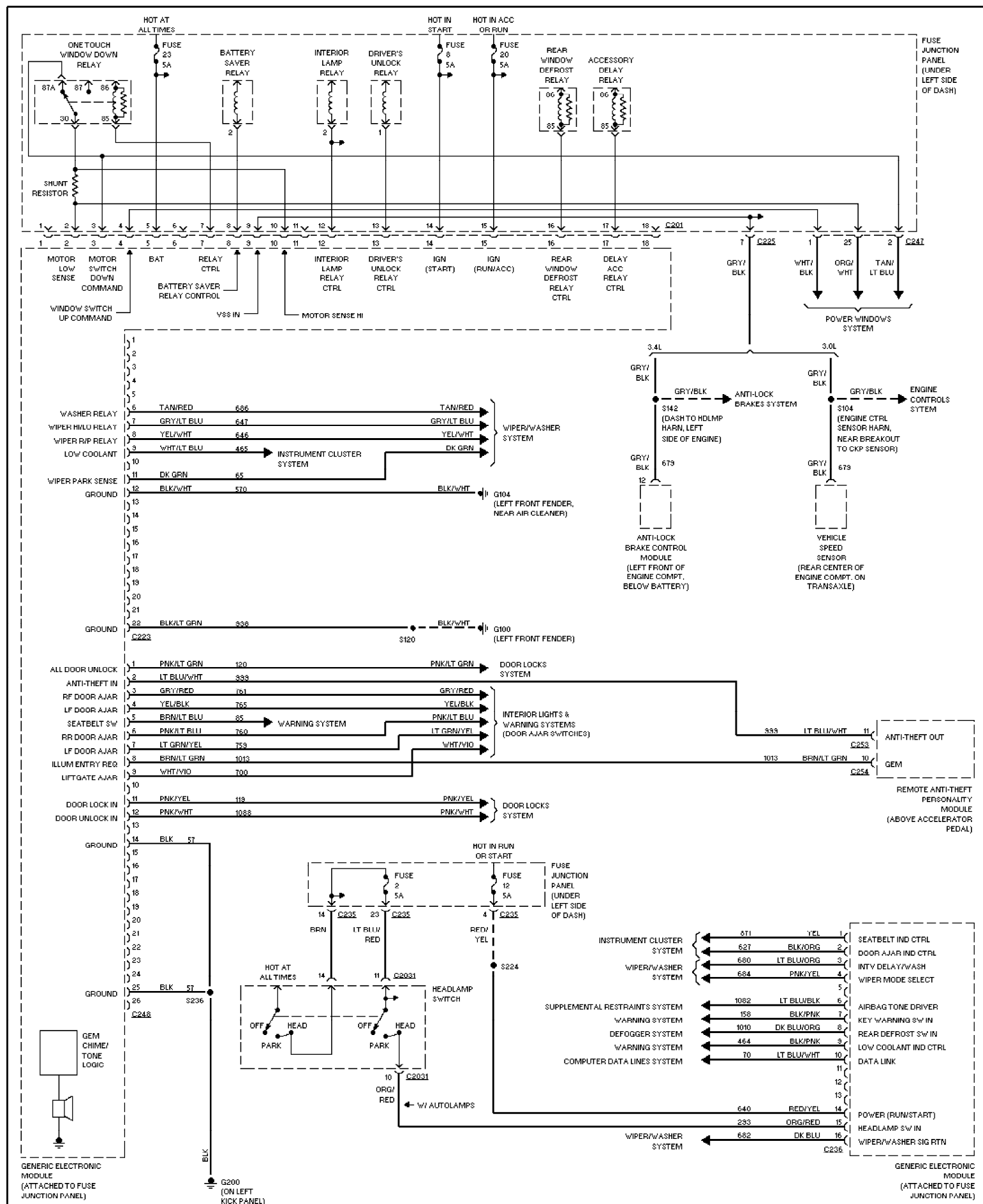
Fig. 7: Body Computer Circuits 1999 Ford Taurus LX
