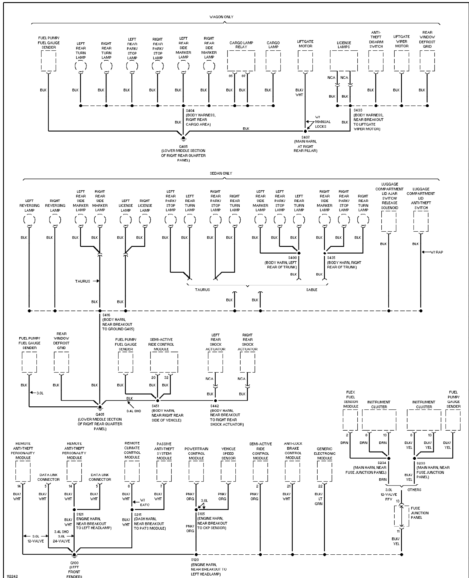
Fig. 33: Ground Distribution Circuit (3 of 3) 1999 Ford Taurus LX
