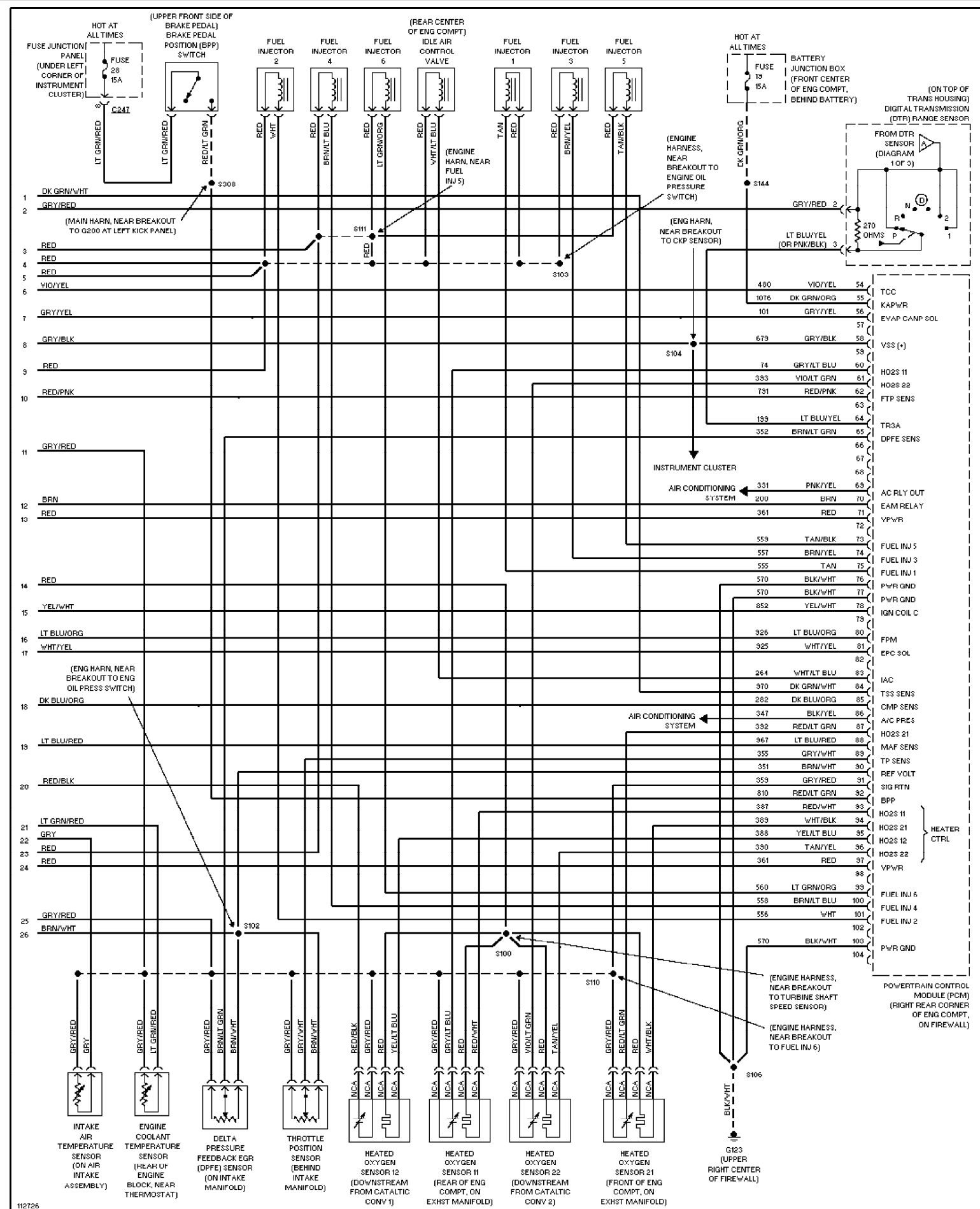
Fig. 16: 3.0L 12-Valve, Engine Performance Circuits (3 of 3)
