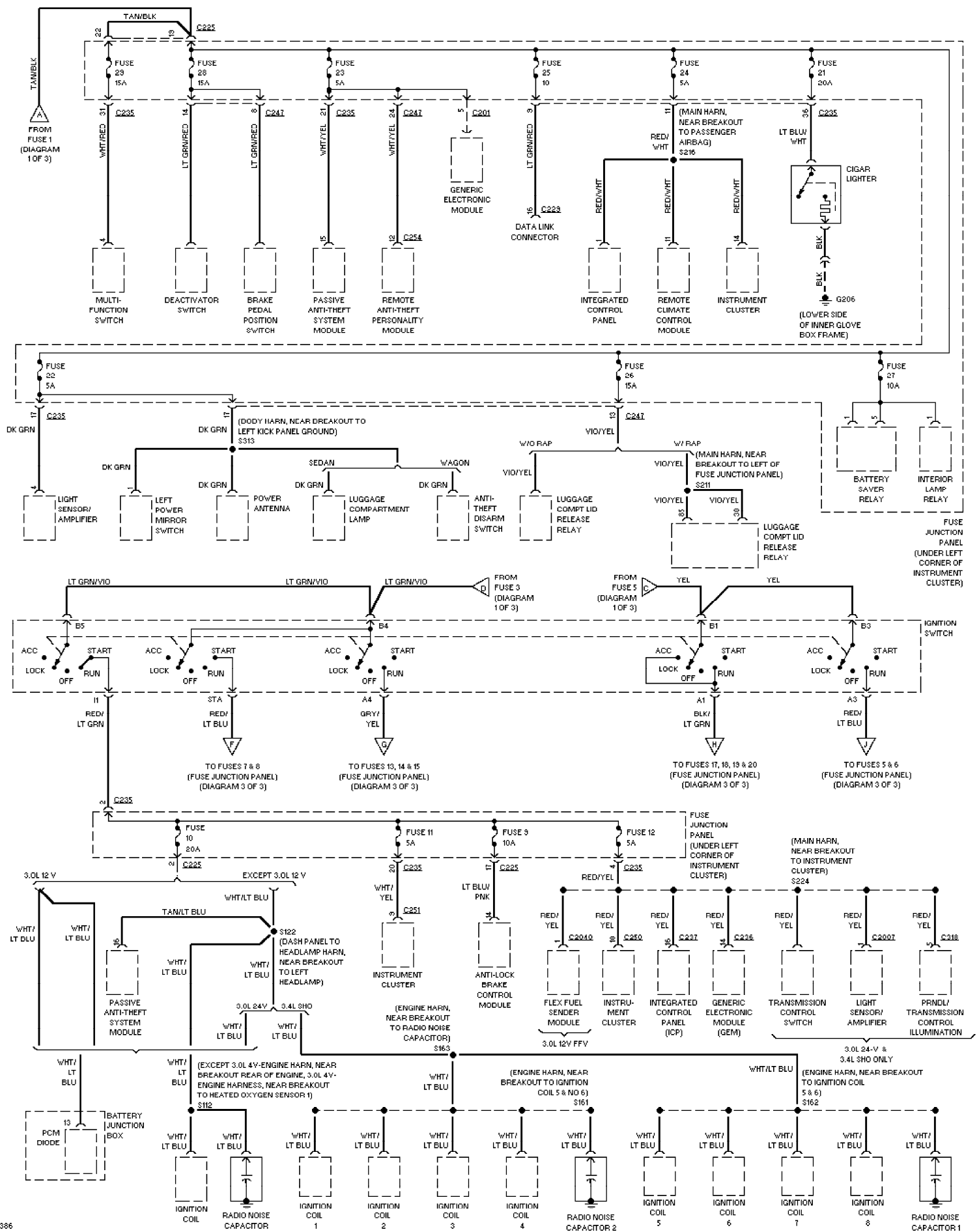
Fig. 46: Power Distribution Circuit (2 of 3) 1999 Ford Taurus LX
