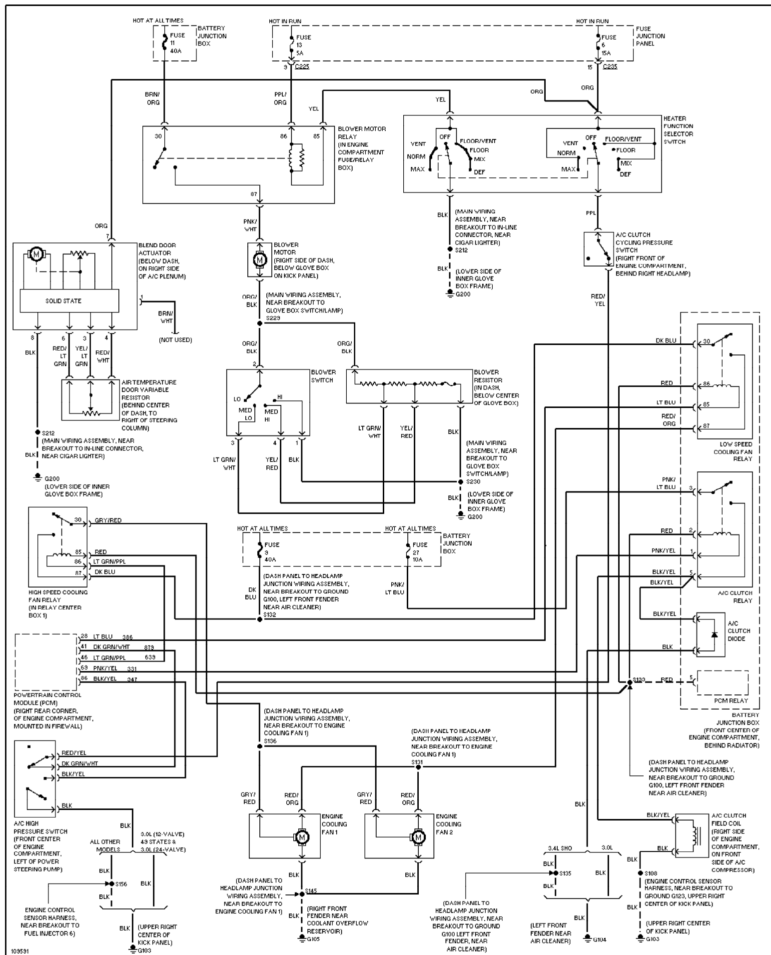
Fig. 3: Manual A/C Circuit 1999 Ford Taurus LX
