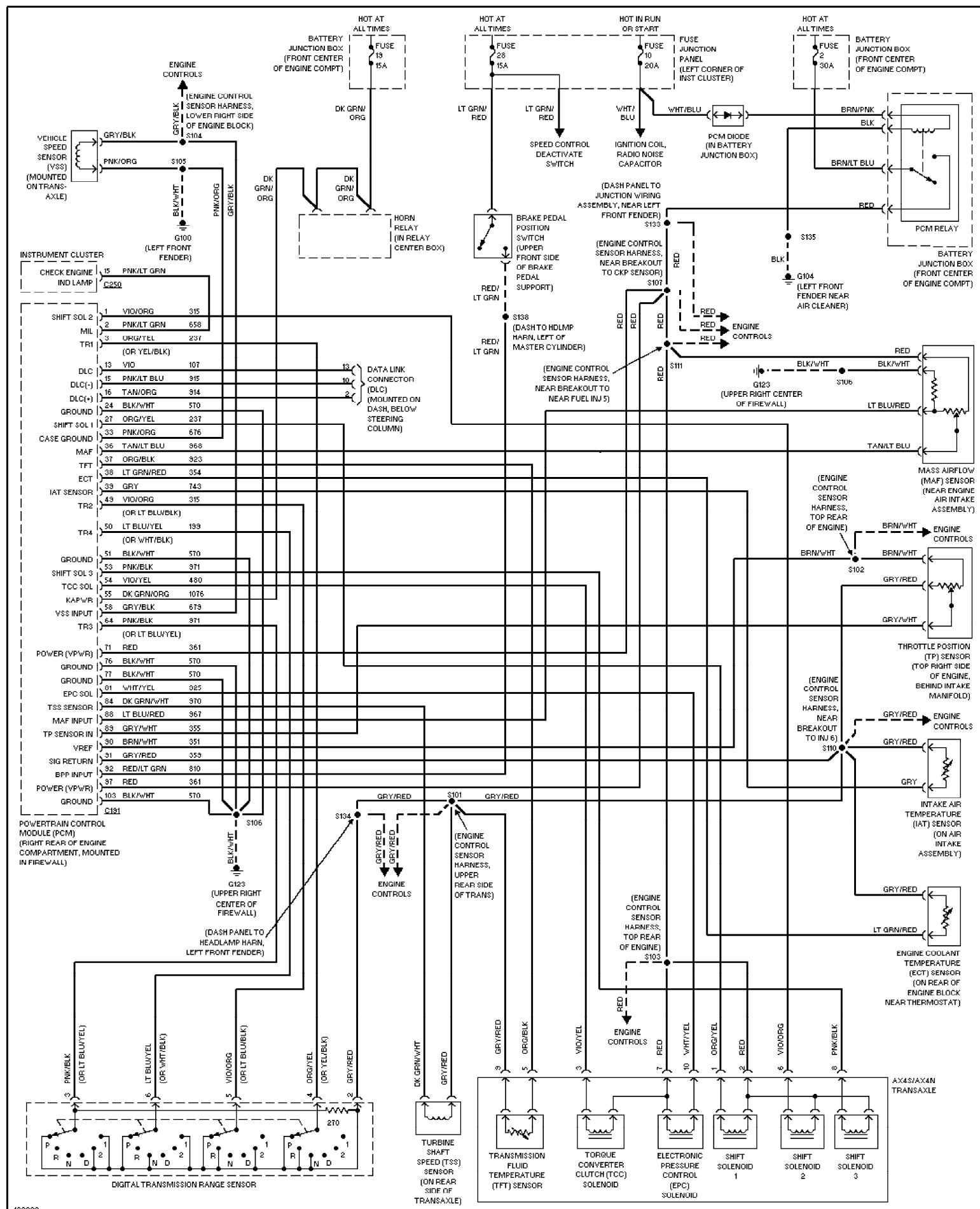
Fig. 61: 3.0L 12-Valve, A/T Circuit 1999 Ford Taurus LX
