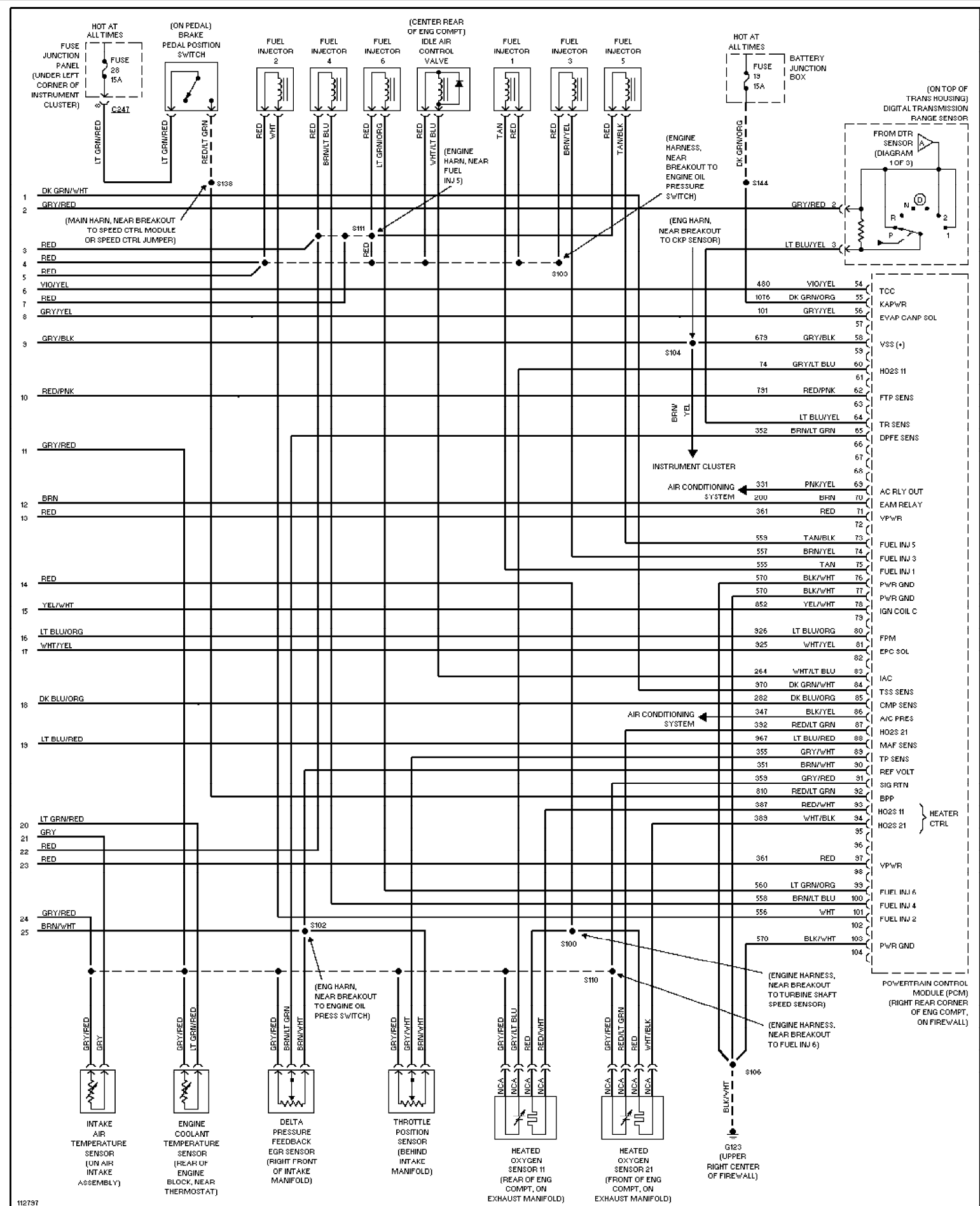
Fig. 22: 3.0L Flex Fuel, Engine Performance Circuits (3 of 3)
