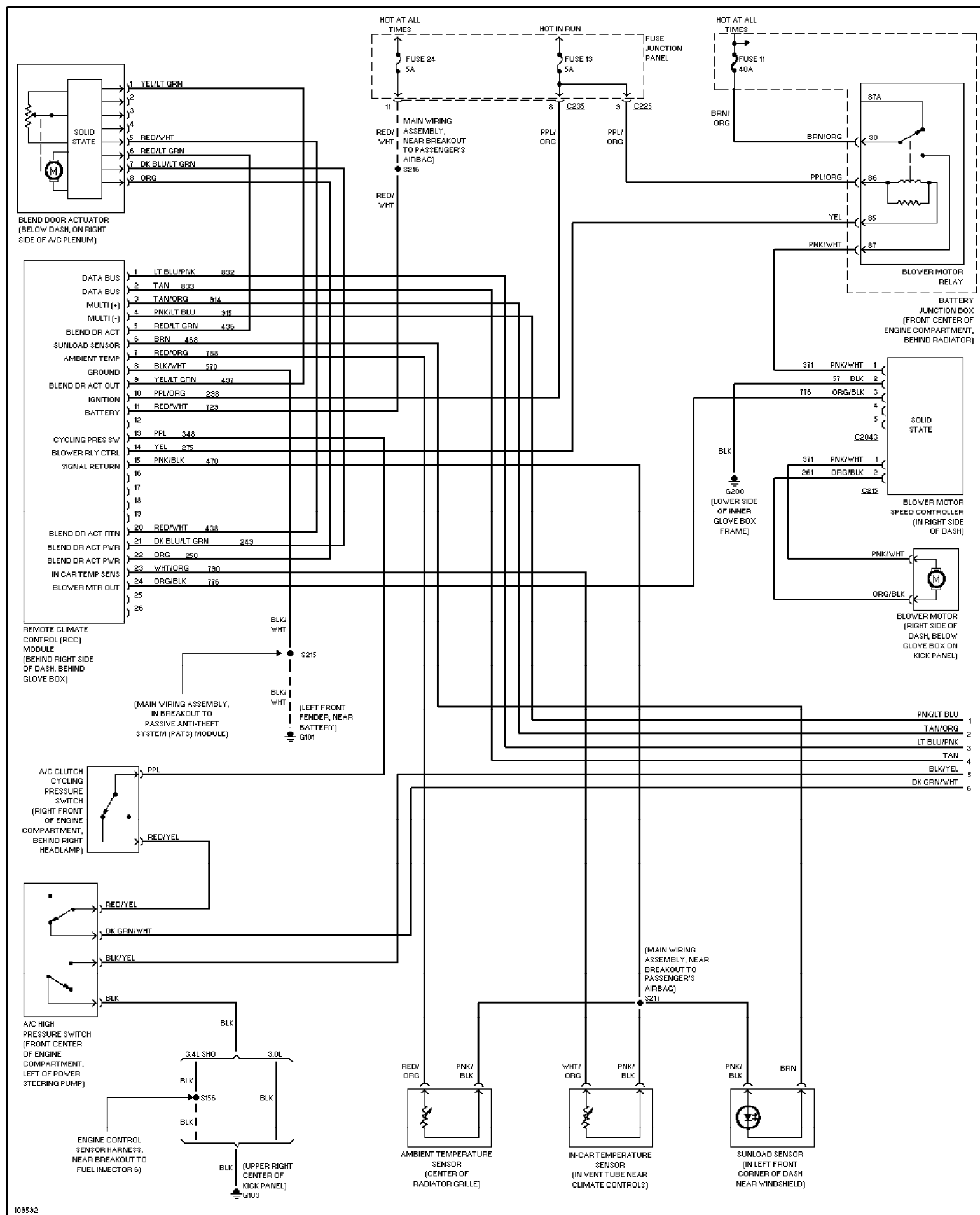
Fig. 1: Automatic A/C Circuit (1 of 2) 1999 Ford Taurus LX
