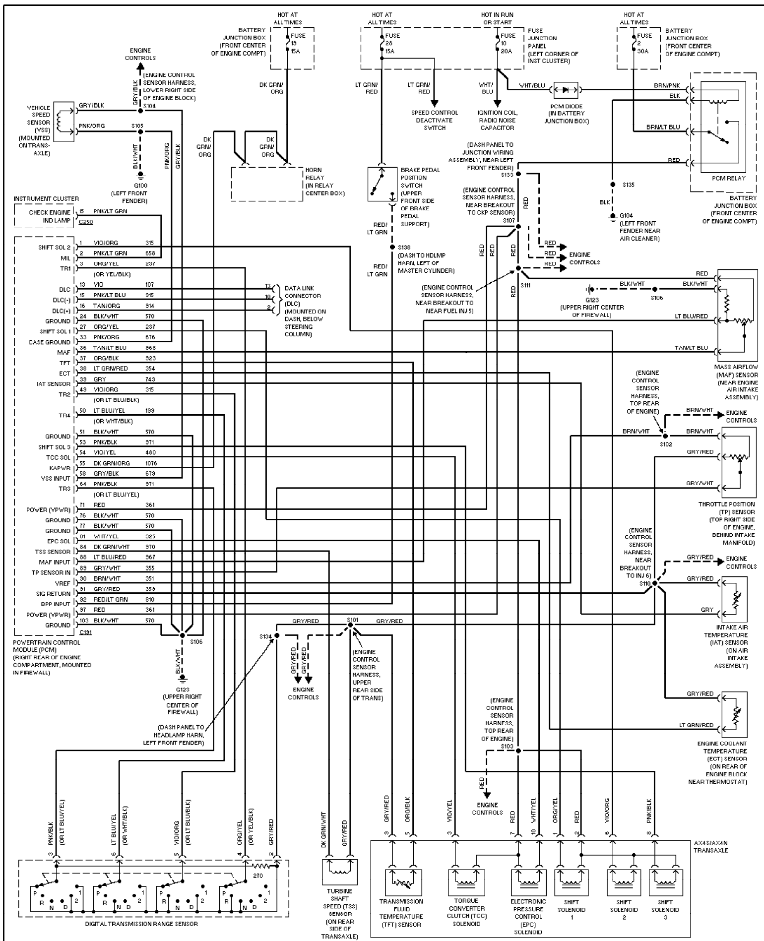
Fig. 63: 3.0L Flex Fuel, A/T Circuit 1999 Ford Taurus LX
