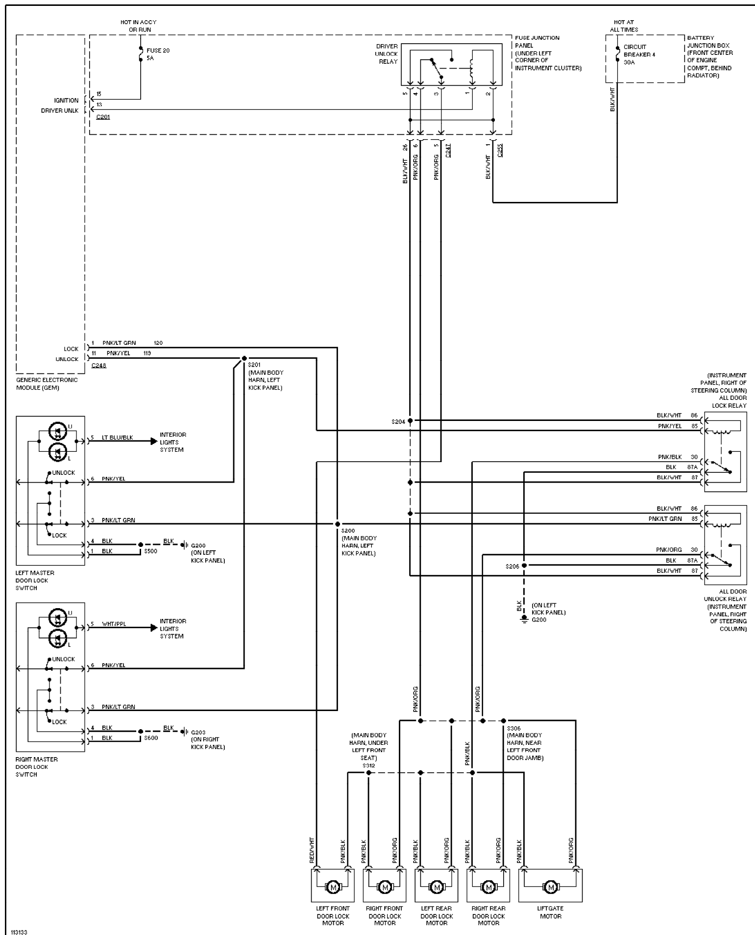
Fig. 50: Power Door Lock Circuit, W/O Keyless Entry 1999 Ford Taurus LX
