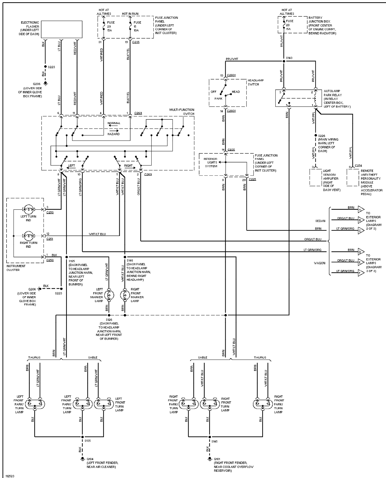
Fig. 28: Exterior Lamps Circuit (1 of 3) 1999 Ford Taurus LX
