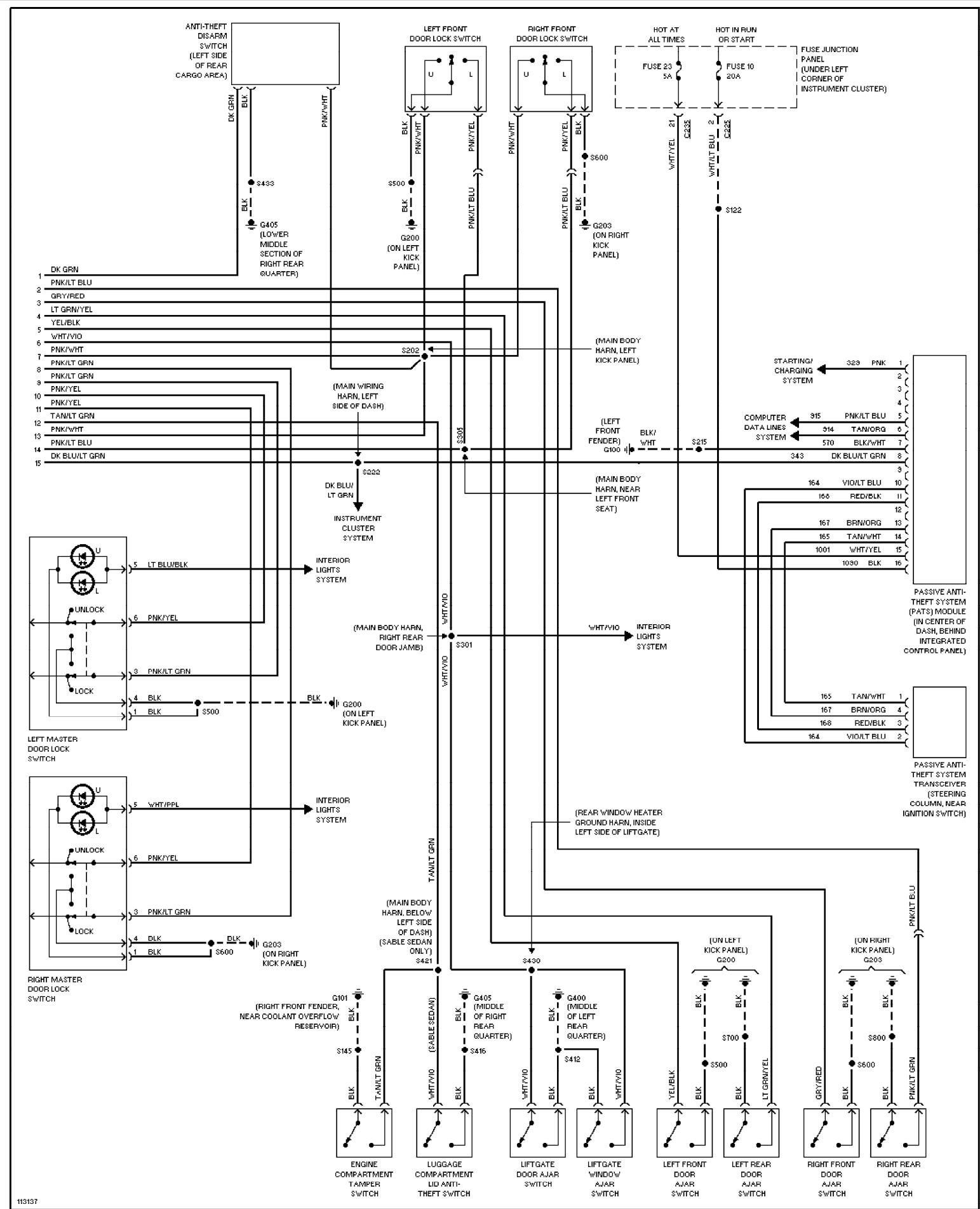
Fig. 49: Power Door Lock Circuit, W/ Keyless Entry (2 of 2)
