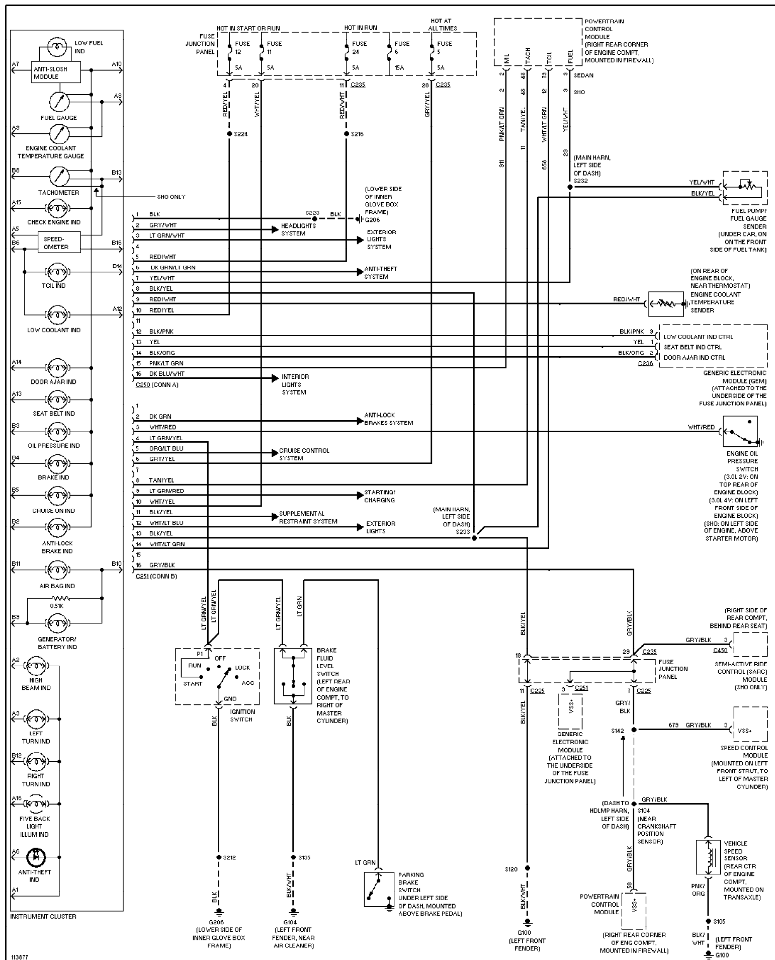
Fig. 40: 3.0L, Instrument Cluster Circuit 1999 Ford Taurus LX
