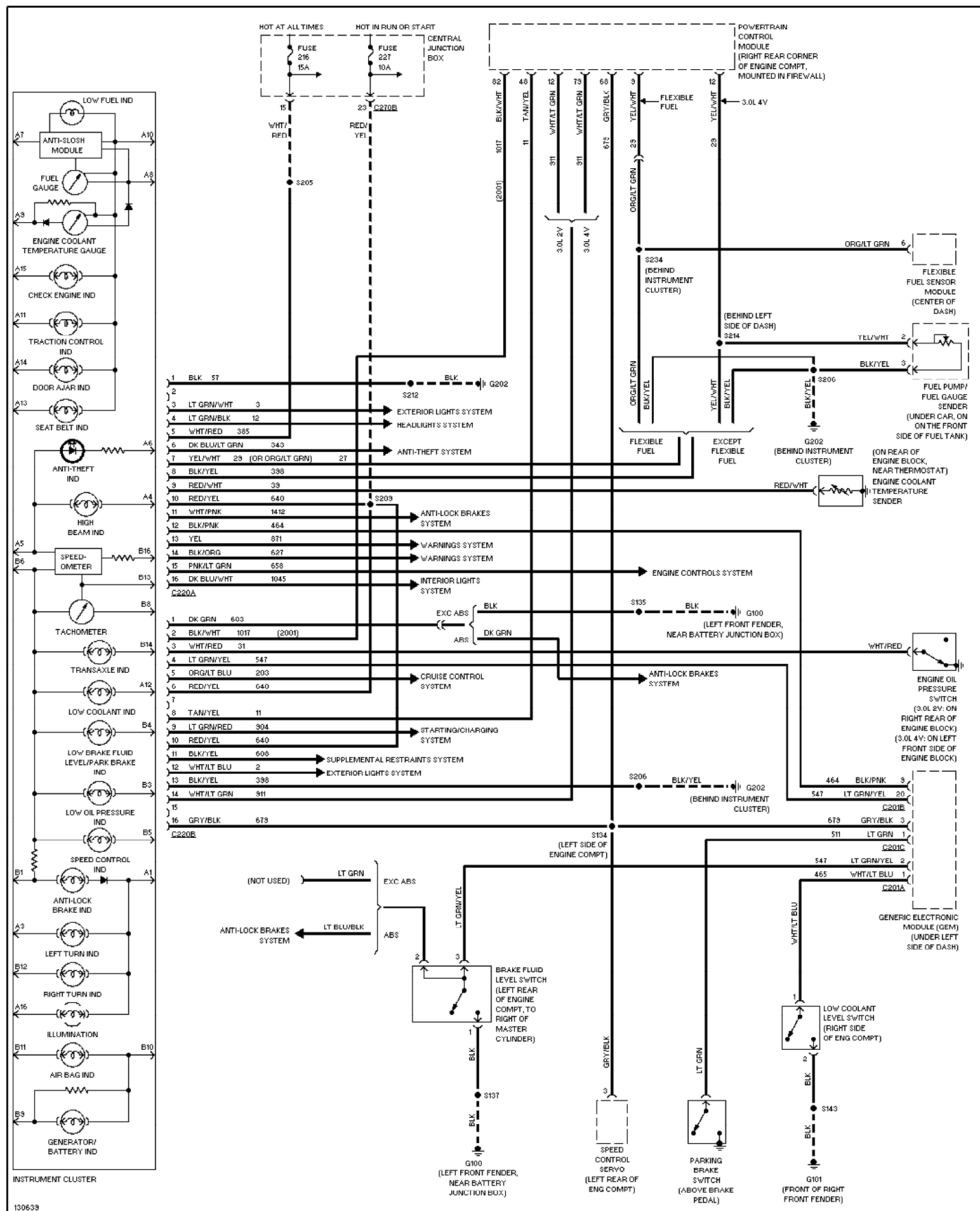
Fig. 36: Instrument Cluster Circuit 2000 Ford Taurus SES
