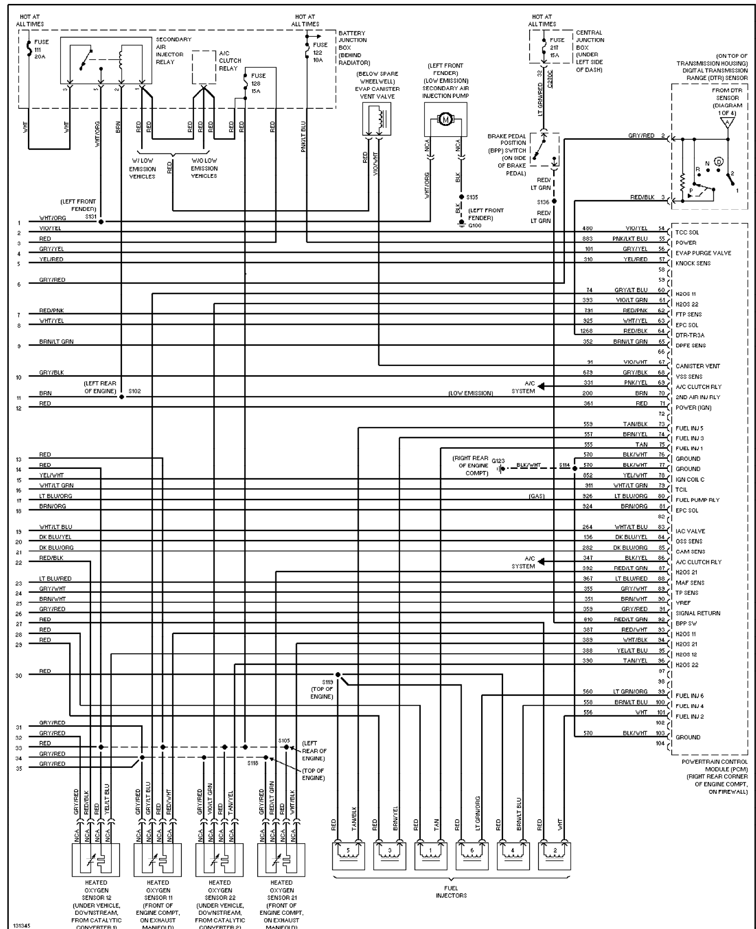
Fig. 16: 3.0L 12-Valve, Engine Performance Circuits (4 of 4)
