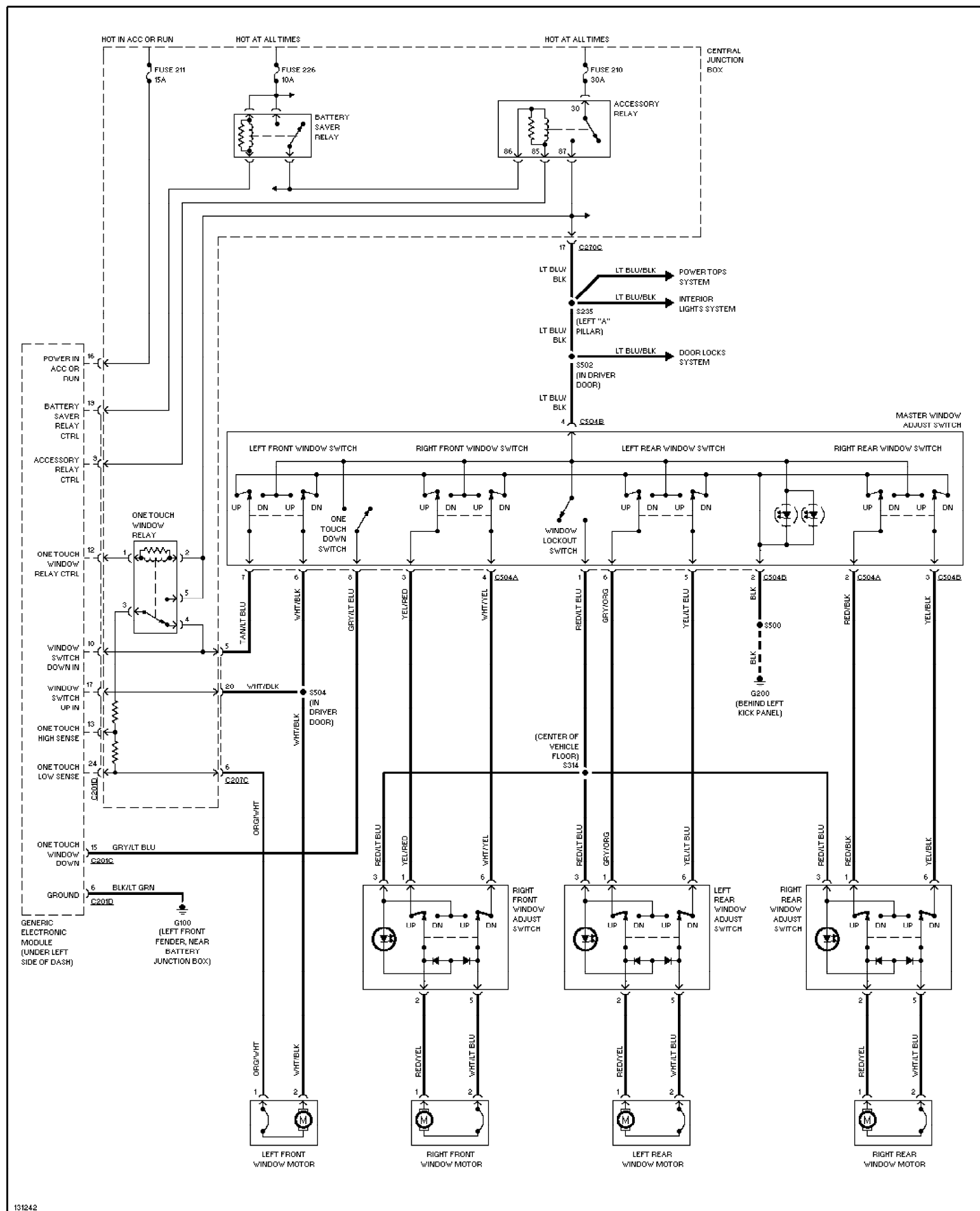
Fig. 49: Power Window Circuit 2000 Ford Taurus SES
