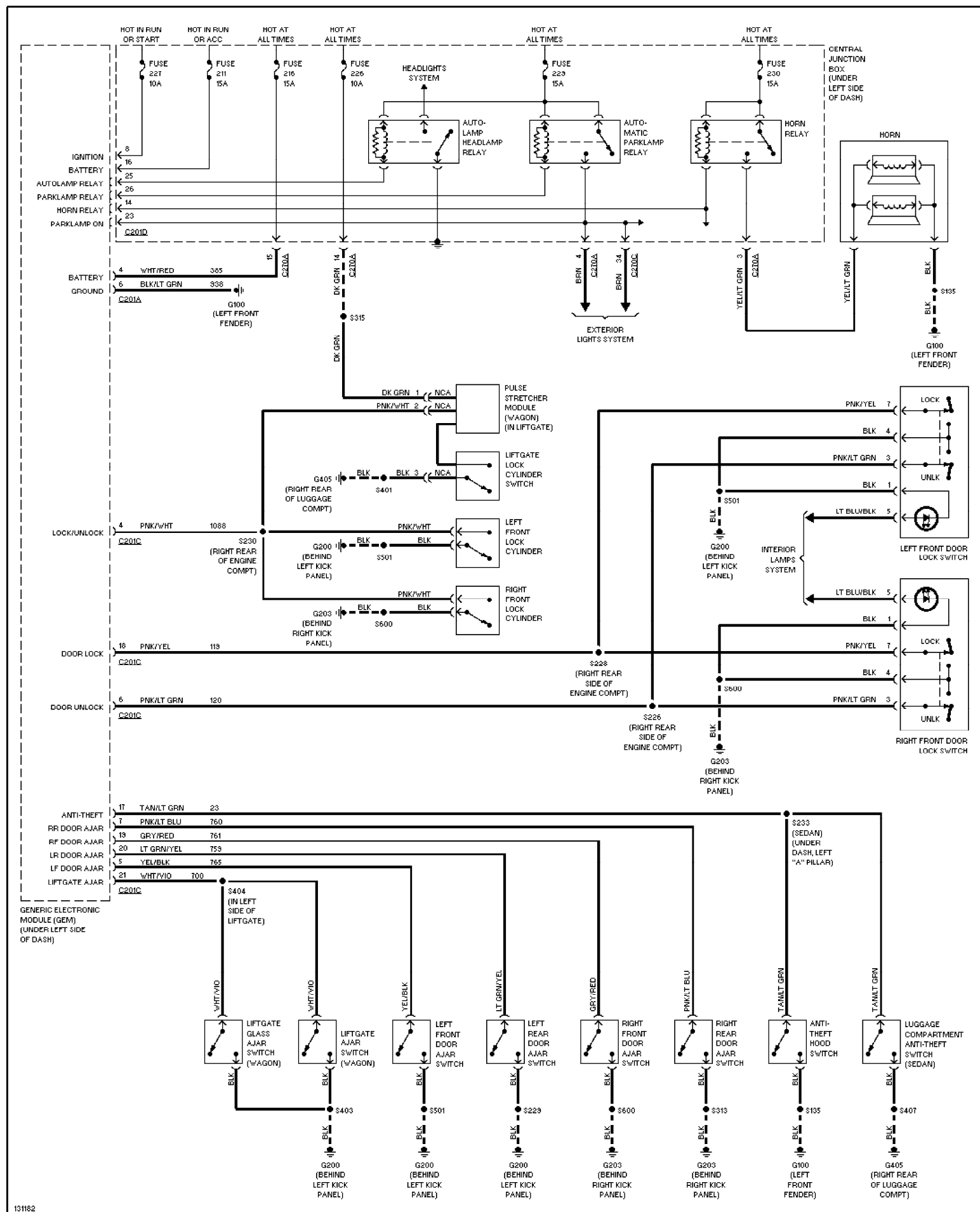
Fig. 6: Forced Entry Circuit 2000 Ford Taurus SES
