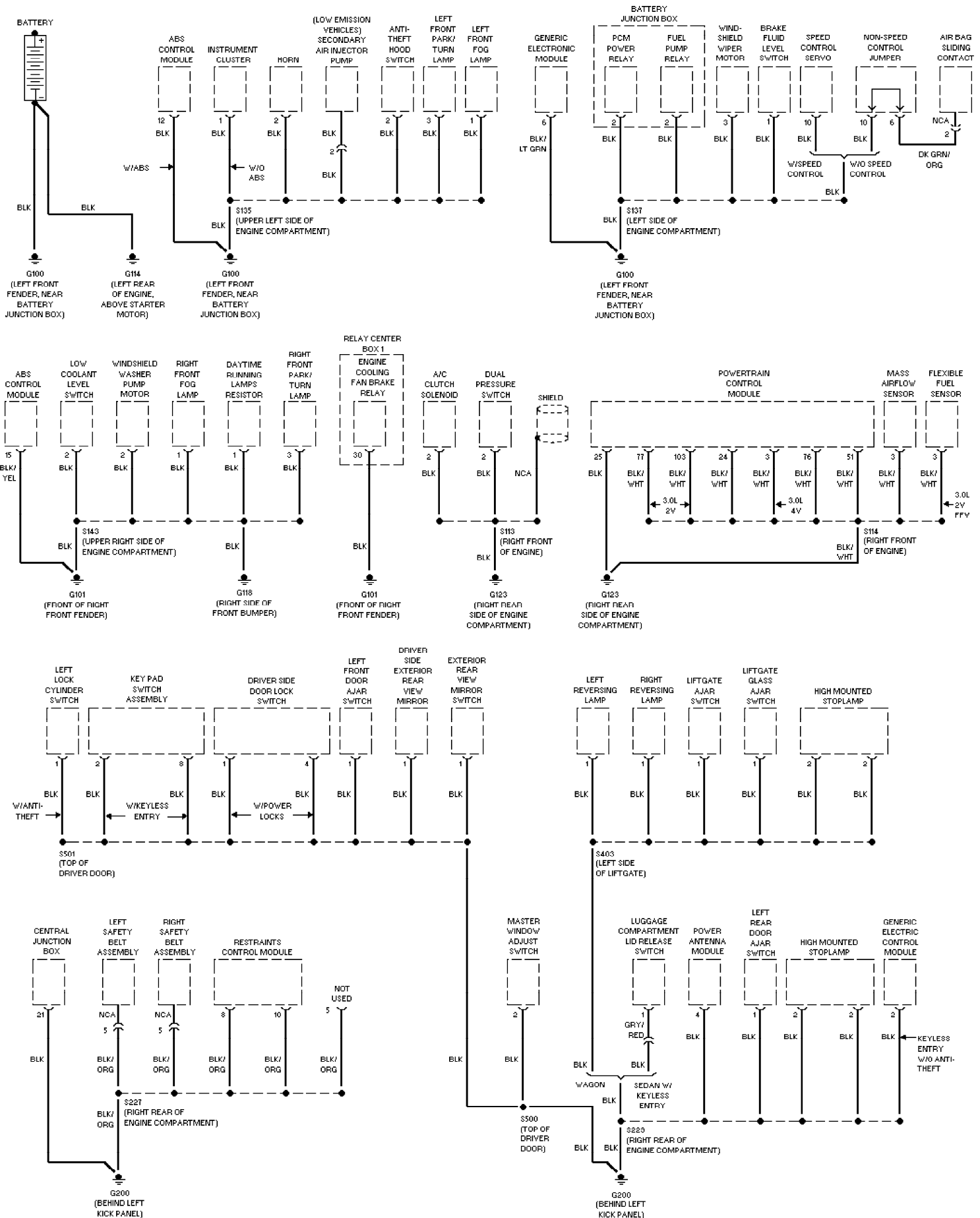
Fig. 28: Ground Distribution Circuit (1 of 3) 2000 Ford Taurus SES
