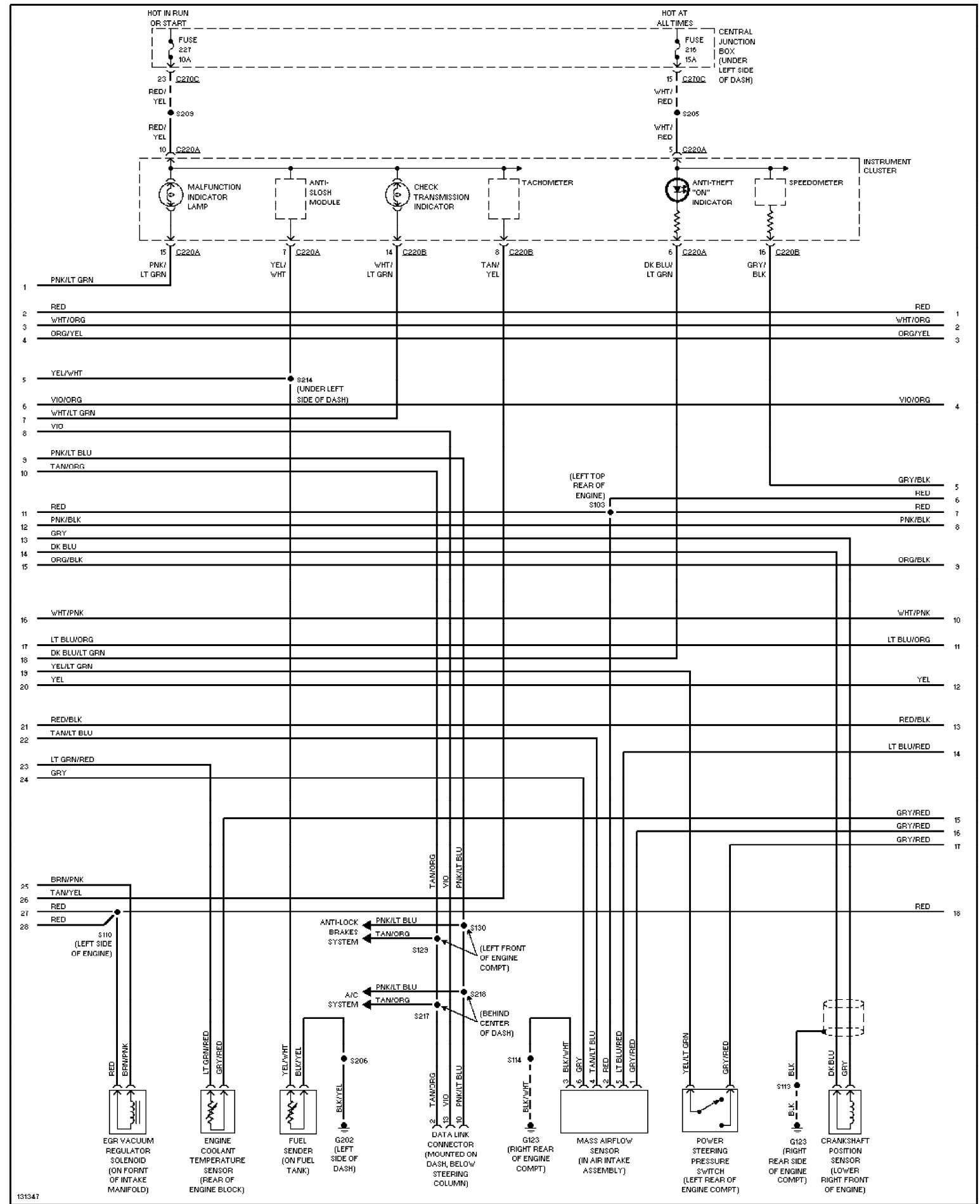
Fig. 18: 3.0L 24-Valve, Engine Performance Circuits (2 of 4) 2000 Ford Taurus SES
