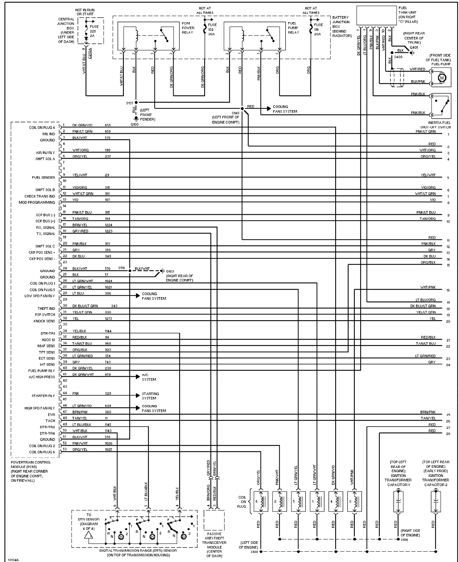
Fig. 17: 3.0L 24-Valve, Engine Performance Circuits (1 of 4)
