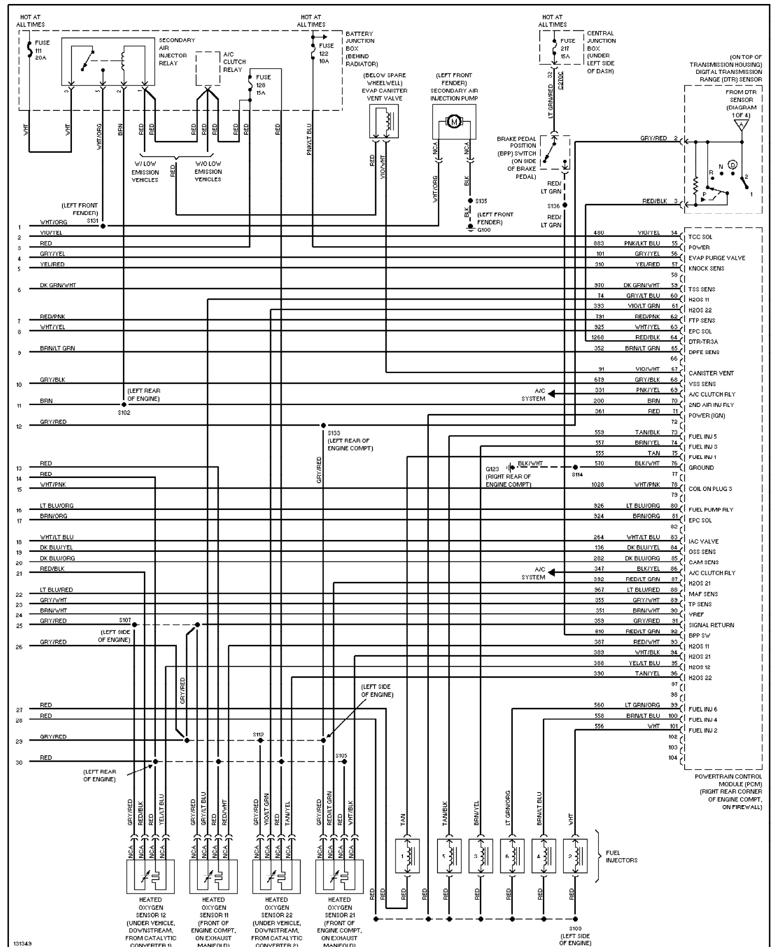
Fig. 20: 3.0L 24-Valve, Engine Performance Circuits (4 of 4) 2000 Ford Taurus SES
