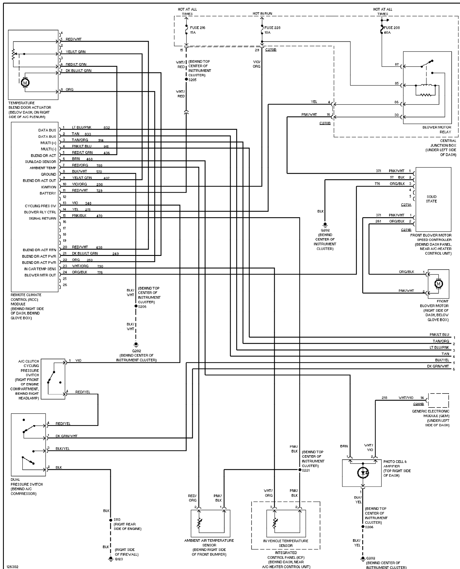
Fig. 1: Automatic A/C Circuit (1 of 2) 2000 Ford Taurus SES
