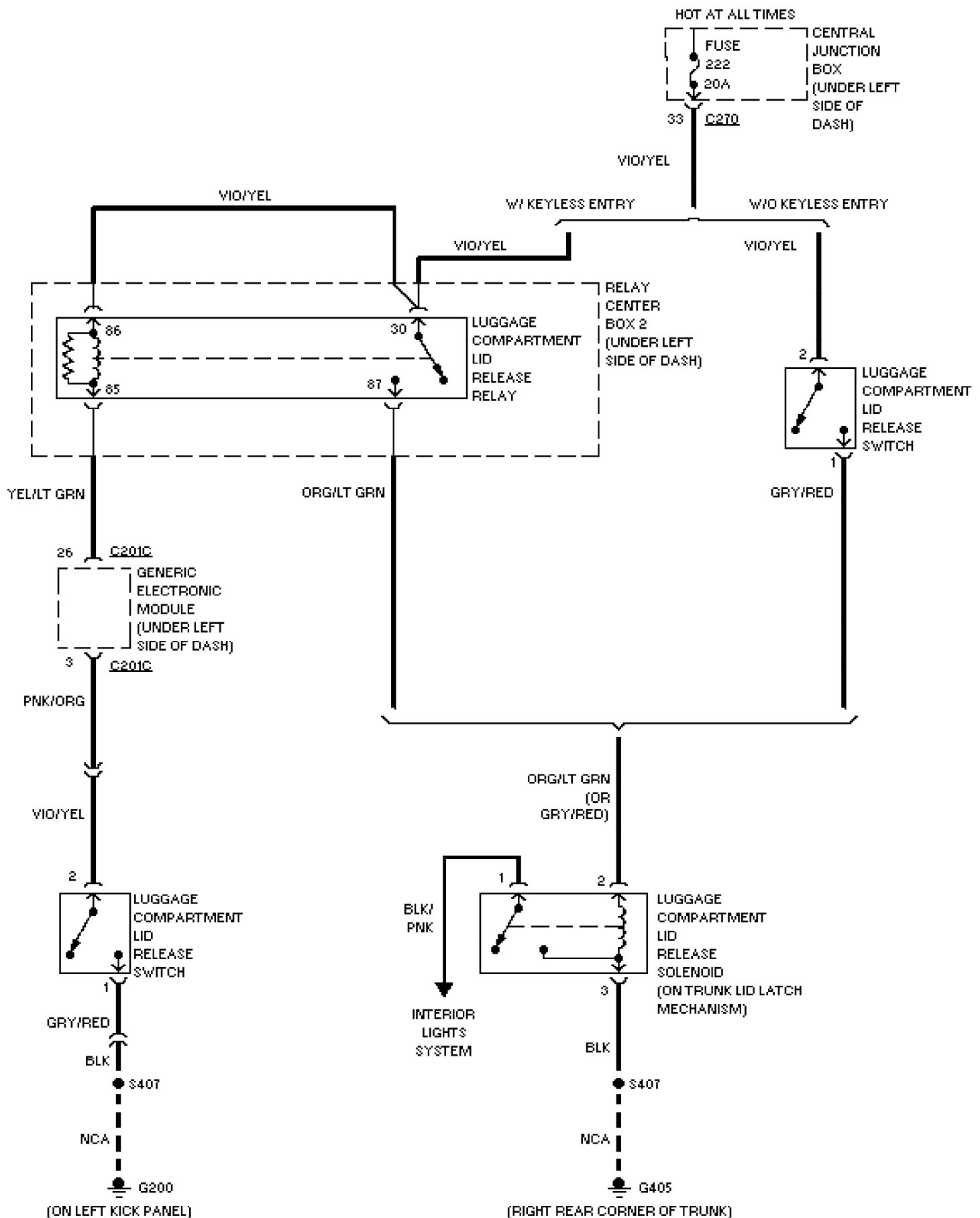
Fig. 58: Trunk Release Circuit 2000 Ford Taurus SES
