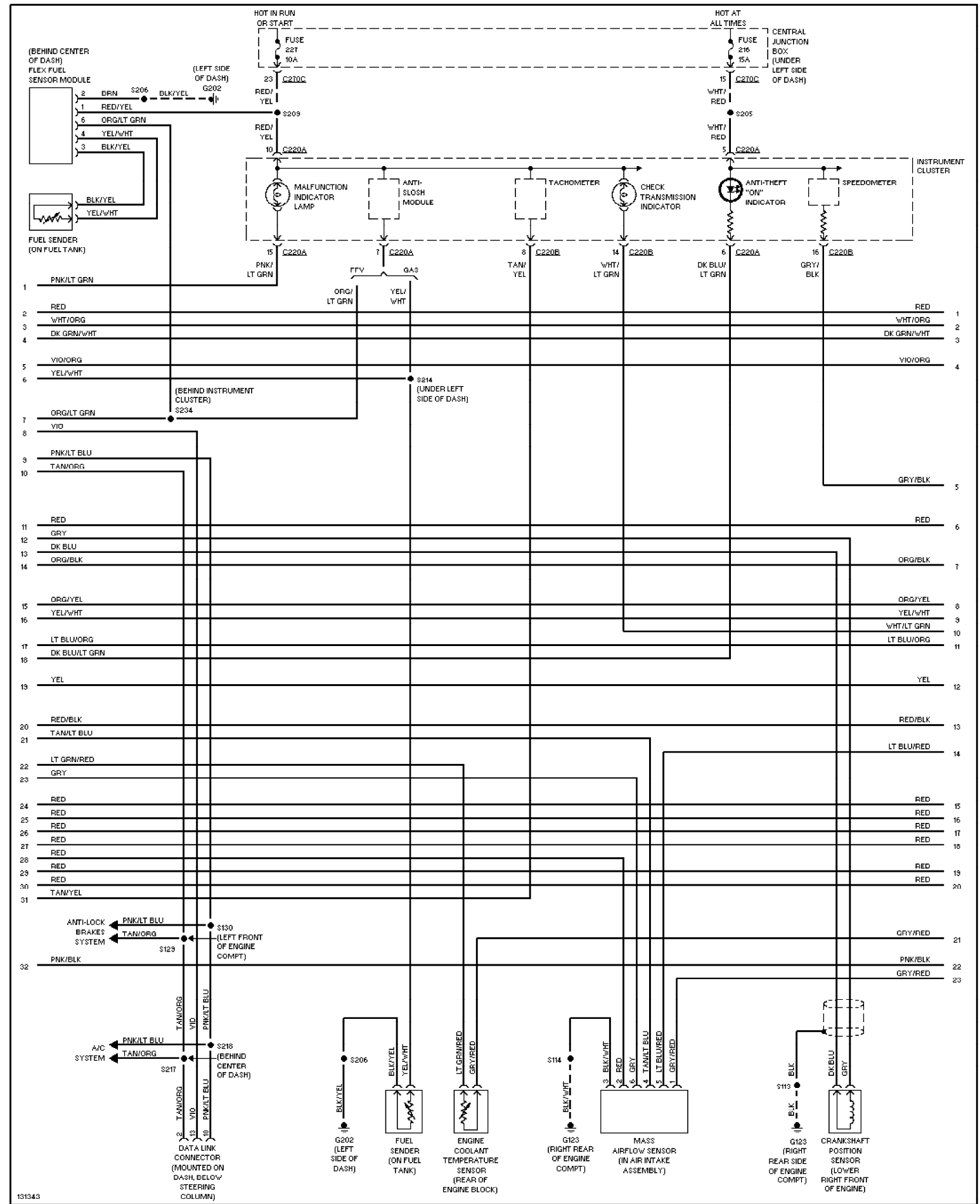
Fig. 22: 3.0L Flex Fuel, Engine Performance Circuits (2 of 4) 2000 Ford Taurus SES
