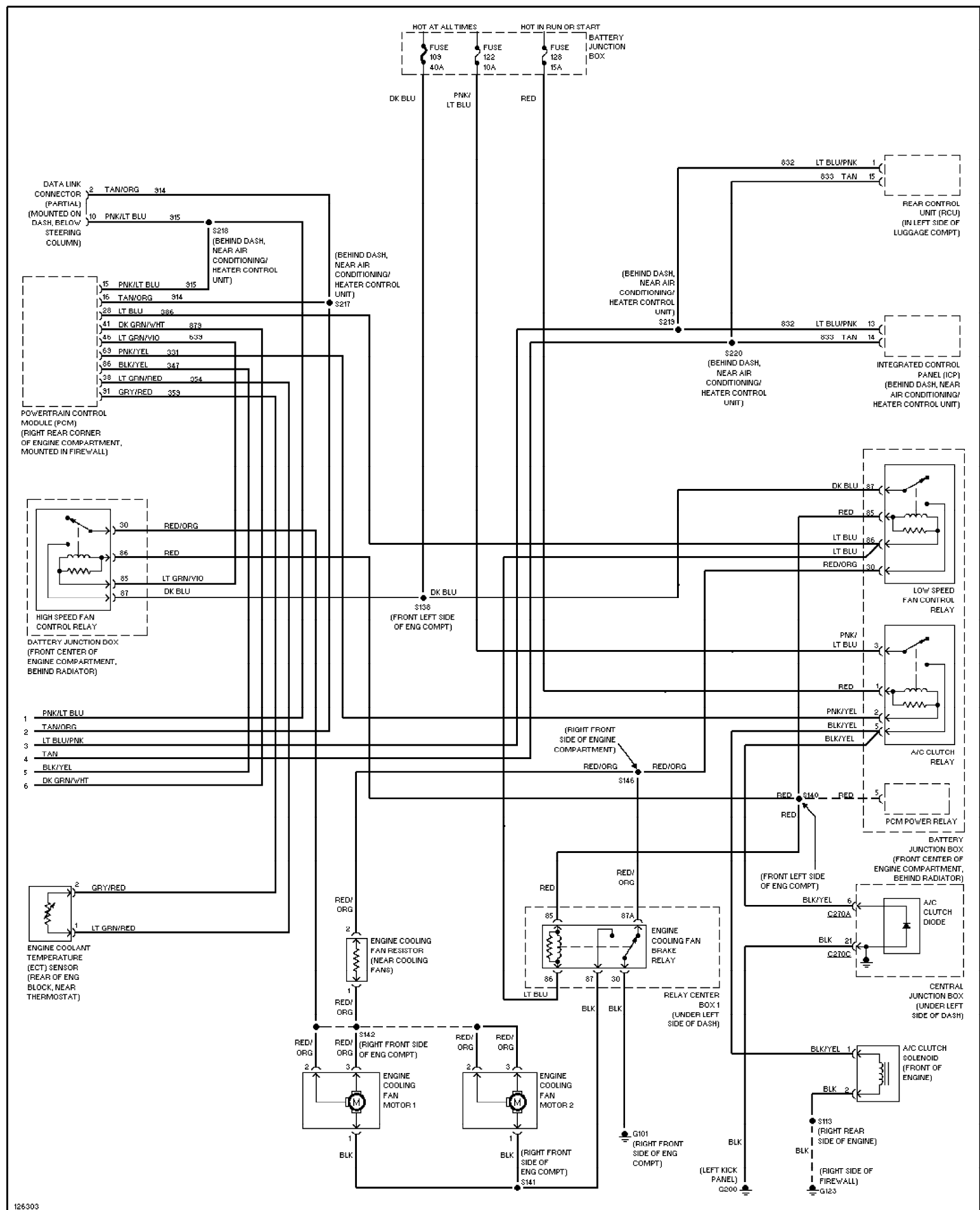
Fig. 2: Automatic A/C Circuit (2 of 2) 2000 Ford Taurus SES
