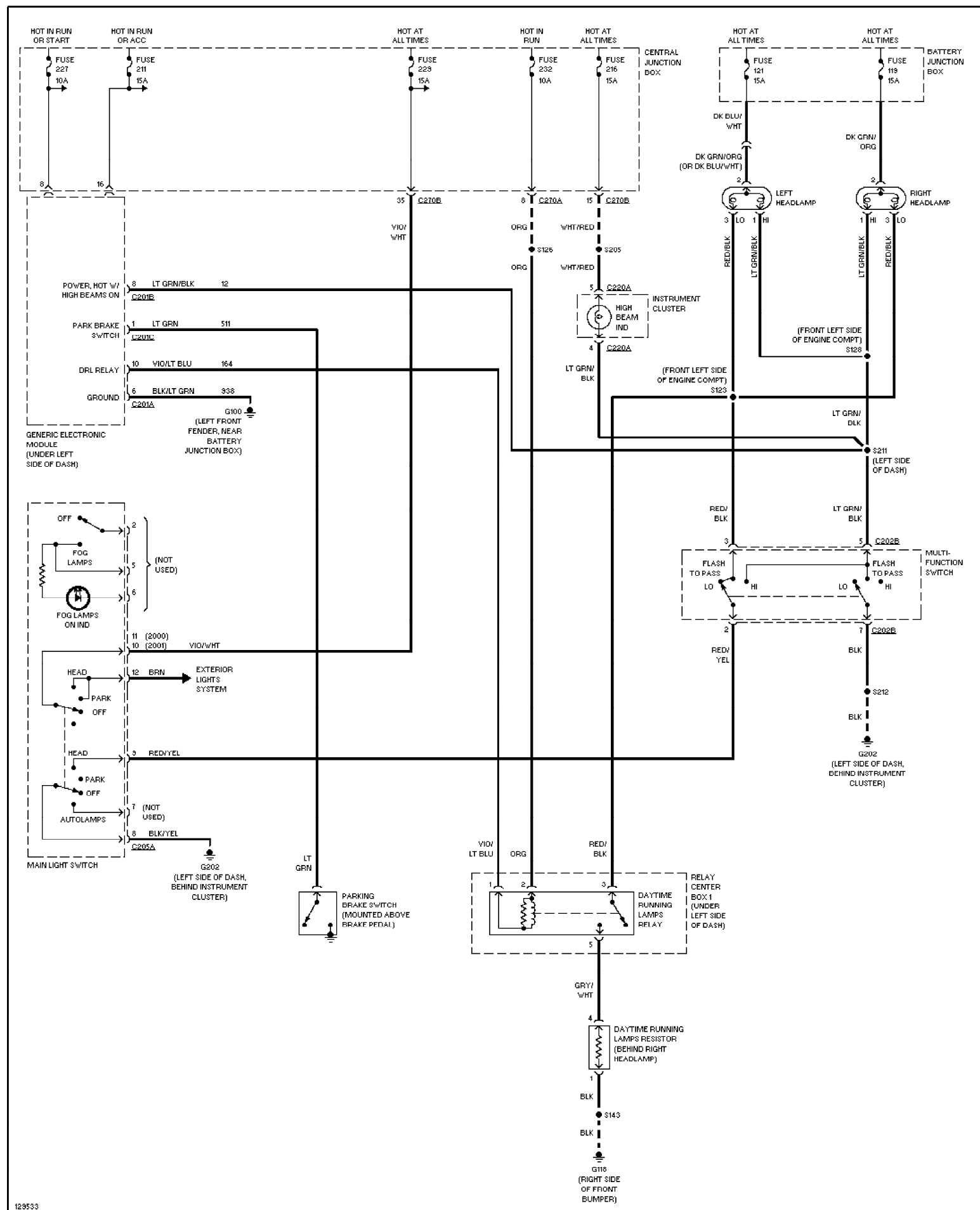
Fig. 33: Headlamps Circuit, W/ DRL 2000 Ford Taurus SES
