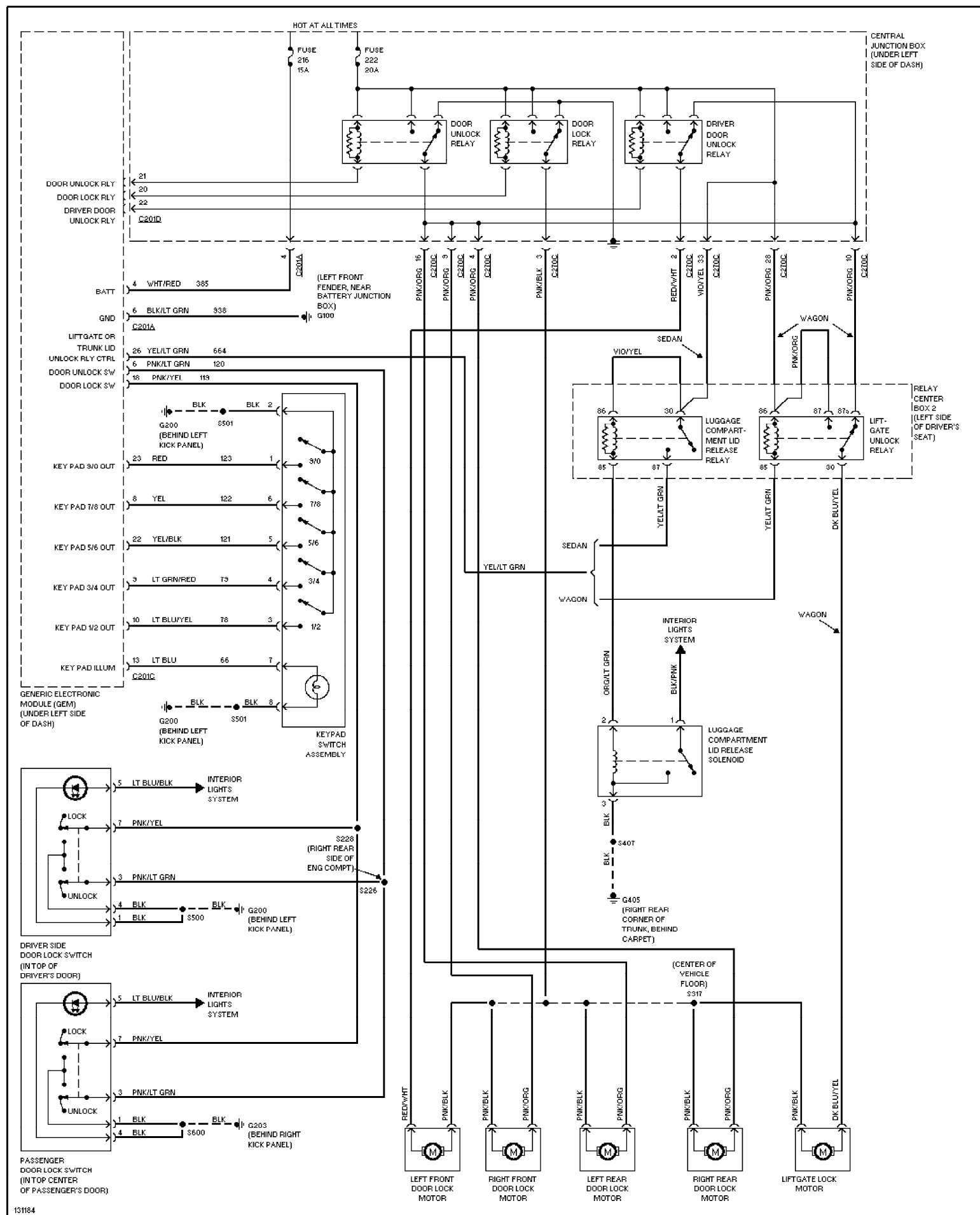
Fig. 43: Power Door Lock Circuit, W/ Keyless Entry 2000 Ford Taurus SES
