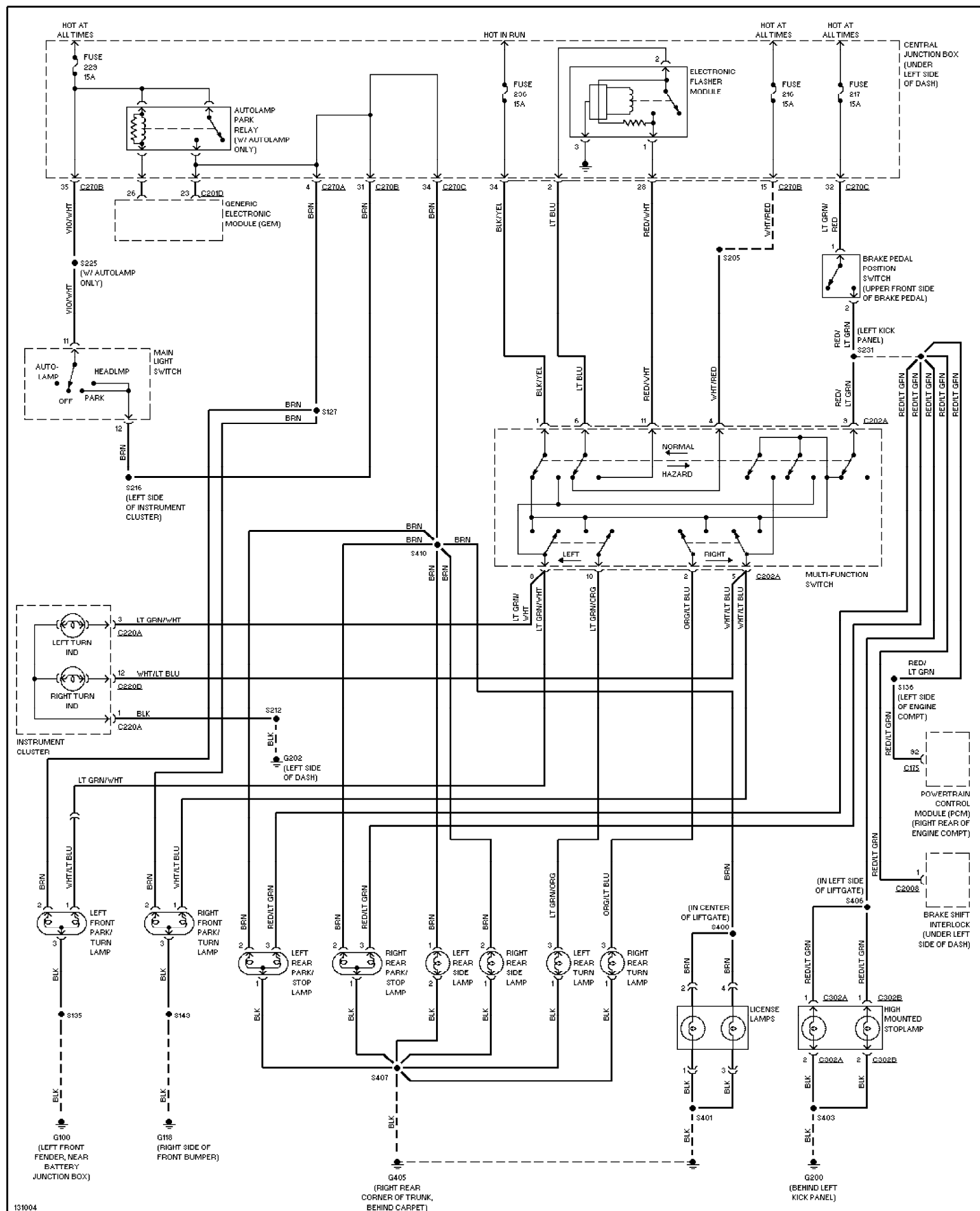
Fig. 27: Exterior Lamps Circuit, Wagon 2000 Ford Taurus SES
