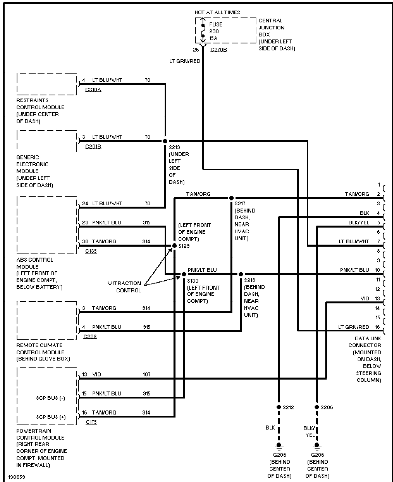
Fig. 9: Computer Data Lines 2000 Ford Taurus SES
