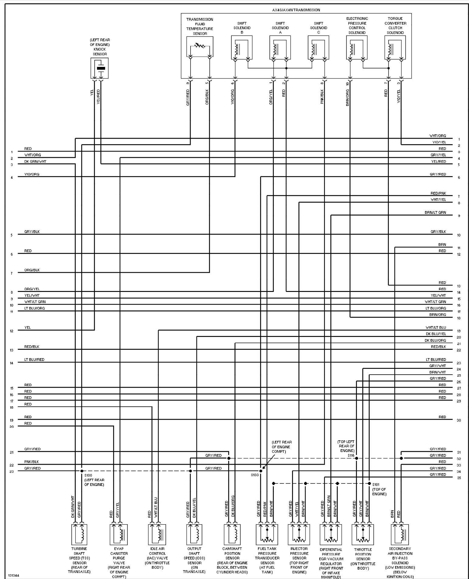
Fig. 23: 3.0L Flex Fuel, Engine Performance Circuits (3 of 4)
