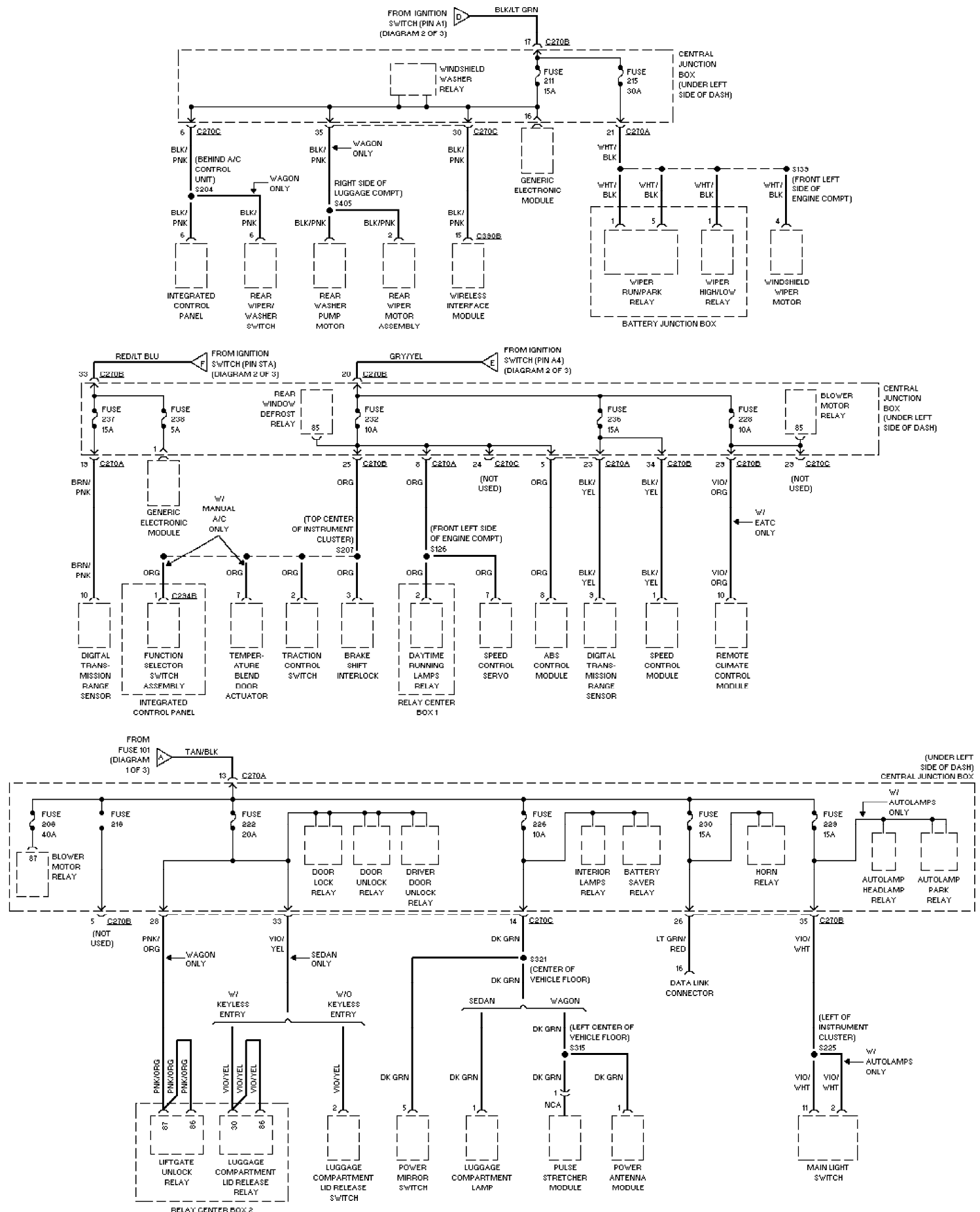
Fig. 42: Power Distribution Circuit (3 of 3) 2000 Ford Taurus SES
