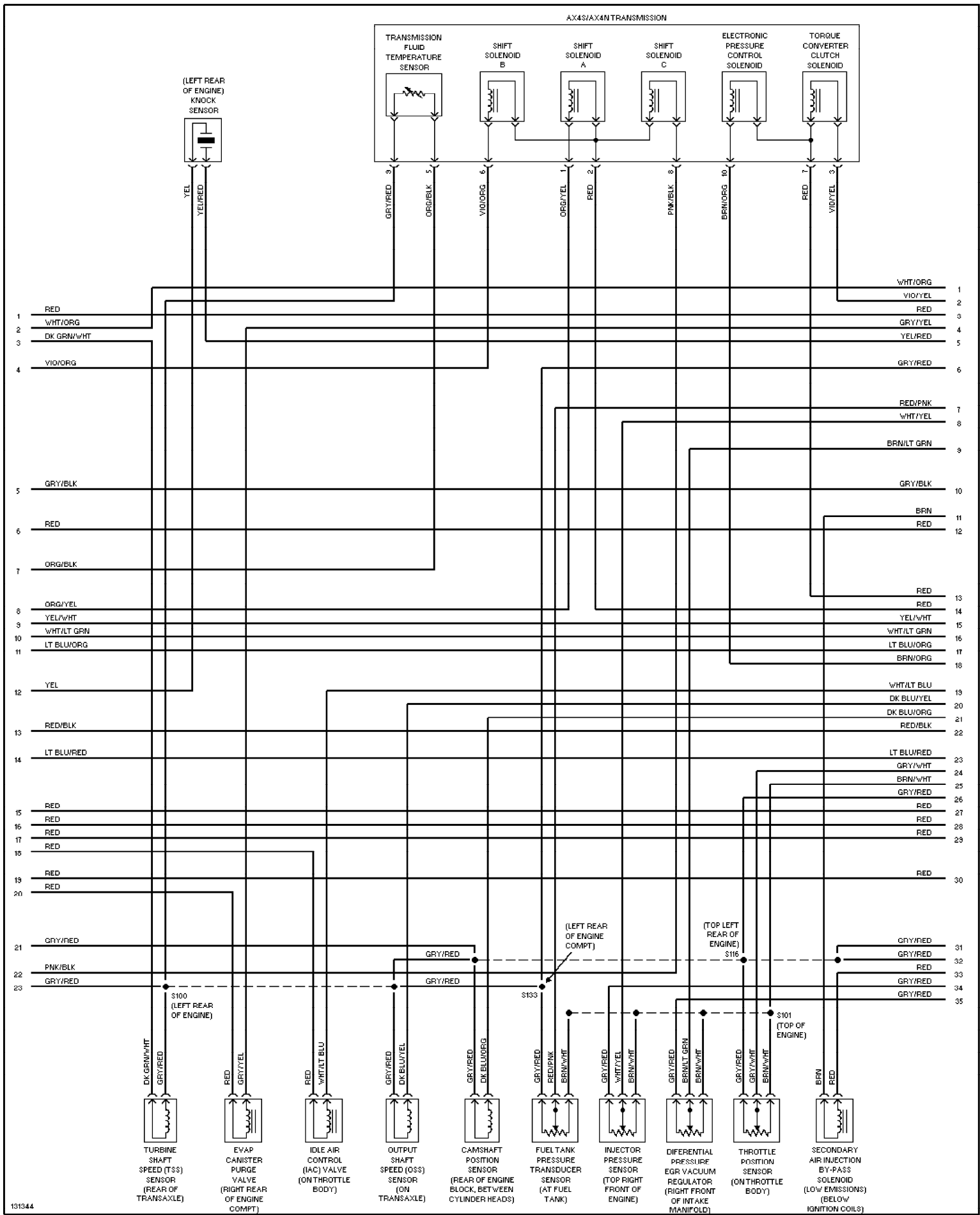
Fig. 15: 3.0L 12-Valve, Engine Performance Circuits (3 of 4)
