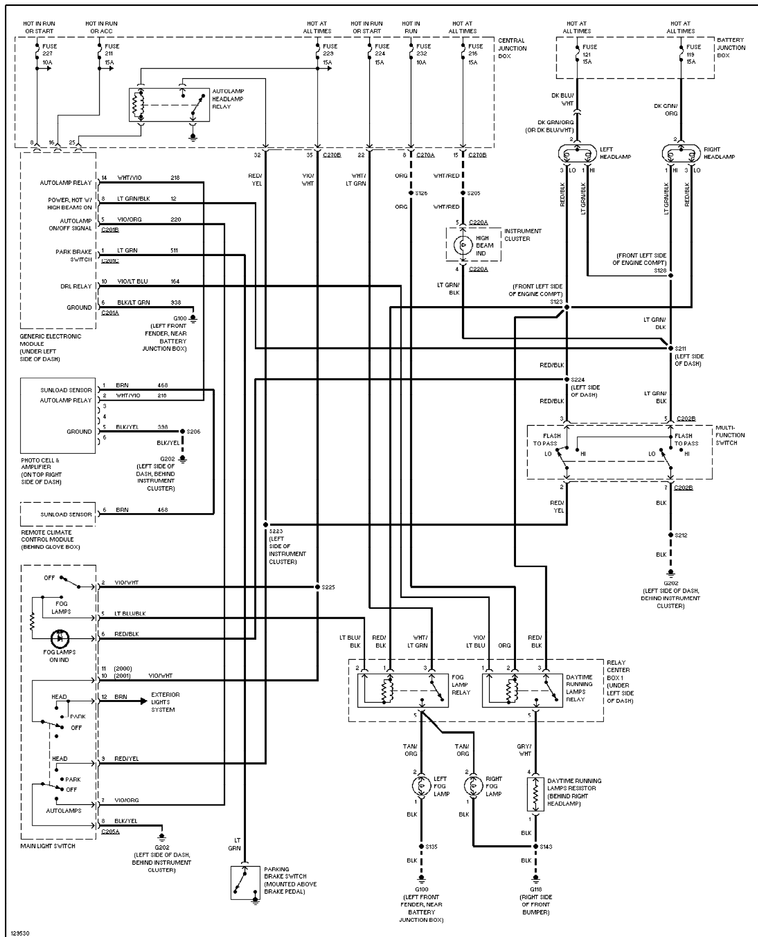
Fig. 31: Autolamps Circuit, W/ DRL 2000 Ford Taurus SES
