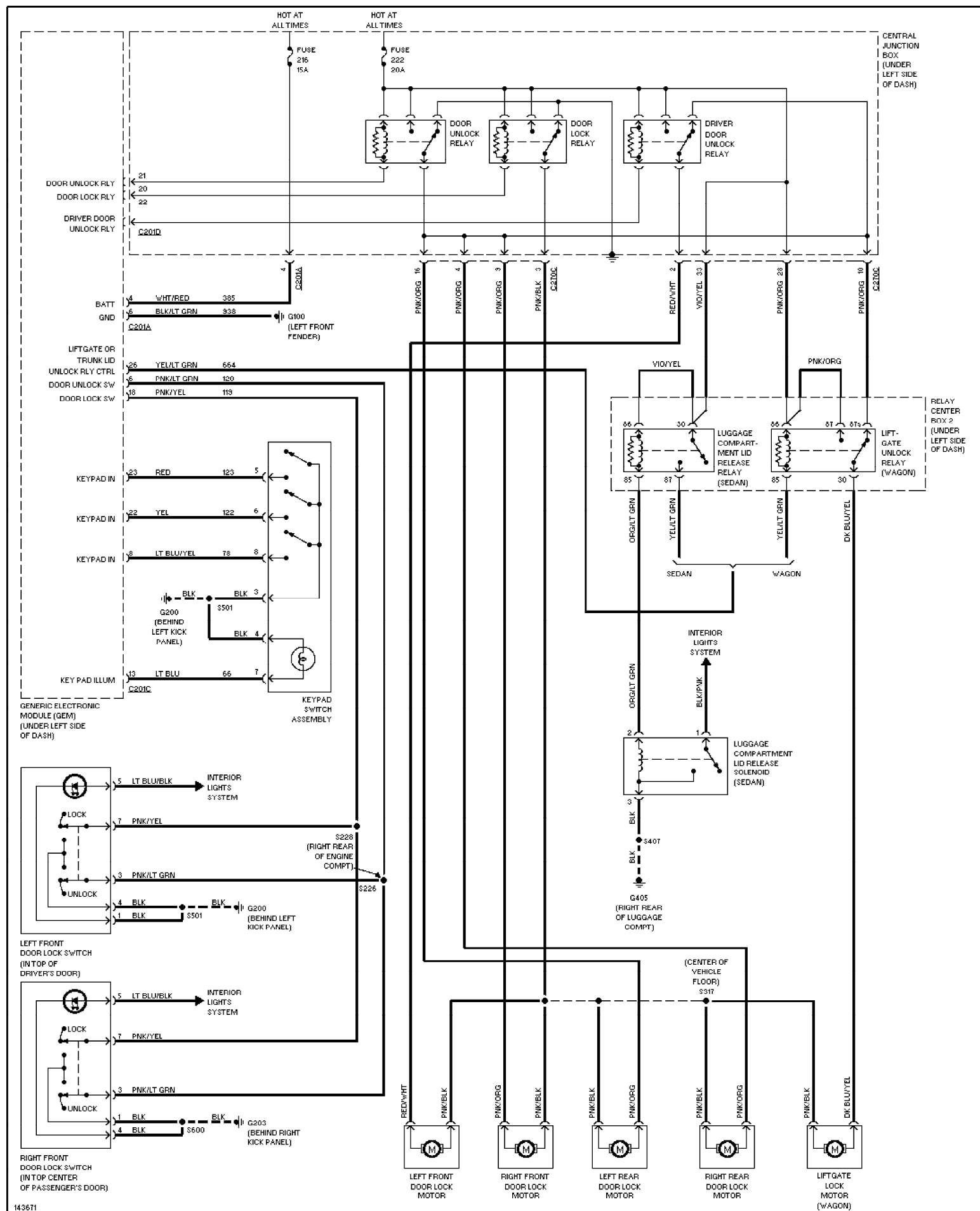
Fig. 43: Power Door Lock Circuit, W/ Keyless Entry 2001 Ford Taurus SEL
