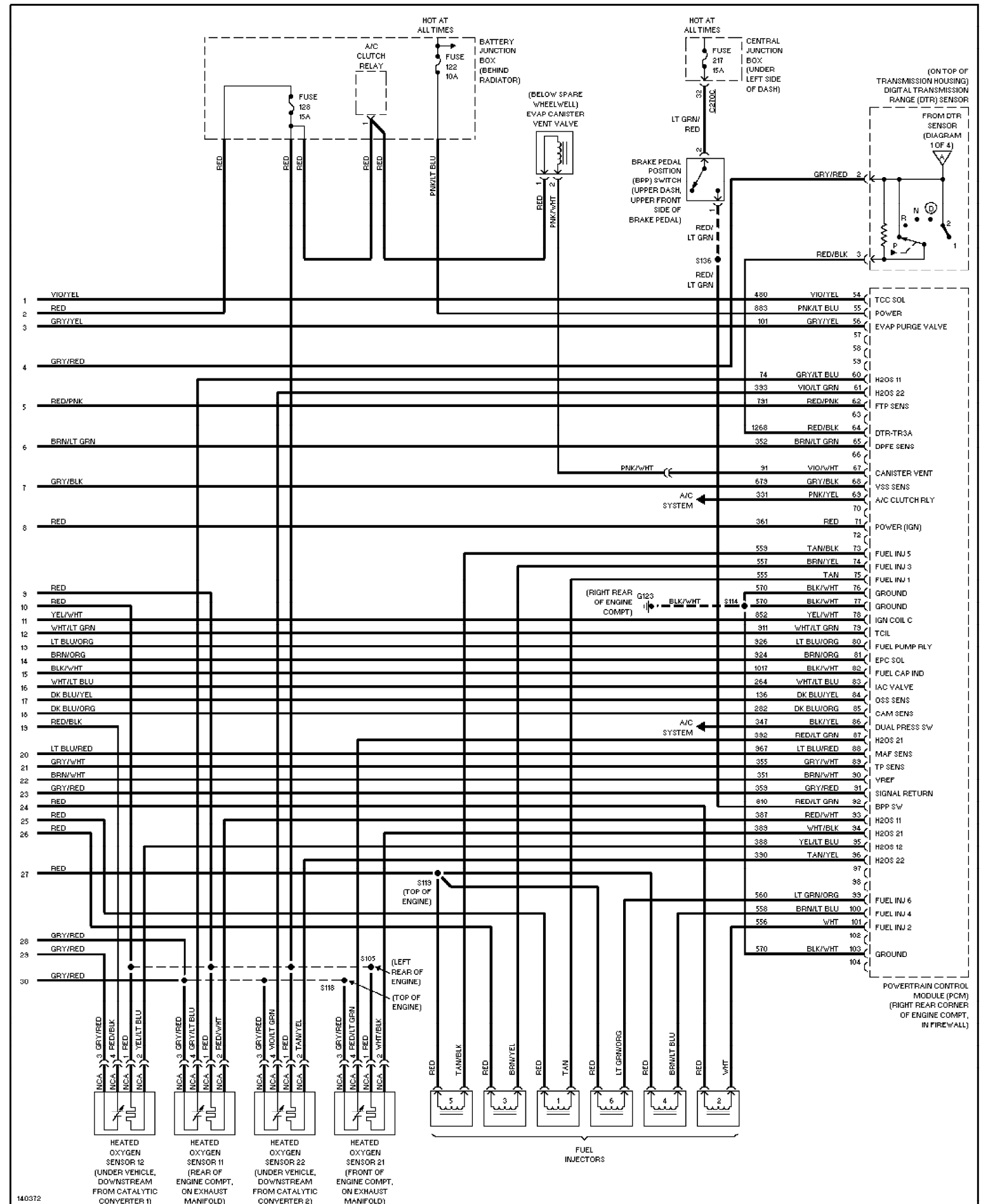
Fig. 24: 3.0L Flex Fuel, Engine Performance Circuits (4 of 4) 2001 Ford Taurus SEL
