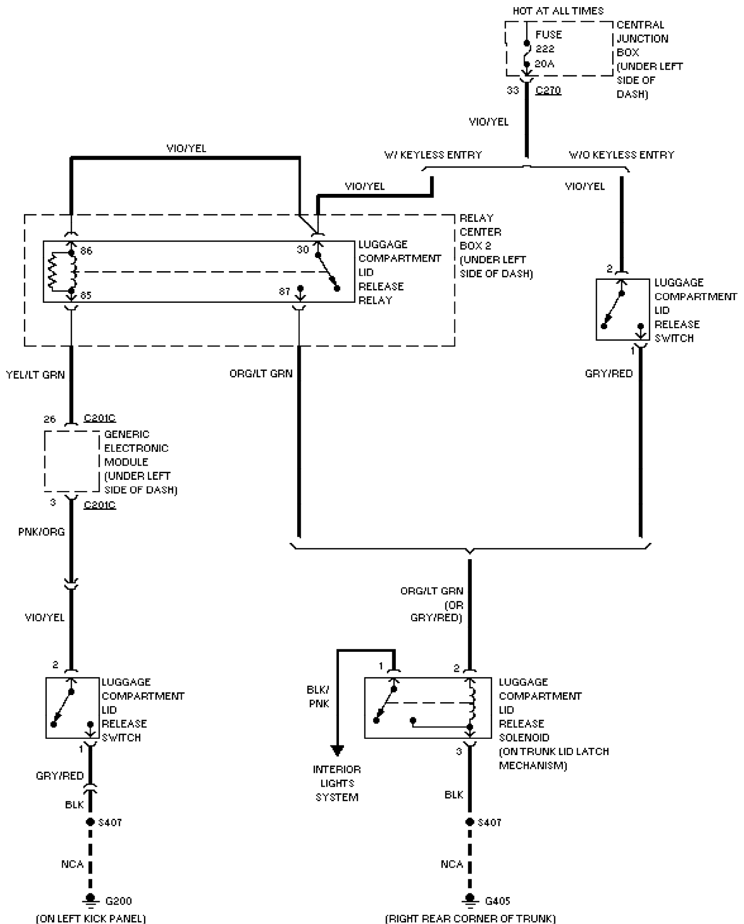
Fig. 58: Trunk Release Circuit 2001 Ford Taurus SEL
