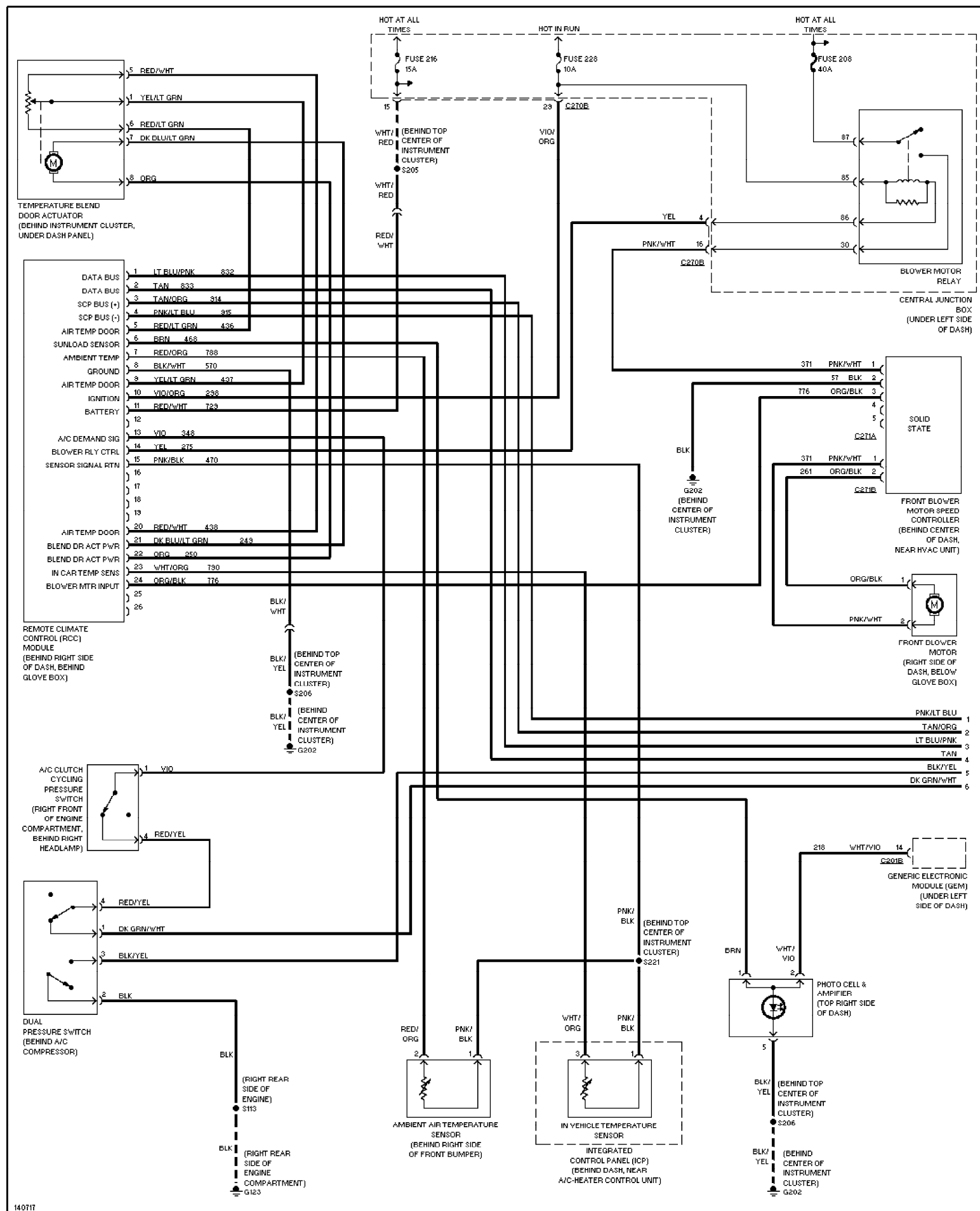
Fig. 1: Automatic A/C Circuit (1 of 2) 2001 Ford Taurus SEL
