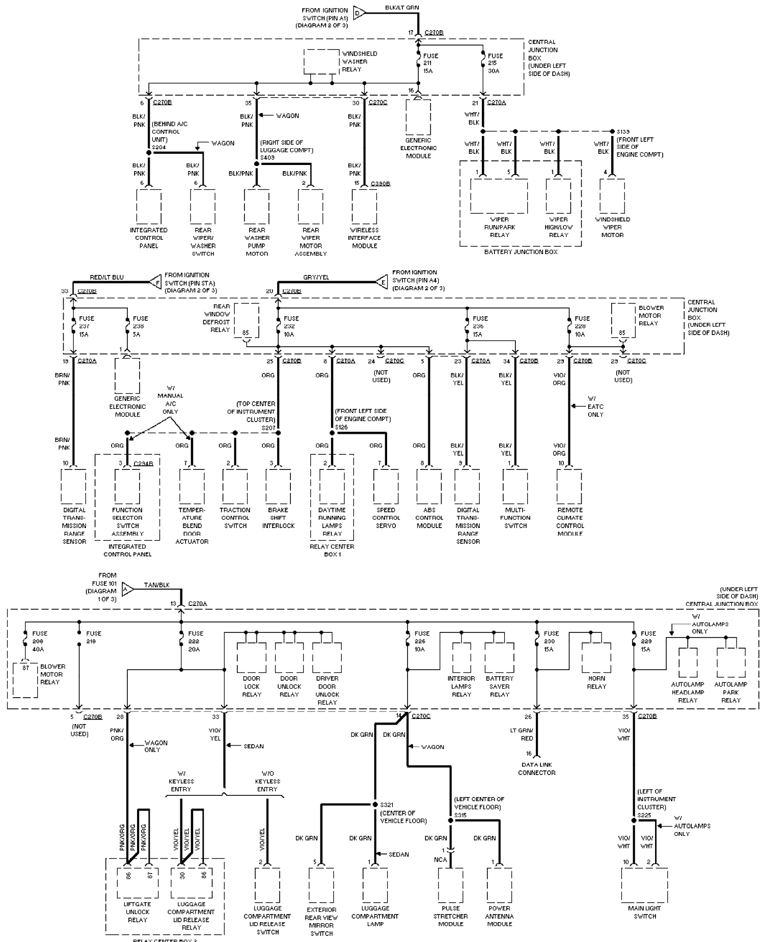
Fig. 42: Power Distribution Circuit (3 of 3) 2001 Ford Taurus SEL
