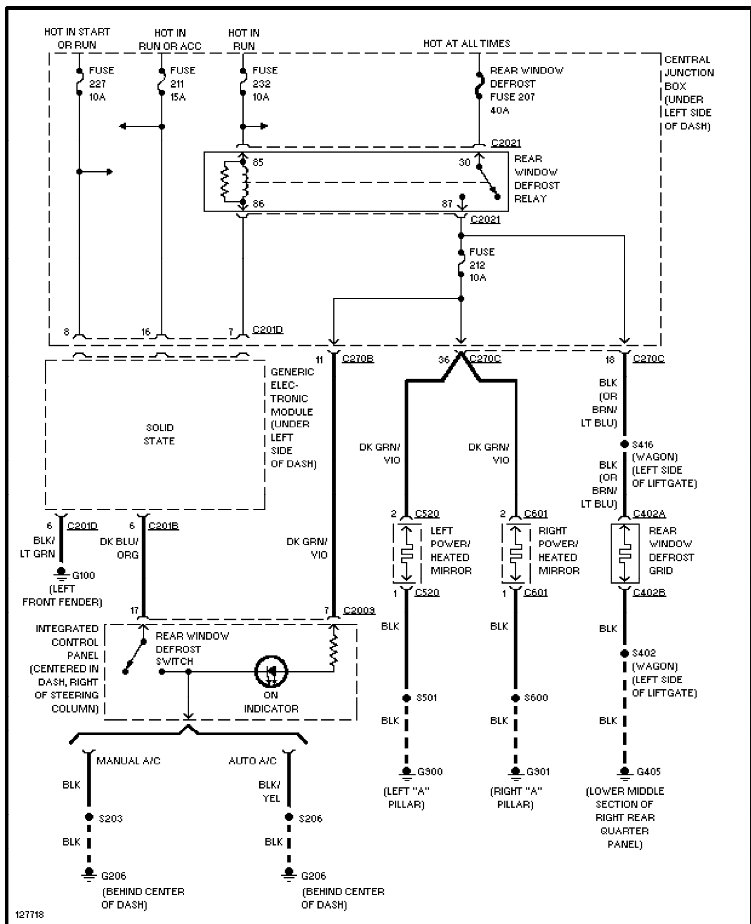
Fig. 12: Defogger Circuit 2001 Ford Taurus SEL
