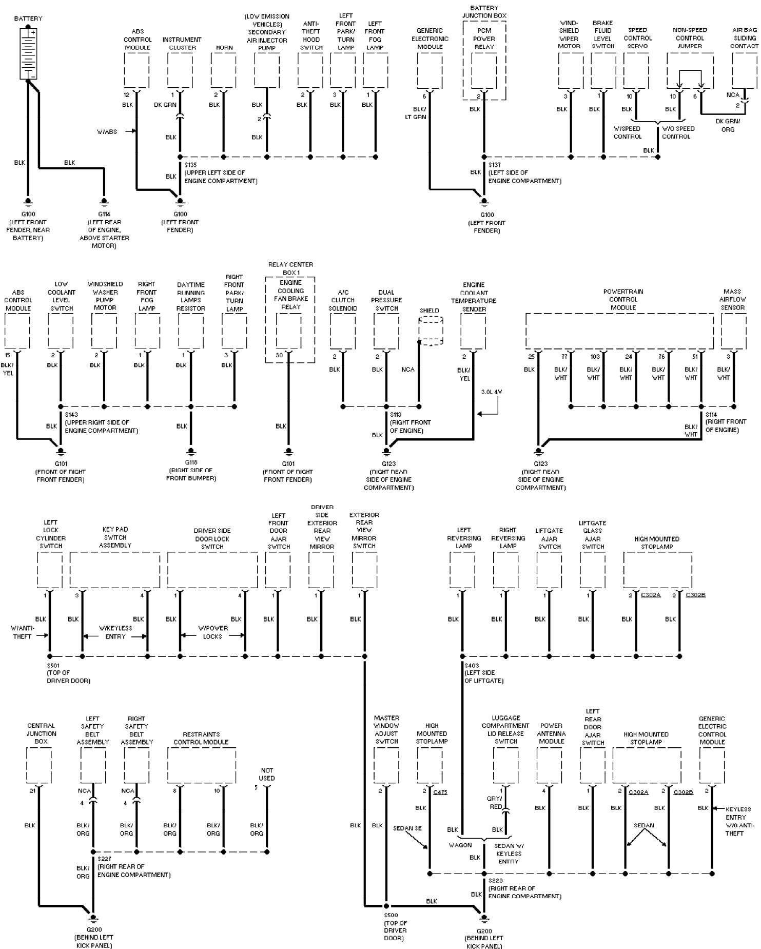
Fig. 28: Ground Distribution Circuit (1 of 3) 2001 Ford Taurus SEL
