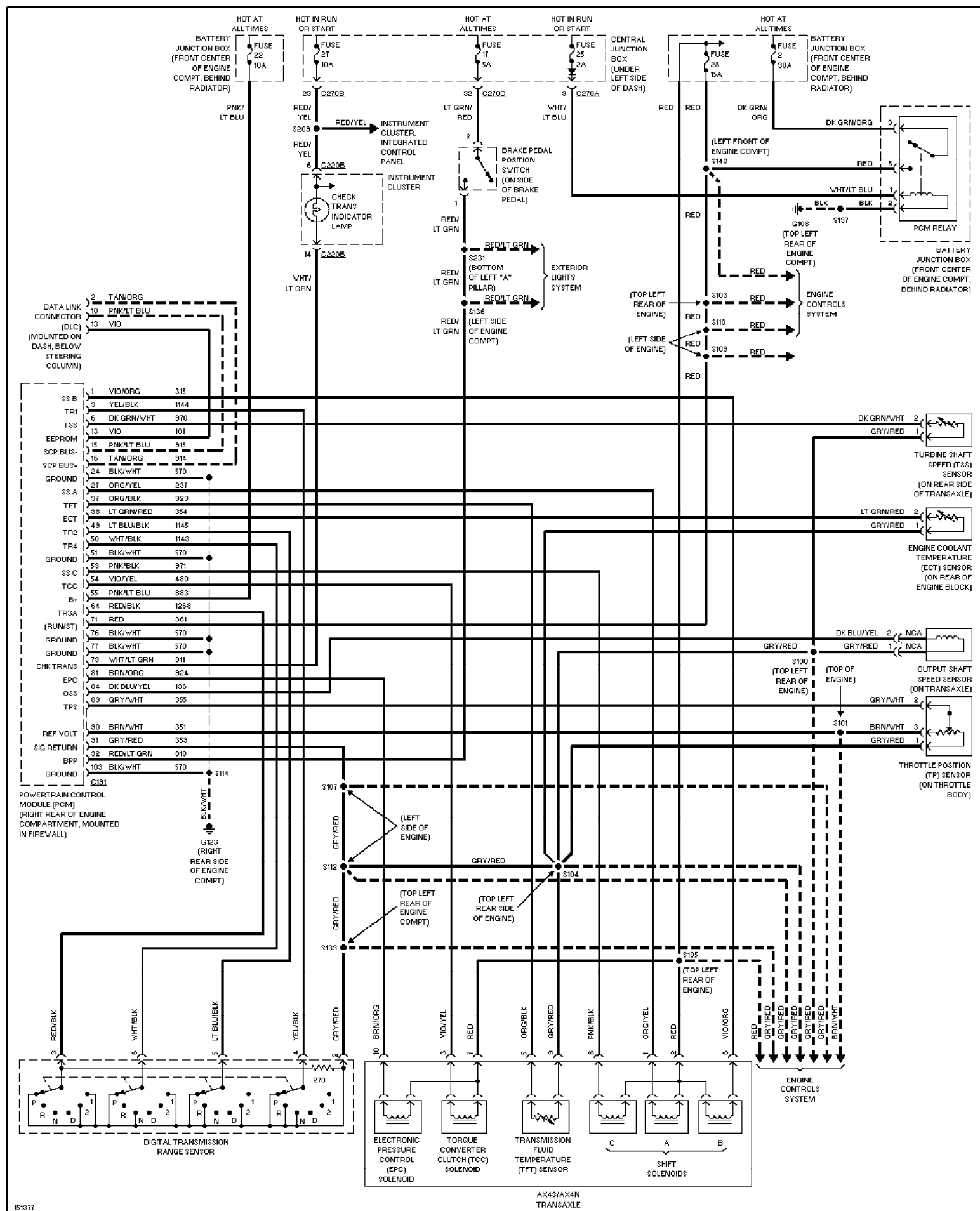
Fig. 56: 3.0L 24-Valve, A/T Circuit 2001 Ford Taurus SEL
