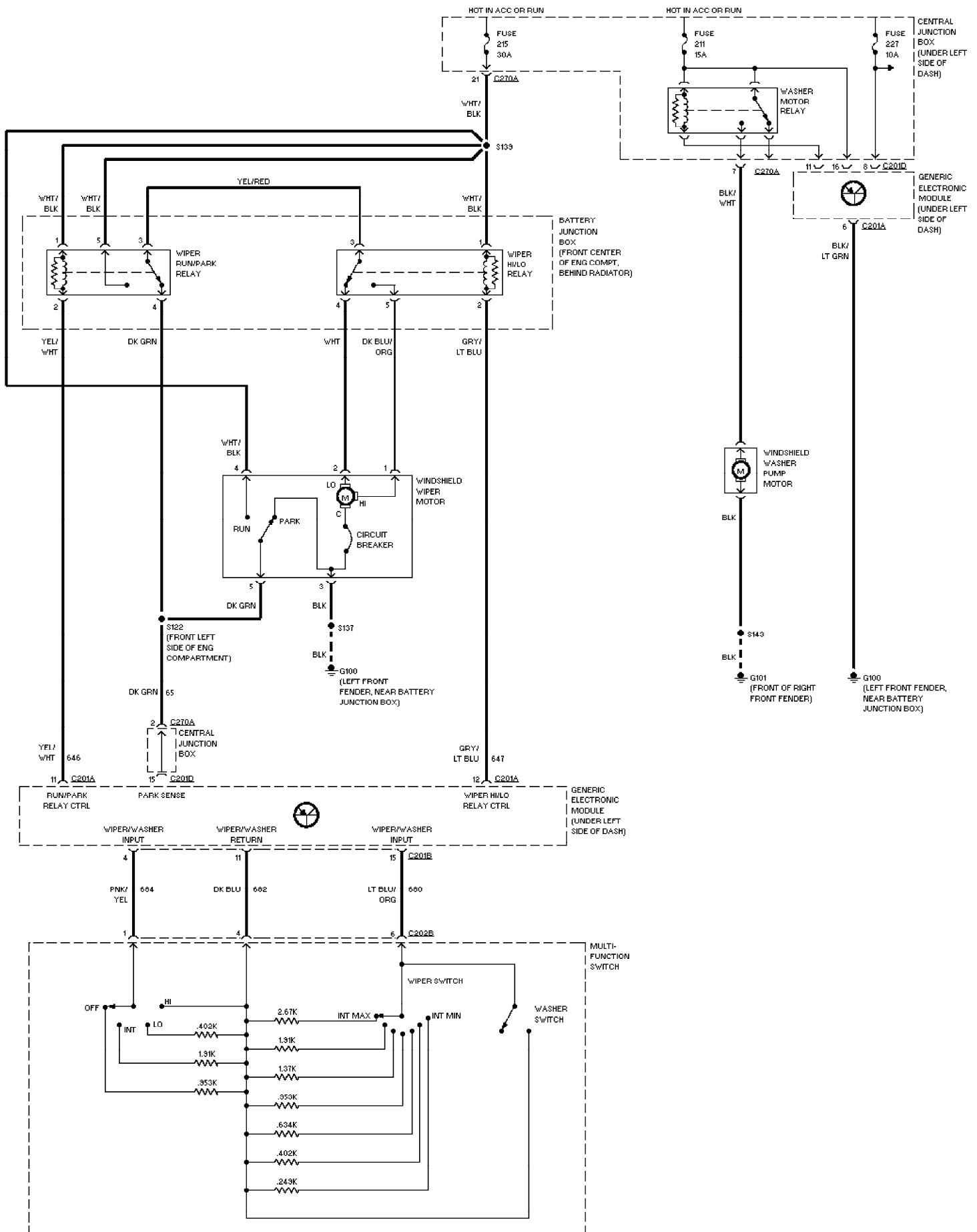
Fig. 60: Front Washer/Wiper Circuit 2001 Ford Taurus SEL
