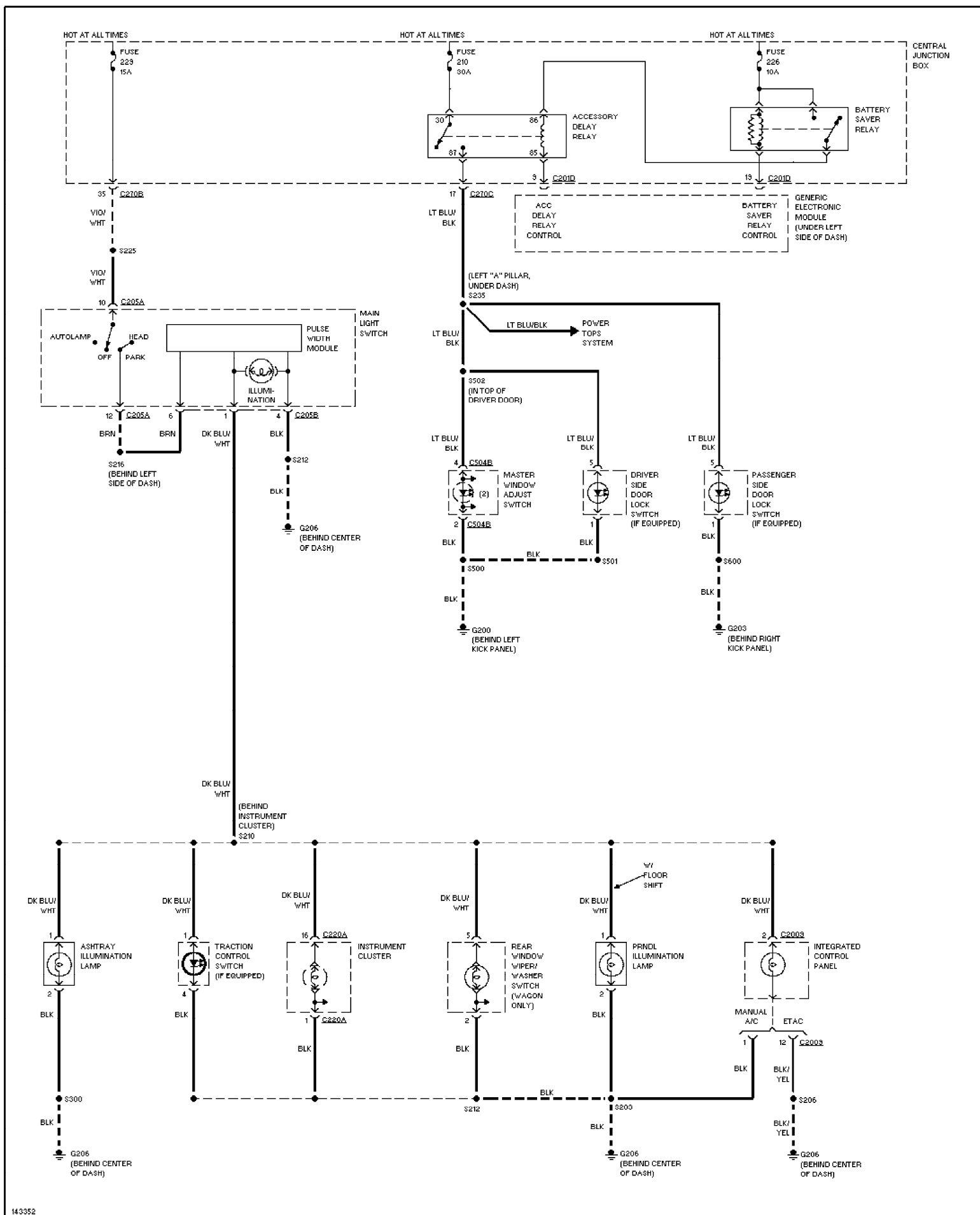
Fig. 38: Instrument Illumination Circuit 2001 Ford Taurus SEL
