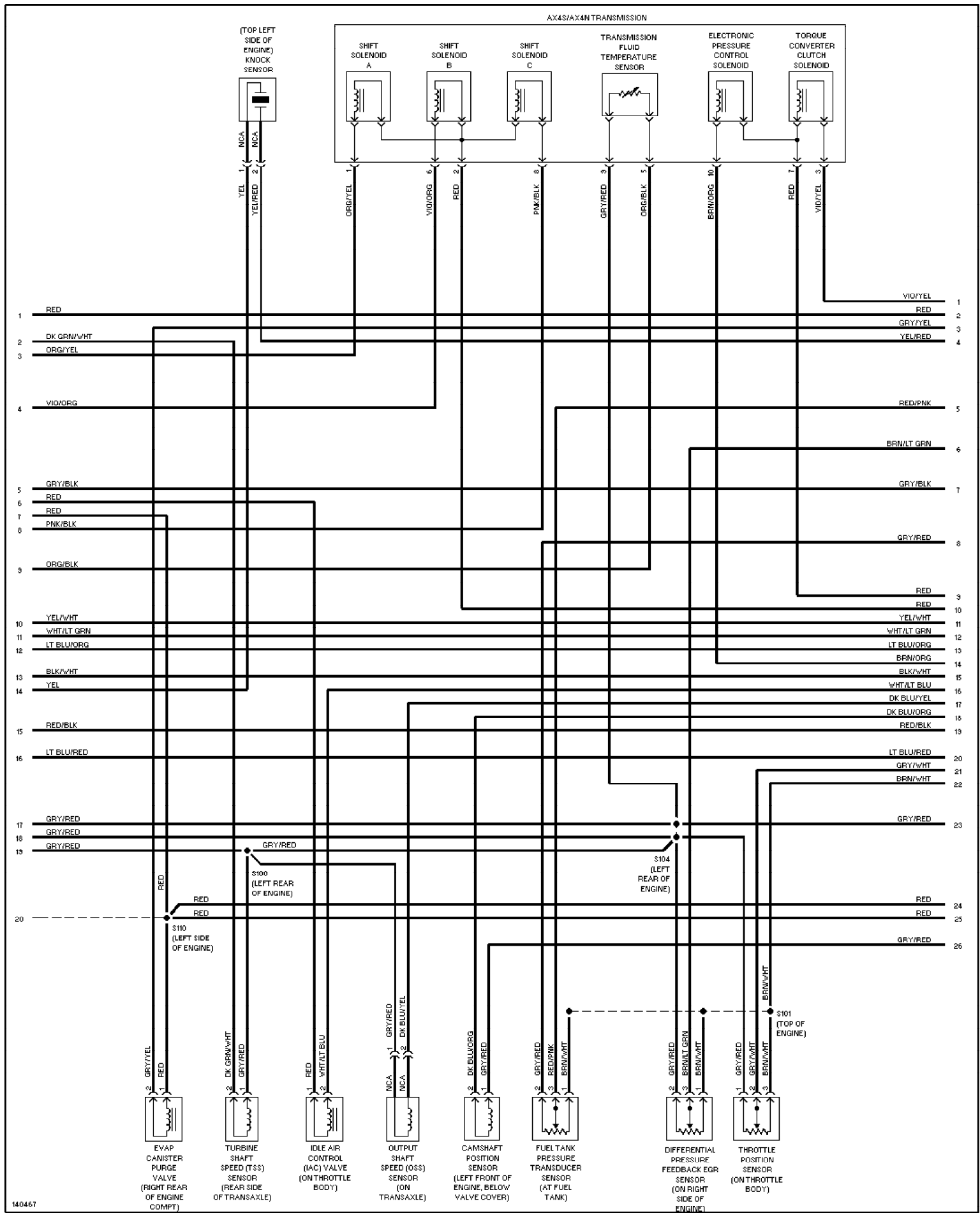
Fig. 19: 3.0L 24-Valve, Engine Performance Circuits (3 of 4)
