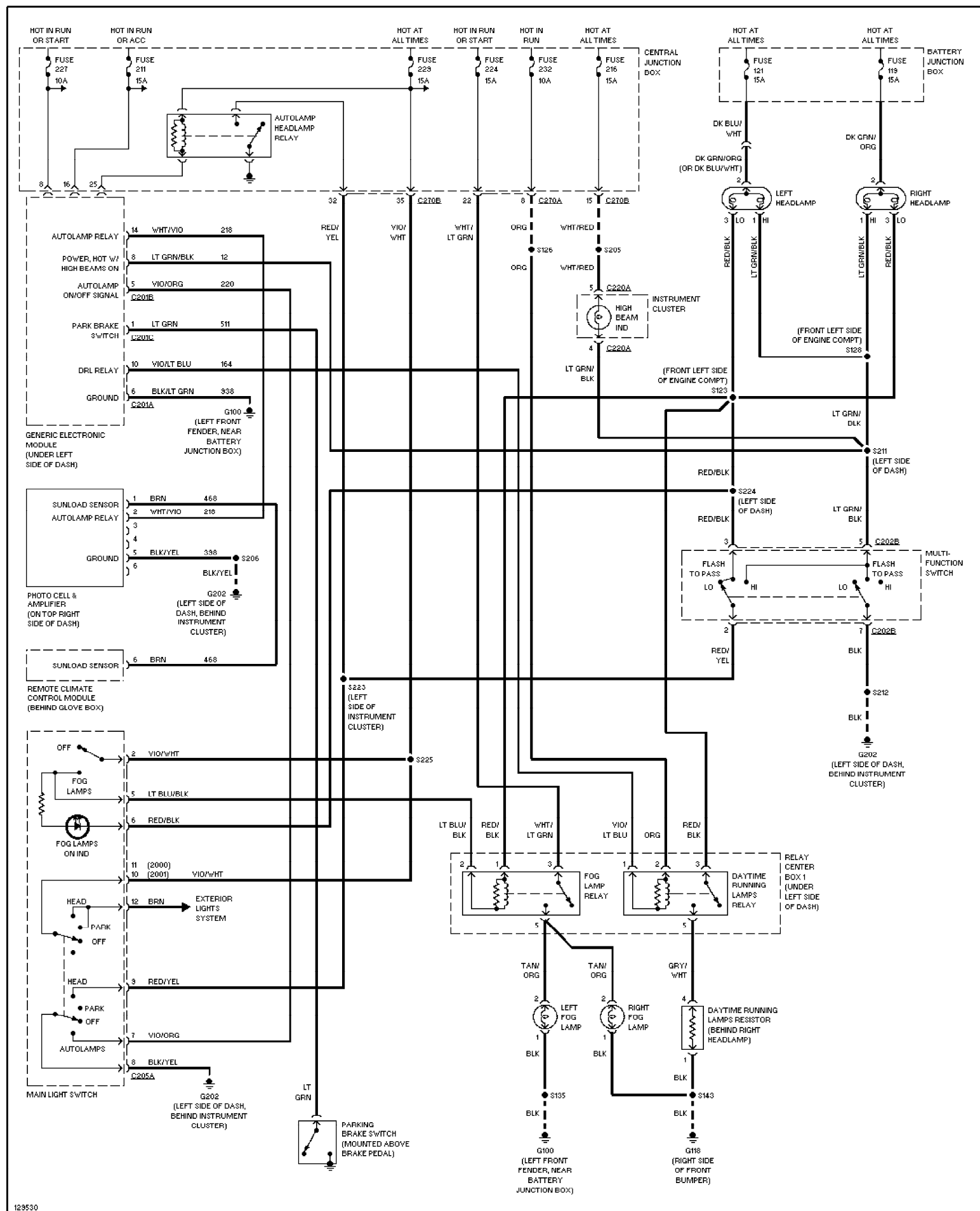
Fig. 31: Autolamps Circuit, W/ DRL 2001 Ford Taurus SEL
