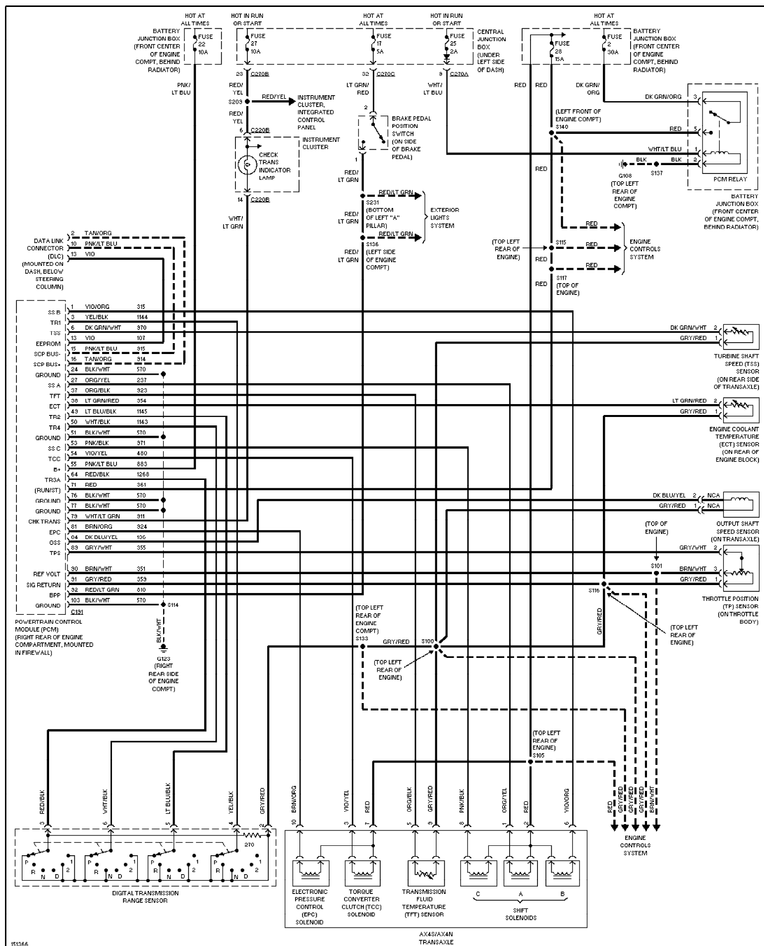
Fig. 55: 3.0L 12-Valve, A/T Circuit 2001 Ford Taurus SEL
