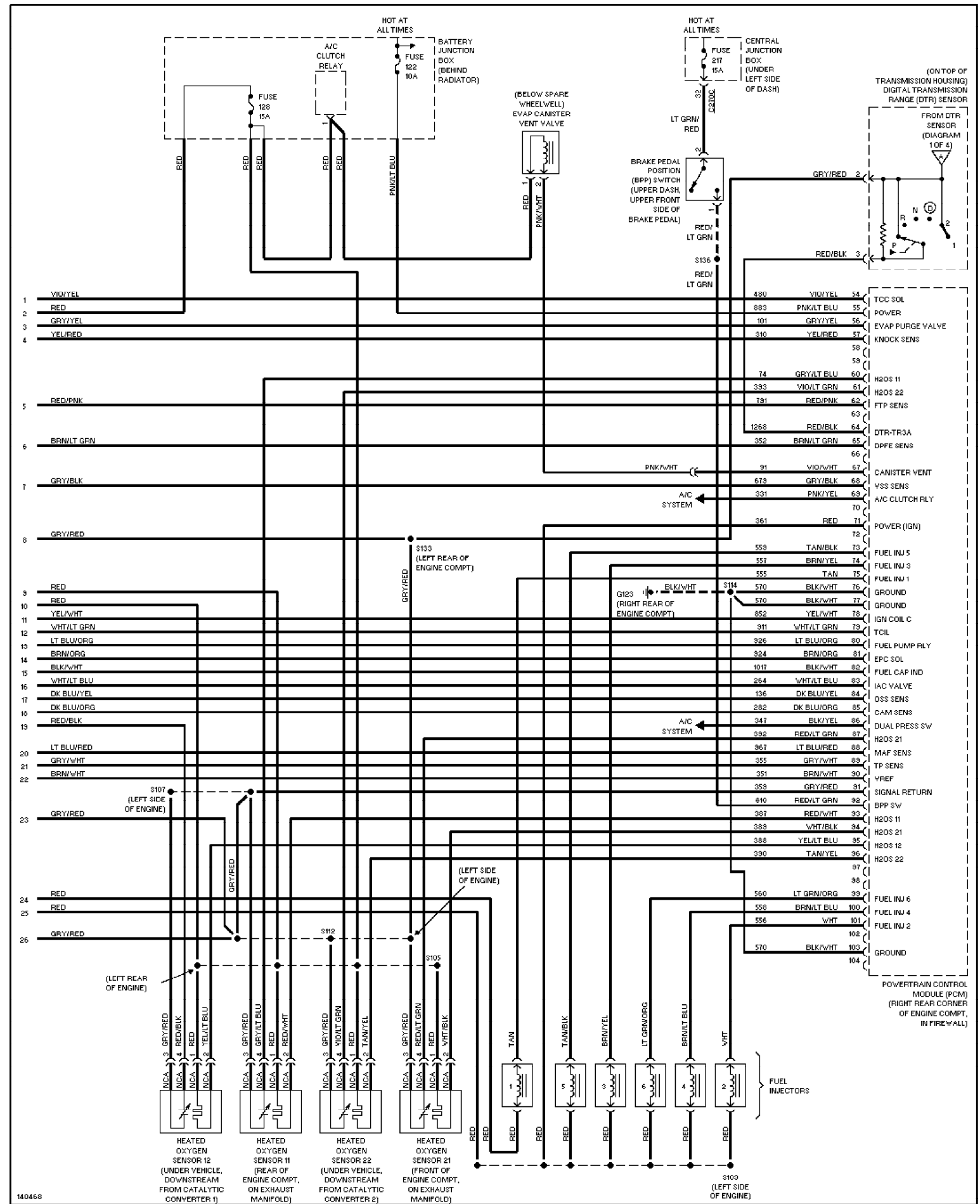
Fig. 20: 3.0L 24-Valve, Engine Performance Circuits (4 of 4)
