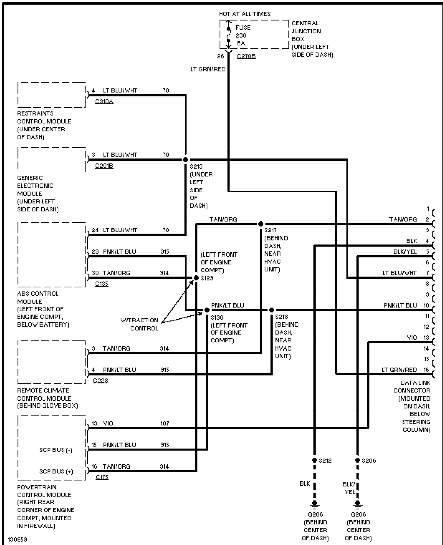
Fig. 9: Computer Data Lines 2001 Ford Taurus SEL
