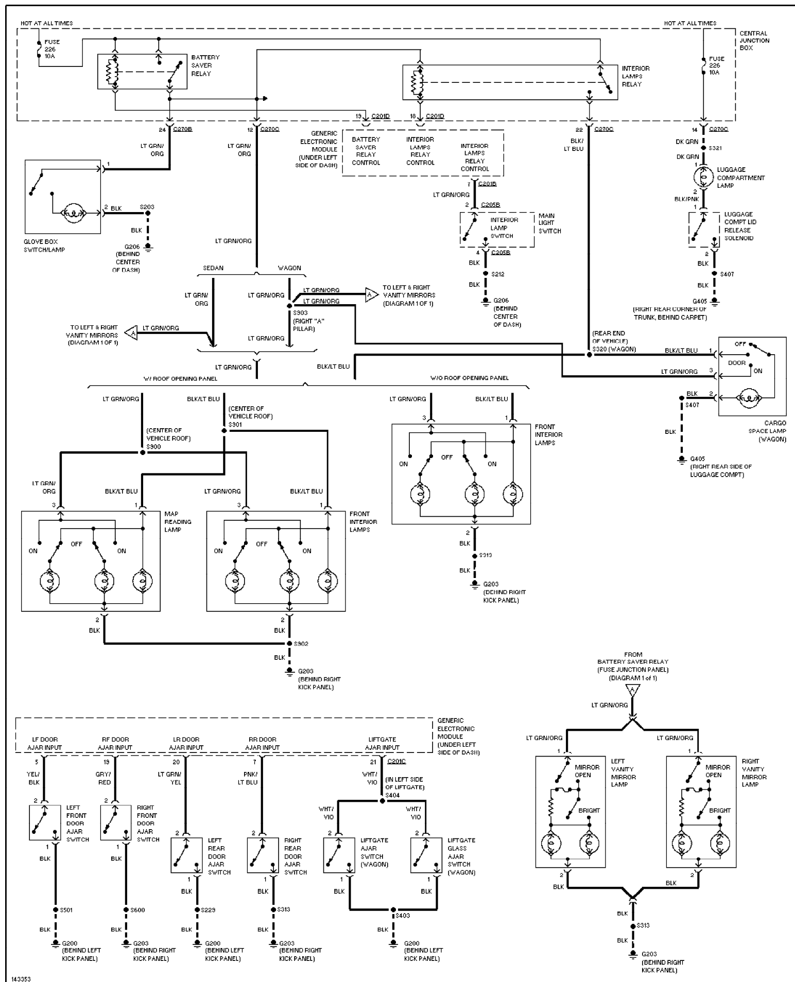
Fig. 37: Courtesy Lamps Circuit 2001 Ford Taurus SEL
