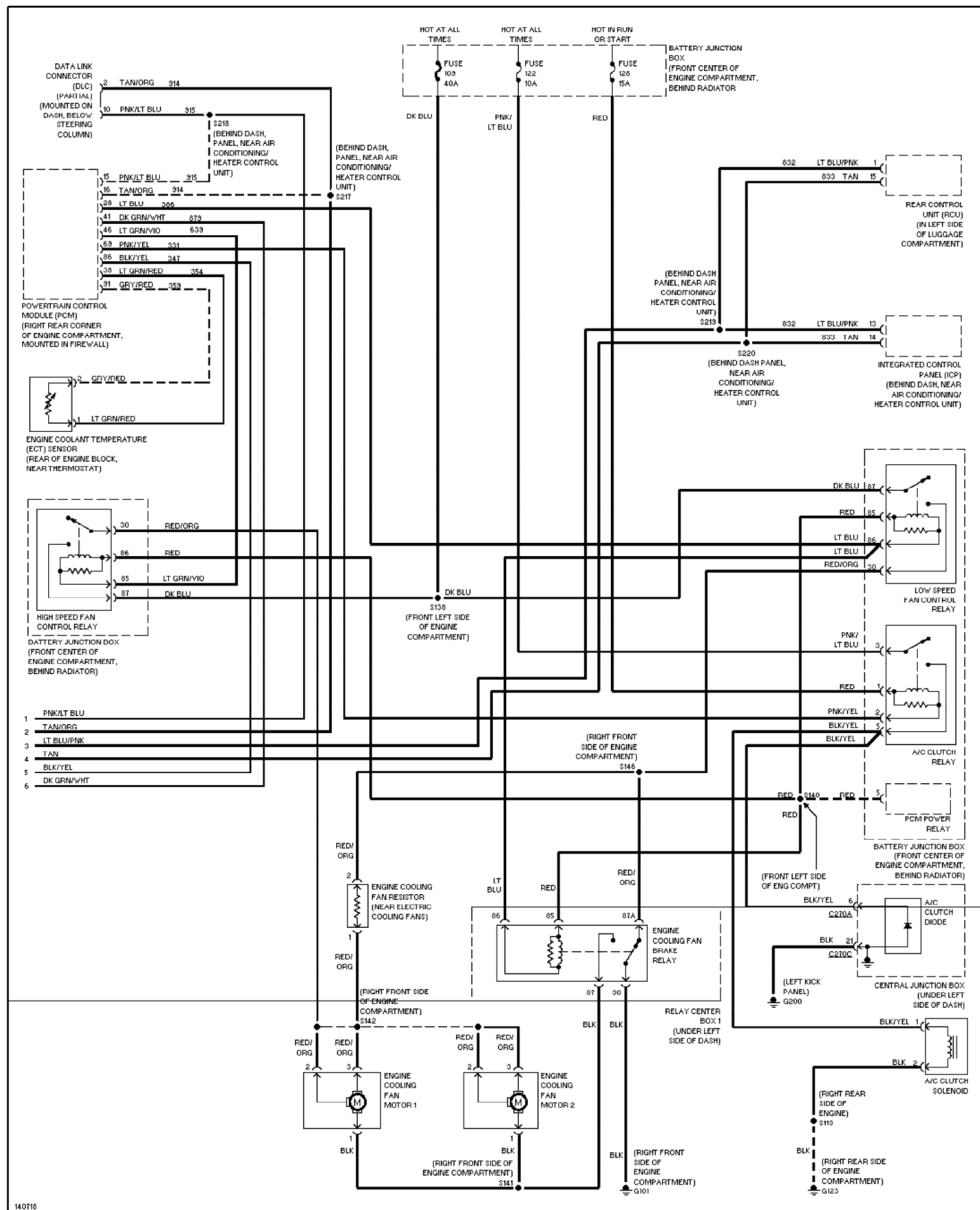
Fig. 2: Automatic A/C Circuit (2 of 2) 2001 Ford Taurus SEL
