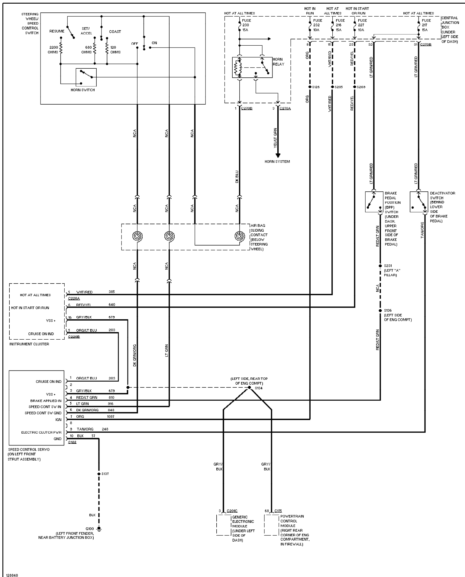
Fig. 11: Cruise Control Circuit 2001 Ford Taurus SEL
