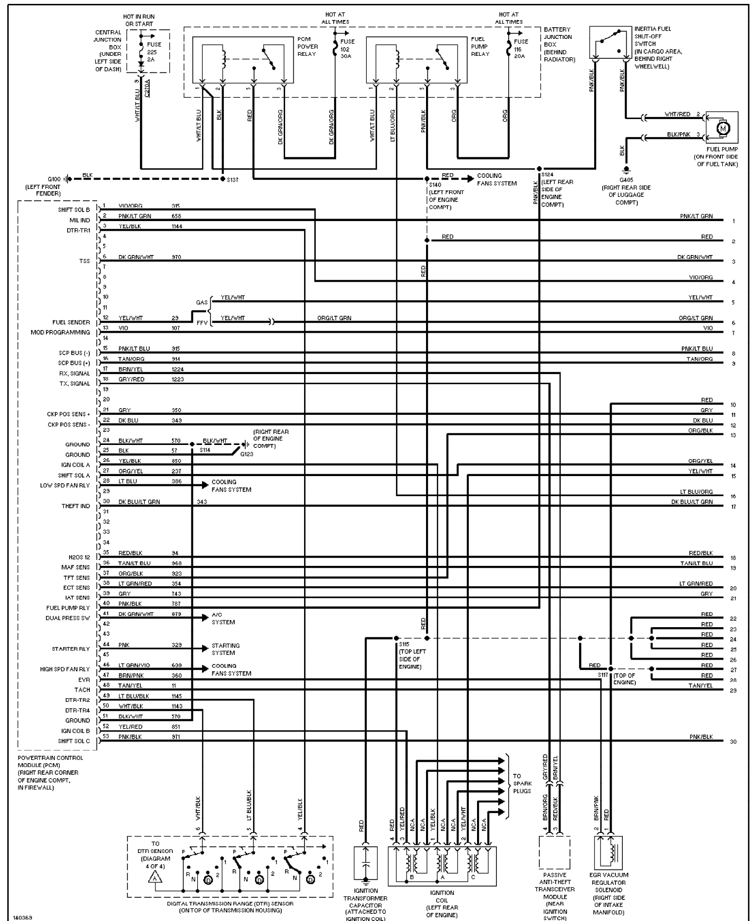
Fig. 13: 3.0L 12-Valve, Engine Performance Circuits (1 of 4)
