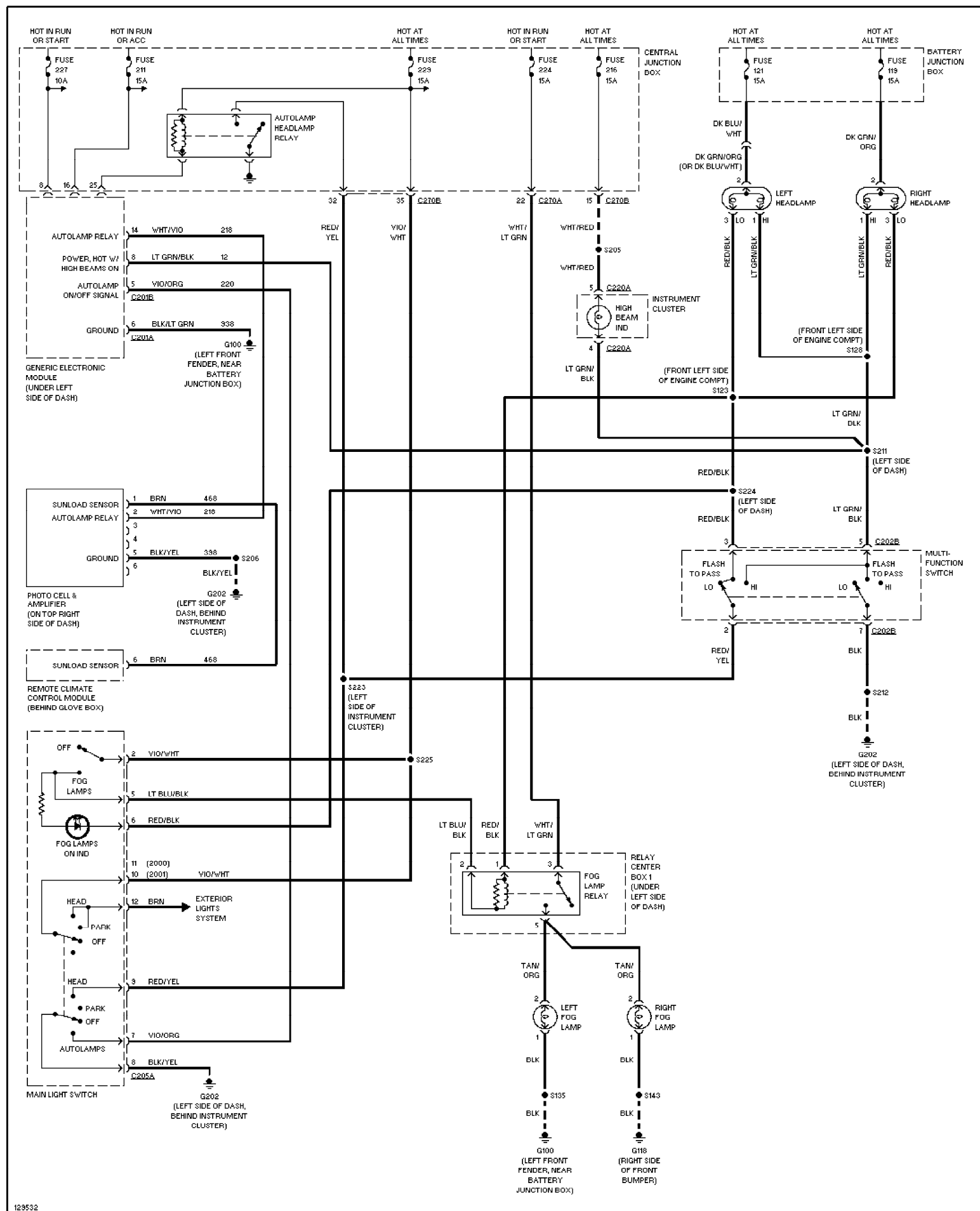
Fig. 32: Autolamps Circuit, W/O DRL 2001 Ford Taurus SEL
