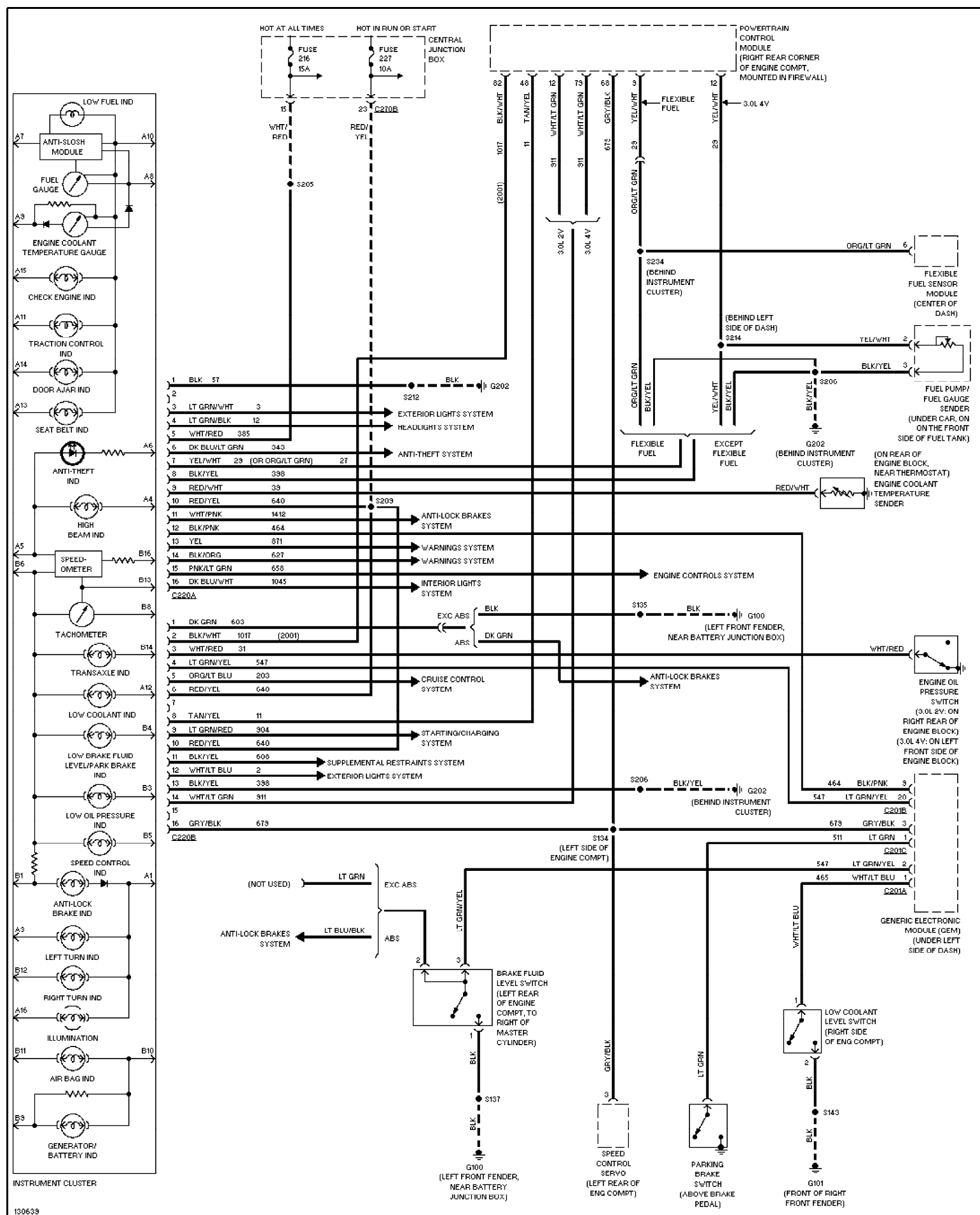
Fig. 36: Instrument Cluster Circuit 2001 Ford Taurus SEL
