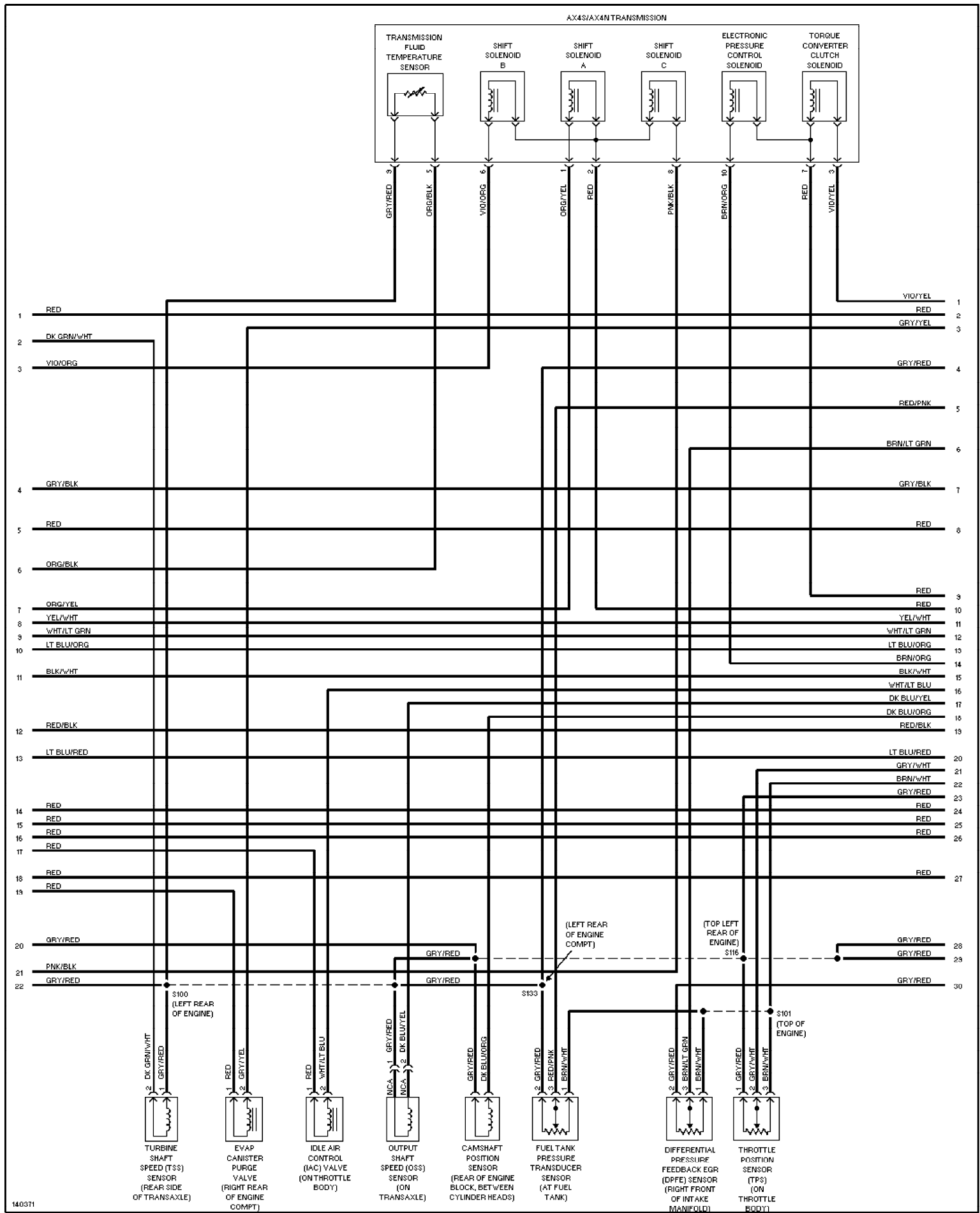
Fig. 23: 3.0L Flex Fuel, Engine Performance Circuits (3 of 4) 2001 Ford Taurus SEL
