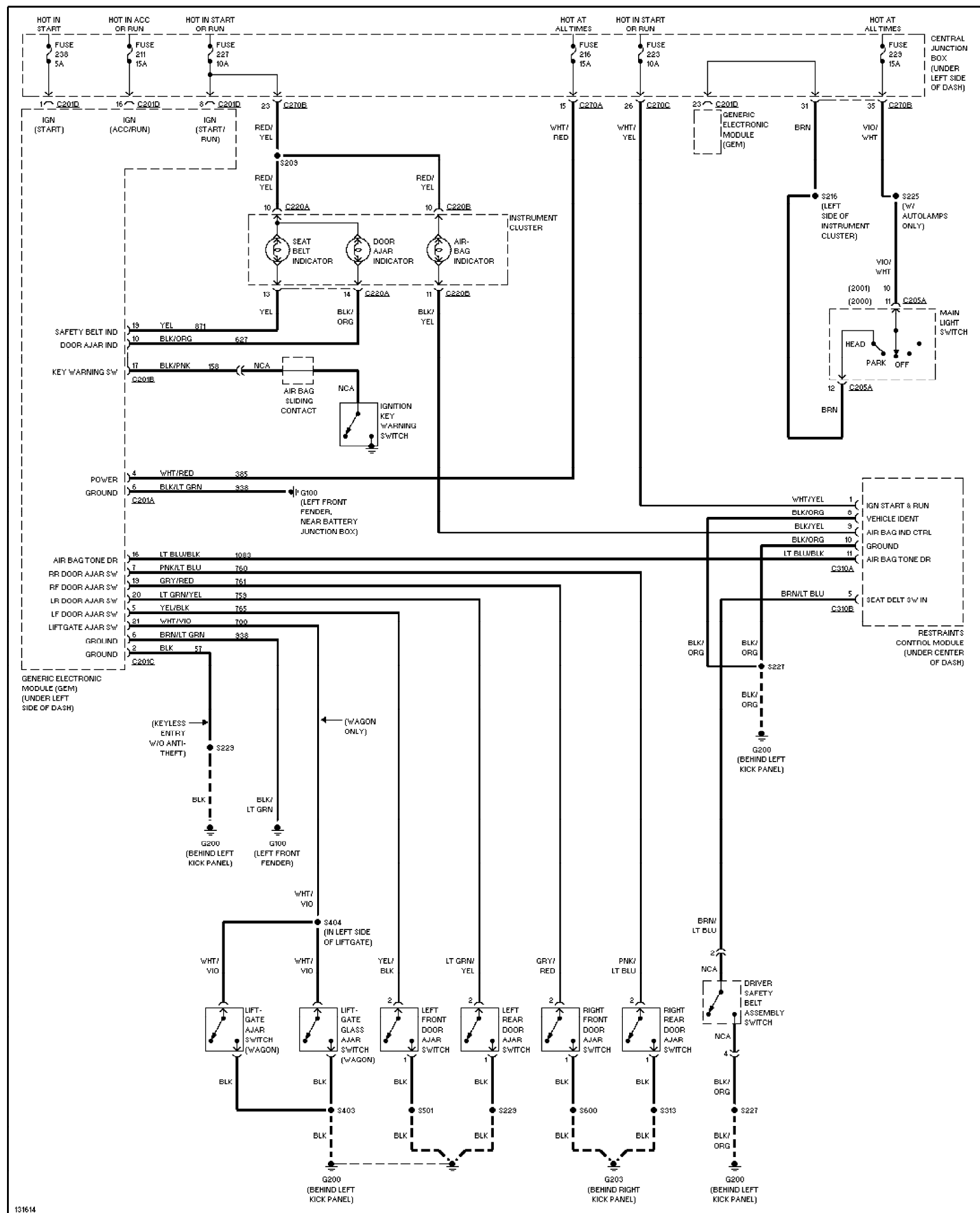
Fig. 59: Warning System Circuits 2001 Ford Taurus SEL
