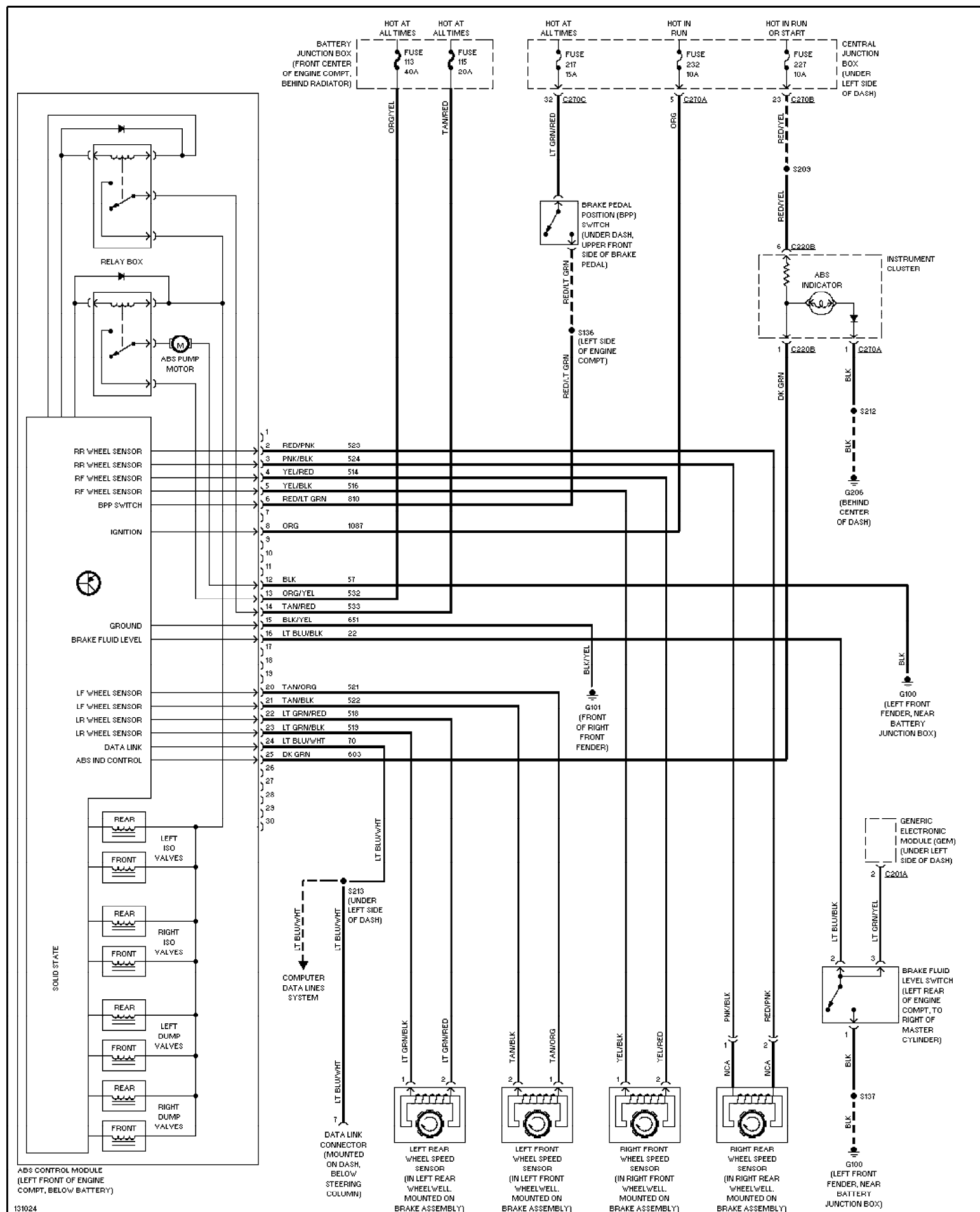
Fig. 5: Anti-lock Brake Circuits, W/O Traction Control 2001 Ford Taurus SEL
