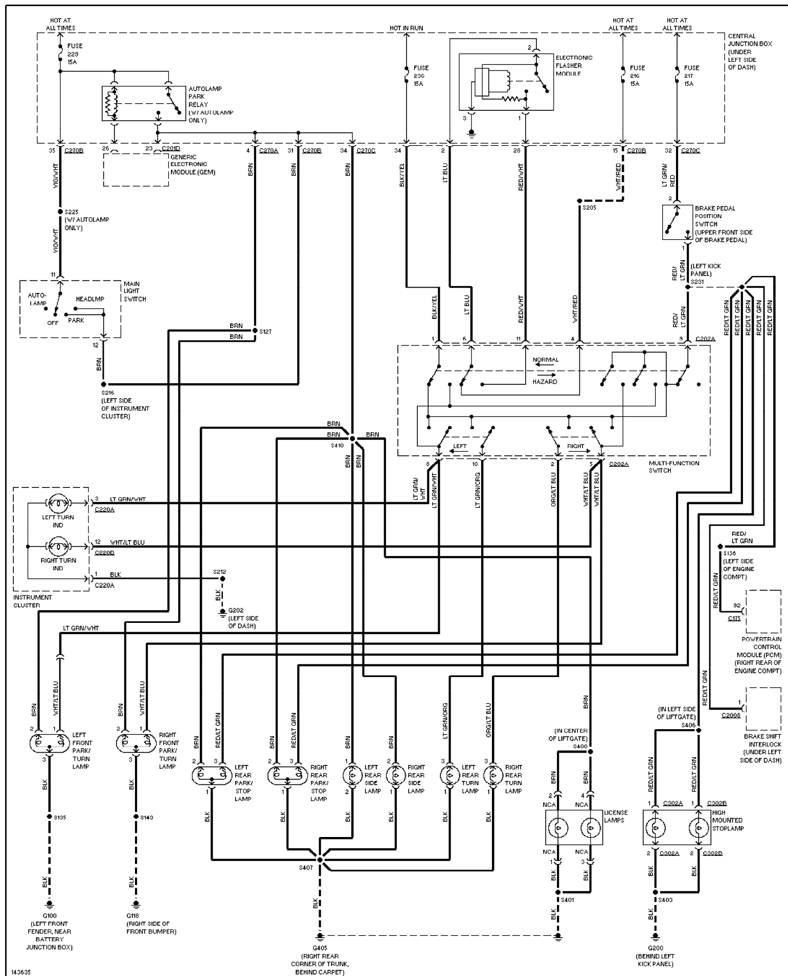
Fig. 27: Exterior Lamps Circuit, Wagon 2001 Ford Taurus SEL
