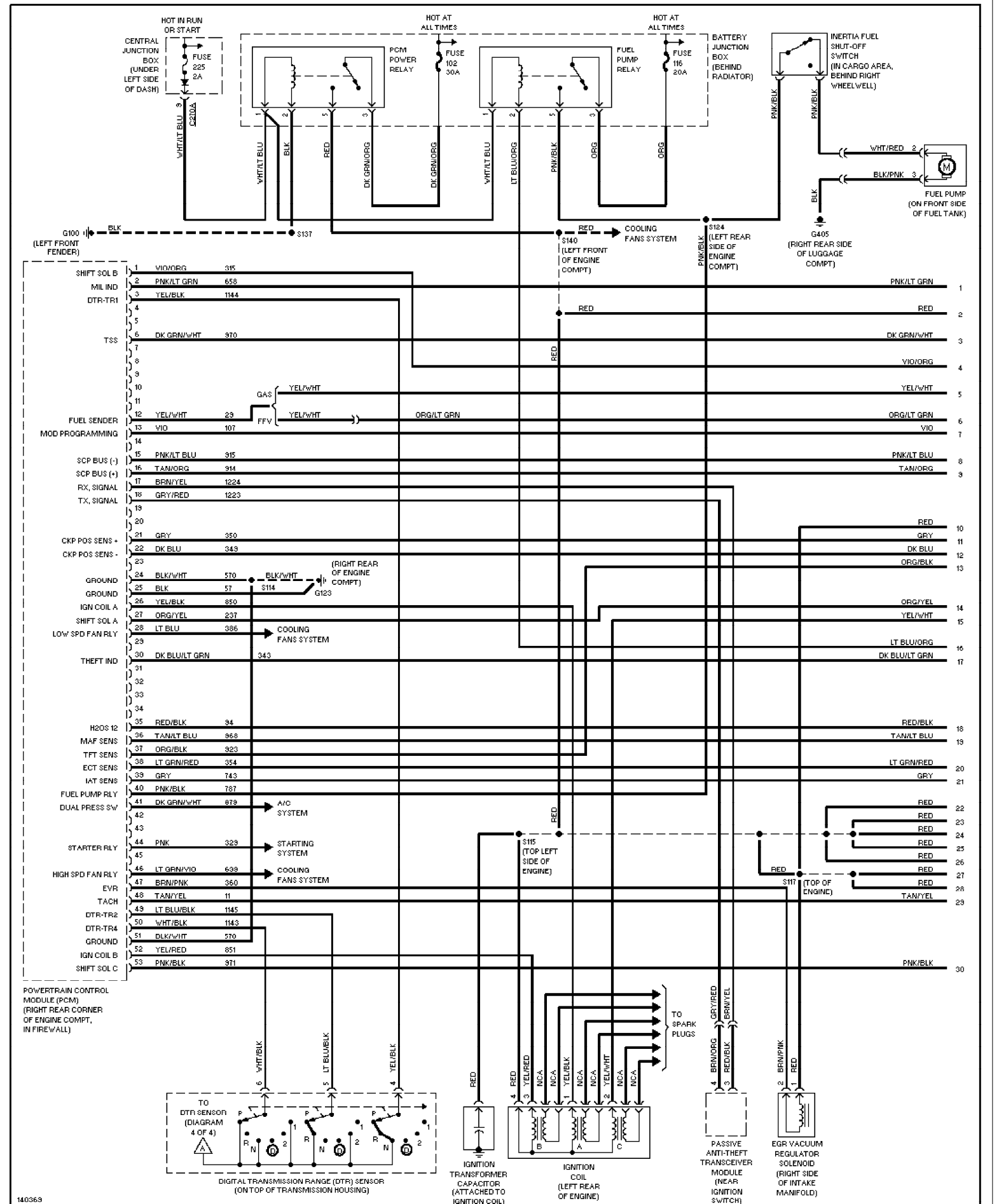
Fig. 21: 3.0L Flex Fuel, Engine Performance Circuits (1 of 4)
