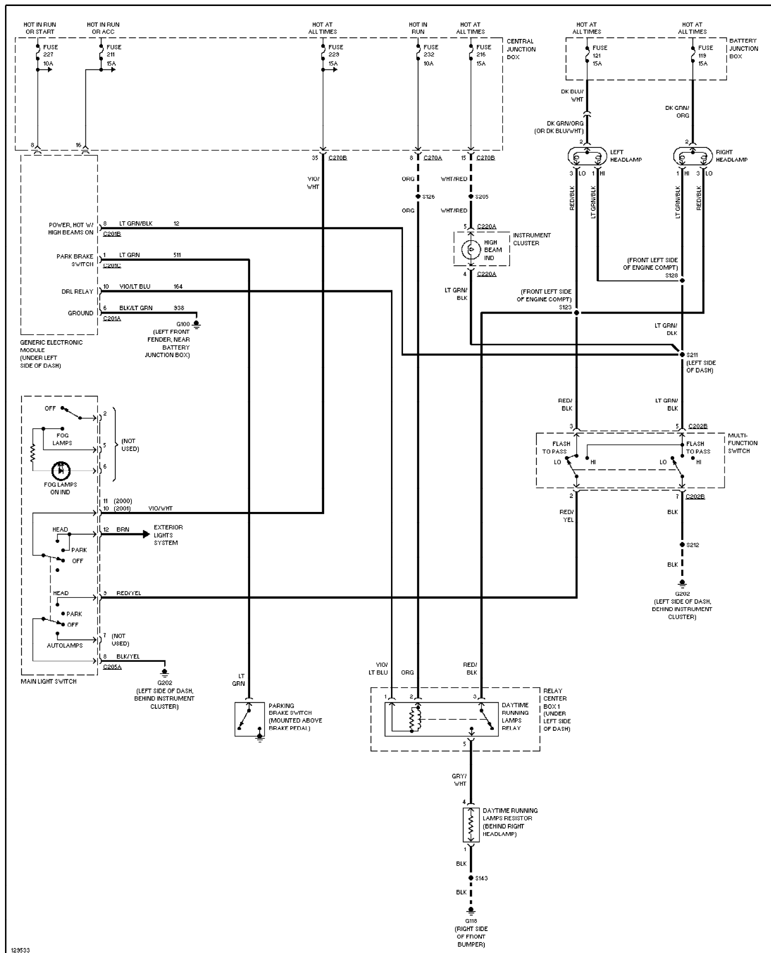
Fig. 33: Headlamps Circuit, W/ DRL 2001 Ford Taurus SEL
