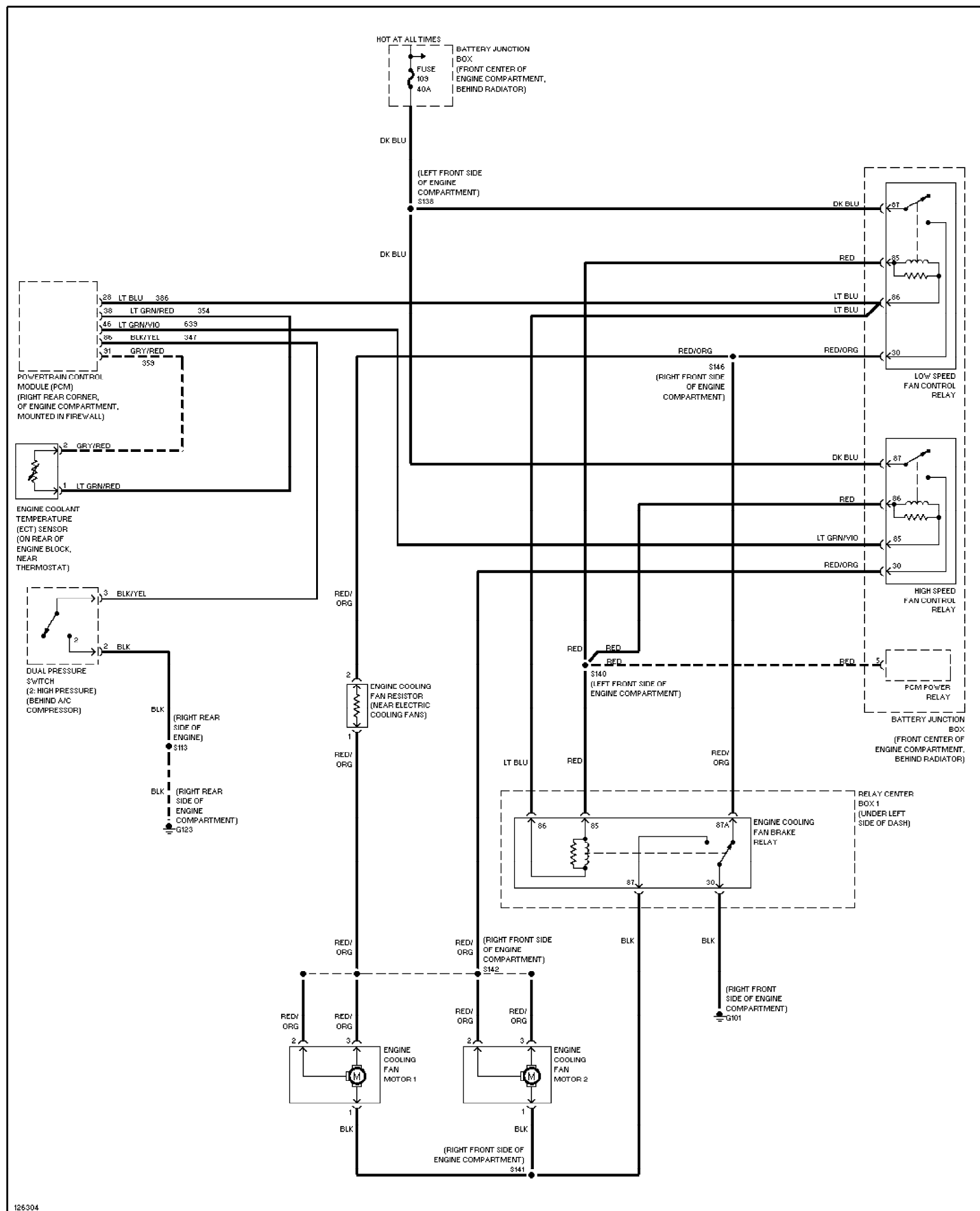
Fig. 10: Cooling Fan Circuit 2001 Ford Taurus SEL
