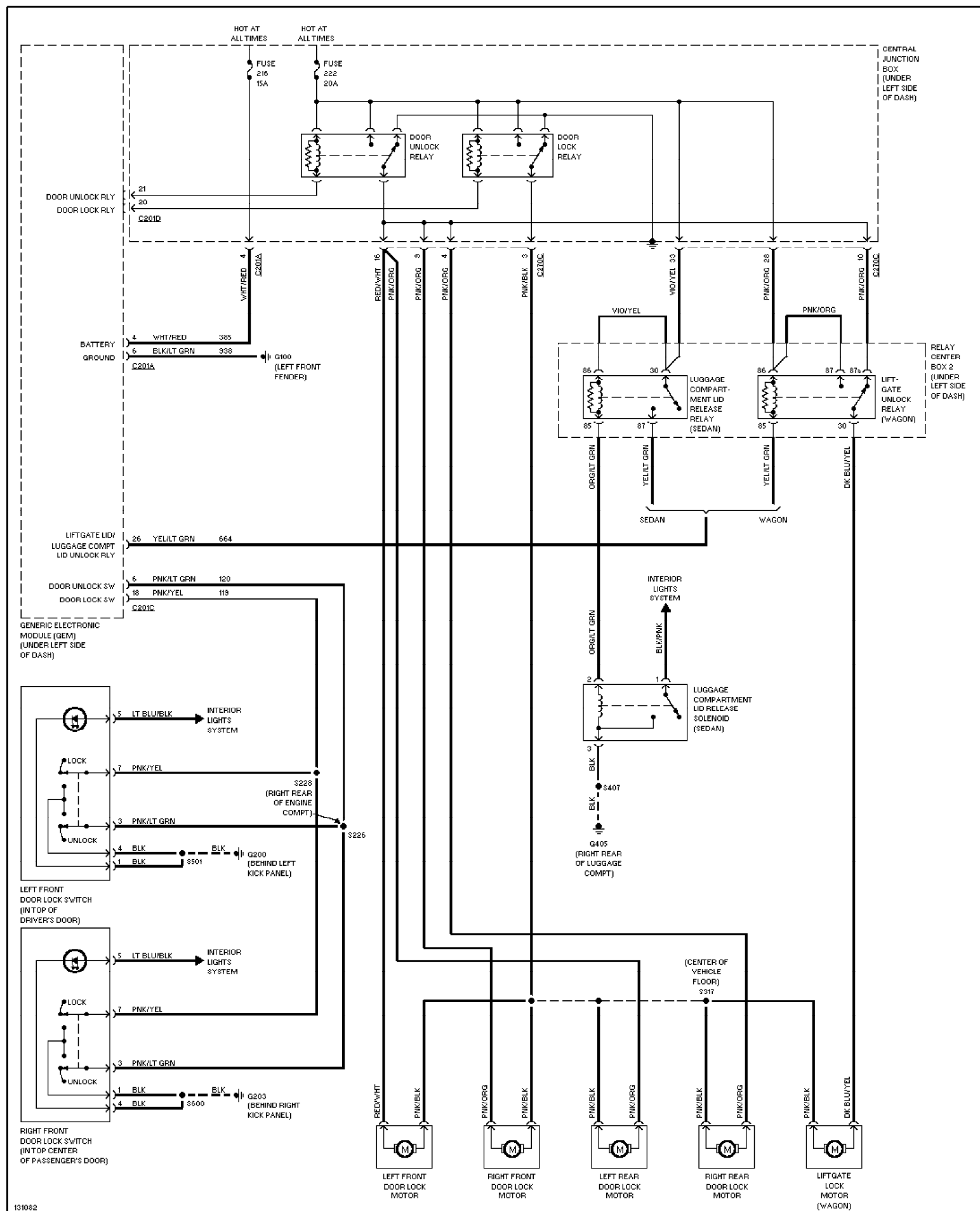
Fig. 44: Power Door Lock Circuit, W/O Keyless Entry 2001 Ford Taurus SEL
