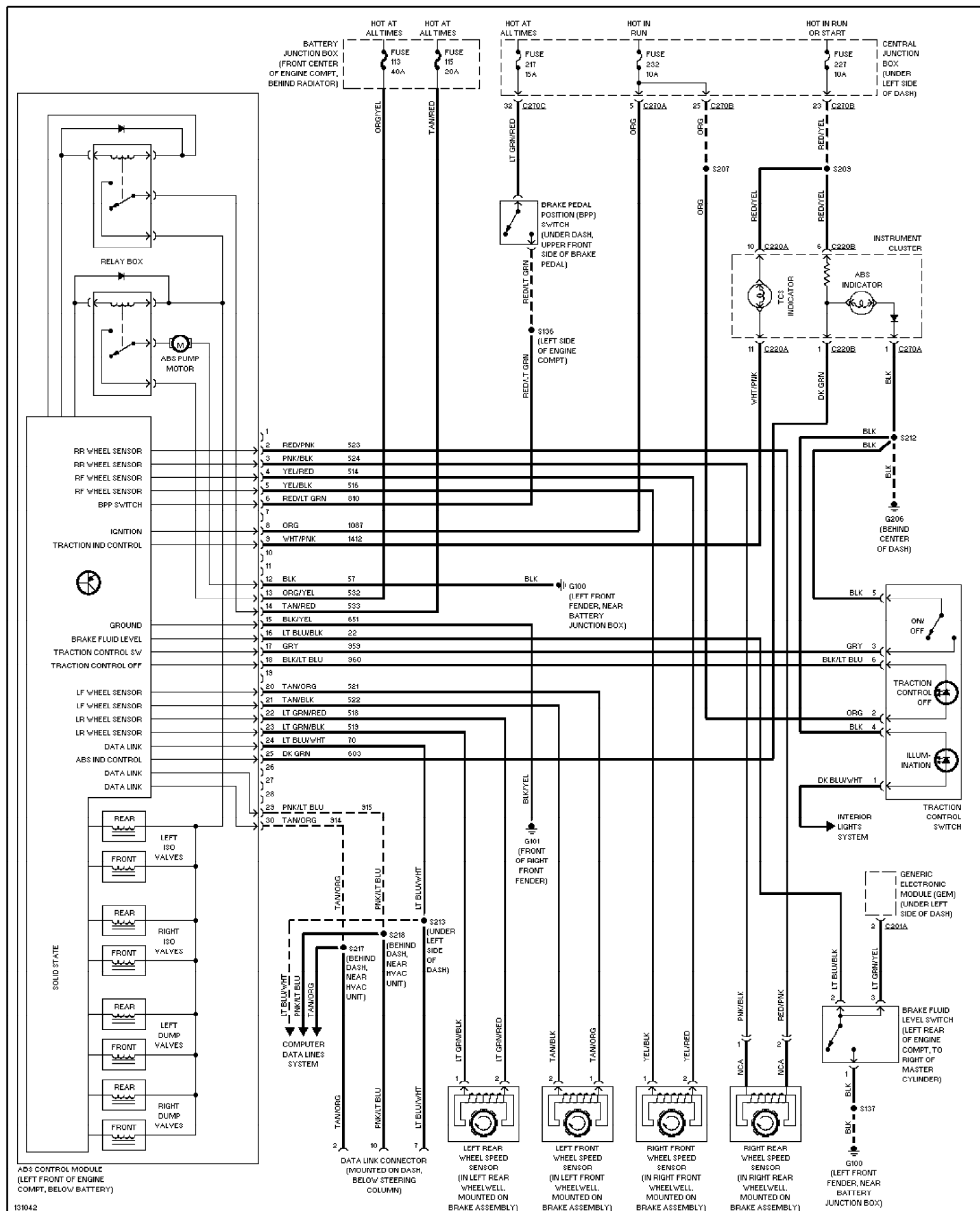
Fig. 4: Anti-lock Brake Circuits, W/ Traction Control 2001 Ford Taurus SEL
