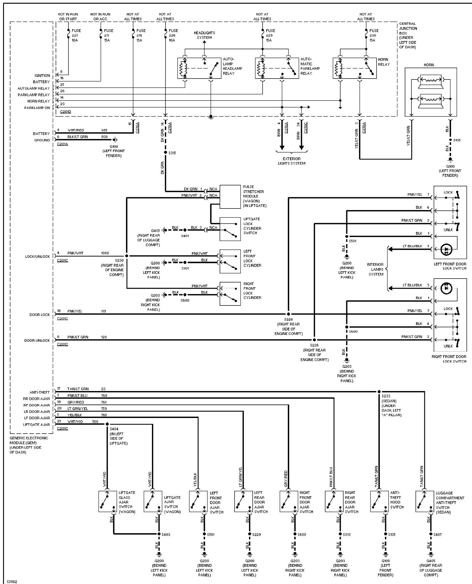
Fig. 6: Forced Entry Circuit 2001 Ford Taurus SEL
