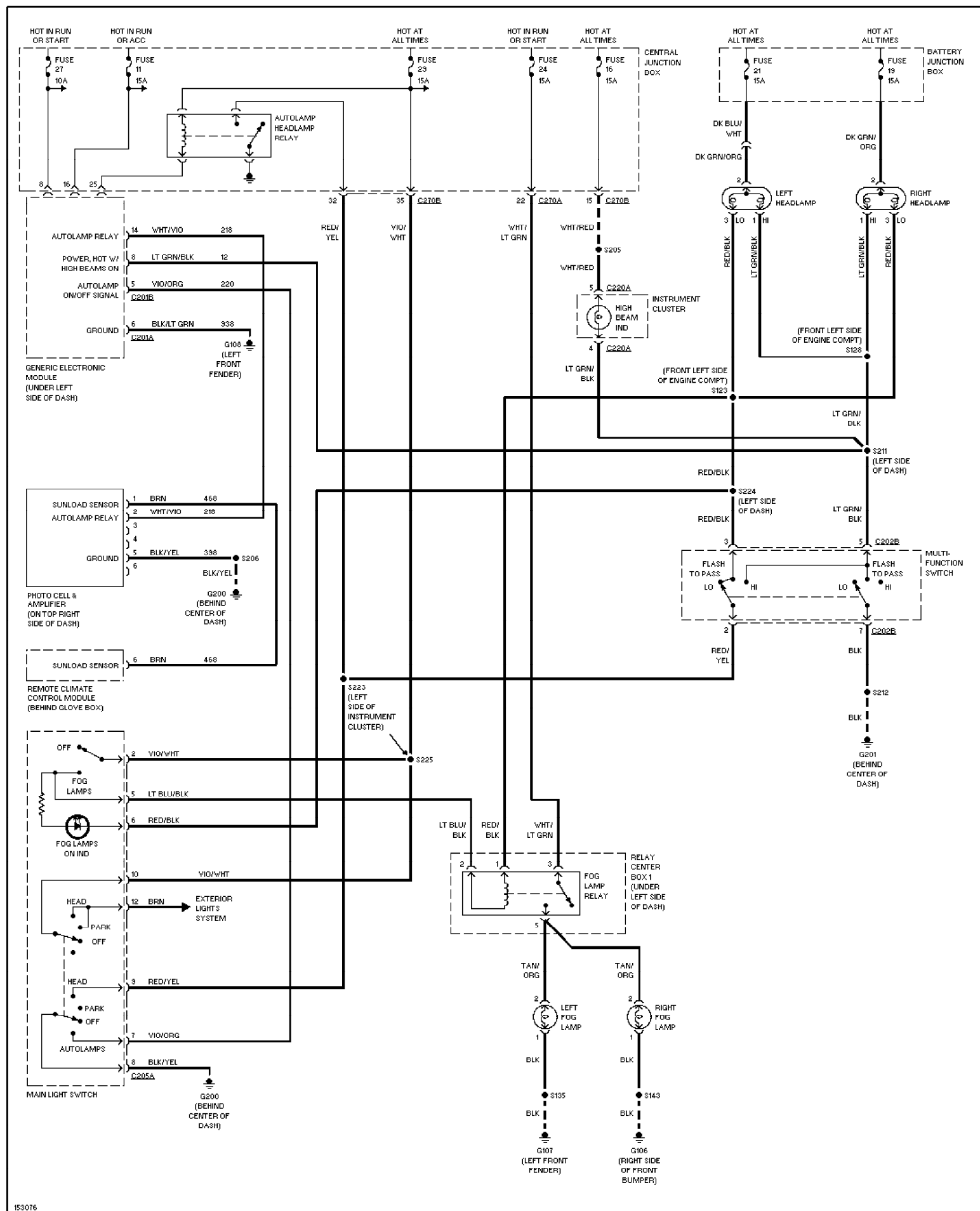
Fig. 33: Autolamps Circuit, W/O DRL 2002 Ford Taurus SEL
