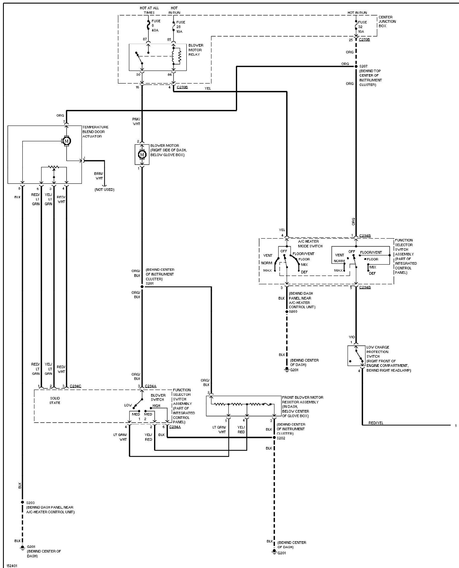
Fig. 3: Manual A/C Circuit (1 of 2) 2002 Ford Taurus SEL
