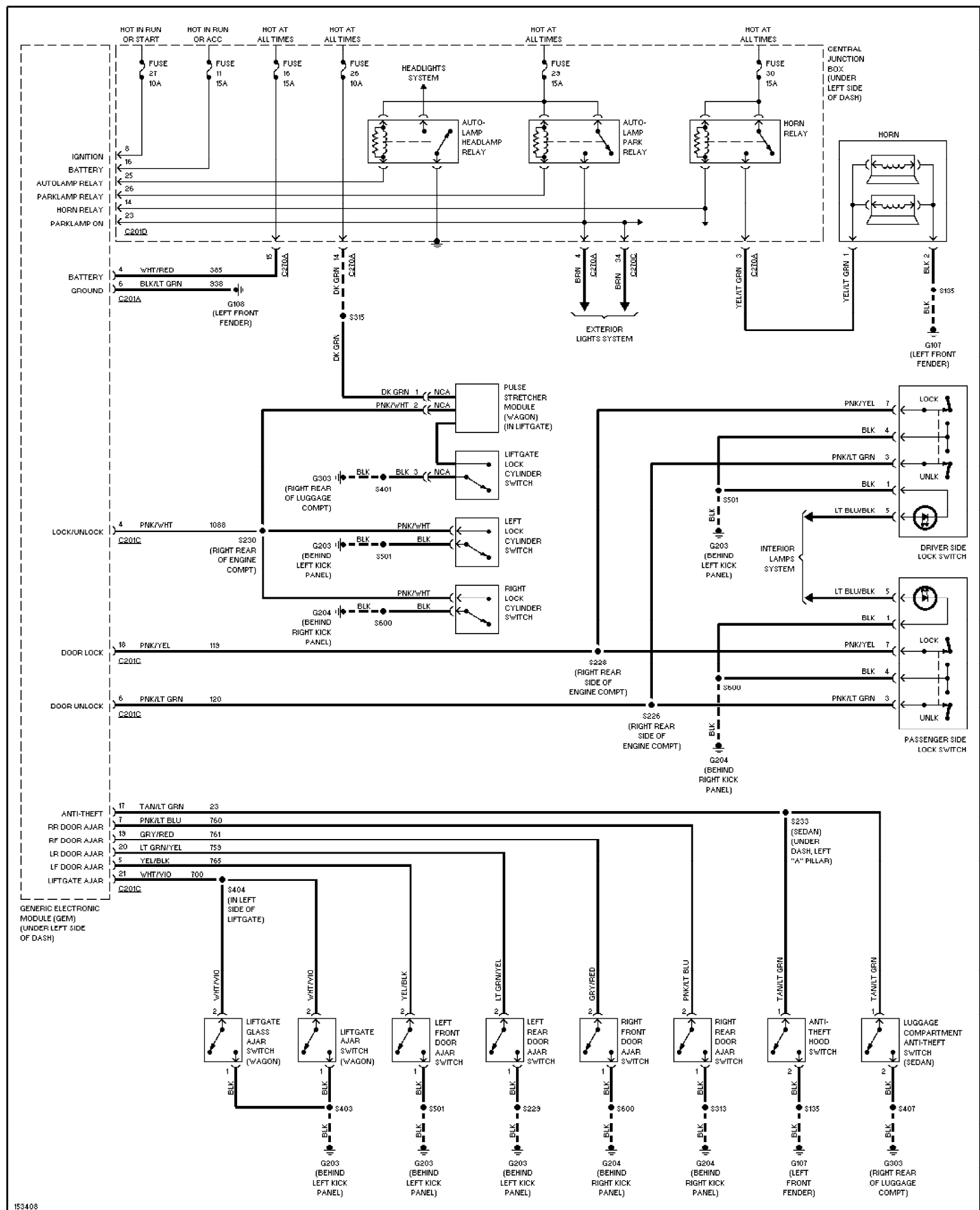
Fig. 7: Forced Entry Circuit 2002 Ford Taurus SEL
