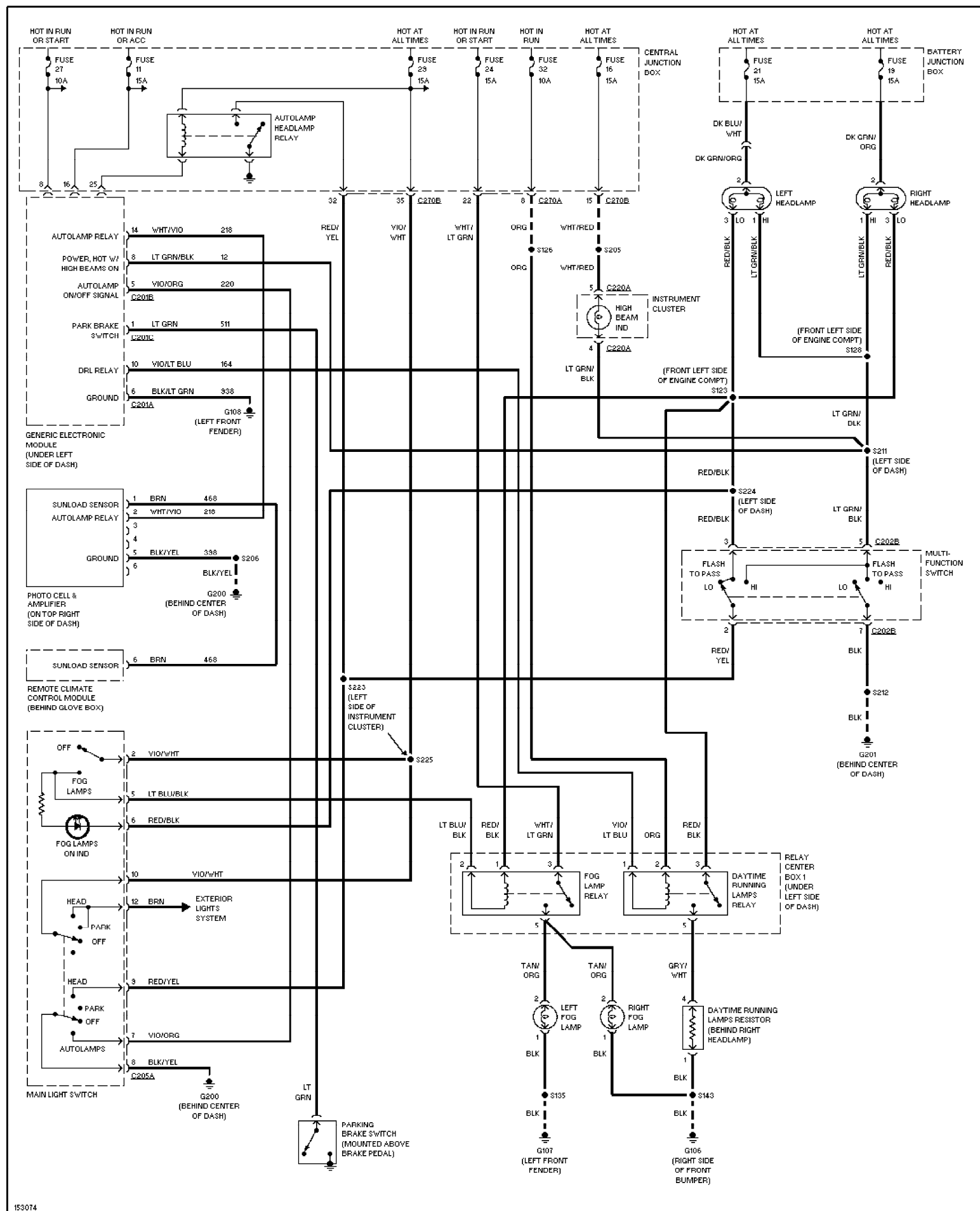
Fig. 32: Autolamps Circuit, W/ DRL 2002 Ford Taurus SEL
