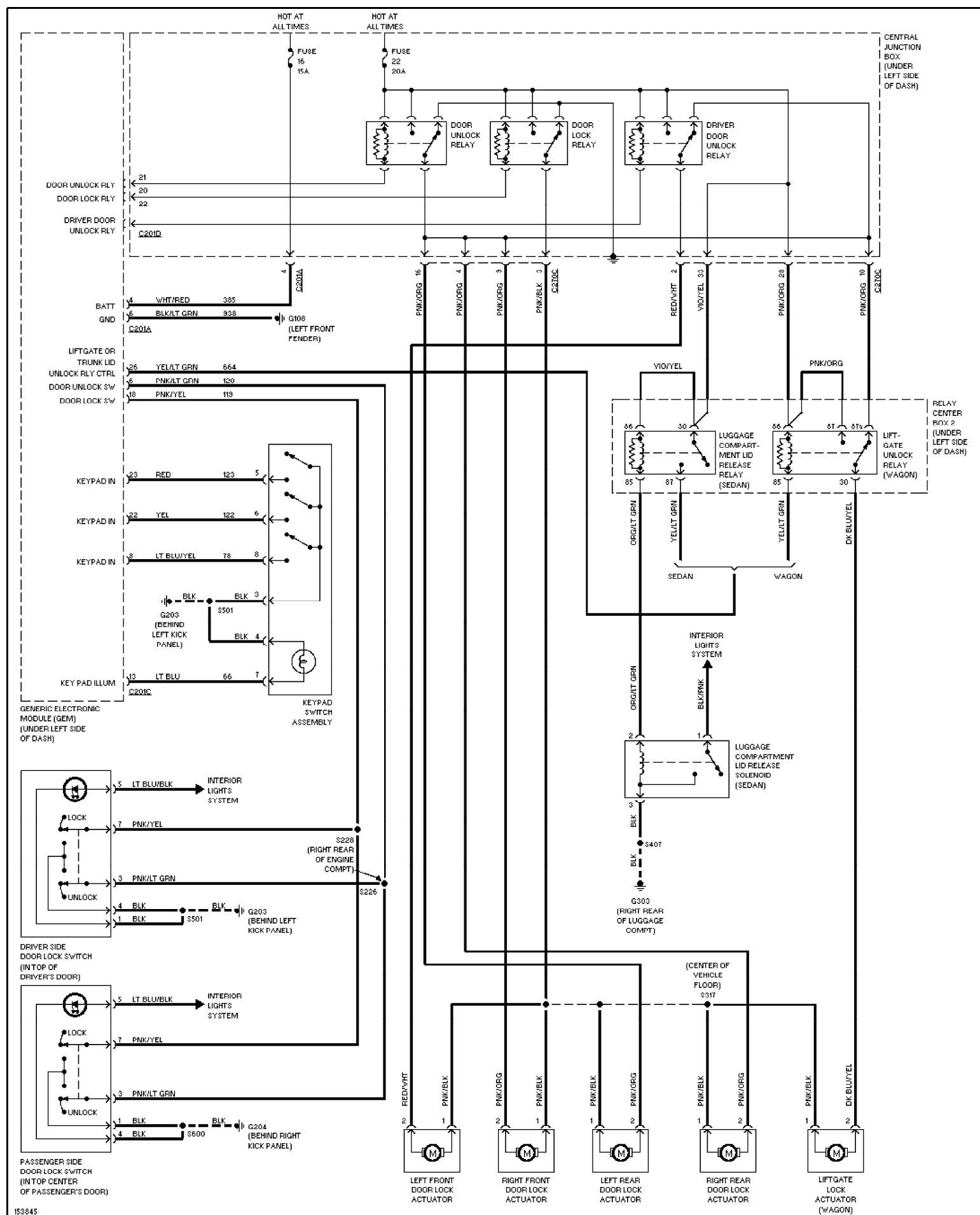
Fig. 45: Power Door Lock Circuit, W/ Keyless Entry 2002 Ford Taurus SEL
