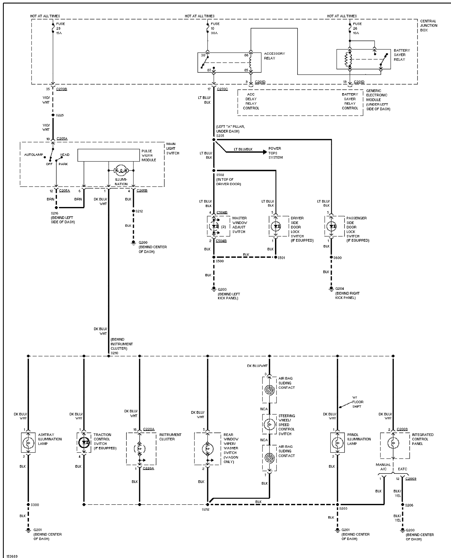
Fig. 40: Instrument Illumination Circuit 2002 Ford Taurus SEL
