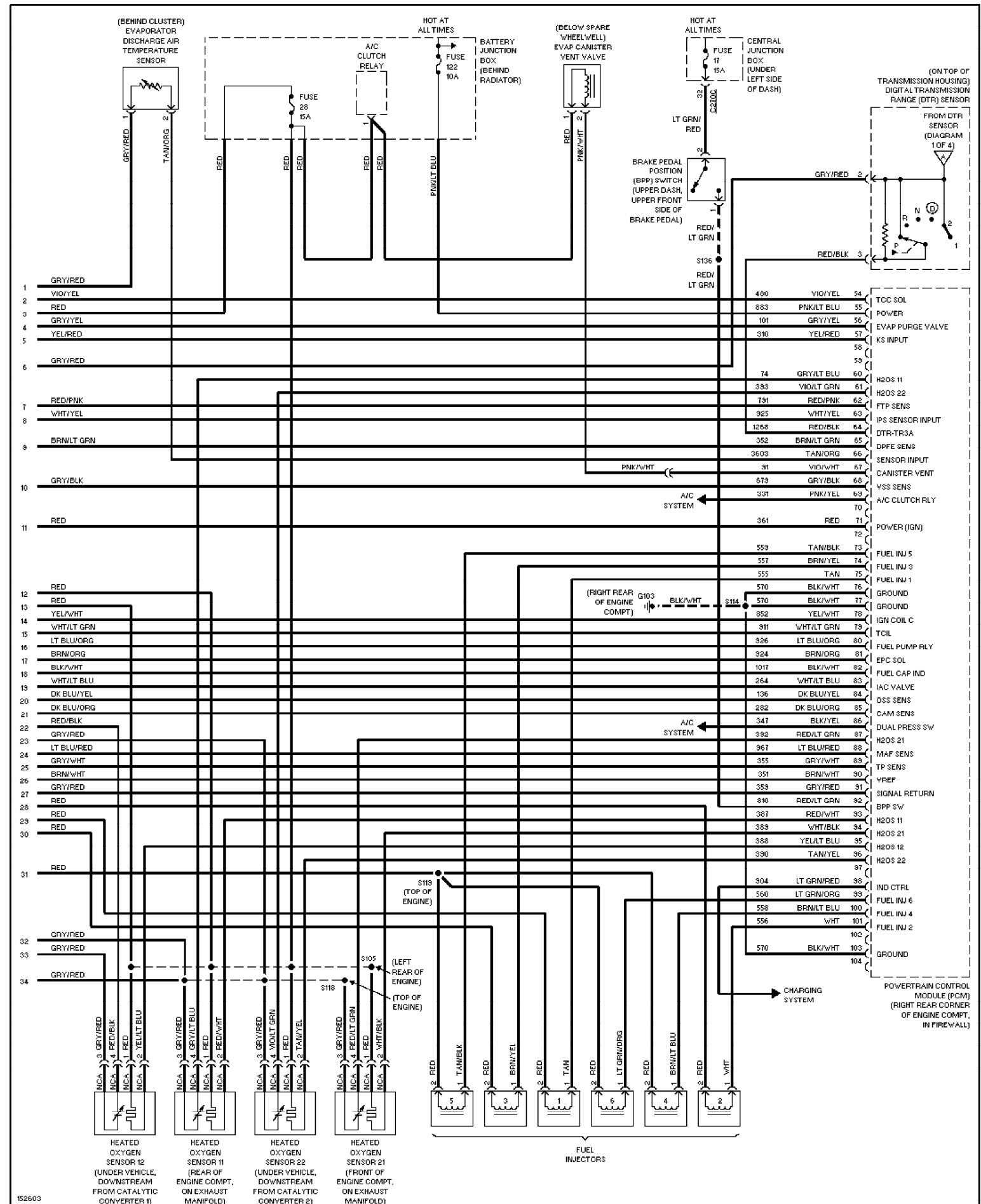
Fig. 17: 3.0L 12-Valve, Engine Performance Circuits (4 of 4) 2002 Ford Taurus SEL
