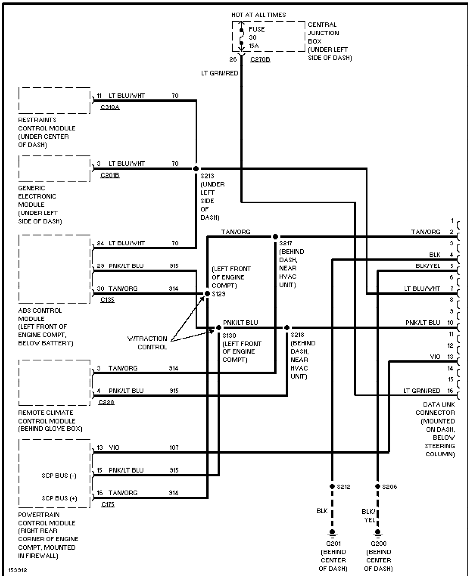
Fig. 10: Computer Data Lines 2002 Ford Taurus SEL
