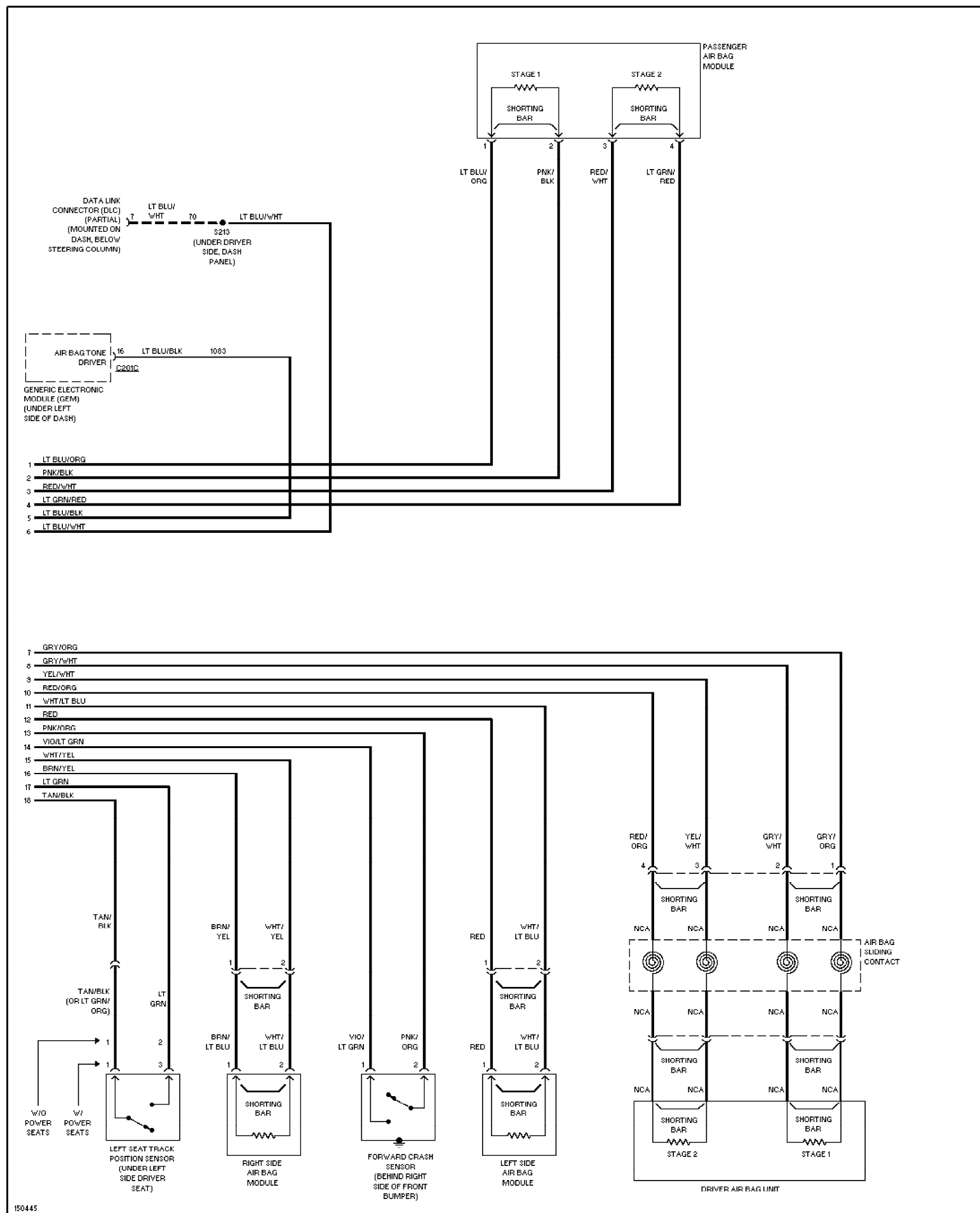
Fig. 58: Supplemental Restraint Circuit (2 of 2) 2002 Ford Taurus SEL
