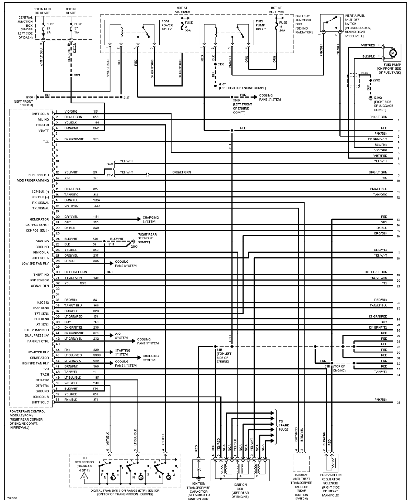
Fig. 22: 3.0L Flex Fuel, Engine Performance Circuits (1 of 4) 2002 Ford Taurus SEL
