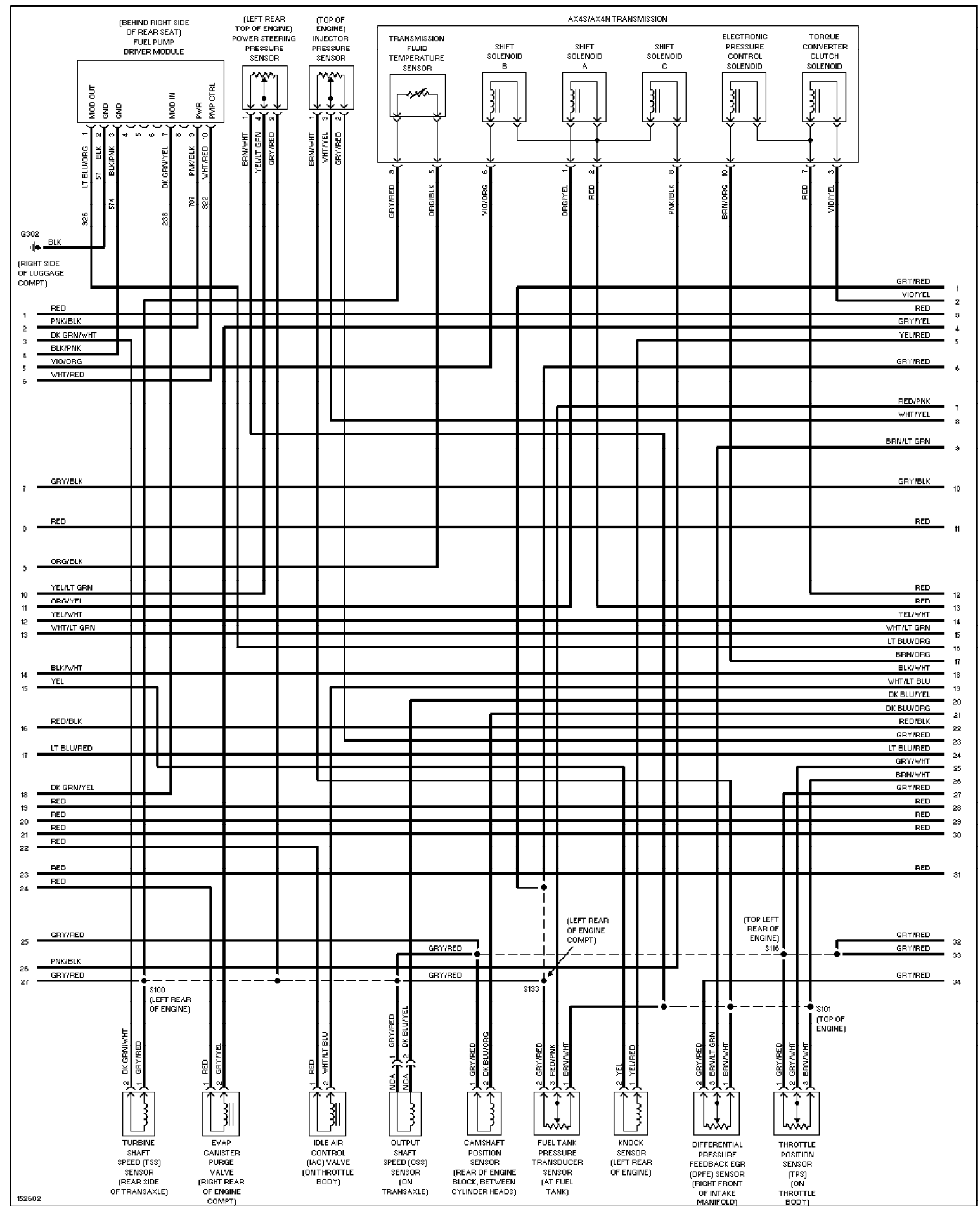
Fig. 24: 3.0L Flex Fuel, Engine Performance Circuits (3 of 4) 2002 Ford Taurus SEL
