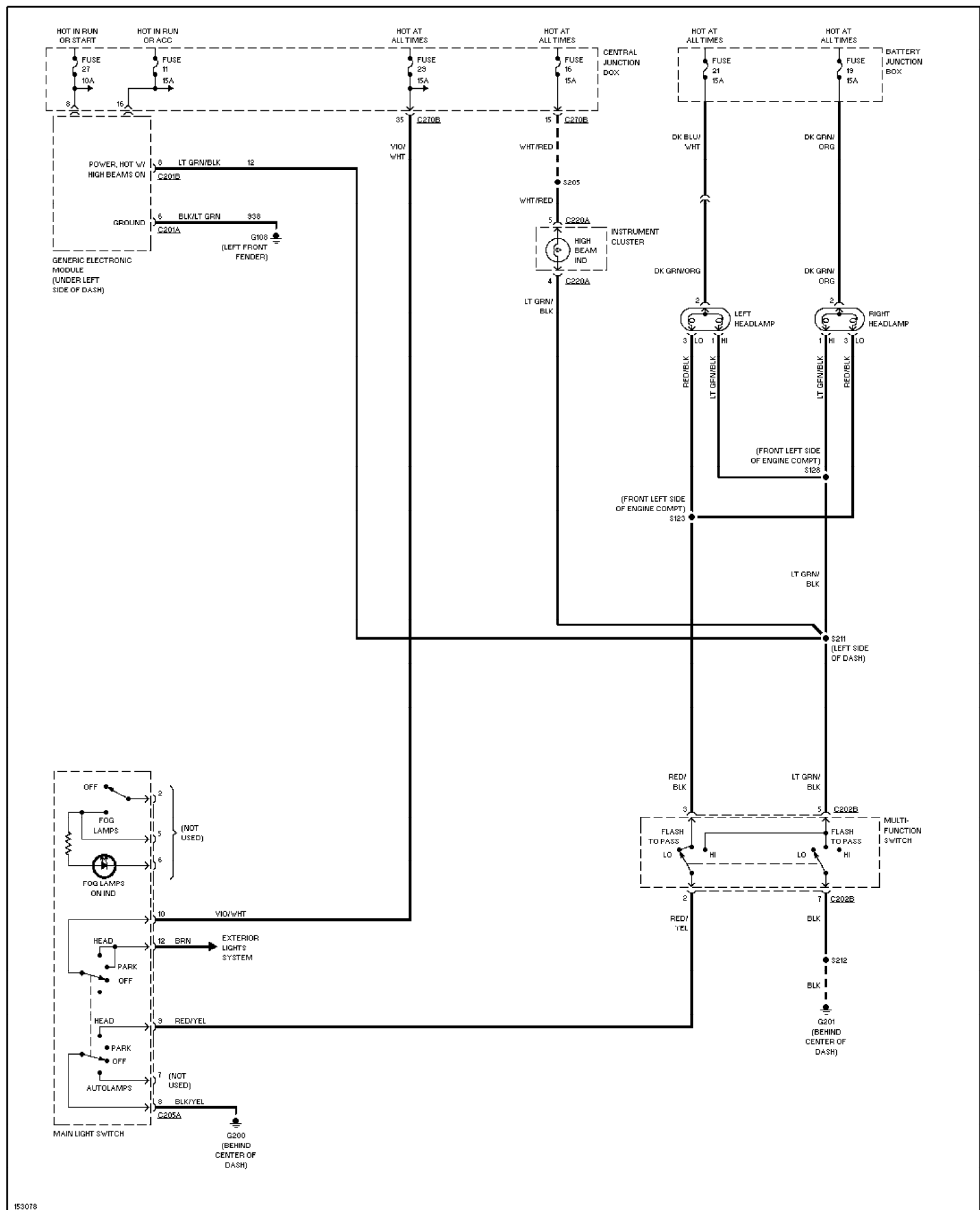
Fig. 35: Headlamps Circuit, W/O DRL 2002 Ford Taurus SEL
