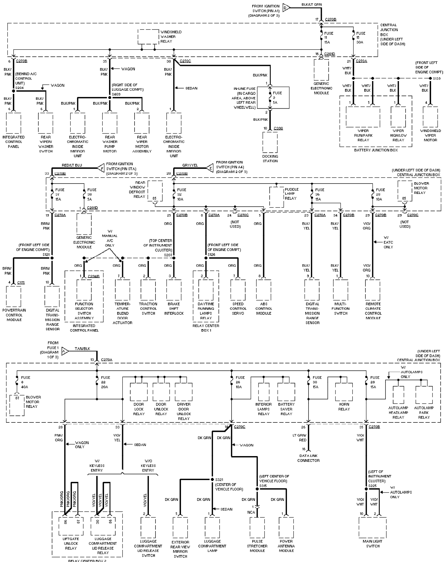
Fig. 44: Power Distribution Circuit (3 of 3) 2002 Ford Taurus SEL
