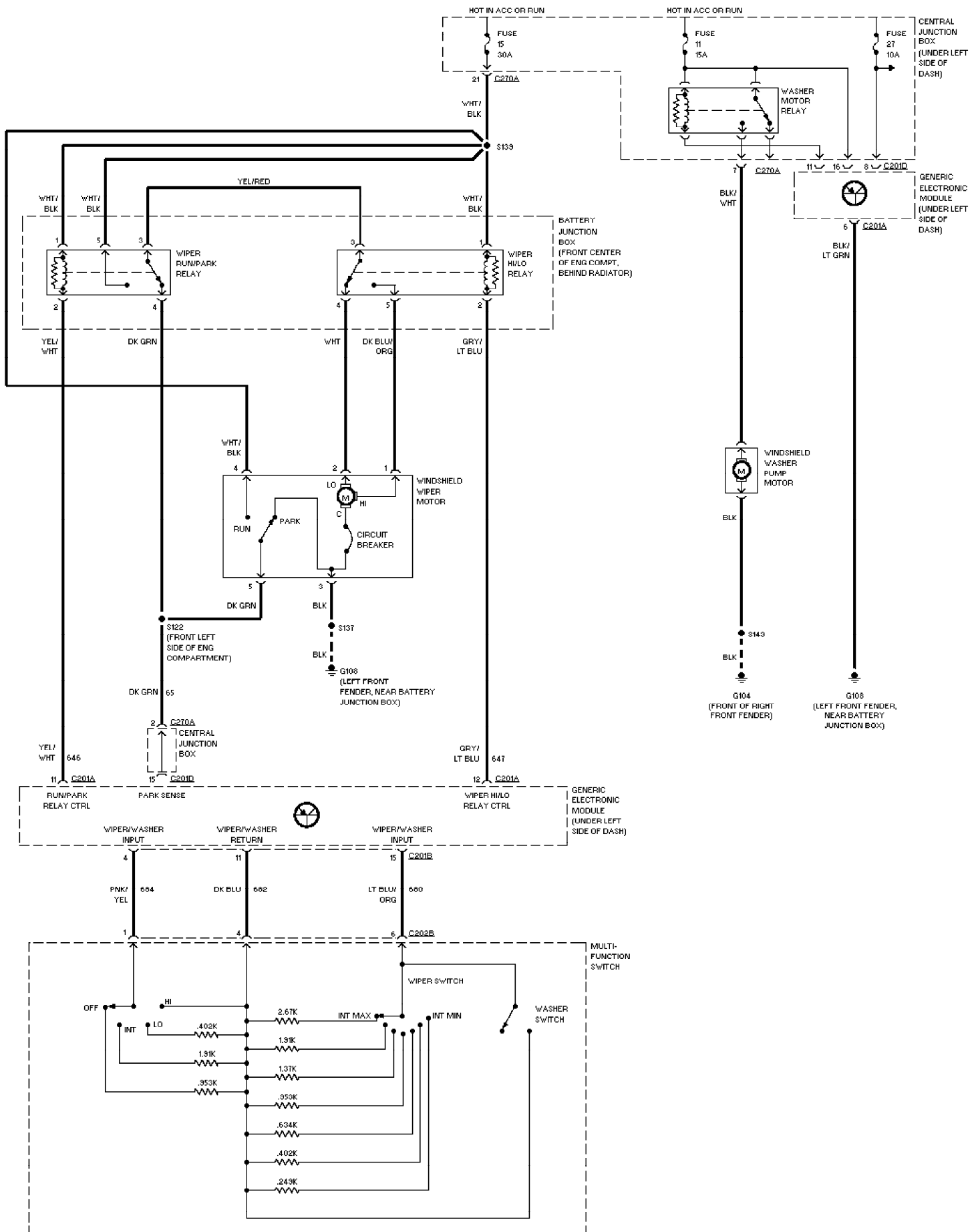
Fig. 64: Front Washer/Wiper Circuit 2002 Ford Taurus SEL
