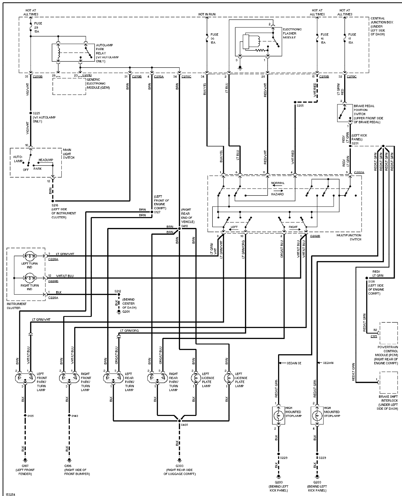
Fig. 27: Exterior Lamps Circuit, Sedan 2002 Ford Taurus SEL
