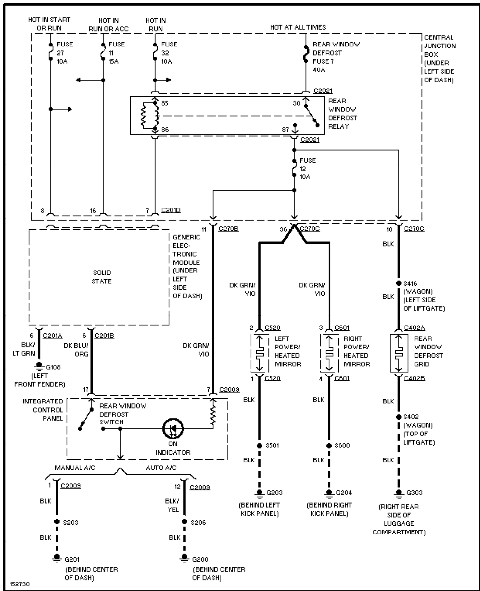
Fig. 13: Defogger Circuit 2002 Ford Taurus SEL
