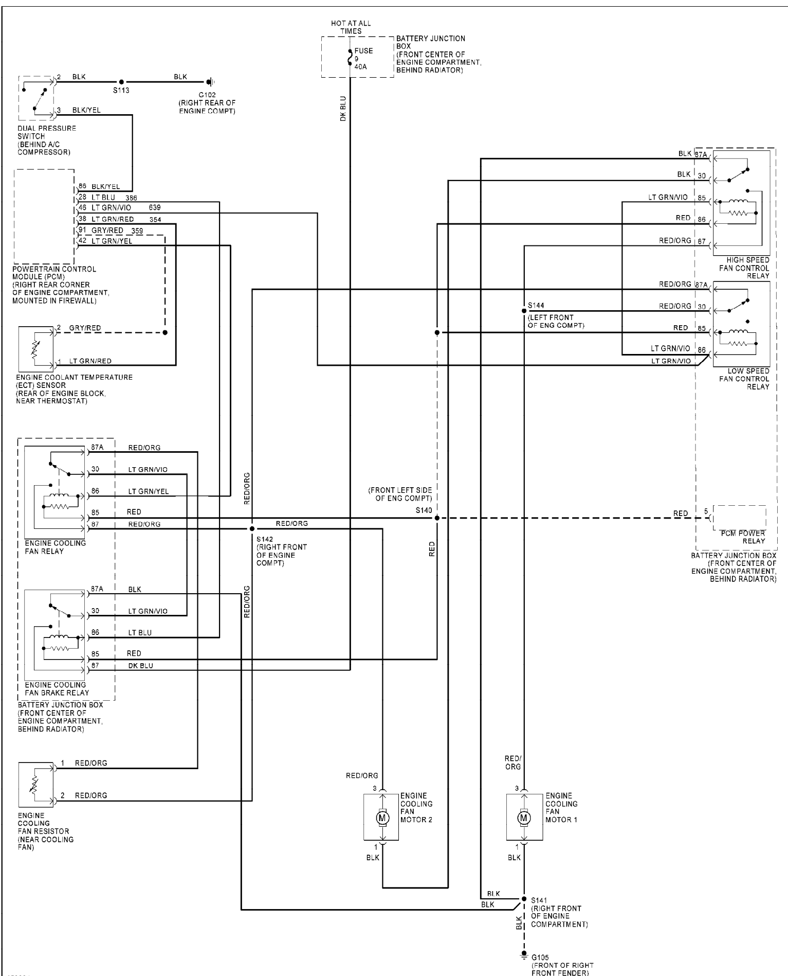
Fig. 11: Cooling Fan Circuit 2002 Ford Taurus SEL
