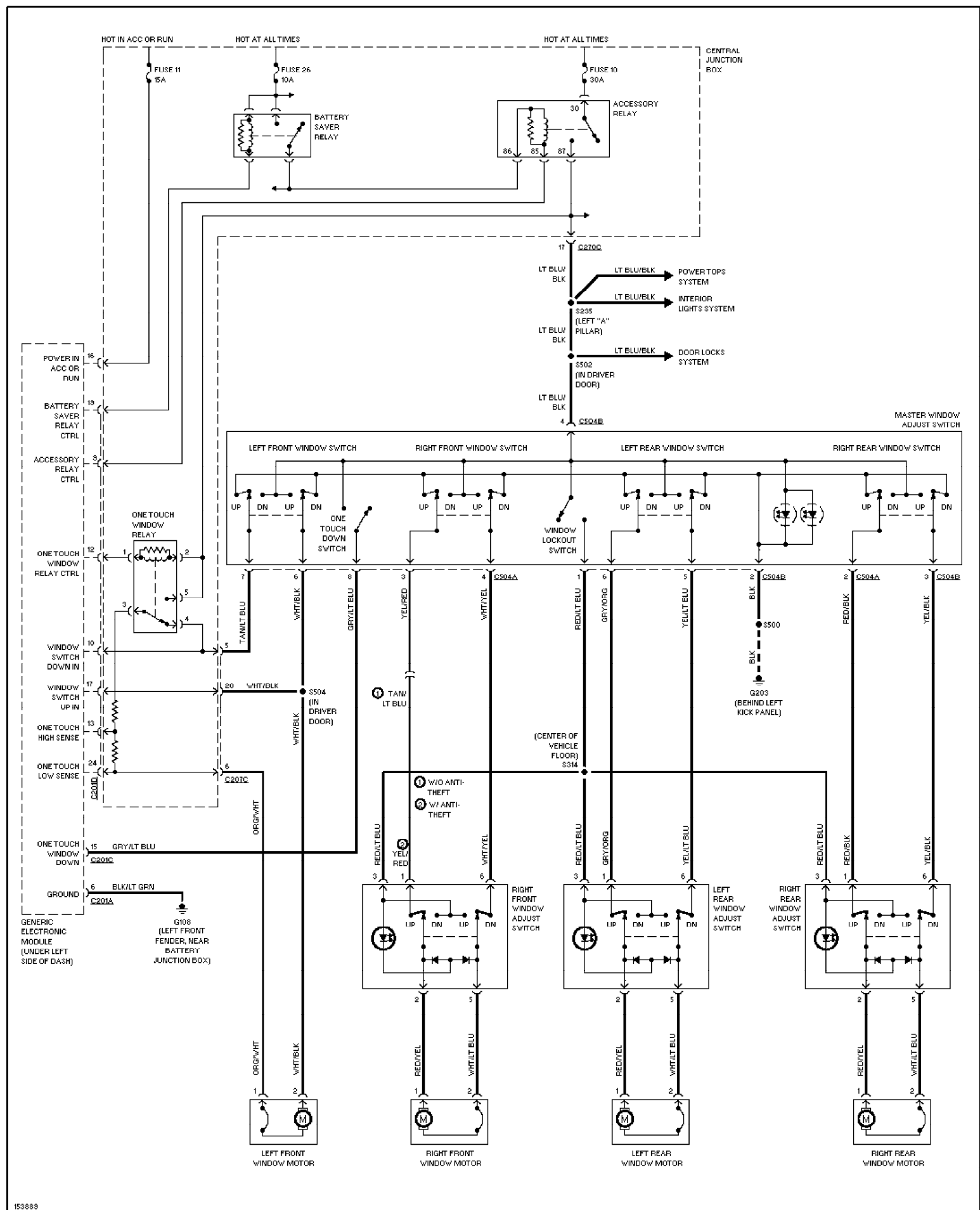
Fig. 52: Power Window Circuit 2002 Ford Taurus SEL
