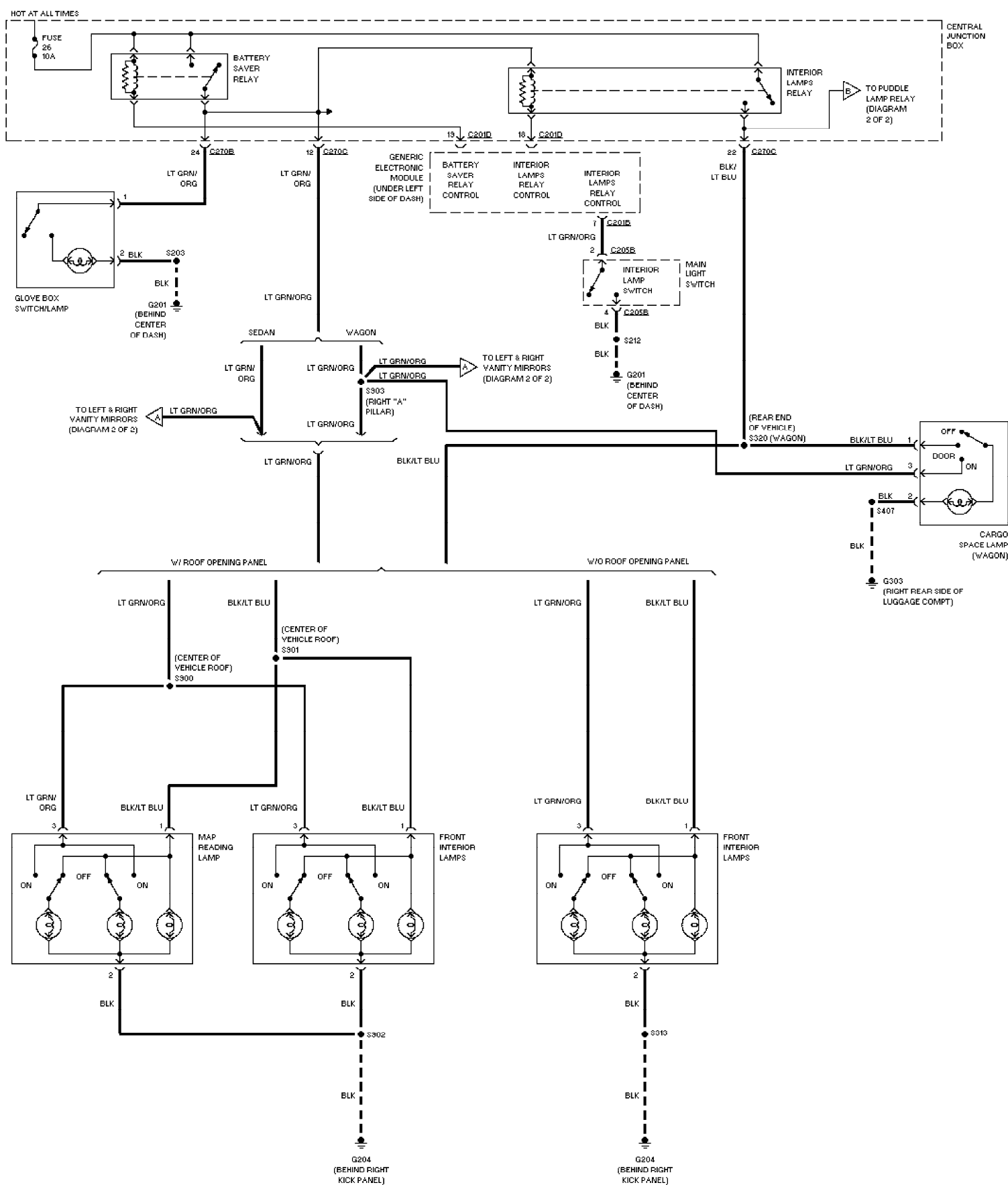
Fig. 38: Courtesy Lamps Circuit (1 of 2) 2002 Ford Taurus SEL
