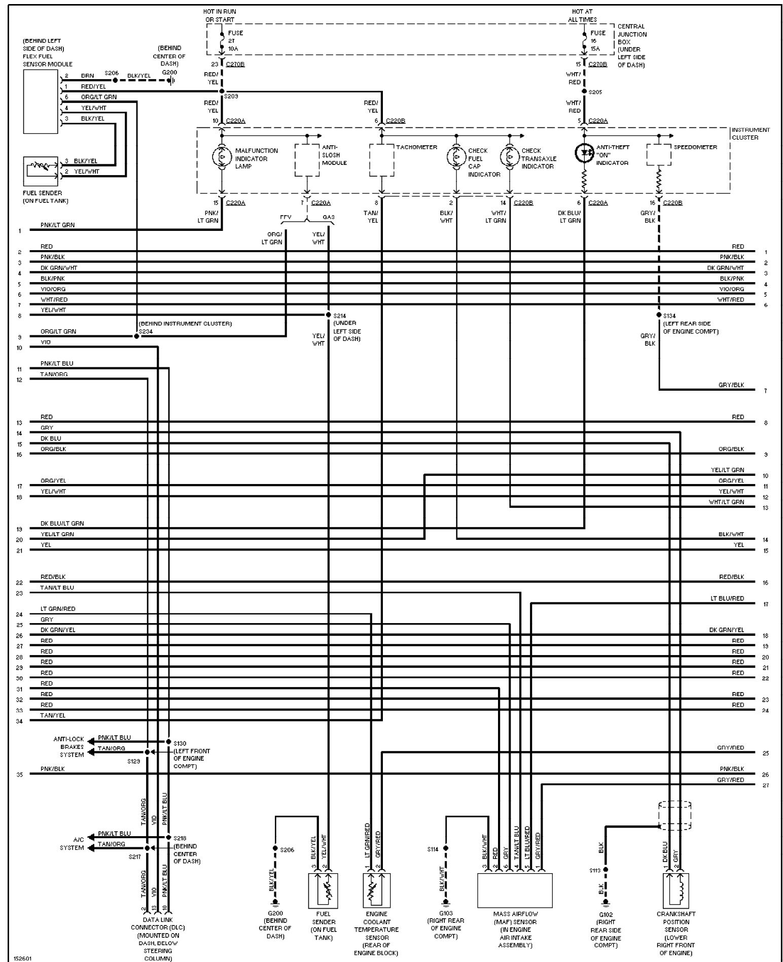
Fig. 23: 3.0L Flex Fuel, Engine Performance Circuits (2 of 4) 2002 Ford Taurus SEL
