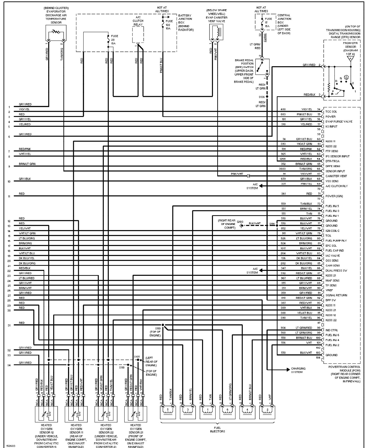
Fig. 25: 3.0L Flex Fuel, Engine Performance Circuits (4 of 4) 2002 Ford Taurus SEL
