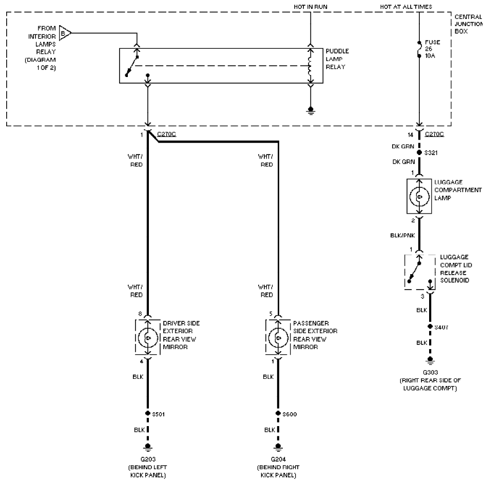
Fig. 39: Courtesy Lamps Circuit (2 of 2) 2002 Ford Taurus SEL
