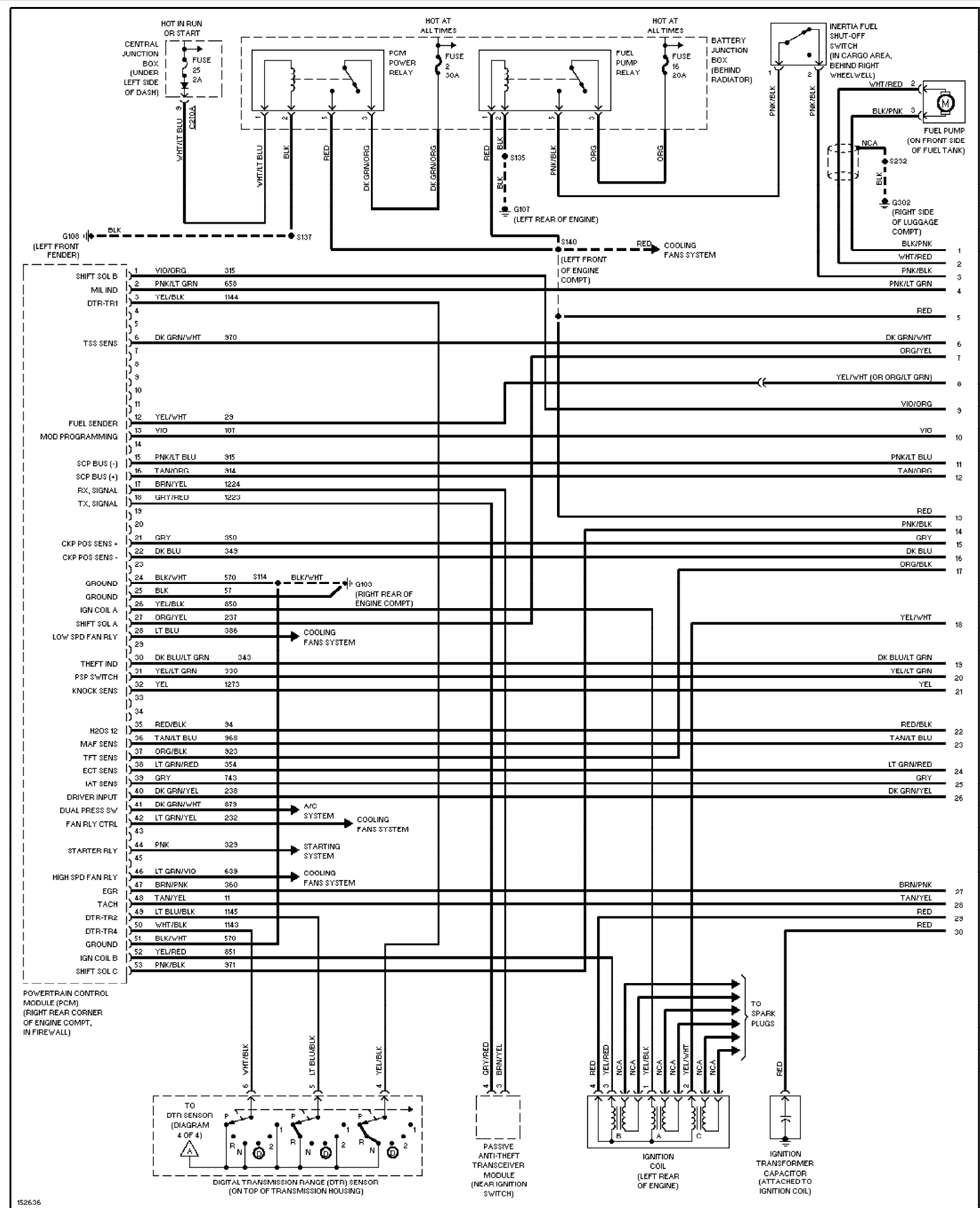
Fig. 18: 3.0L 24-Valve, Engine Performance Circuits (1 of 4)
