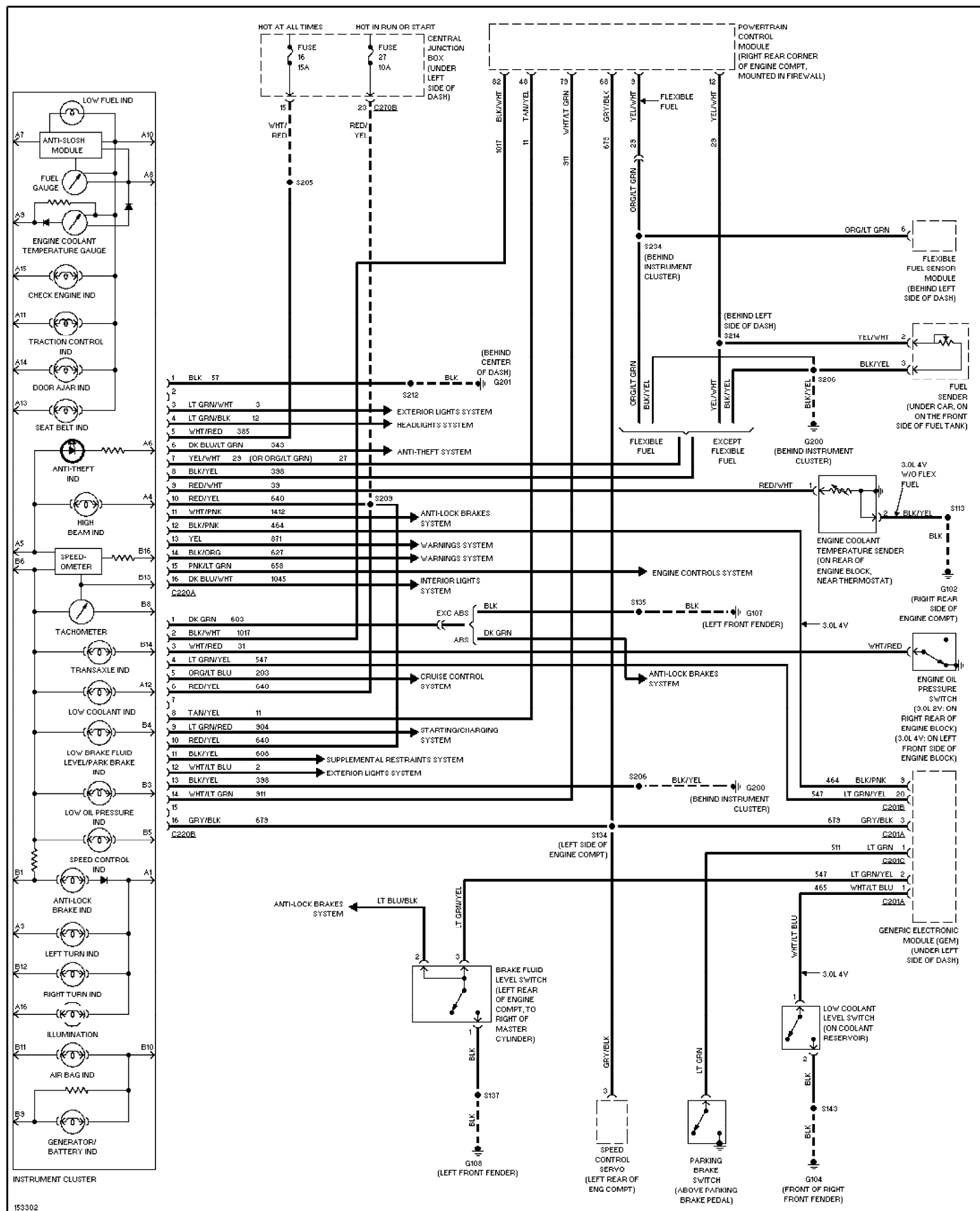
Fig. 37: Instrument Cluster Circuit 2002 Ford Taurus SEL
