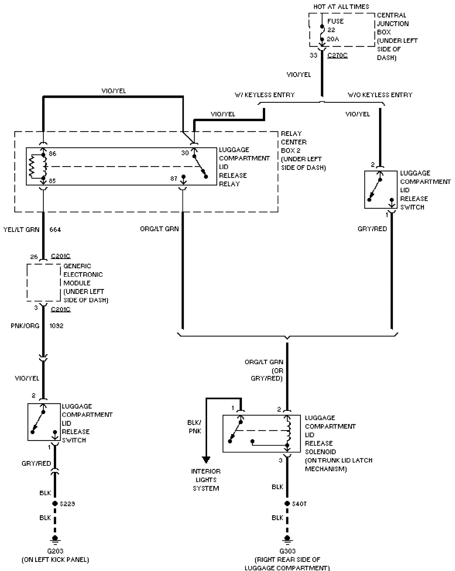
Fig. 62: Trunk Release Circuit 2002 Ford Taurus SEL
