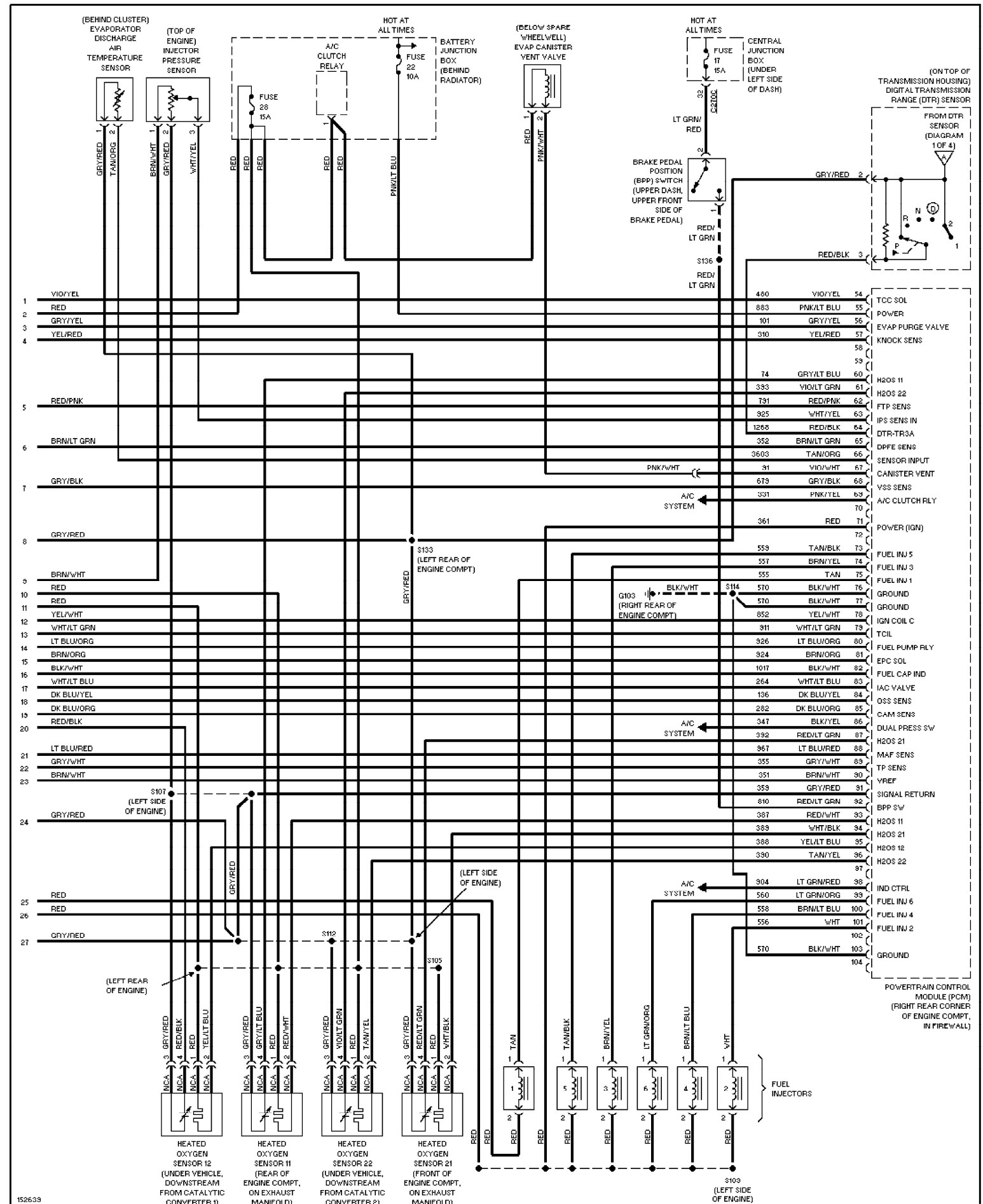
Fig. 21: 3.0L 24-Valve, Engine Performance Circuits (4 of 4)
