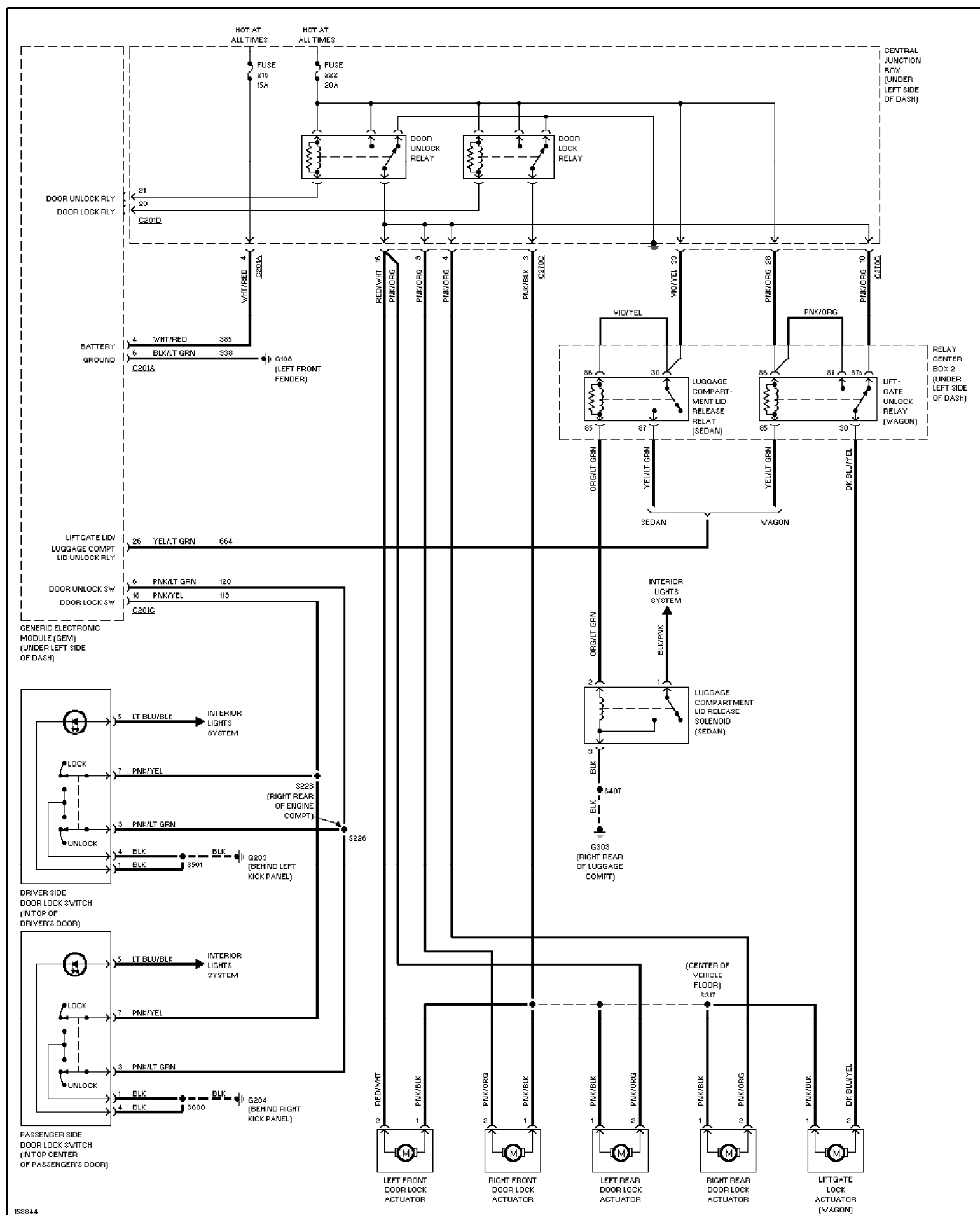
Fig. 46: Power Door Lock Circuit, W/O Keyless Entry 2002 Ford Taurus SEL
