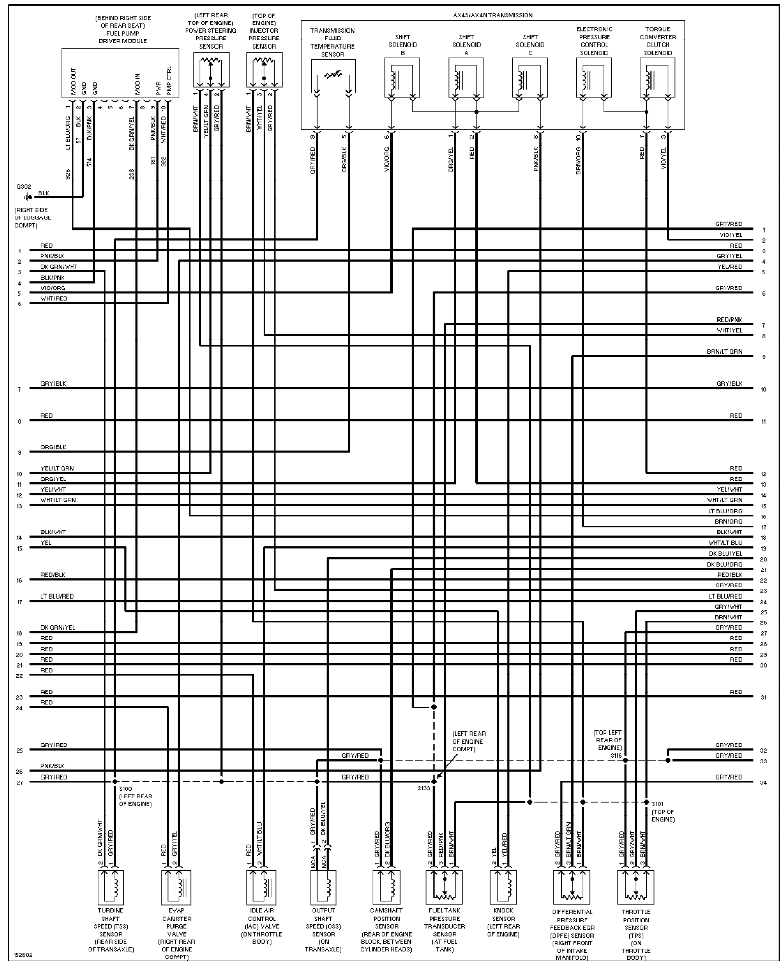
Fig. 16: 3.0L 12-Valve, Engine Performance Circuits (3 of 4)
