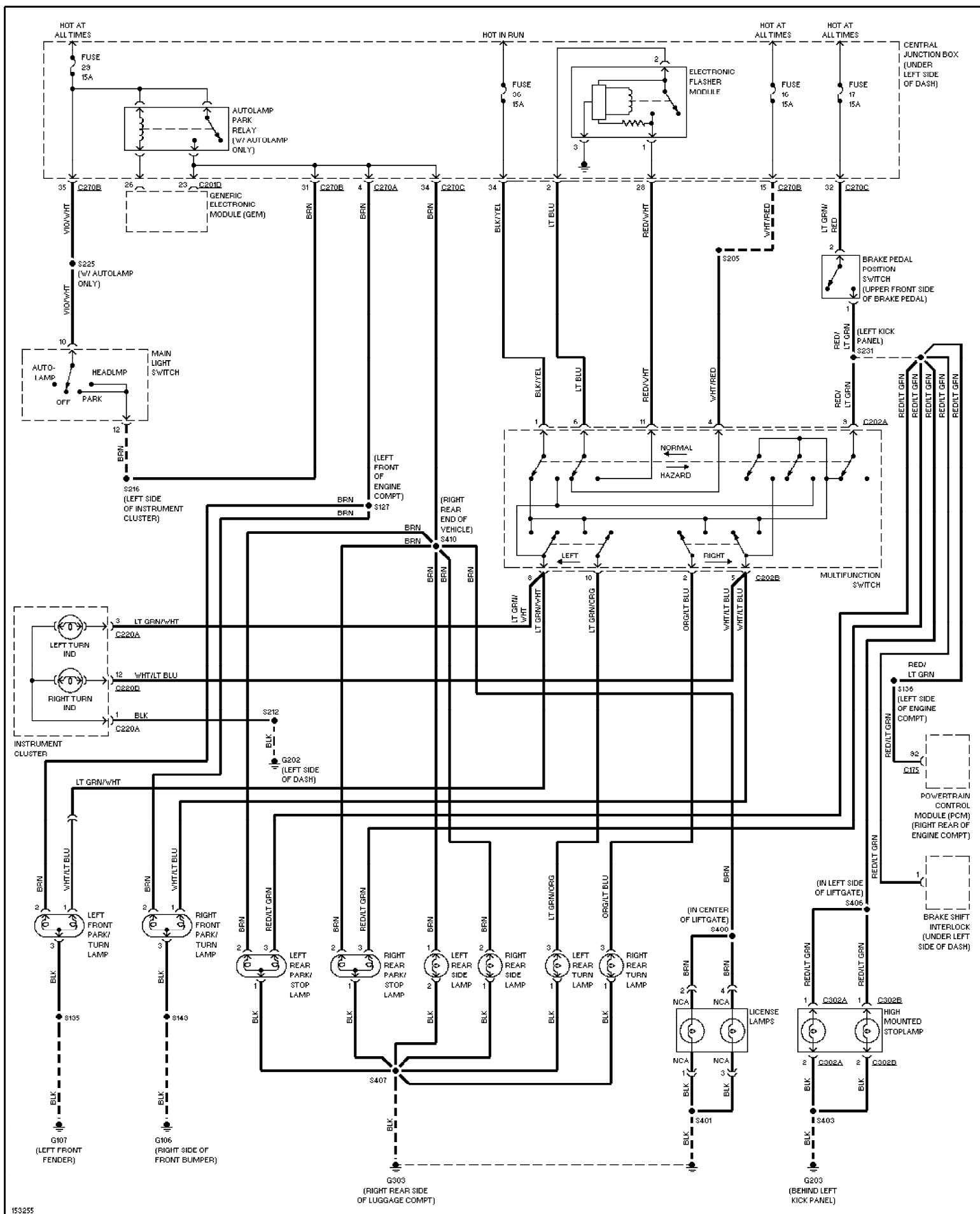
Fig. 28: Exterior Lamps Circuit, Wagon 2002 Ford Taurus SEL
