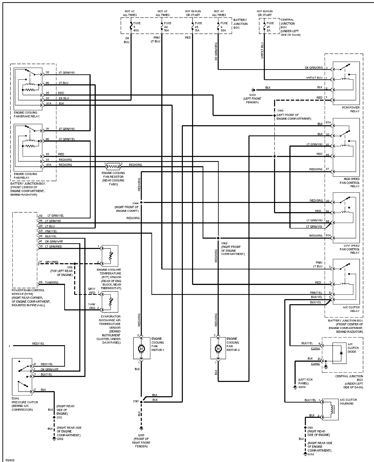
Fig. 4: Manual A/C Circuit (2 of 2) 2002 Ford Taurus SEL
