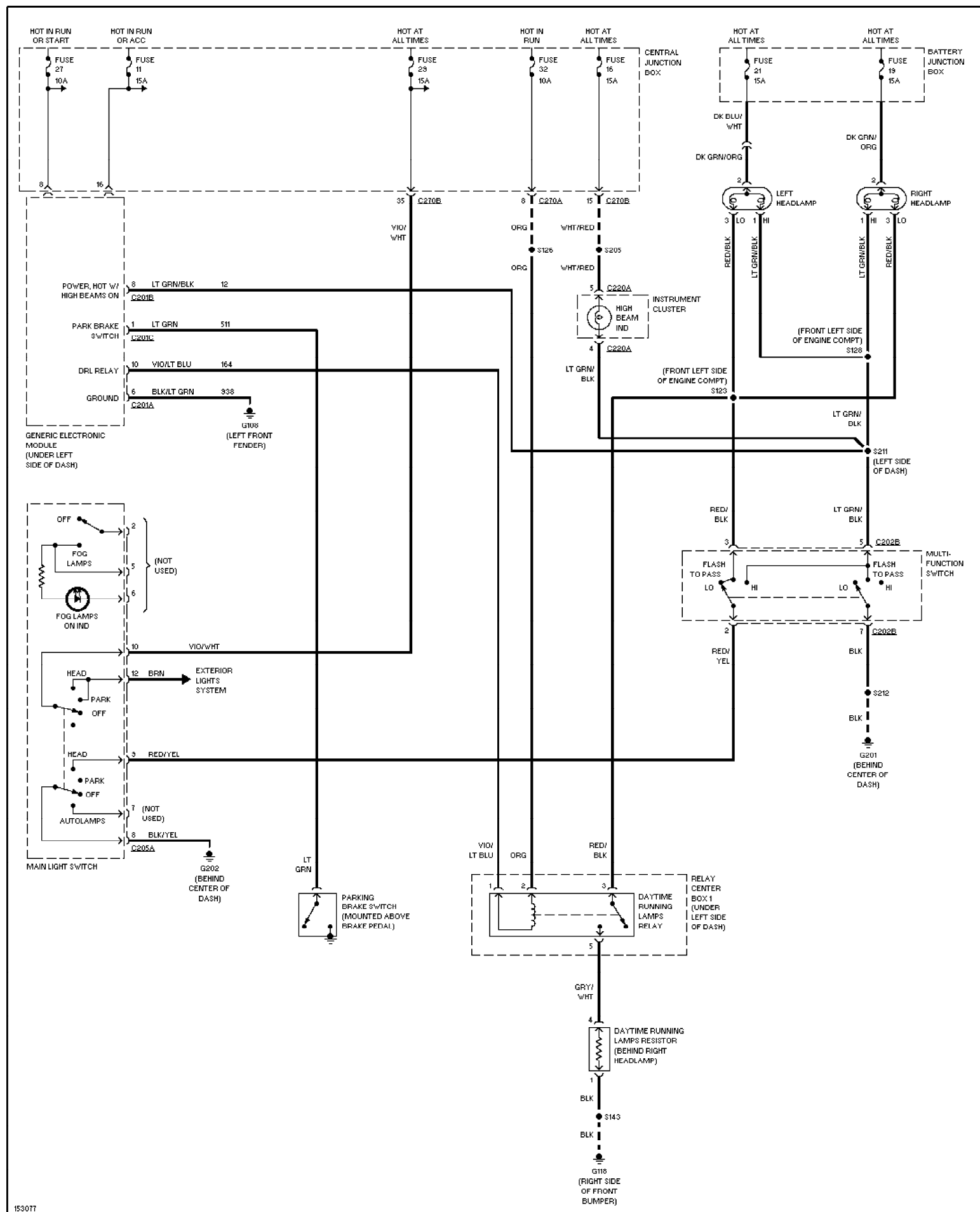
Fig. 34: Headlamps Circuit, W/ DRL 2002 Ford Taurus SEL
