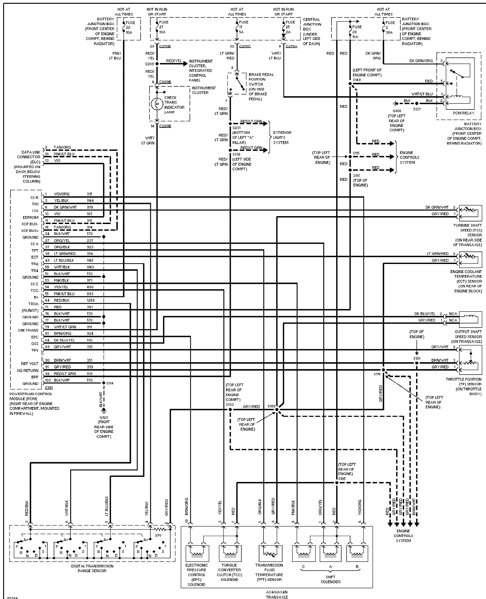
Fig. 59: 3.0L 12-Valve, A/T Circuit 2002 Ford Taurus SEL
